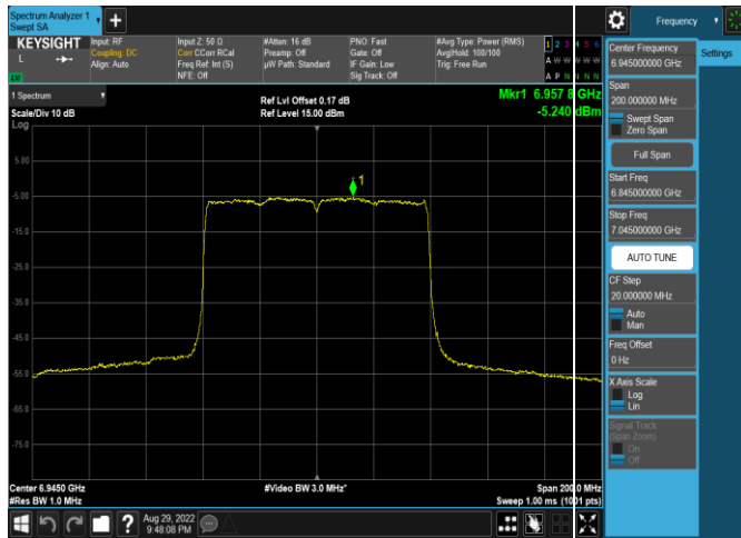
Plot 7-139. Power Spectral Density Plot Antenna WF5t (80MHz 802.11ax (UNII Band 8) – Ch. 199, MCS2)
