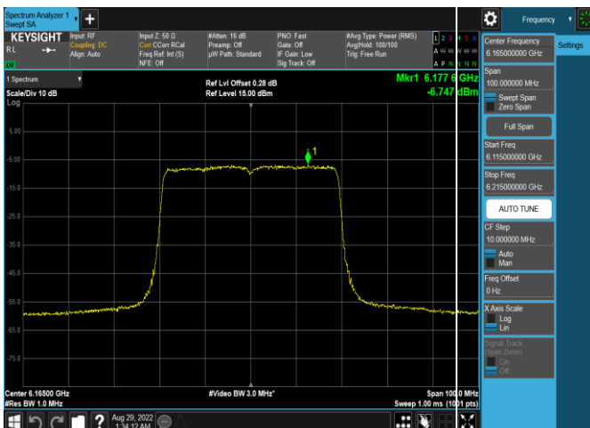
Plot 7-123. Power Spectral Density Plot Antenna WF5t (40MHz 802.11ax (UNII Band 5) – Ch. 43, MCS2)
