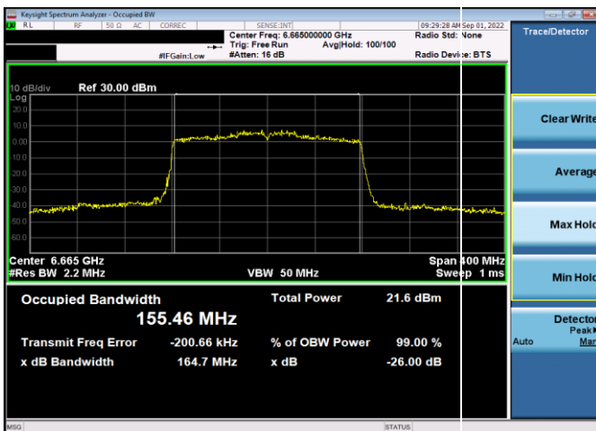
Plot 7-75. 26dB & 99% Bandwidth Plot Antenna WF5b (160MHz) 802.11ax (UNII Band 7) – Ch. 143, MCS2)
