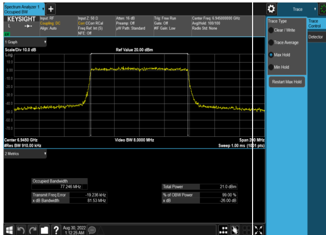
Plot 7-79. 26dB & 99% Bandwidth Plot Antenna WF5b (80MHz 802.11ax (UNII Band 8) – Ch. 199, MCS2)
