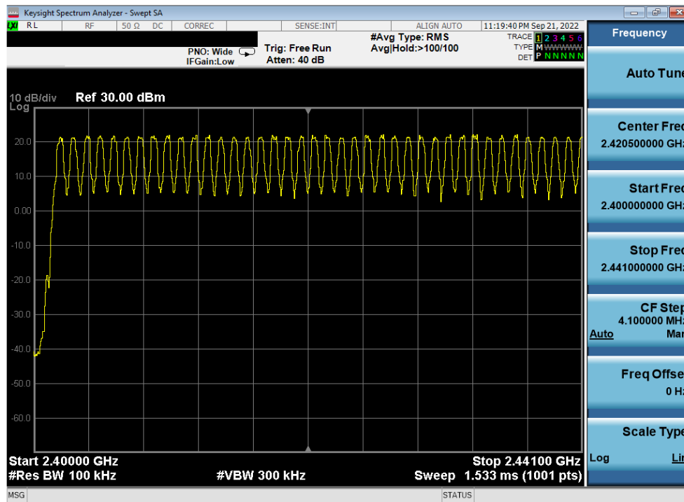
Plot 7-41. Low End Spectrum Channel Hopping Plot Antenna WF7 (Bluetooth, GFSK, ePA, 2.4GHz)
