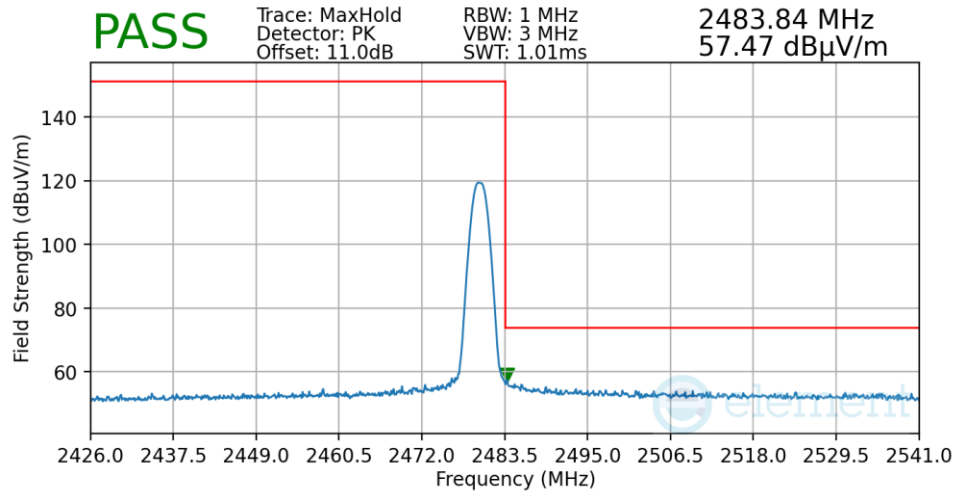
Plot 7-78. Radiated Restricted Upper Band Edge Measurement TxBF, 2.4GHz
