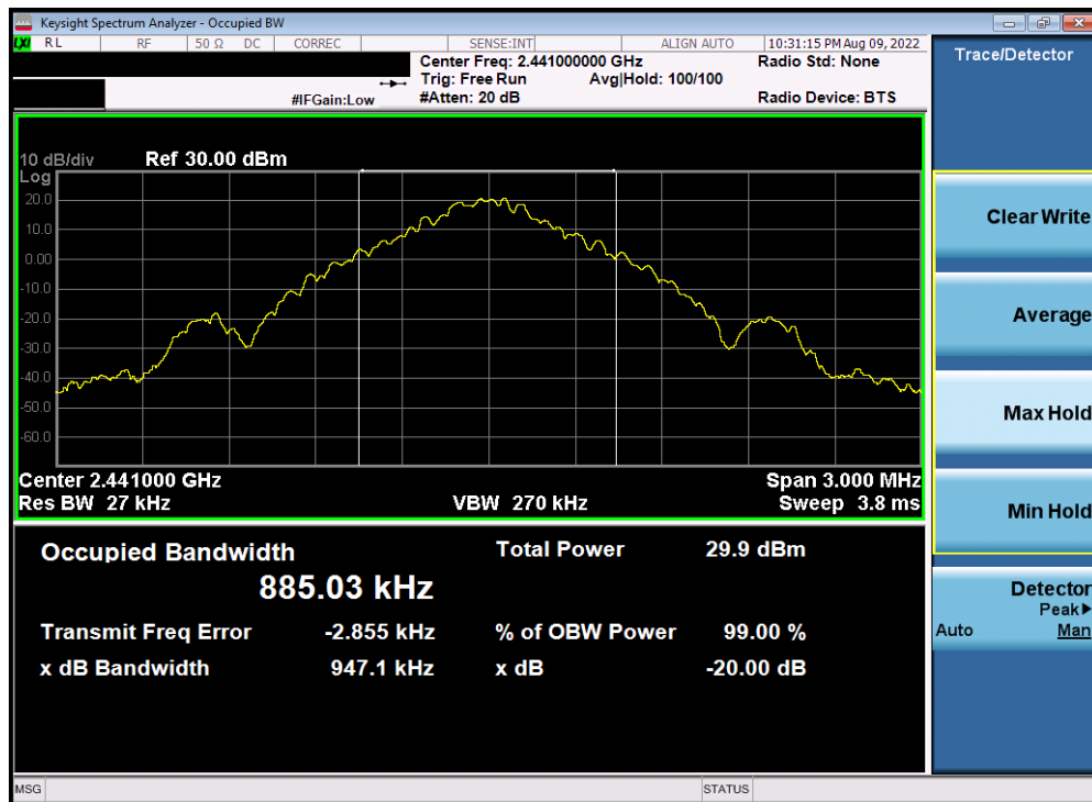
Plot 7-2. 20dB BW and 99% OBW Plot Antenna WF8 (Bluetooth, GFSK, ePA – 2441 MHz)
