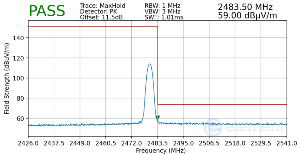
Plot 7-71. Radiated Restricted Upper Band Edge Measurement Antenna WF8
