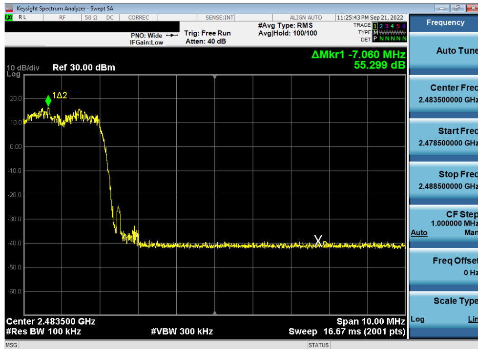
Plot 7-28. Band Edge Plot Antenna WF7 (Bluetooth with Hopping Enabled, 8DPSK, ePA, 2.4GHz)
