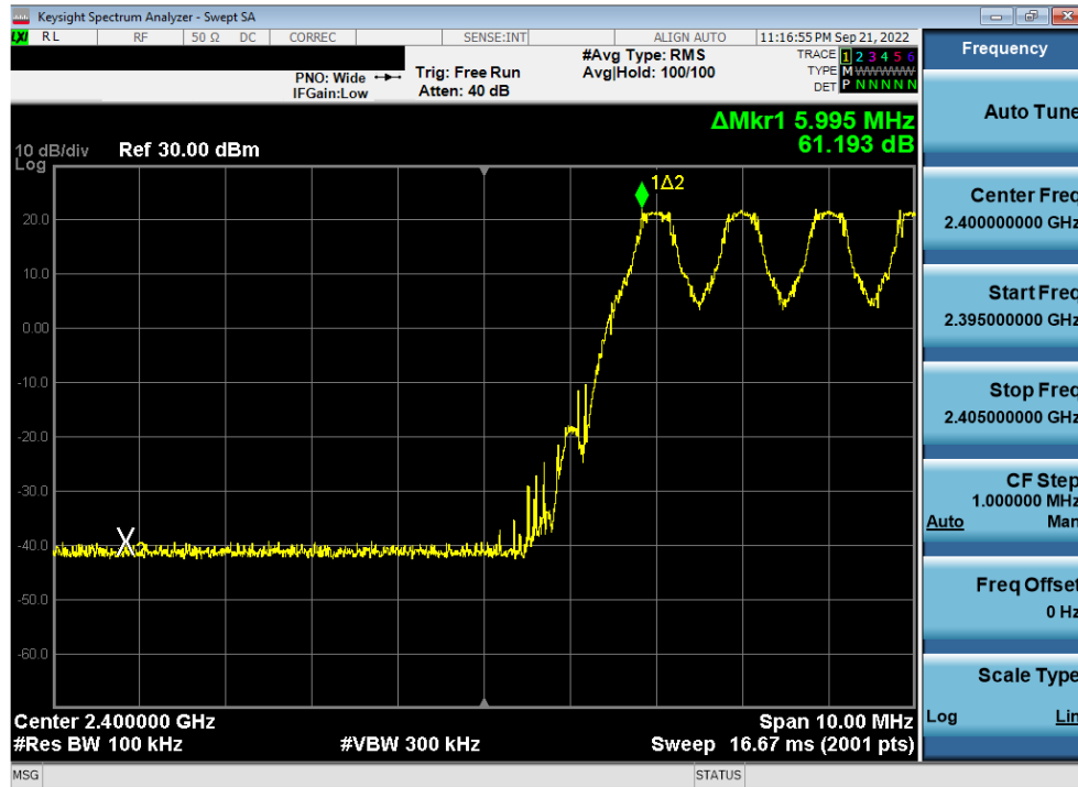
Plot 7-23. Band Edge Plot Antenna WF7 (Bluetooth with Hopping Enabled, GFSK, ePA, 2.4GHz)
