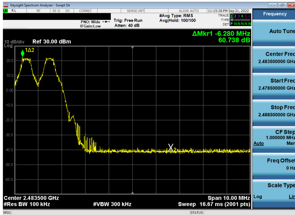
Plot 7-24. Band Edge Plot Antenna WF7 (Bluetooth with Hopping Enabled, GFSK, ePA, 2.4GHz)
