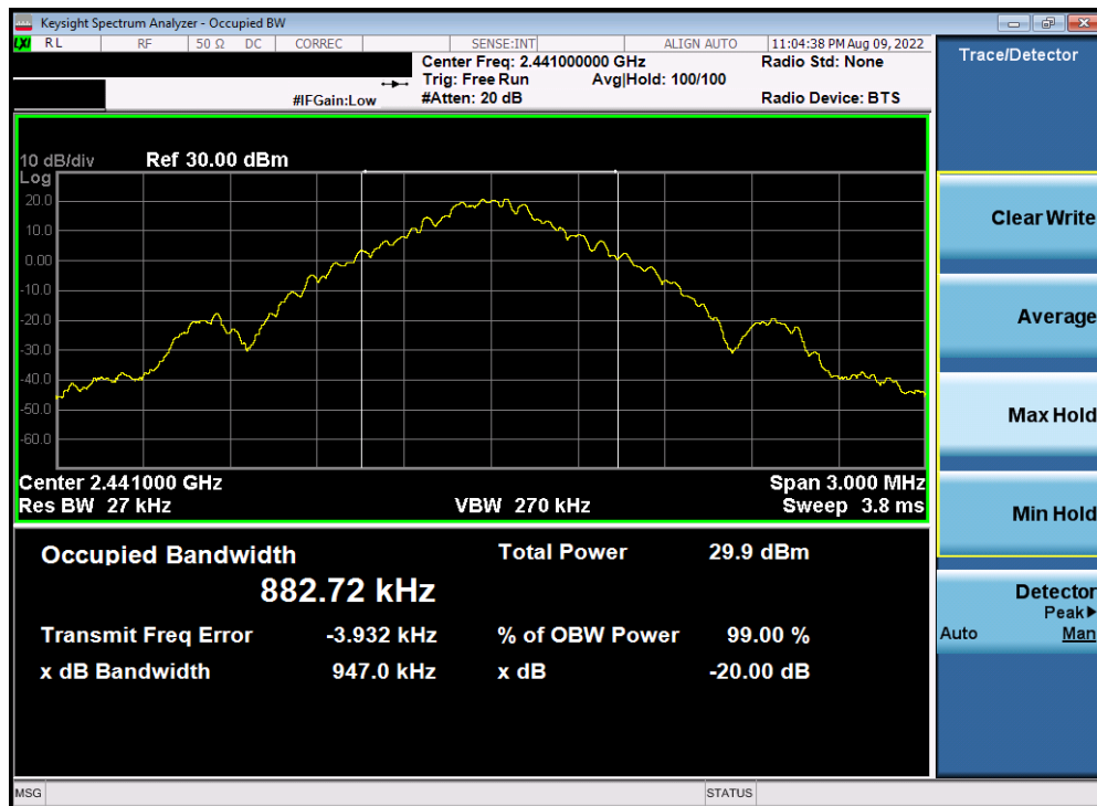
Plot 7-8. 20dB BW and 99% OBW Plot Antenna WF7 (Bluetooth, GFSK, ePA – 2441 MHz)
