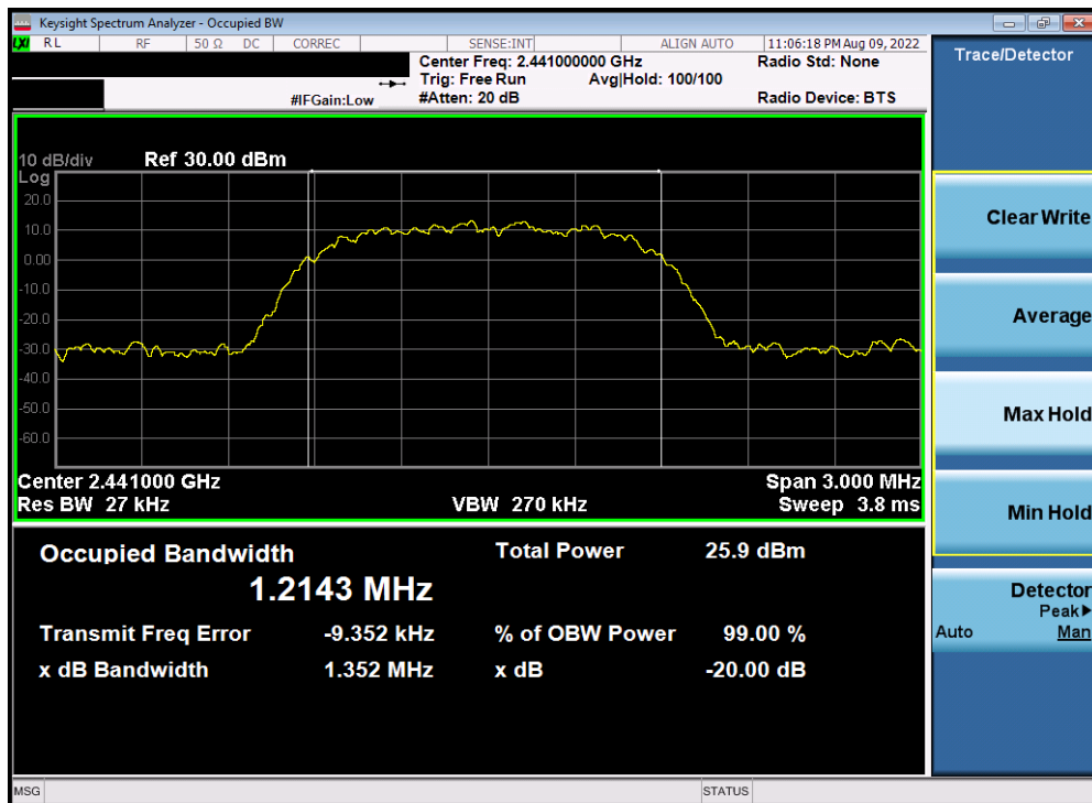
Plot 7-11. 20dB BW and 99% OBW Plot Antenna WF7 (Bluetooth, 8DPSK, ePA – 2441 MHz)
