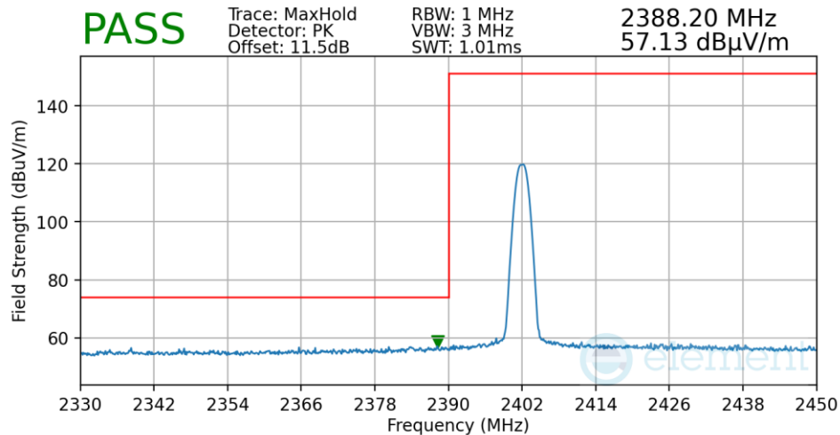
Plot 7-76. Radiated Restricted Lower Band Edge Measurement TxBF, 2.4GHz
