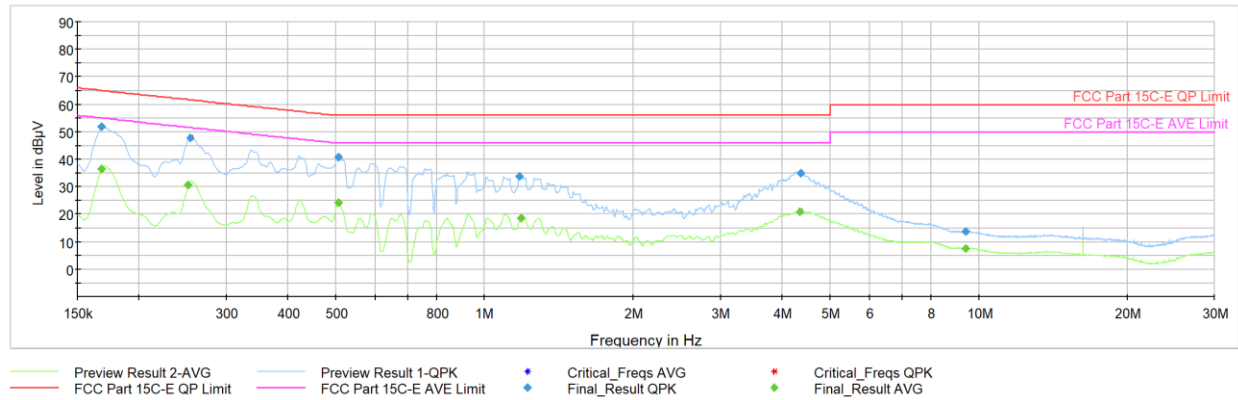
Plot 7-81. AC Line-Conducted Test Plot TxBF, 2.4GHz (L1, GFSK ePA – 2480 MHz, with AC/DC Adapter)
