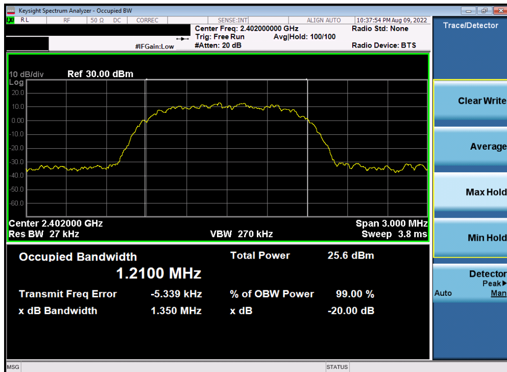
Plot 7-4. 20dB BW and 99% OBW Plot Antenna WF8 (Bluetooth, 8DPSK, ePA – 2402 MHz)
