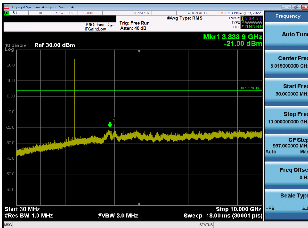
Plot 7-51. Conducted Spurious Plot Antenna WF7 (Bluetooth, GFSK, ePA – 2402 MHz)
