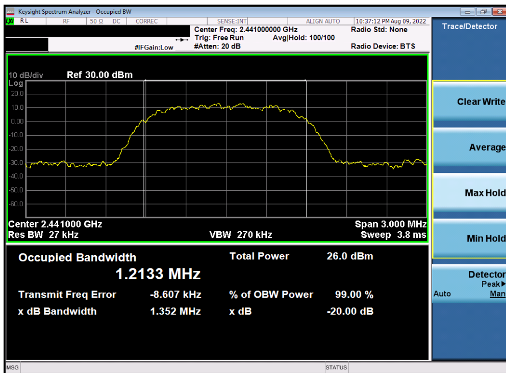
Plot 7-5. 20dB BW and 99% OBW Plot Antenna WF8 (Bluetooth, 8DPSK, ePA – 2441 MHz)
