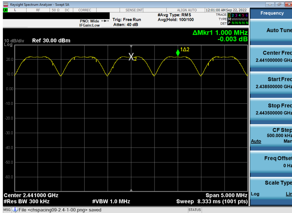
Plot 7-29. Channel Spacing Plot Antenna WF8 (Bluetooth, GFSK, ePA, 2.4GHz)
