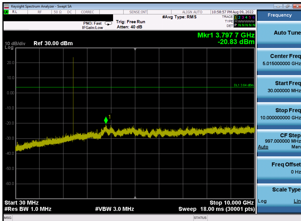
Plot 7-47. Conducted Spurious Plot Antenna WF8 (Bluetooth, GFSK, ePA – 2441 MHz)
