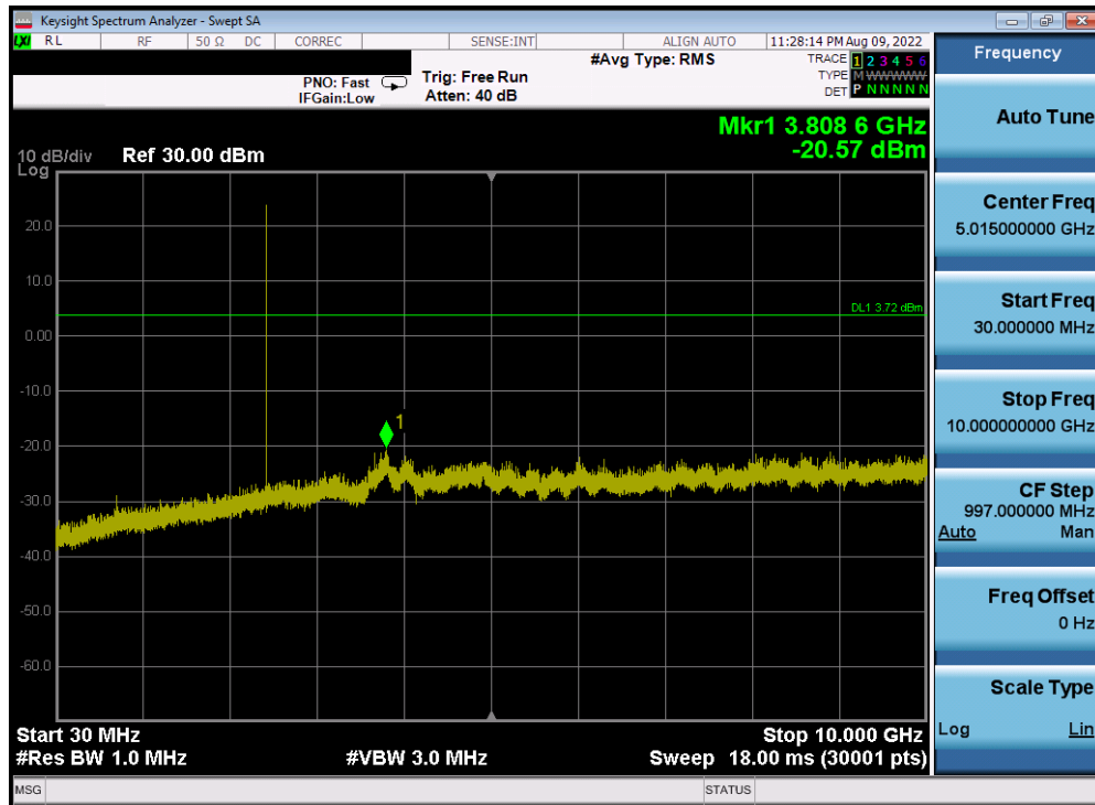
Plot 7-53. Conducted Spurious Plot Antenna WF7 (Bluetooth, GFSK, ePA – 2441 MHz)
