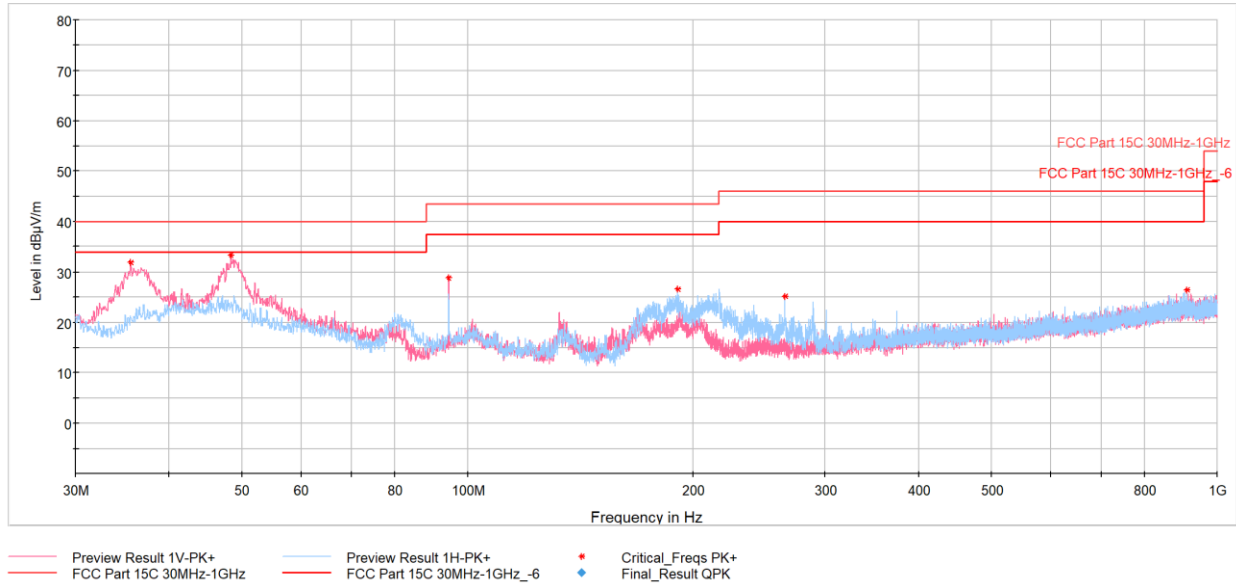
Plot 7-80. Radiated Spurious Emissions Below 1GHz TxBF, 2.4GHz (GFSK ePA – 2480 MHz, with AC/DC Adapter)
