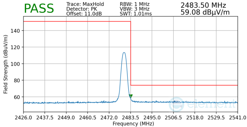
Plot 7-74. Radiated Restricted Upper Band Edge Measurement Antenna WF7
