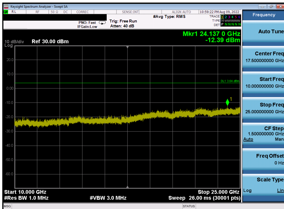
Plot 7-48. Conducted Spurious Plot Antenna WF8 (Bluetooth, GFSK, ePA 2441 MHz)
