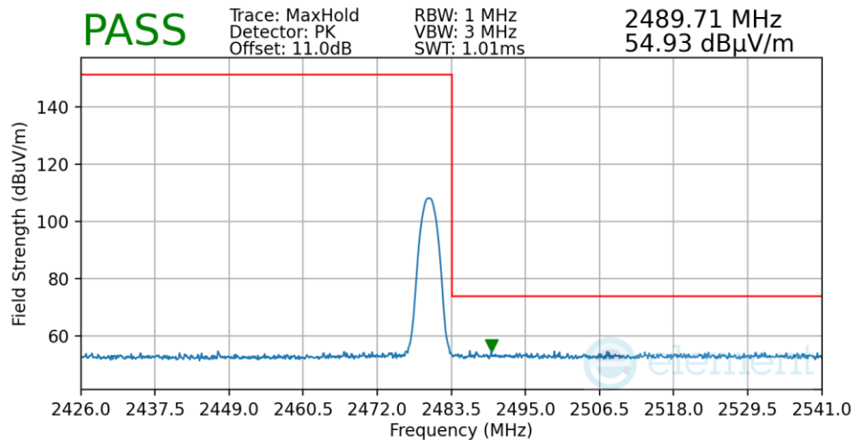
Plot 7-75. Radiated Restricted Upper Band Edge Measurement Antenna WF7
