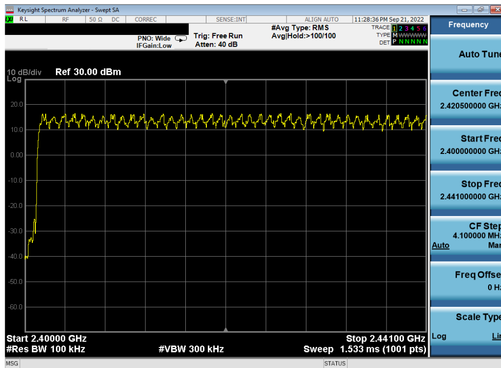
Plot 7-43. Low End Spectrum Channel Hopping Plot Antenna WF7 (Bluetooth, 8DPSK, ePA, 2.4GHz)
