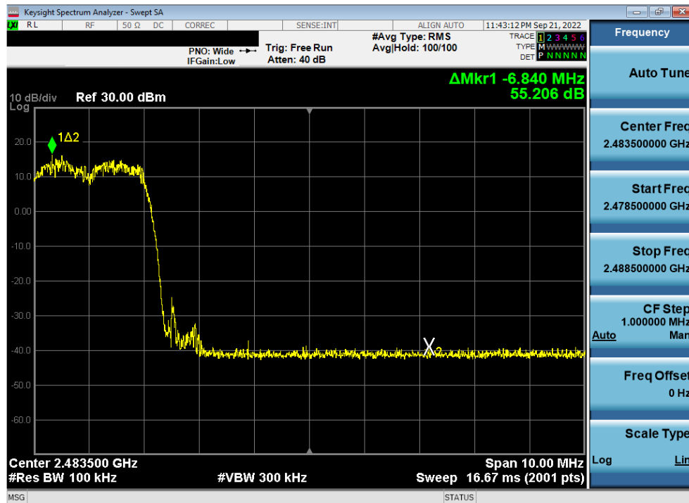
Plot 7-20. Band Edge Plot Antenna WF8 (Bluetooth with Hopping Enabled, 8DPSK, ePA, 2.4GHz)
