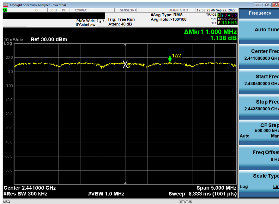
Plot 7-30. Channel Spacing Plot Antenna WF8 (Bluetooth, 8DPSK, ePA, 2.4GHz)
