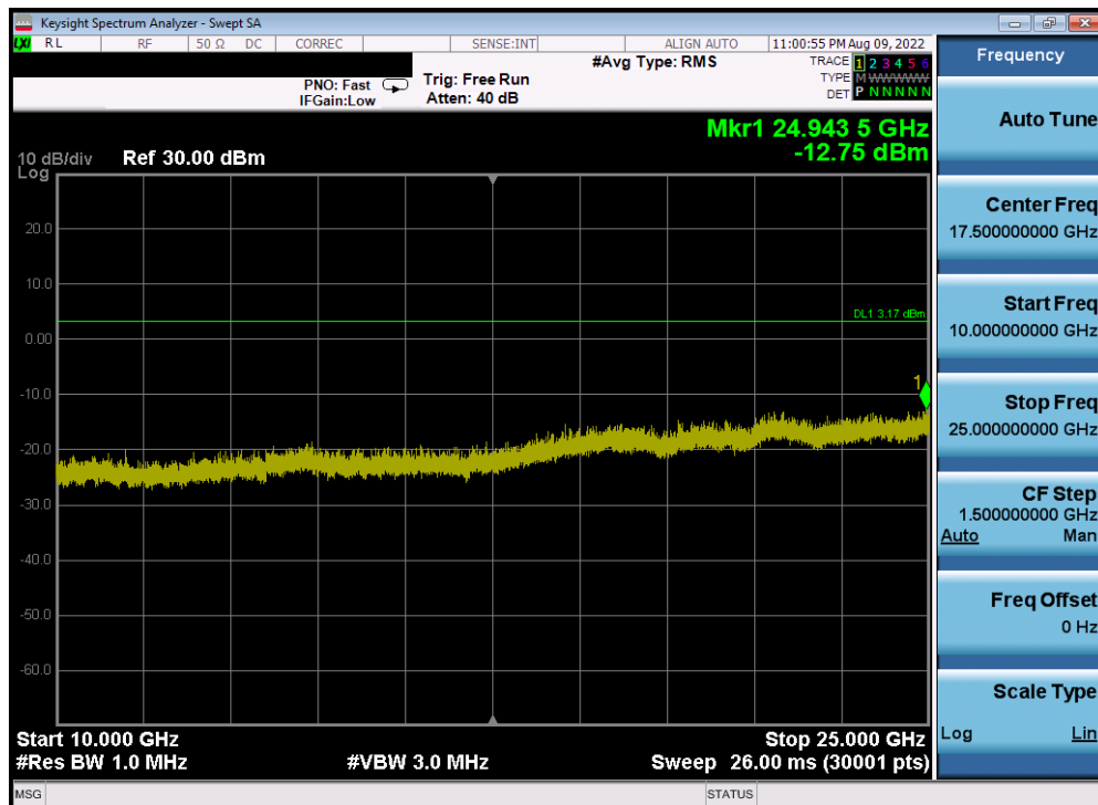
Plot 7-50. Conducted Spurious Plot Antenna WF8 (Bluetooth, GFSK, ePA – 2480 MHz)
