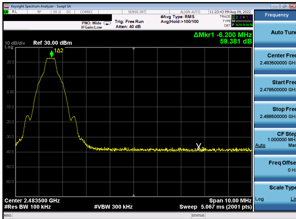
Plot 7-22. Band Edge Plot Antenna WF7 (Bluetooth with Hopping Disabled, GFSK, ePA – 2480 MHz)
