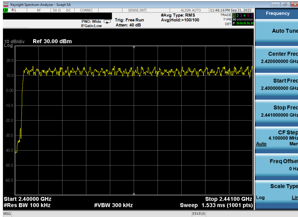
Plot 7-39. Low End Spectrum Channel Hopping Plot Antenna WF8 (Bluetooth, 8DPSK, ePA, 2.4GHz)
