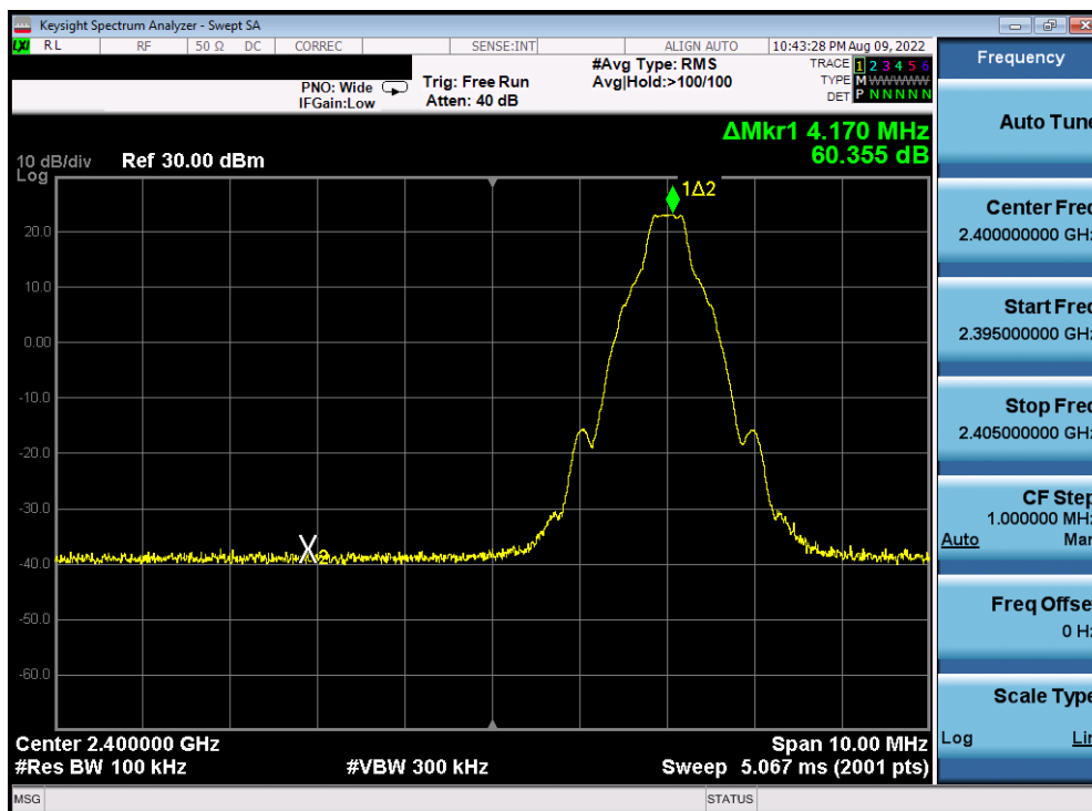
Plot 7-13. Band Edge Plot Antenna WF8 (Bluetooth with Hopping Disabled, GFSK, ePA – 2402 MHz)
