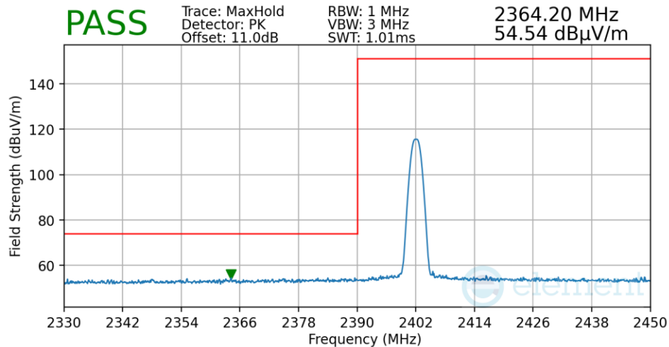
Plot 7-68. Radiated Restricted Lower Band Edge Measurement Antenna WF8
