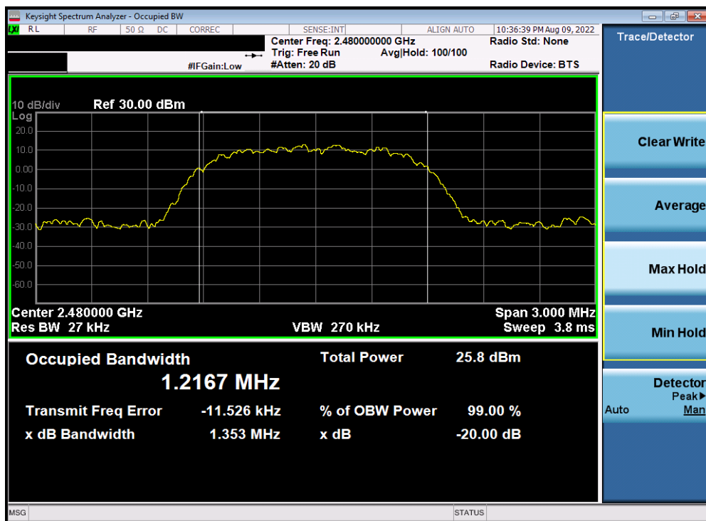
Plot 7-6. 20dB BW and 99% OBW Plot Antenna WF8 (Bluetooth, 8DPSK, ePA – 2480 MHz)
