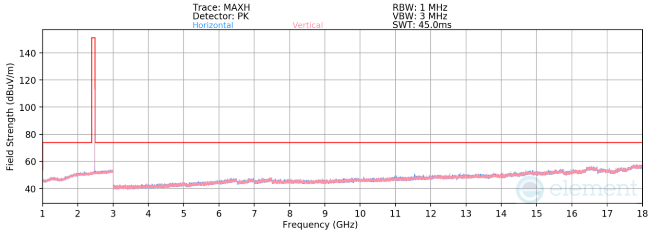
Plot 7-59. Radiated Spurious Emissions 1-18GHz Antenna WF8 (BT GFSK ePA – 2480 MHz)
