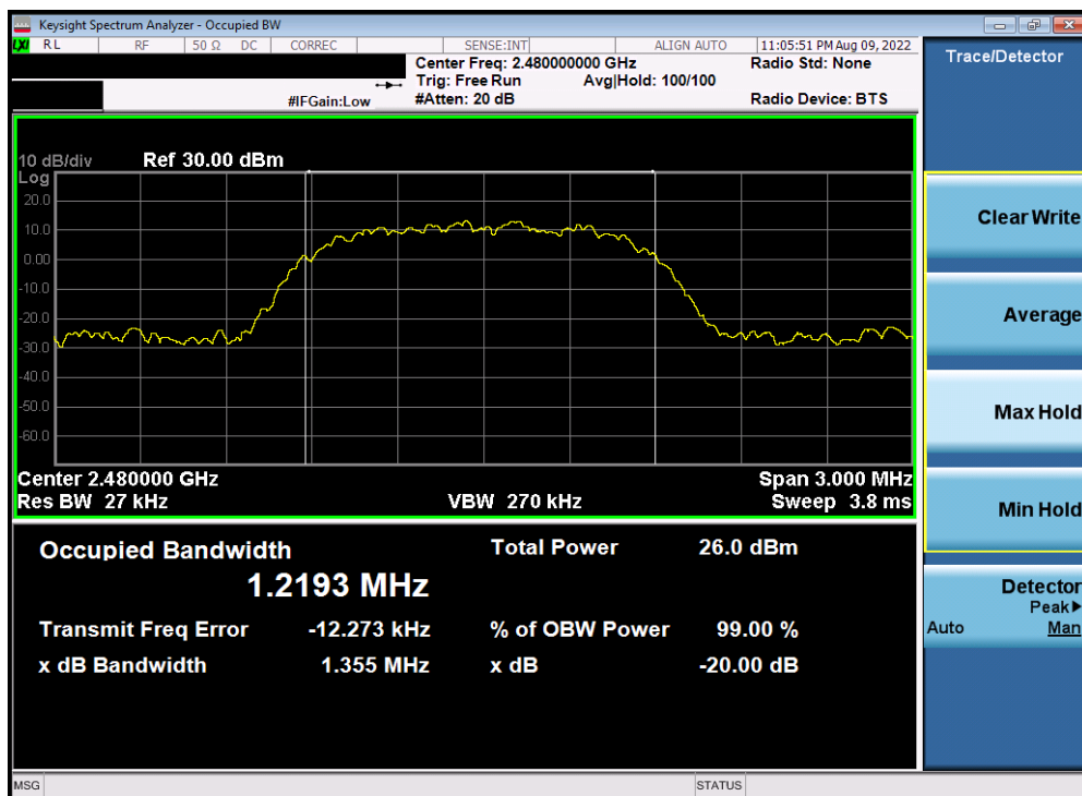
Plot 7-12. 20dB BW and 99% OBW Plot Antenna WF7 (Bluetooth, 8DPSK, ePA – 2480 MHz)
