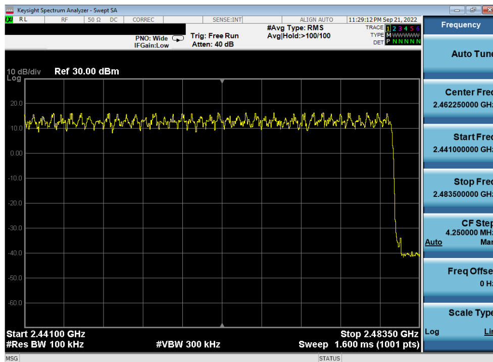
Plot 7-44. High End Spectrum Channel Hopping Plot Antenna WF7 (Bluetooth, 8DPSK, ePA, 2.4GHz)
