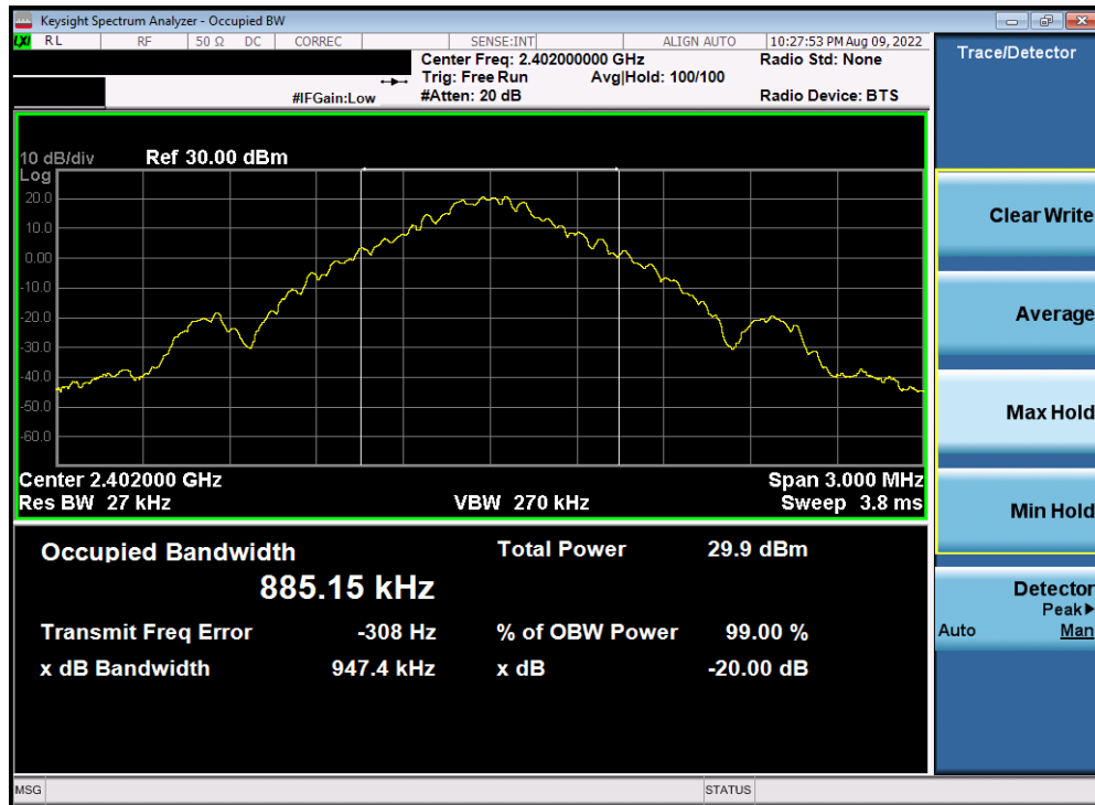
Plot 7-1. 20dB BW and 99% OBW Plot Antenna WF8 (Bluetooth, GFSK, ePA – 2402 MHz)
