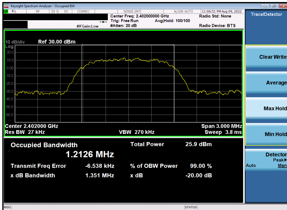
Plot 7-10. 20dB BW and 99% OBW Plot Antenna WF7 (Bluetooth, 8DPSK, ePA – 2402 MHz)
