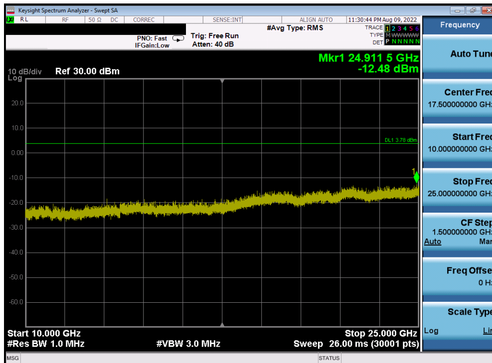
Plot 7-52. Conducted Spurious Plot Antenna WF7 (Bluetooth, GFSK, ePA – 2402 MHz)
