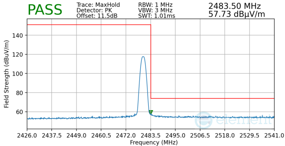
Plot 7-70. Radiated Restricted Upper Band Edge Measurement Antenna WF8
