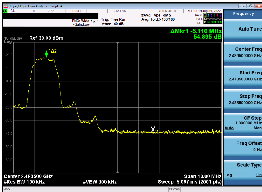
Plot 7-26. Band Edge Plot Antenna WF7 (Bluetooth with Hopping Disabled, 8DPSK, ePA – 2480 MHz)
