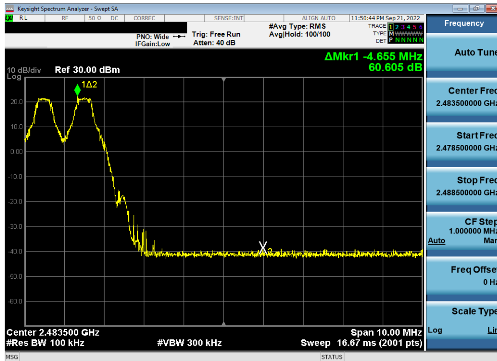
Plot 7-16. Band Edge Plot Antenna WF8 (Bluetooth with Hopping Enabled, GFSK, ePA, 2.4GHz)
