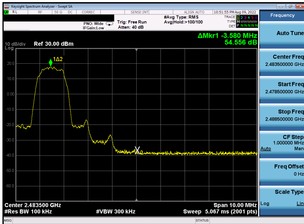
Plot 7-18. Band Edge Plot Antenna WF8 (Bluetooth with Hopping Disabled, 8DPSK, ePA – 2480 MHz)
