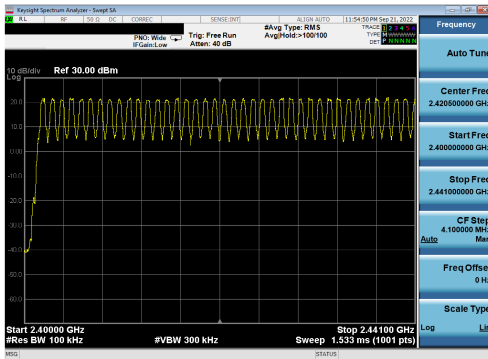
Plot 7-37. Low End Spectrum Channel Hopping Plot Antenna WF8 (Bluetooth, GFSK, ePA, 2.4GHz)
