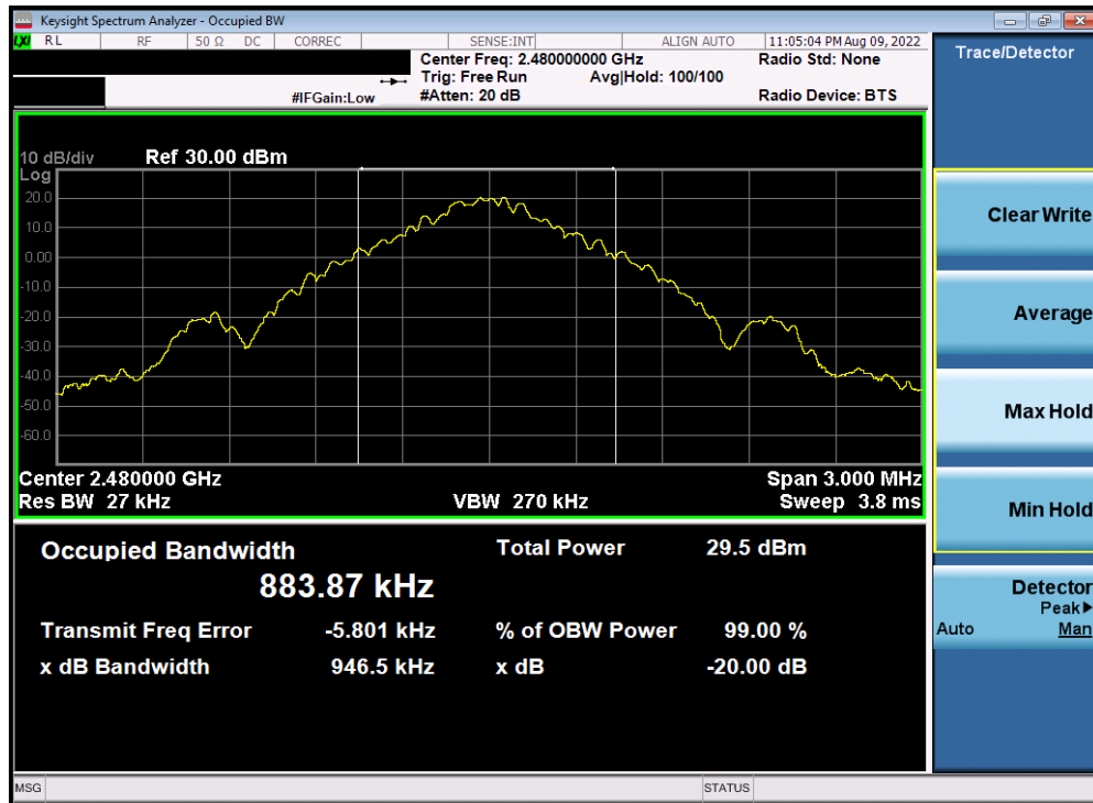
Plot 7-9. 20dB BW and 99% OBW Plot Antenna WF7 (Bluetooth, GFSK, ePA – 2480 MHz)
