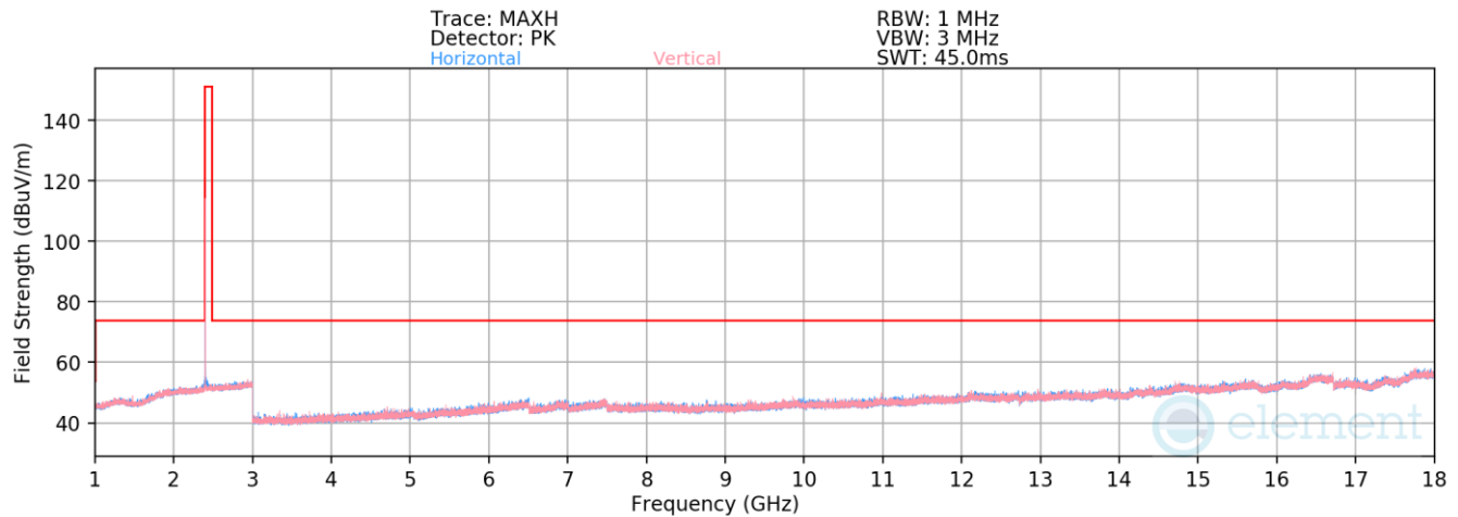
Plot 7-60. Radiated Spurious Emissions 1-18GHz Antenna WF7 (BT GFSK ePA – 2402 MHz)
