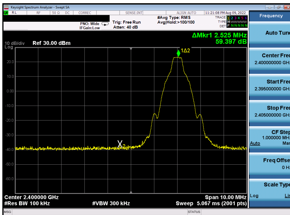
Plot 7-21. Band Edge Plot Antenna WF7 (Bluetooth with Hopping Disabled, GFSK, ePA – 2402 MHz)
