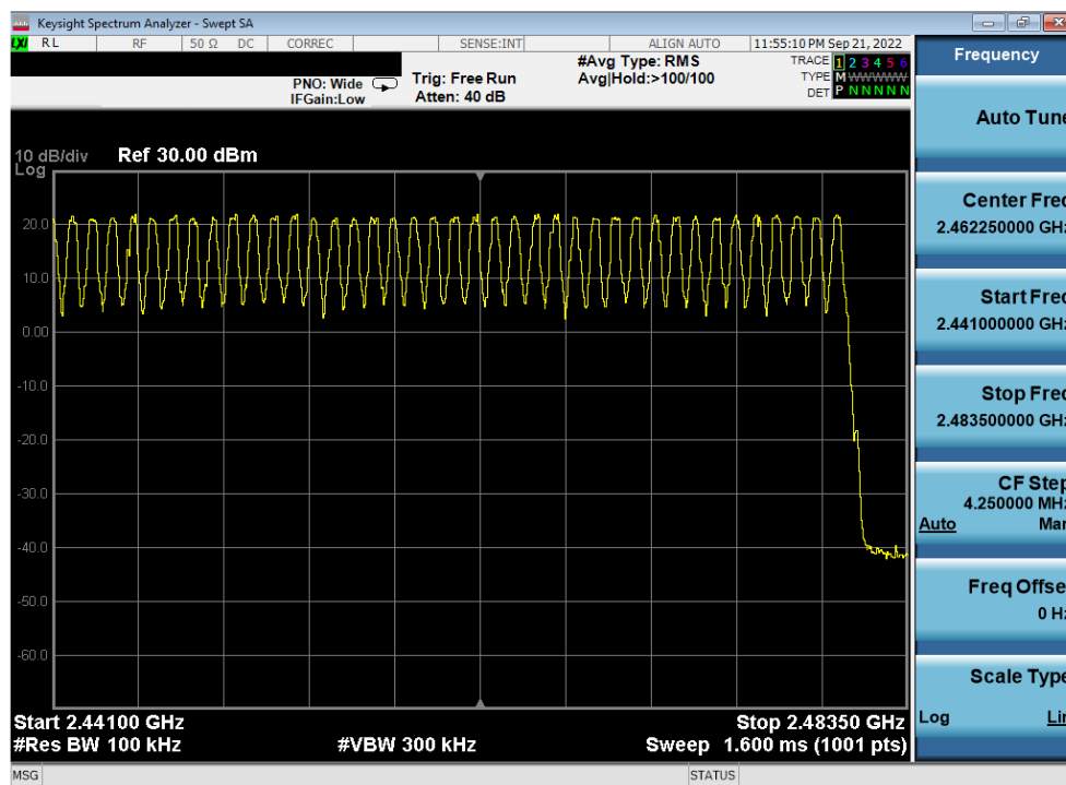
Plot 7-38. High End Spectrum Channel Hopping Plot Antenna WF8 (Bluetooth, GFSK, ePA, 2.4GHz)
