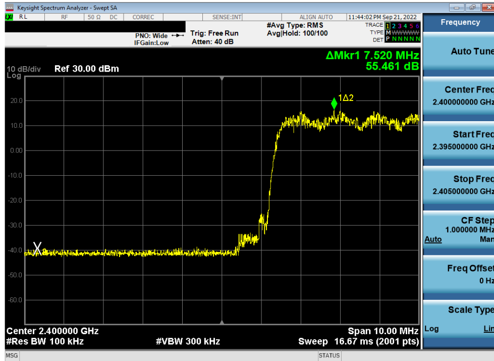
Plot 7-19. Band Edge Plot Antenna WF8 (Bluetooth with Hopping Enabled, 8DPSK, ePA, 2.4GHz)
