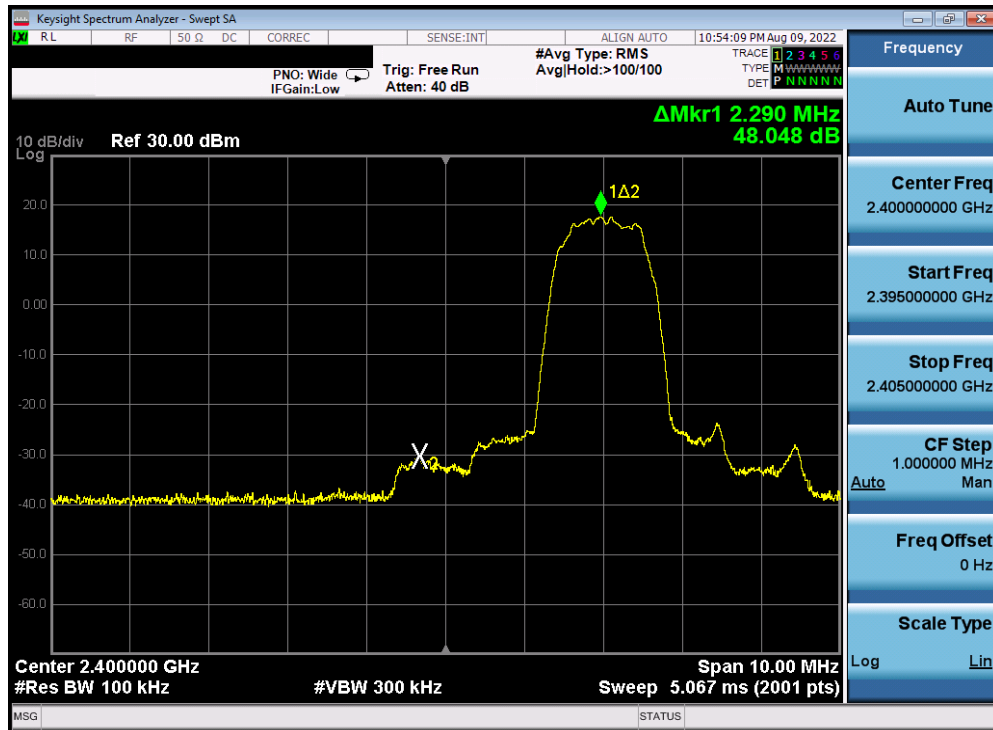
Plot 7-17. Band Edge Plot Antenna WF8 (Bluetooth with Hopping Disabled, 8DPSK, ePA – 2402 MHz)
