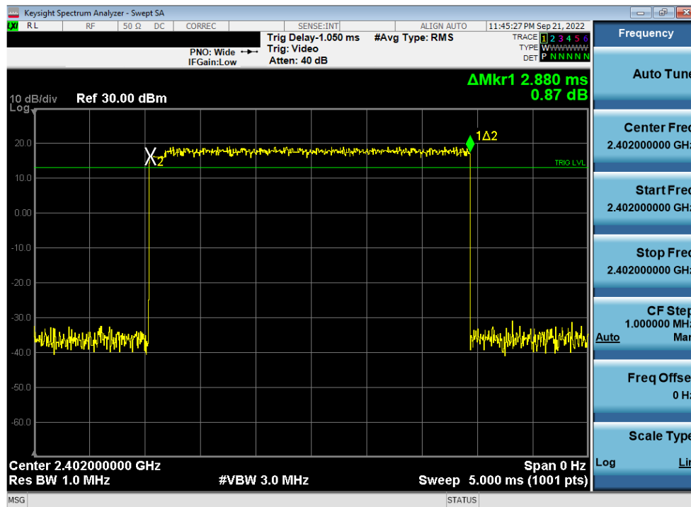
Plot 7-34. Time of Occupancy Plot Antenna WF8 (Bluetooth, 8DPSK, ePA, 2.4GHz)
