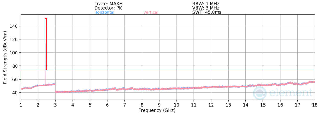
Plot 7-58. Radiated Spurious Emissions 1-18GHz Antenna WF8 (BT GFSK ePA – 2441 MHz)
