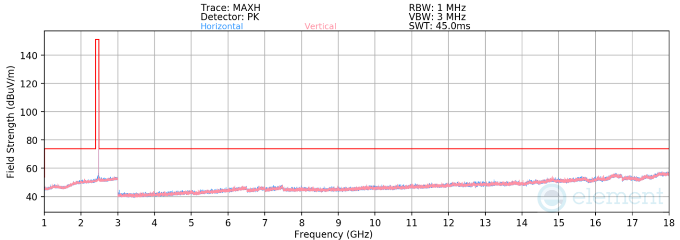
Plot 7-62. Radiated Spurious Emissions 1-18GHz Antenna WF7 (BT GFSK ePA – 2480 MHz)
