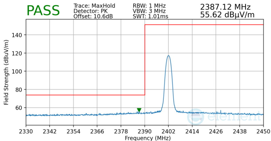
Plot 7-73. Radiated Restricted Lower Band Edge Measurement Antenna WF7
