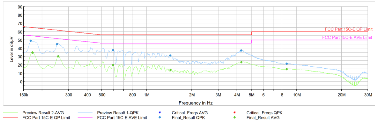
Plot 7-82. AC Line-Conducted Test Plot TxBF, 2.4GHz (N, GFSK ePA – 2480 MHz, with AC/DC Adapter)
