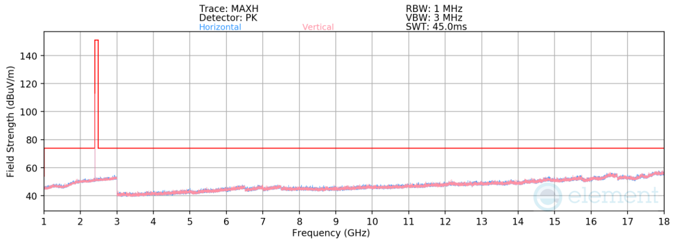
Plot 7-57. Radiated Spurious Emissions 1-18GHz Antenna WF8 (BT GFSK ePA – 2402 MHz)
