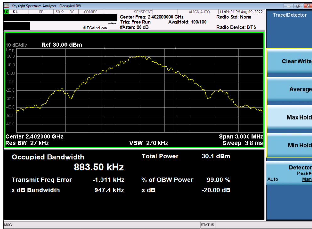
Plot 7-7. 20dB BW and 99% OBW Plot Antenna WF7 (Bluetooth, GFSK, ePA – 2402 MHz)
