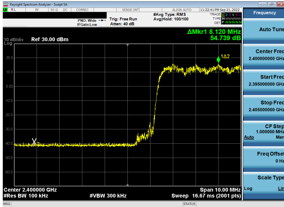
Plot 7-27. Band Edge Plot Antenna WF7 (Bluetooth with Hopping Enabled, 8DPSK, ePA, 2.4GHz)
