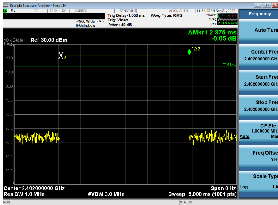
Plot 7-33. Time of Occupancy Plot Antenna WF8 (Bluetooth, GFSK, ePA, 2.4GHz)
