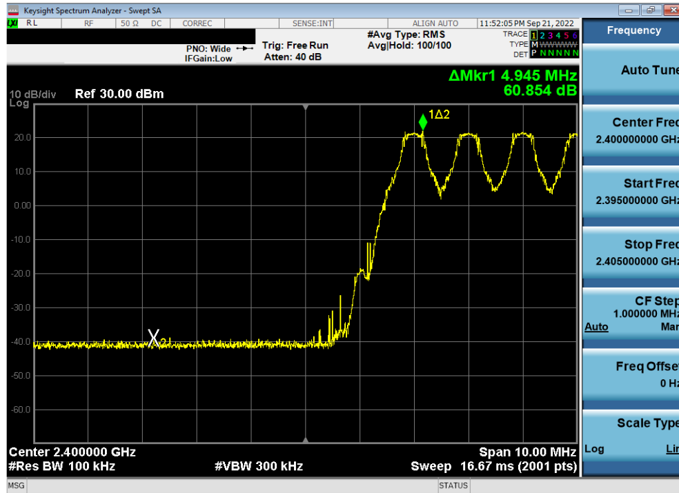
Plot 7-15. Band Edge Plot Antenna WF8 (Bluetooth with Hopping Enabled, GFSK, ePA, 2.4GHz)
