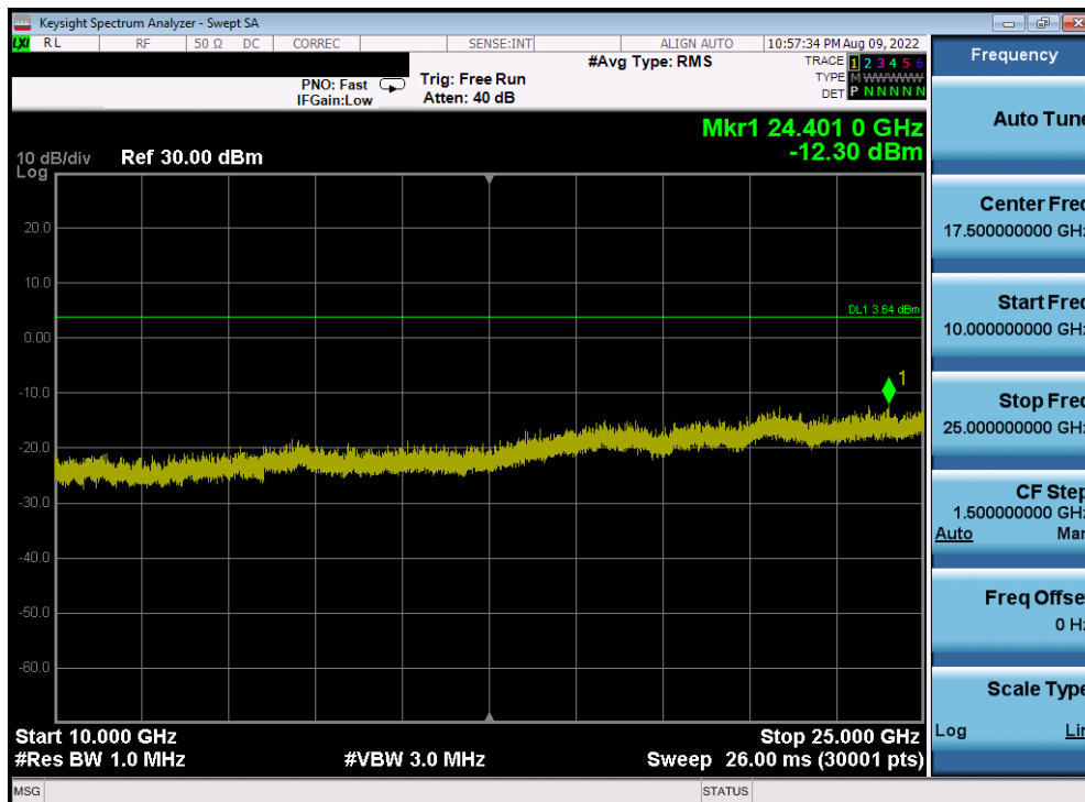
Plot 7-46. Conducted Spurious Plot Antenna WF8 (Bluetooth, GFSK, ePA – 2402 MHz)
