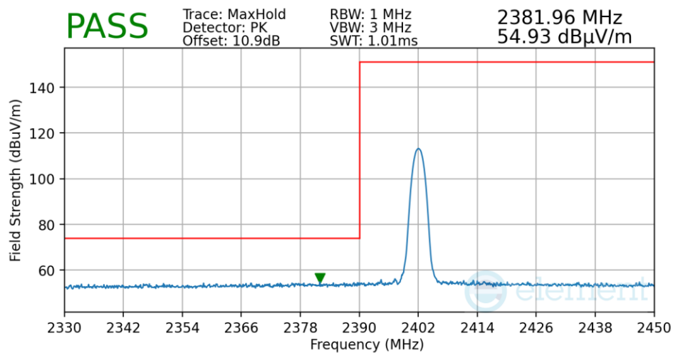
Plot 7-69. Radiated Restricted Lower Band Edge Measurement Antenna WF8
