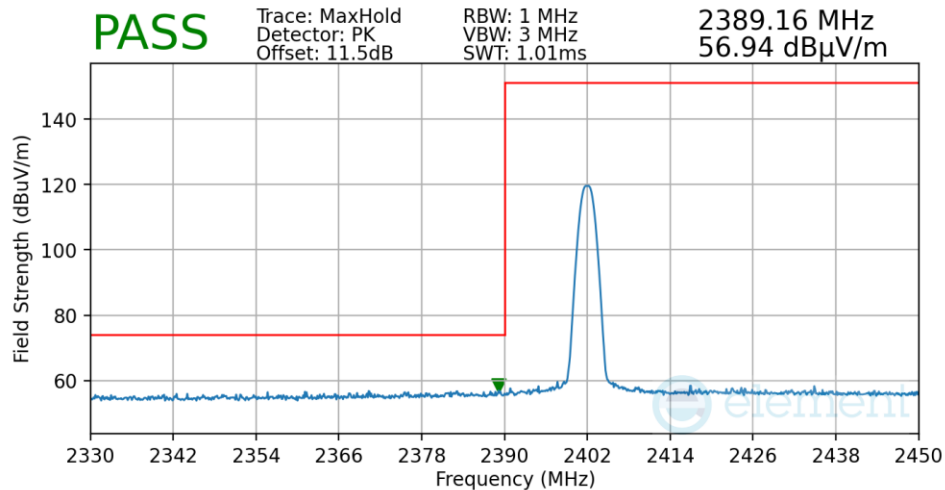
Plot 7-72. Radiated Restricted Lower Band Edge Measurement Antenna WF7
