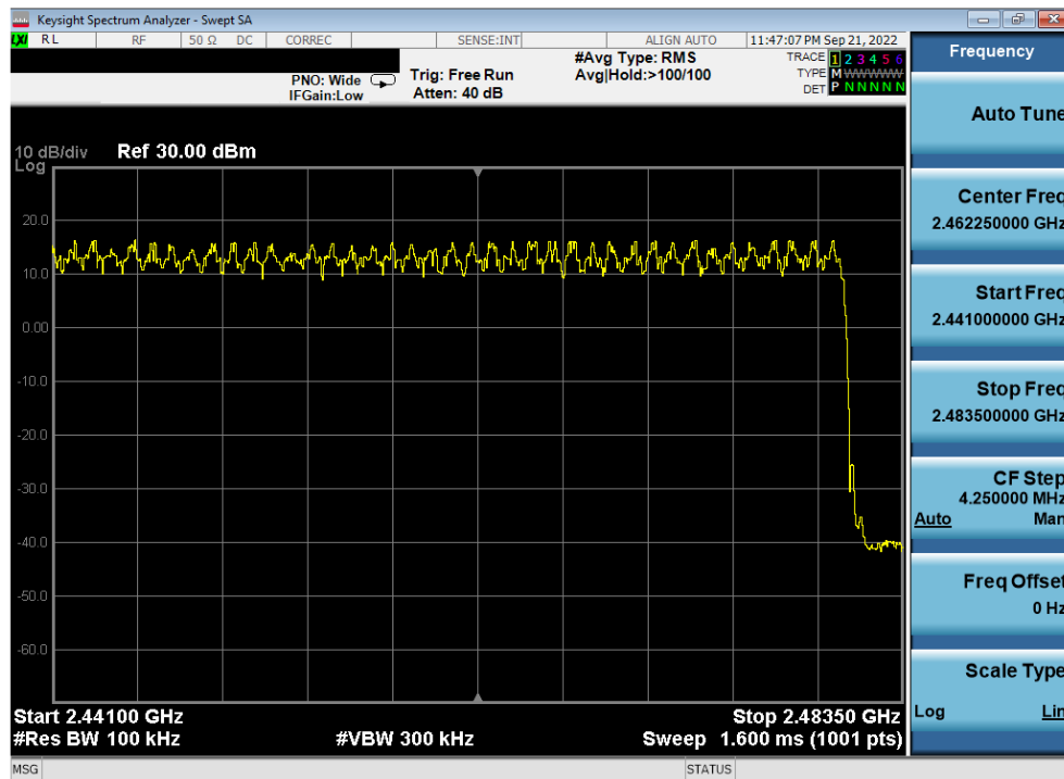
Plot 7-40. High End Spectrum Channel Hopping Plot Antenna WF8 (Bluetooth, 8DPSK, ePA, 2.4GHz)
