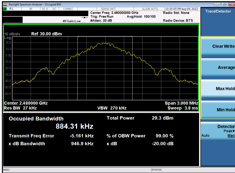
Plot 7-3. 20dB BW and 99% OBW Plot Antenna WF8 (Bluetooth, GFSK, ePA – 2480 MHz)
