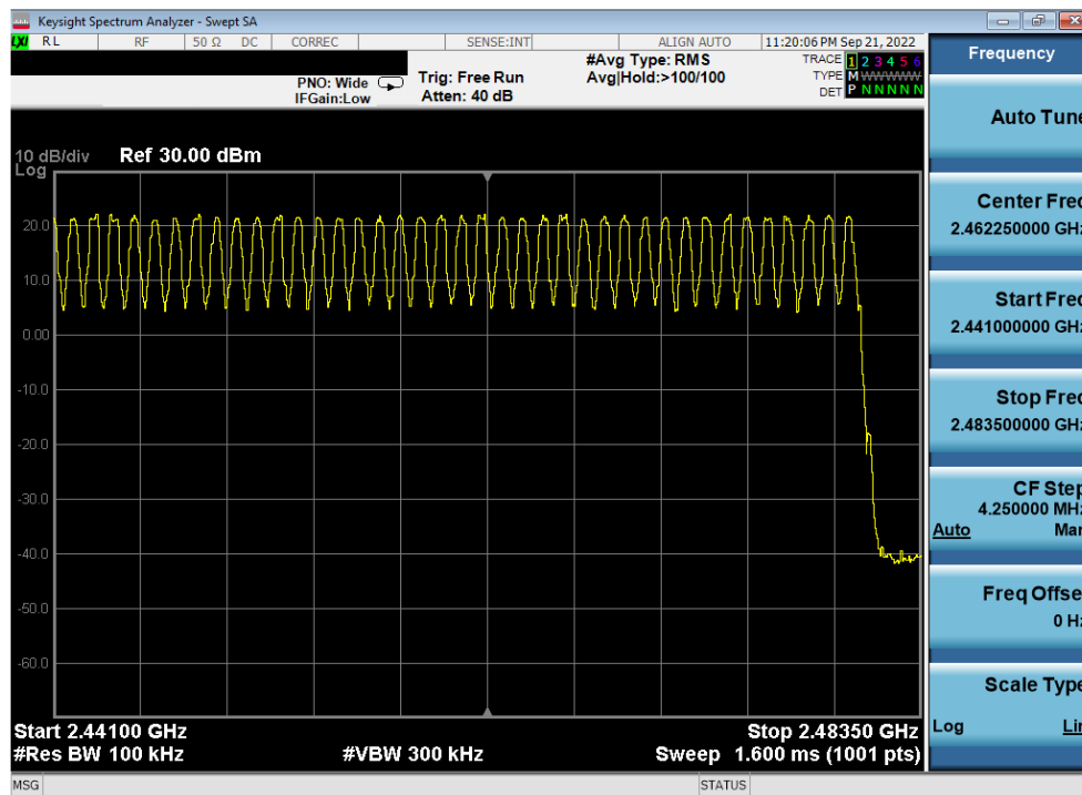
Plot 7-42. High End Spectrum Channel Hopping Plot Antenna WF7 (Bluetooth, GFSK, ePA, 2.4GHz)
