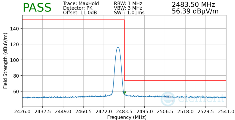
Plot 7-79. Radiated Restricted Upper Band Edge Measurement TxBF, 2.4GHz
