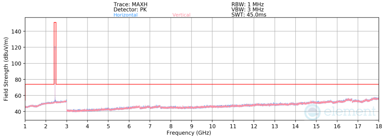
Plot 7-61. Radiated Spurious Emissions 1-18GHz Antenna WF7 (BT GFSK ePA – 2441 MHz)
