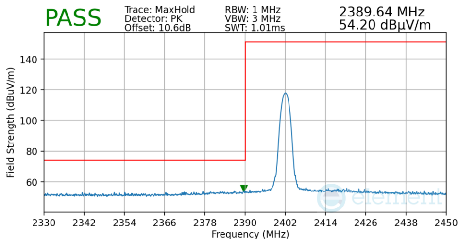
Plot 7-77. Radiated Restricted Lower Band Edge Measurement TxBF, 2.4GHz
