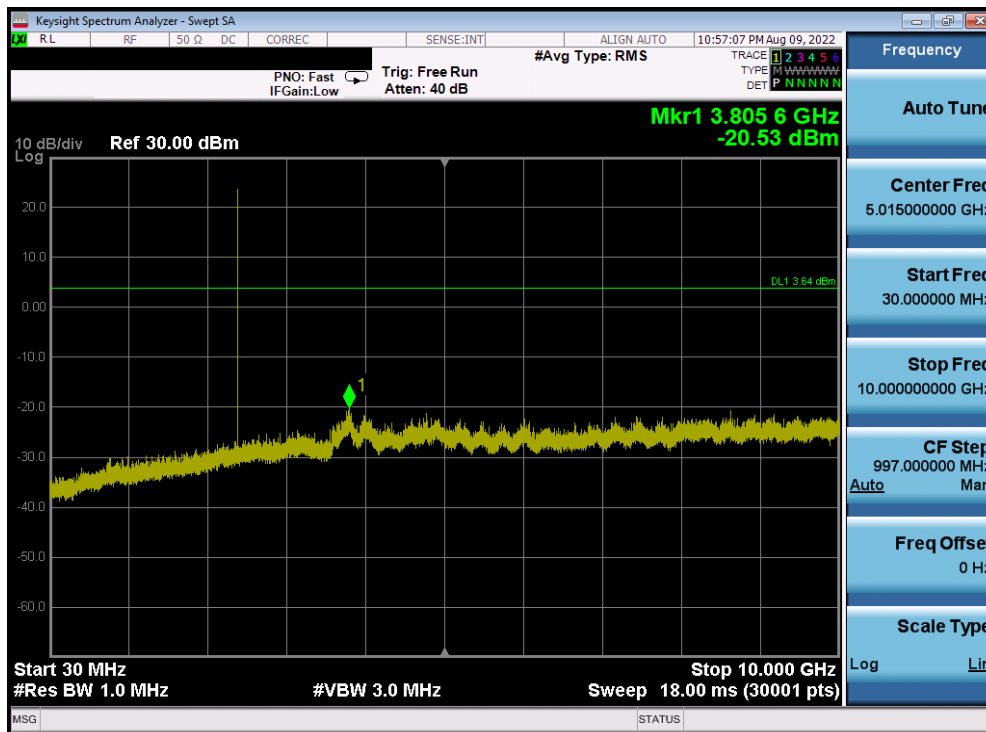
Plot 7-45. Conducted Spurious Plot Antenna WF8 (Bluetooth, GFSK, ePA – 2402 MHz)
