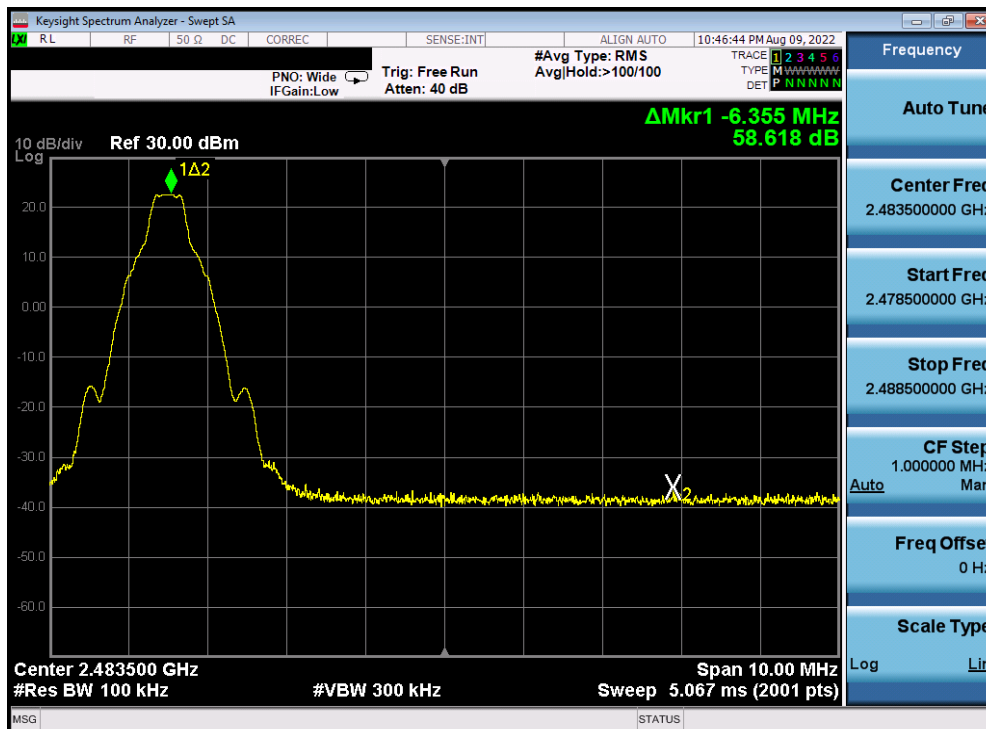
Plot 7-14. Band Edge Plot Antenna WF8 (Bluetooth with Hopping Disabled, GFSK, ePA – 2480 MHz)
