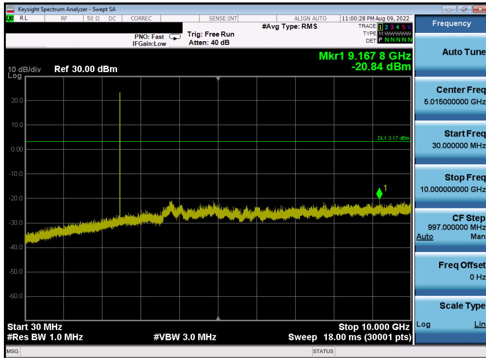
Plot 7-49. Conducted Spurious Plot Antenna WF8 (Bluetooth, GFSK, ePA – 2480 MHz)
