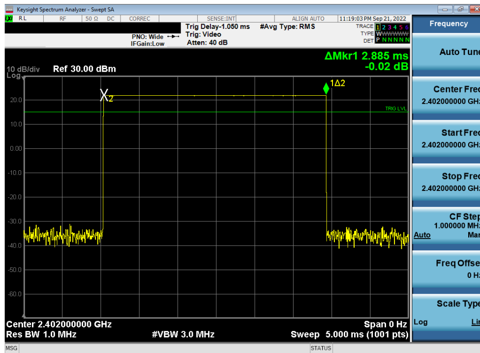
Plot 7-35. Time of Occupancy Plot Antenna WF7 (Bluetooth, GFSK, ePA, 2.4GHz)
