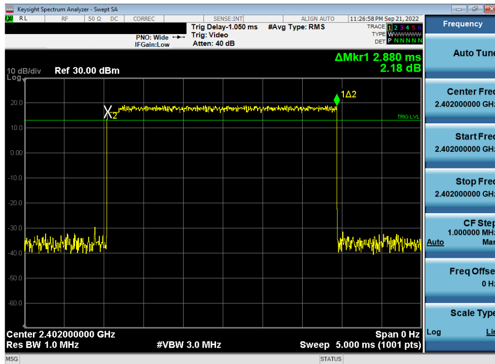
Plot 7-36. Time of Occupancy Plot Antenna WF7 (Bluetooth, 8DPSK, ePA, 2.4GHz)
