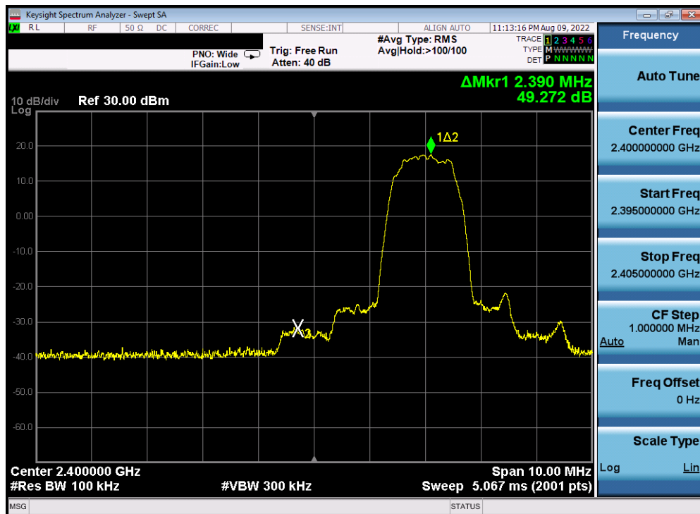
Plot 7-25. Band Edge Plot Antenna WF7 (Bluetooth with Hopping Disabled, 8DPSK, ePA – 2402 MHz)
