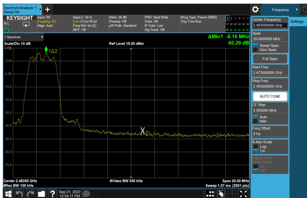
Plot 7-66. Band Edge Plot Antenna WF7 (Bluetooth (HDR4), ePA – Ch. 73)
