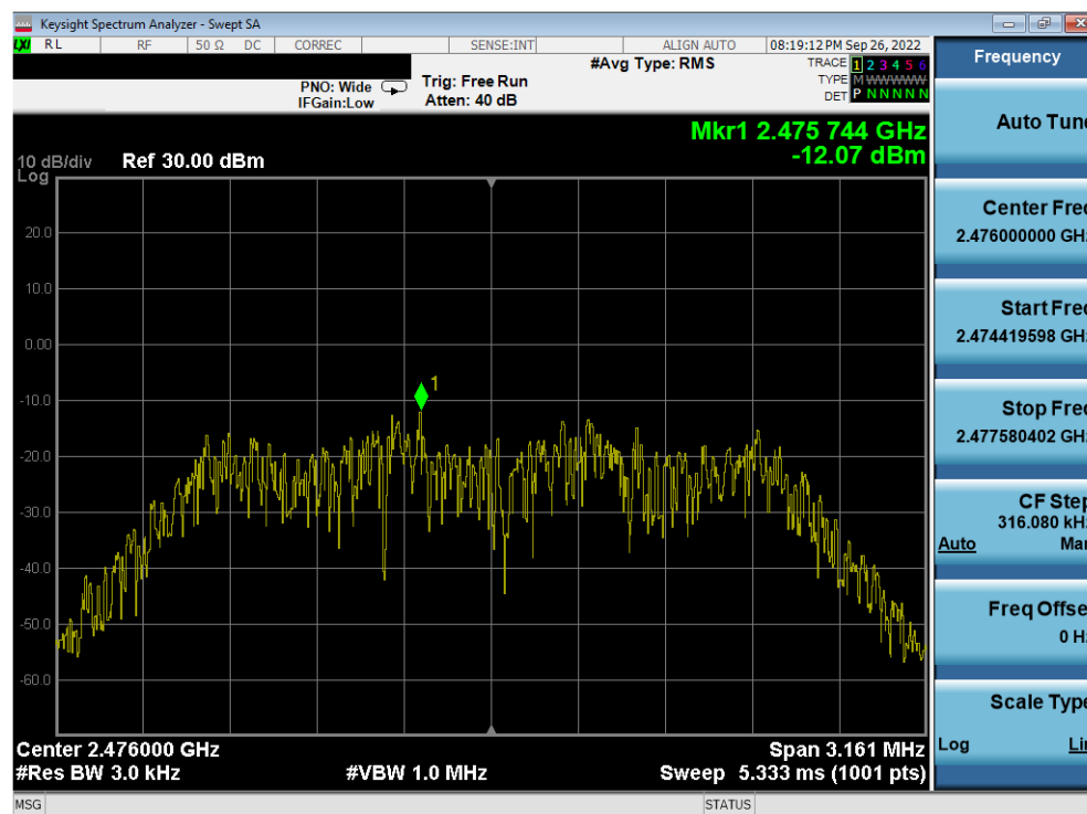
Plot 7-48. Power Spectral Density Plot Antenna WF7 (Bluetooth (HDR4), 4Mbps, iPA – Ch. 73)
