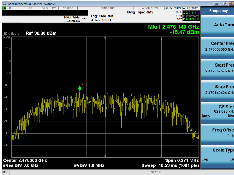
Plot 7-59. Power Spectral Density Plot Antenna WF8 (Bluetooth (HDR8), 8Mbps, iPA – Ch. 73)
