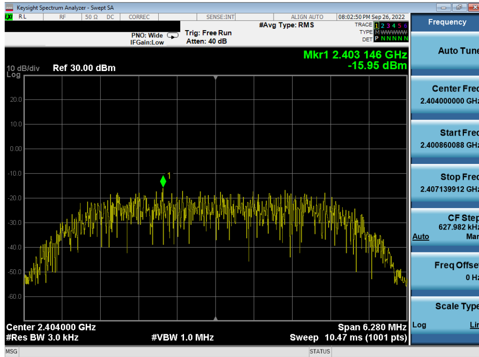
Plot 7-55. Power Spectral Density Plot Antenna WF8 (Bluetooth (HDR8), 8Mbps, iPA – Ch. 1)
