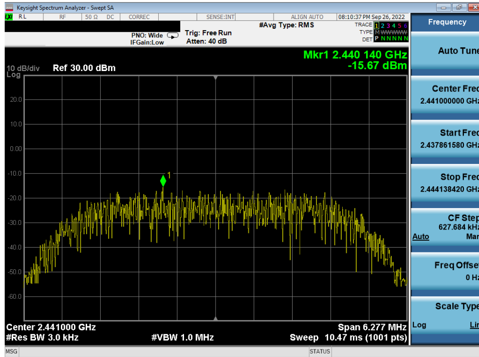
Plot 7-57. Power Spectral Density Plot Antenna WF8 (Bluetooth (HDR8), 8Mbps, iPA – Ch. 38)
