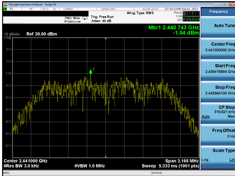
Plot 7-39. Power Spectral Density Plot Antenna WF8 (Bluetooth (HDR4), 4Mbps, ePA – Ch. 38)
