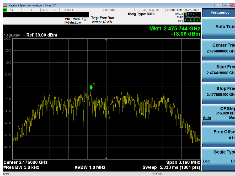
Plot 7-47. Power Spectral Density Plot Antenna WF8 (Bluetooth (HDR4), 4Mbps, iPA – Ch. 73)
