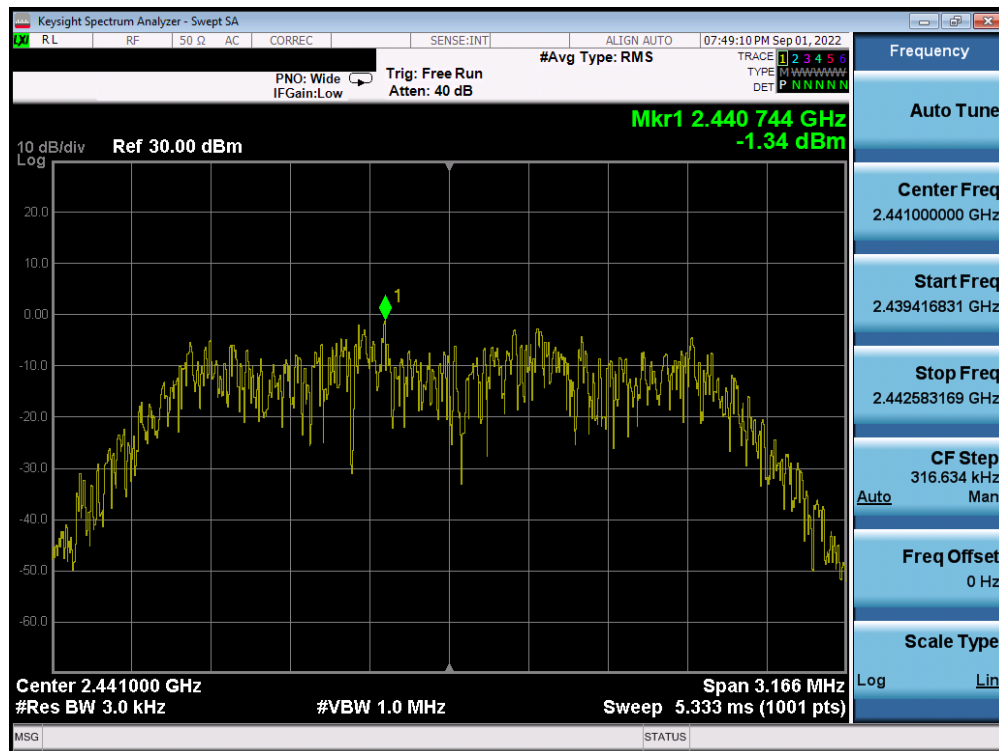
Plot 7-40. Power Spectral Density Plot Antenna WF7 (Bluetooth (HDR4), 4Mbps, ePA – Ch. 38)
