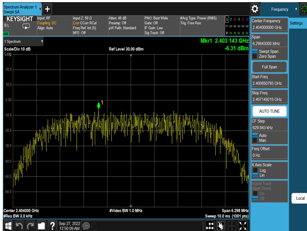
Plot 7-49. Power Spectral Density Plot Antenna WF8 (Bluetooth (HDR8), 8Mbps, ePA – Ch. 1)
