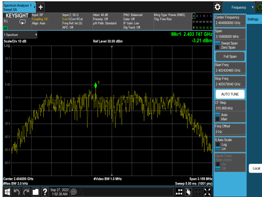
Plot 7-25. Power Spectral Density Plot Antenna WF7 (Bluetooth (HDR4), 4Mbps, ePA – Ch. 1)
