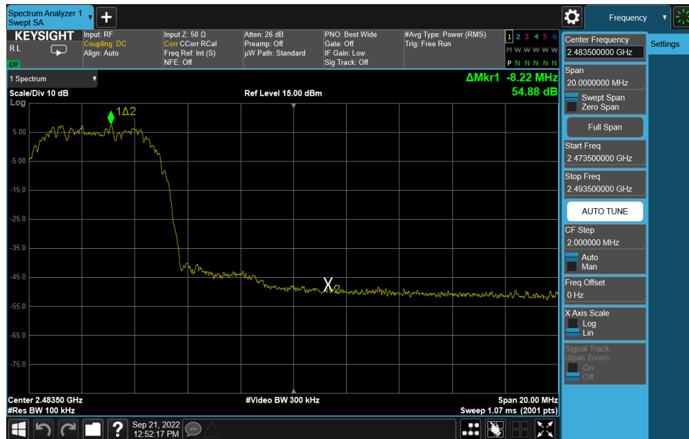
Plot 7-64. Band Edge Plot Antenna WF8 (Bluetooth (HDR8), ePA – Ch. 73)
