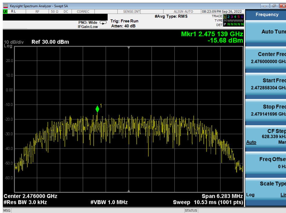
Plot 7-60. Power Spectral Density Plot Antenna WF7 (Bluetooth (HDR8), 8Mbps, iPA – Ch. 73)
