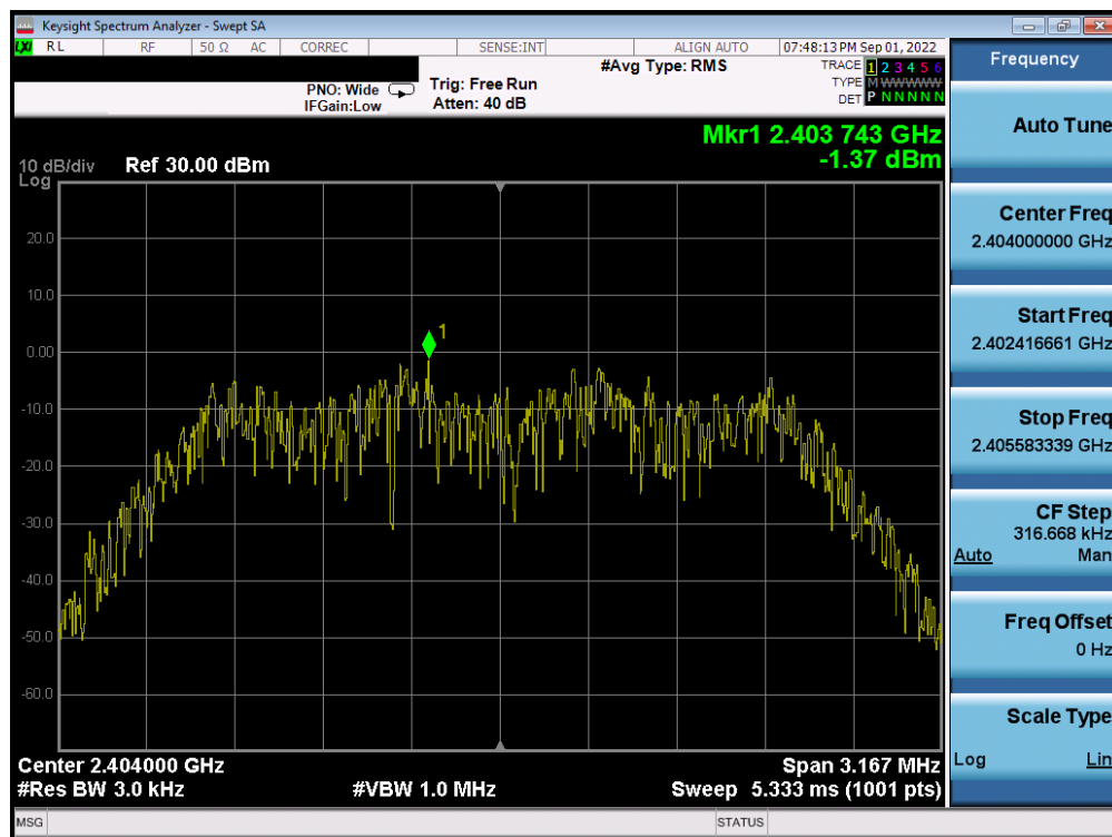
Plot 7-38. Power Spectral Density Plot Antenna WF7 (Bluetooth (HDR4), 4Mbps, ePA – Ch. 1)
