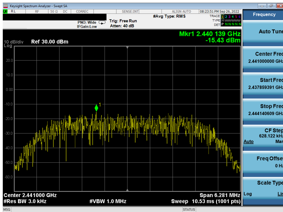
Plot 7-58. Power Spectral Density Plot Antenna WF7 (Bluetooth (HDR8), 8Mbps, iPA – Ch. 38)
