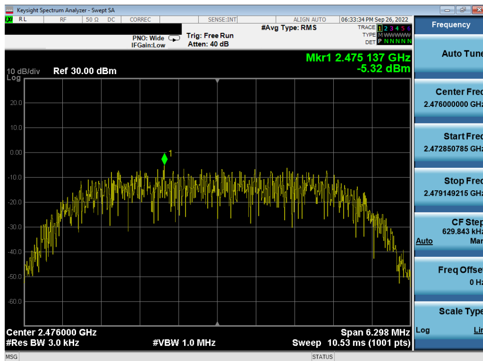
Plot 7-54. Power Spectral Density Plot Antenna WF7 (Bluetooth (HDR8), 8Mbps, ePA – Ch. 73)
