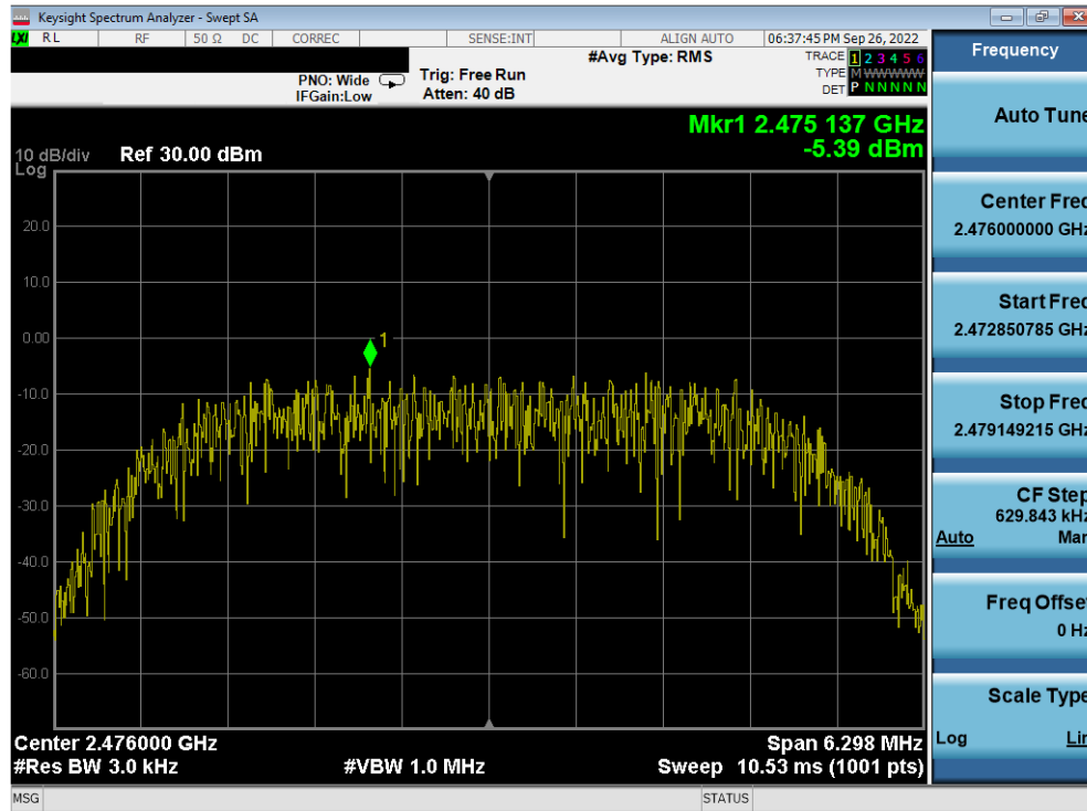
Plot 7-53. Power Spectral Density Plot Antenna WF8 (Bluetooth (HDR8), 8Mbps, ePA – Ch. 73)
