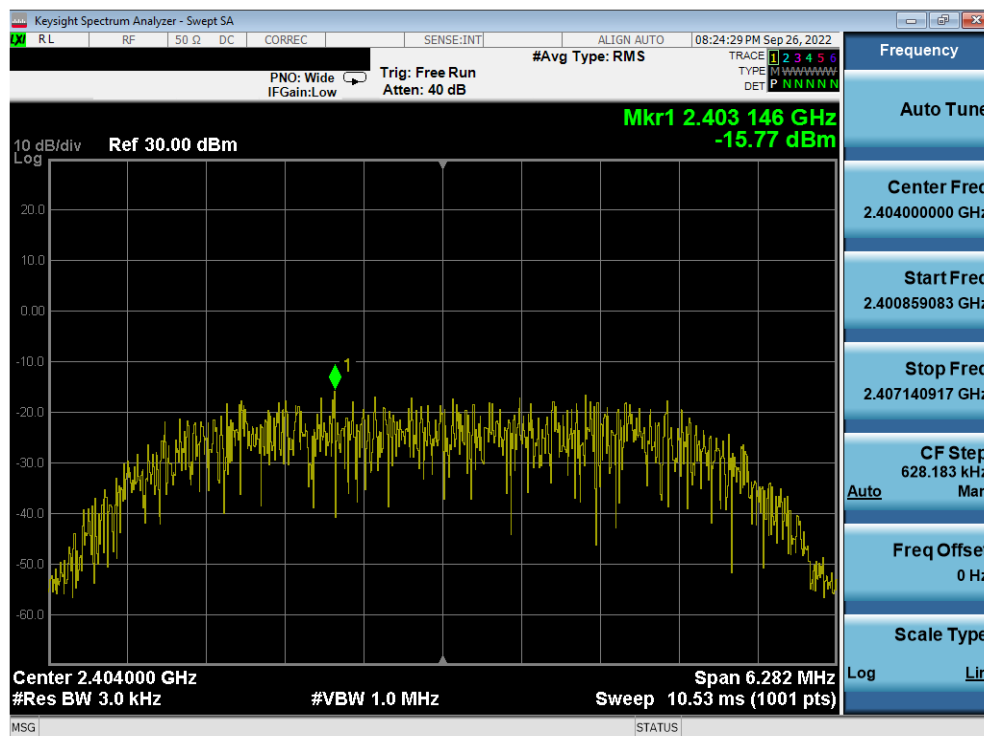
Plot 7-56. Power Spectral Density Plot Antenna WF7 (Bluetooth (HDR8), 8Mbps, iPA – Ch. 1)
