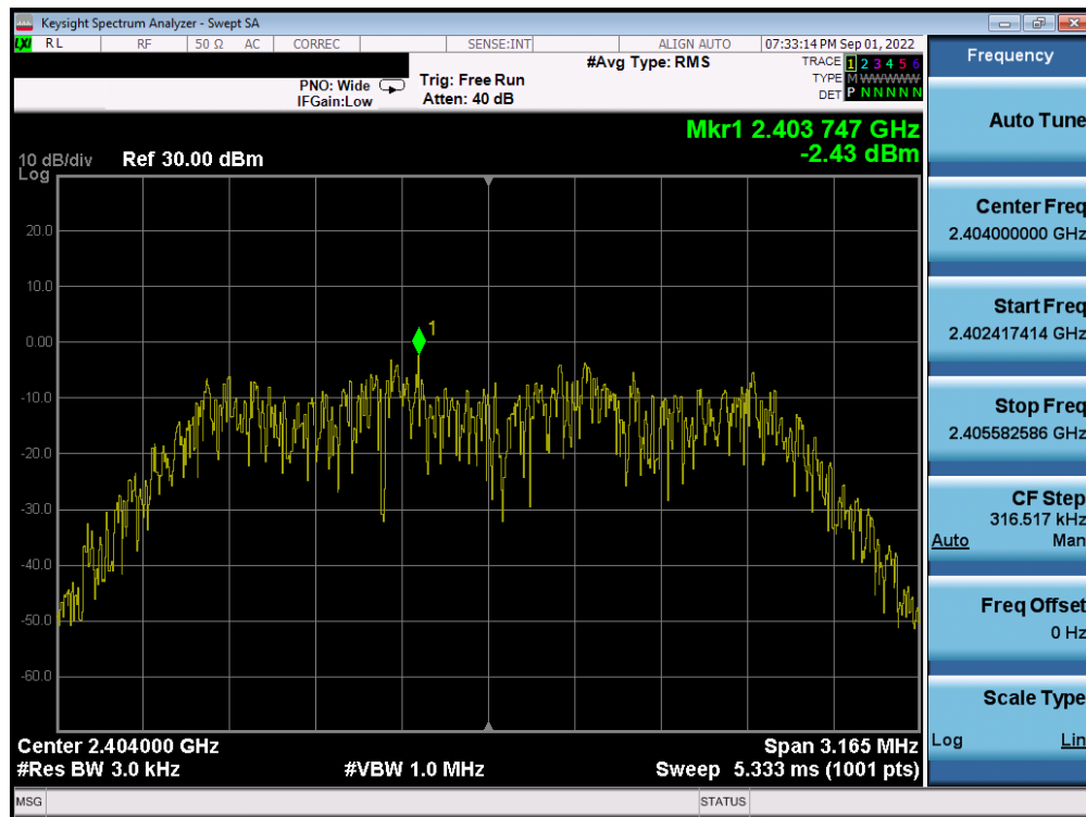
Plot 7-37. Power Spectral Density Plot Antenna WF8 (Bluetooth (HDR4), 4Mbps, ePA – Ch. 1)
