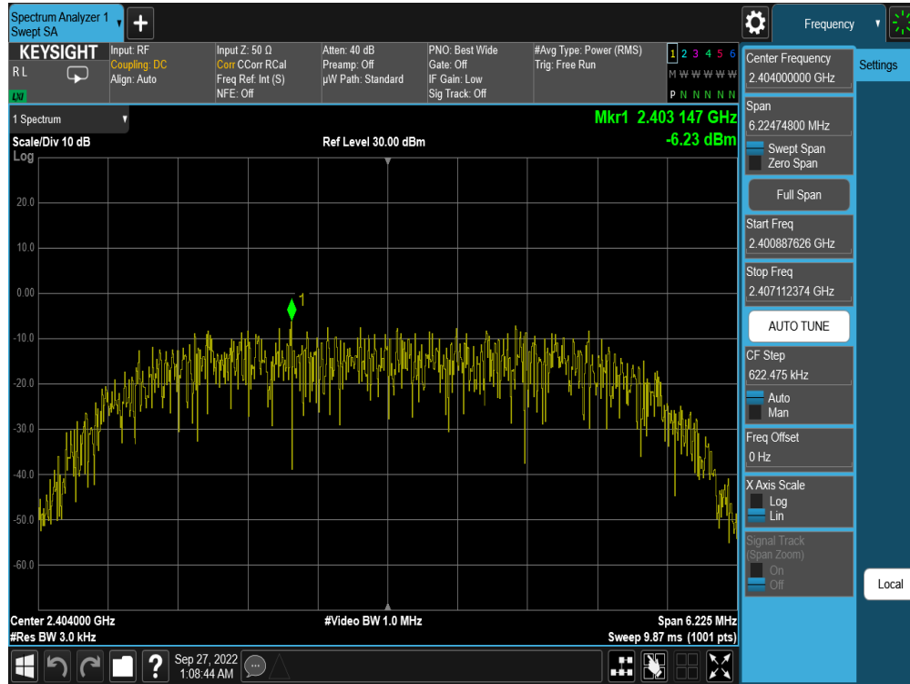
Plot 7-31. Power Spectral Density Plot Antenna WF7 (Bluetooth (HDR8), 8Mbps, ePA – Ch. 1)
