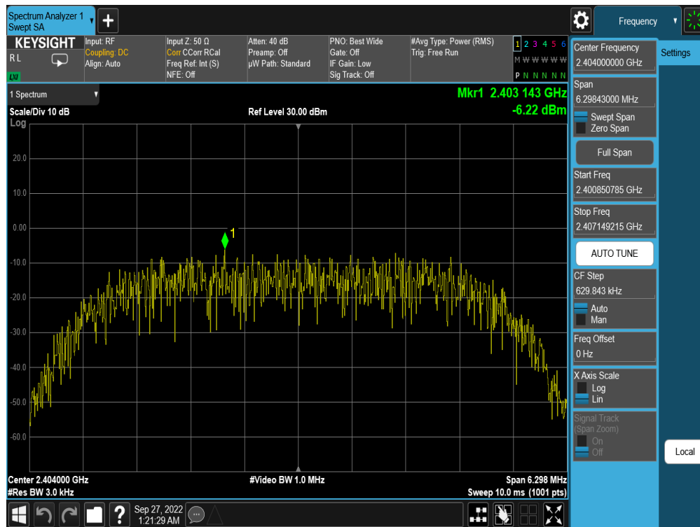
Plot 7-50. Power Spectral Density Plot Antenna WF7 (Bluetooth (HDR8), 8Mbps, ePA – Ch. 1)
