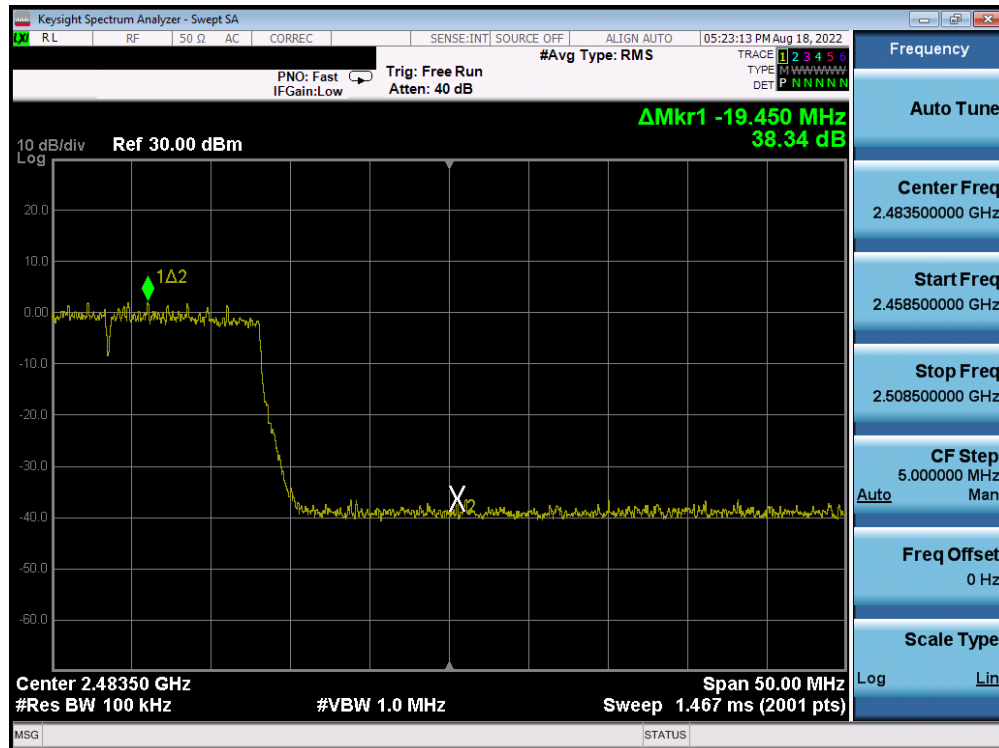
Plot 7-89. Band Edge Antenna WF8 (802.11ax OFDMA – RU242 – Ch. 11)
