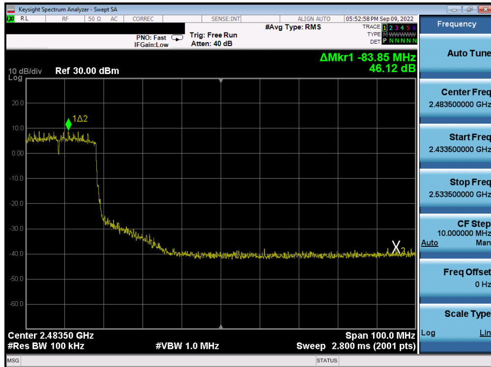
Plot 7-85. Band Edge Antenna WF8 (802.11ax OFDMA – RU242 – Ch. 7)
