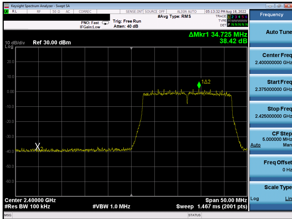
Plot 7-78. Band Edge Antenna WF8 (802.11ax OFDMA – RU242 – Ch. 1)
