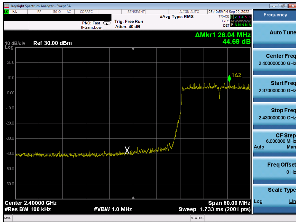
Plot 7-80. Band Edge Antenna WF8 (802.11ax OFDMA – RU242 – Ch. 3)
