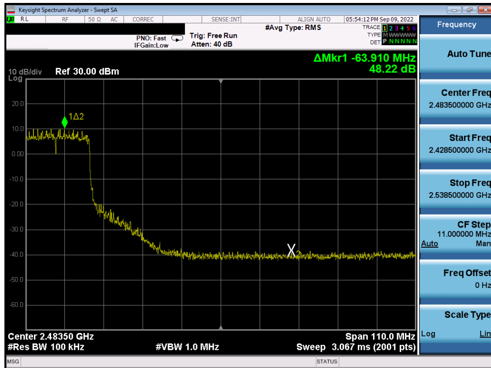
Plot 7-84. Band Edge Antenna WF8 (802.11ax OFDMA – RU242 – Ch. 6 (high))
