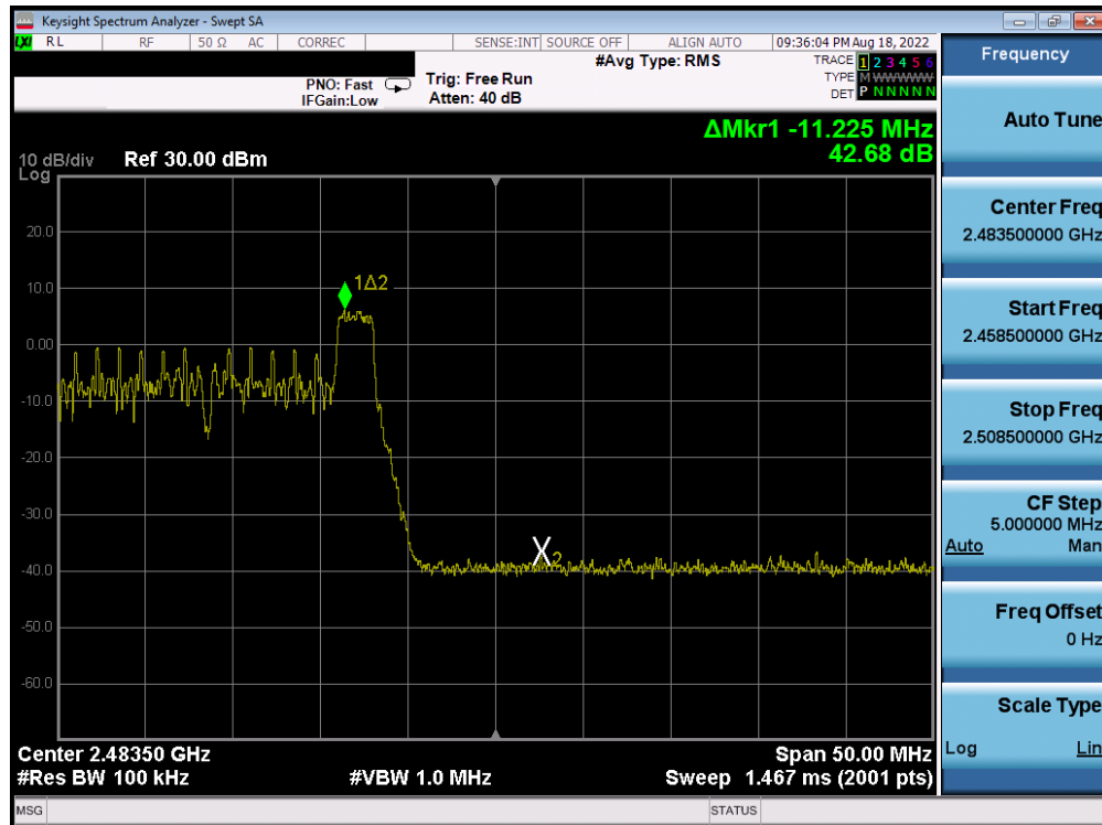
Plot 7-77. Band Edge Antenna WF8 (802.11ax OFDMA – RU26 Index 8 – Ch. 12)
