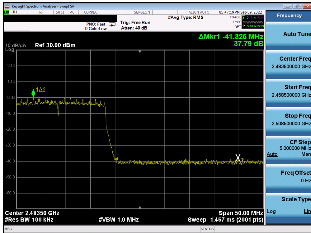
Plot 7-90. Band Edge Antenna WF8 (802.11ax OFDMA – RU242 – Ch. 12)
