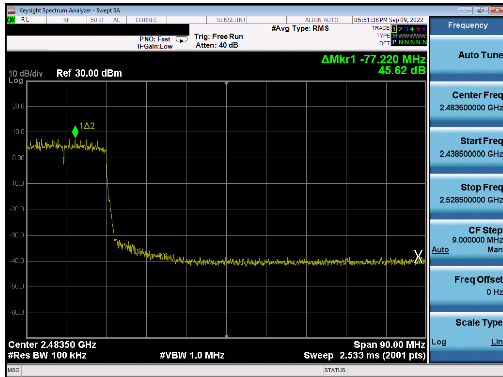
Plot 7-86. Band Edge Antenna WF8 (802.11ax OFDMA – RU242 – Ch. 8)
