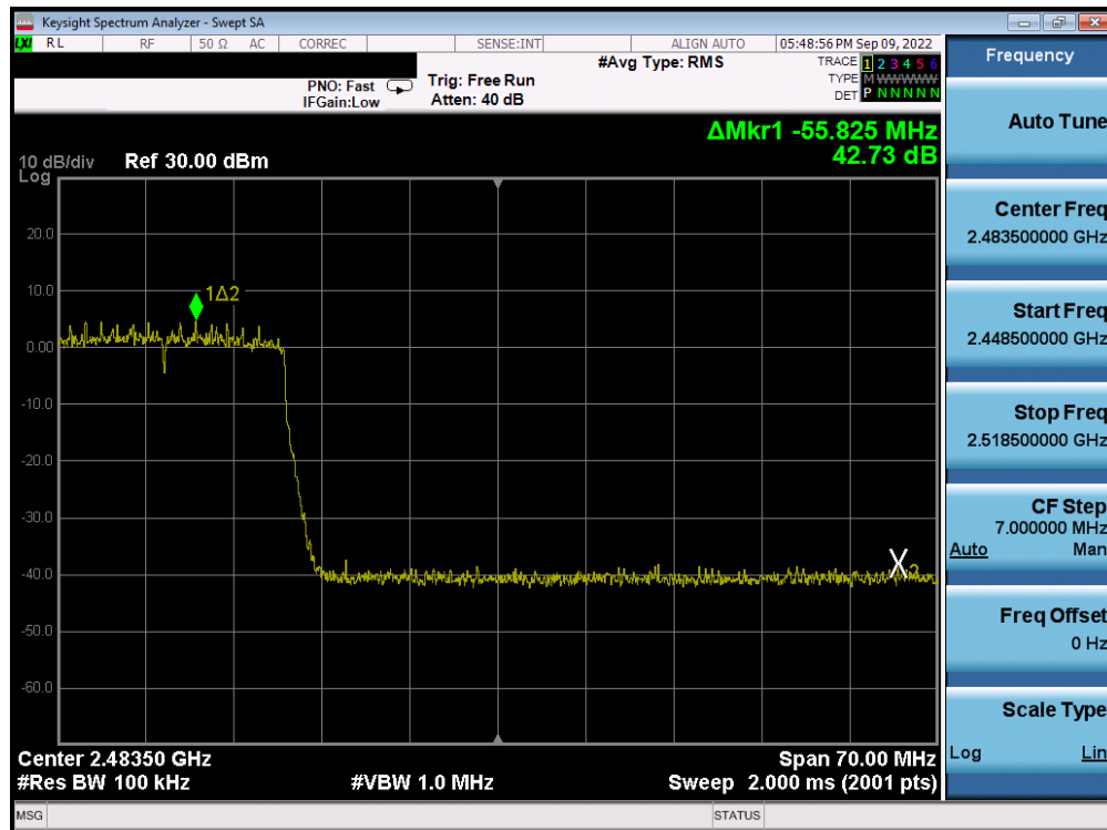
Plot 7-88. Band Edge Antenna WF8 (802.11ax OFDMA – RU242 – Ch. 10)
