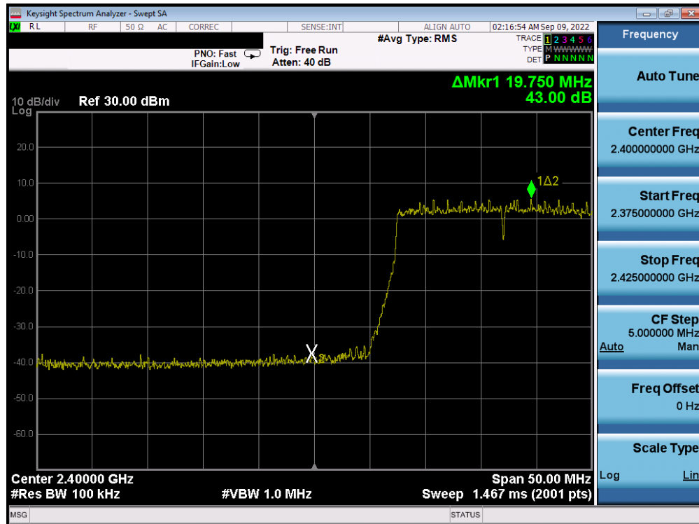
Plot 7-79. Band Edge Antenna WF8 (802.11ax OFDMA – RU242 – Ch. 2)
