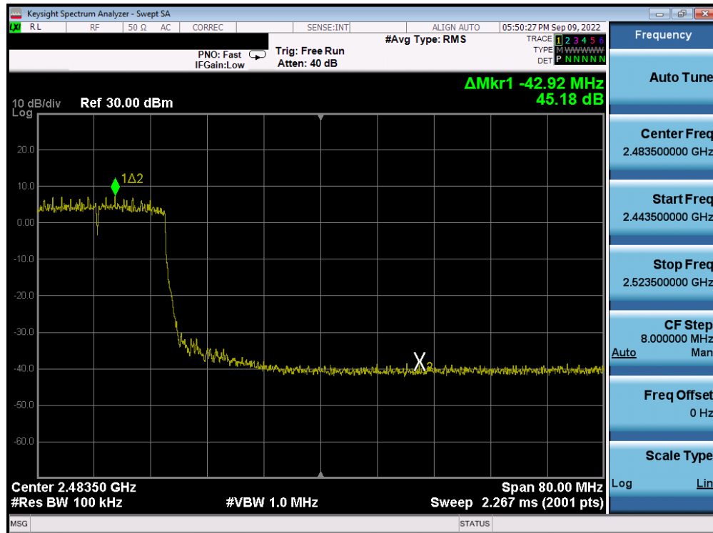
Plot 7-87. Band Edge Antenna WF8 (802.11ax OFDMA – RU242 – Ch. 9)
