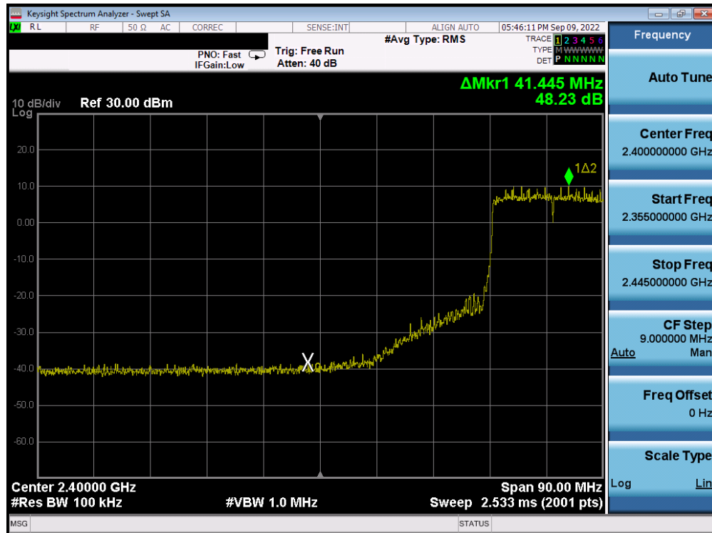
Plot 7-83. Band Edge Antenna WF8 (802.11ax OFDMA – RU242 – Ch. 6 (low))
