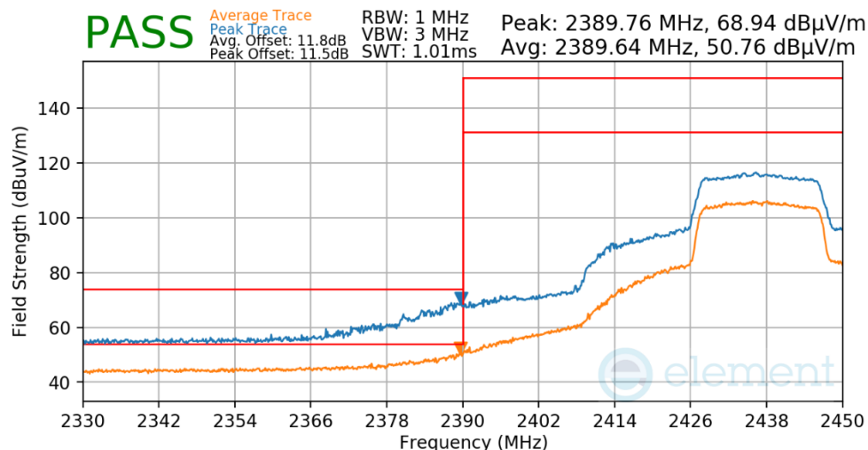
Plot 7-630. Radiated Restricted Lower Band Edge Measurement Antenna WF7
