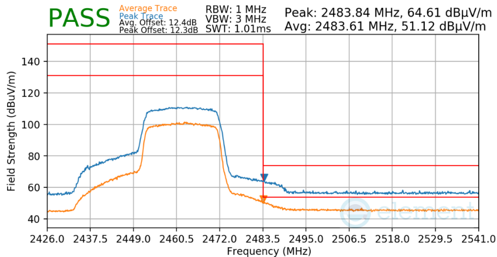
Plot 7-647. Radiated Restricted Upper Band Edge Measurement Antenna WF7
