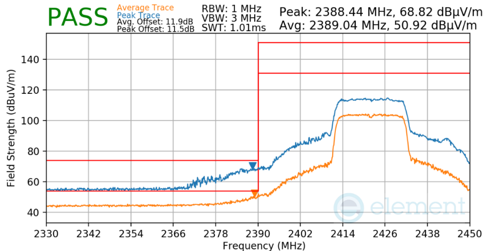
Plot 7-622. Radiated Restricted Lower Band Edge Measurement Antenna WF7
