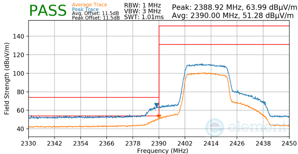
Plot 7-614. Radiated Restricted Lower Band Edge Measurement Antenna WF7
