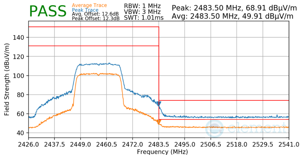
Plot 7-646. Radiated Restricted Upper Band Edge Measurement Antenna WF7
