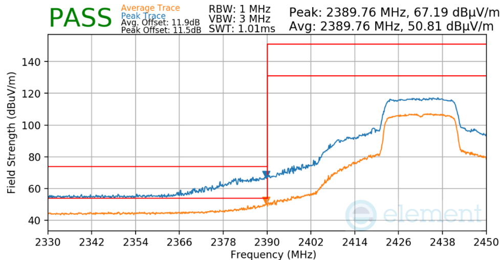
Plot 7-628. Radiated Restricted Lower Band Edge Measurement Antenna WF7
