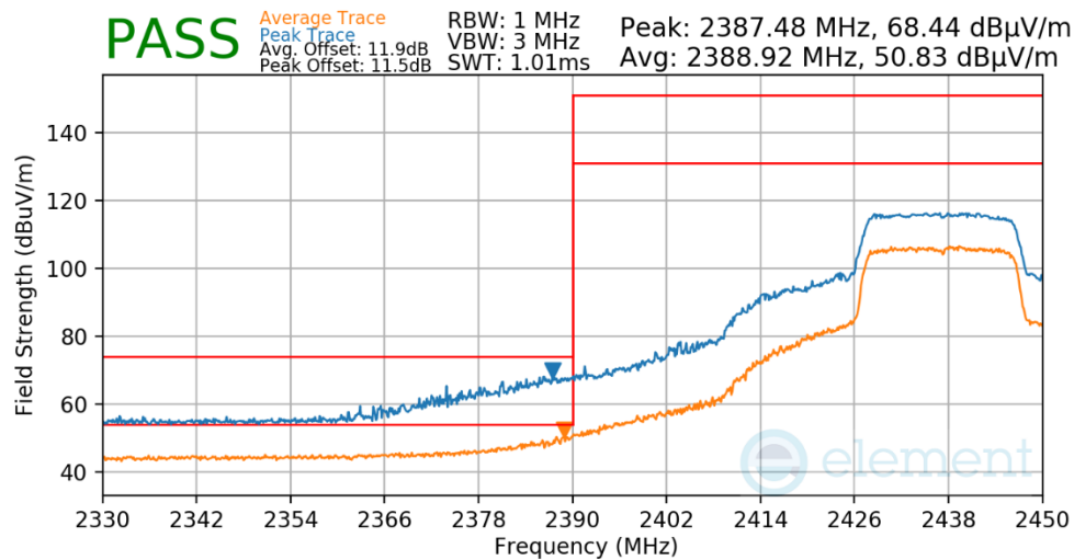
Plot 7-631. Radiated Restricted Lower Band Edge Measurement Antenna WF7
