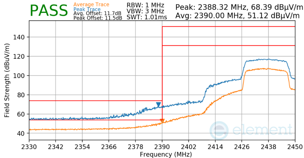
Plot 7-629. Radiated Restricted Lower Band Edge Measurement Antenna WF7
