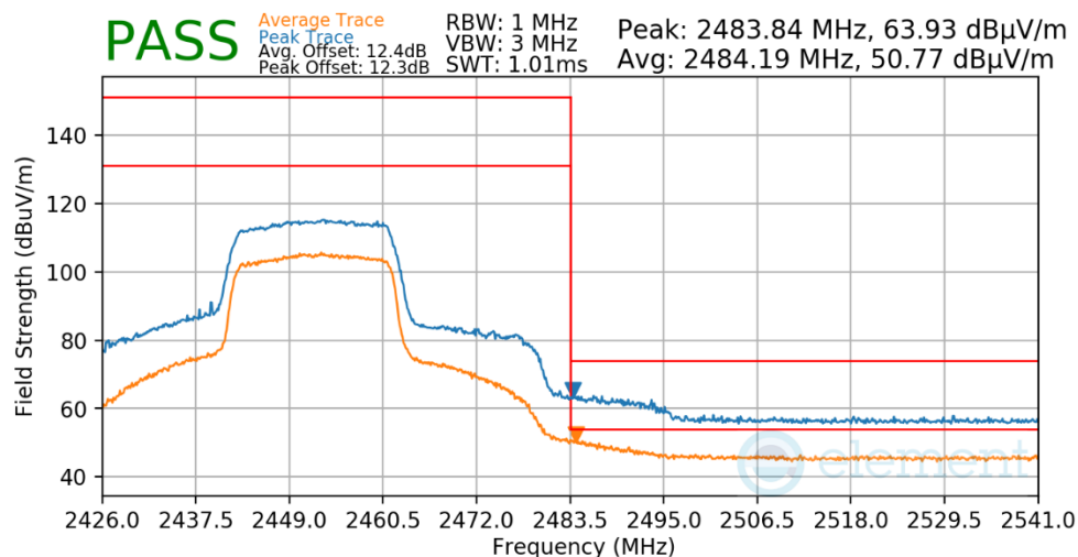
Plot 7-641. Radiated Restricted Upper Band Edge Measurement Antenna WF7
