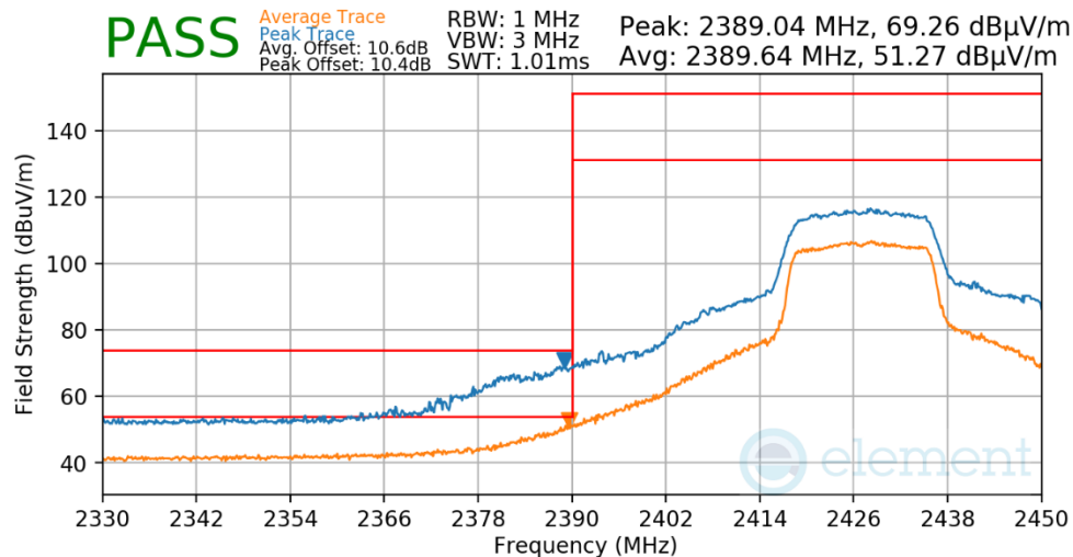
Plot 7-582. Radiated Restricted Lower Band Edge Measurement Antenna WF7
