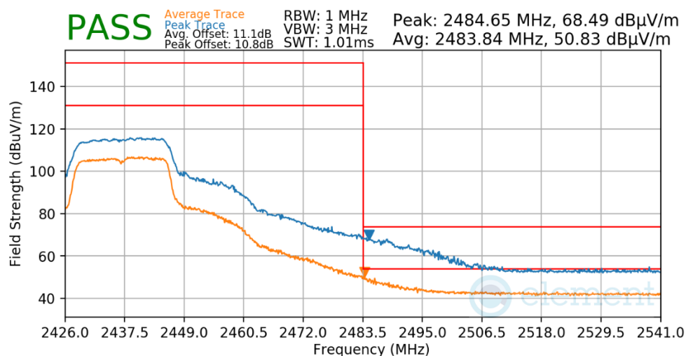
Plot 7-592. Radiated Restricted Upper Band Edge Measurement Antenna WF7
