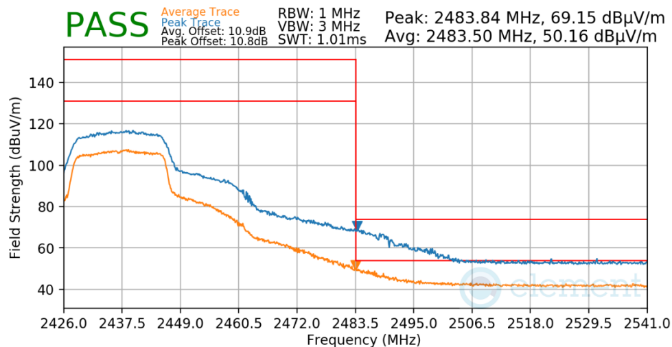
Plot 7-590. Radiated Restricted Upper Band Edge Measurement Antenna WF7
