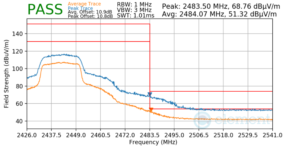
Plot 7-593. Radiated Restricted Upper Band Edge Measurement Antenna WF7
