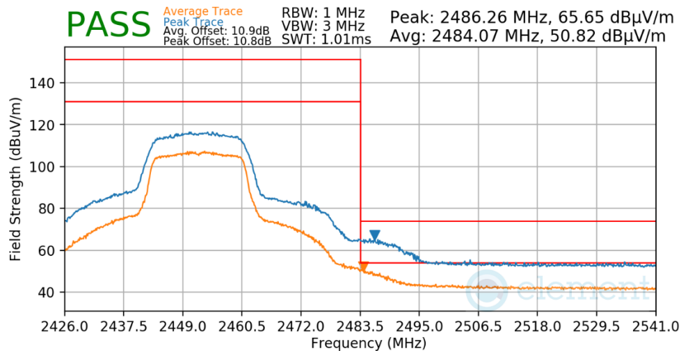
Plot 7-599. Radiated Restricted Upper Band Edge Measurement Antenna WF7
