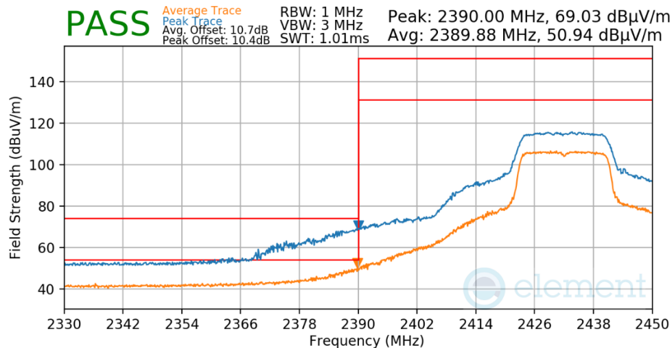
Plot 7-586. Radiated Restricted Lower Band Edge Measurement Antenna WF7
