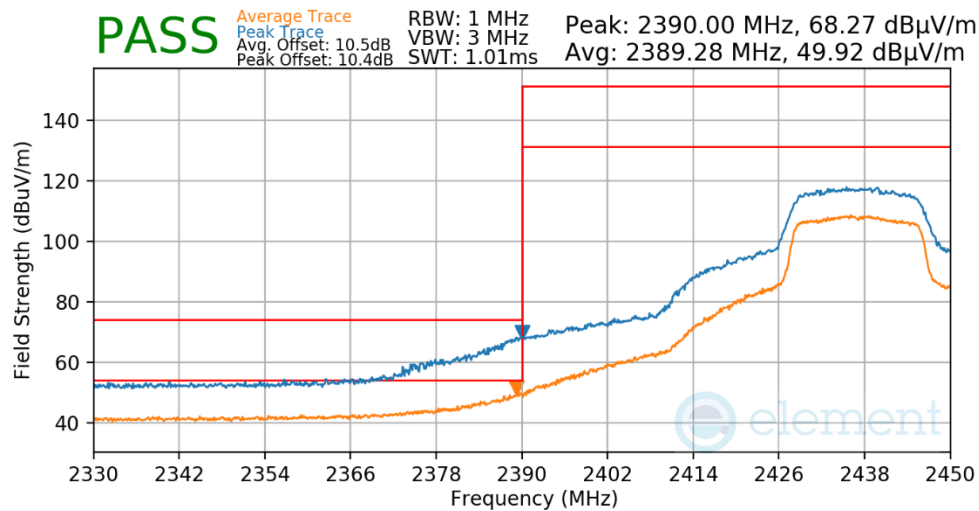
Plot 7-587. Radiated Restricted Lower Band Edge Measurement Antenna WF7
