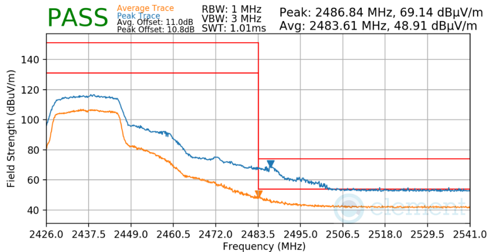
Plot 7-591. Radiated Restricted Upper Band Edge Measurement Antenna WF7
