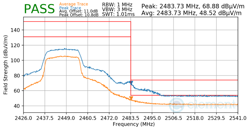
Plot 7-597. Radiated Restricted Upper Band Edge Measurement Antenna WF7
