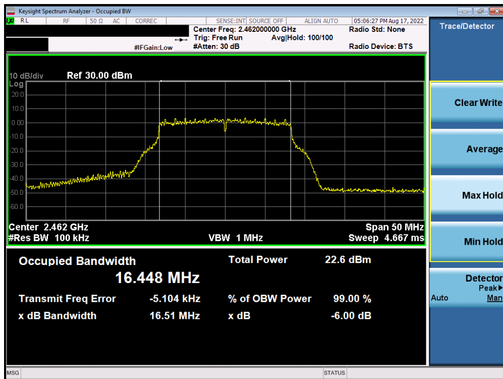
Plot 7-54. 6dB BW and 99% OBW Plot Antenna WF7 (802.11g – Ch. 11) – 36Mbps
