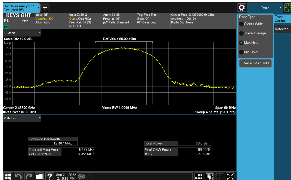
Plot 7-50. 6dB BW and 99% OBW Plot Antenna WF7 (802.11b – Ch. 6) – 11Mbps
