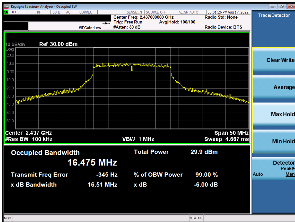
Plot 7-53. 6dB BW and 99% OBW Plot Antenna WF7 (802.11g – Ch. 6) – 36Mbps
