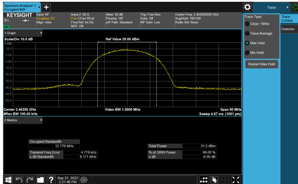
Plot 7-51. 6dB BW and 99% OBW Plot Antenna WF7 (802.11b – Ch. 11) – 11Mbps
