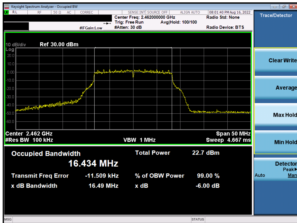
Plot 7-24. 6dB BW and 99% OBW Plot Antenna WF8 (802.11g – Ch. 11) – 36Mbps
