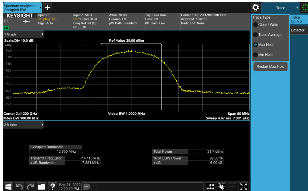
Plot 7-19. 6dB BW and 99% OBW Plot Antenna WF8 (802.11b – Ch. 1) – 11Mbps
