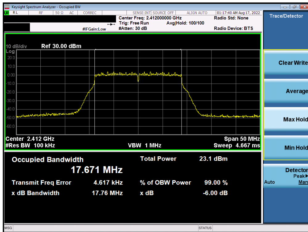
Plot 7-55. 6dB BW and 99% OBW Plot Antenna WF7 (802.11n (2.4GHz) – Ch. 1) – MCS5
