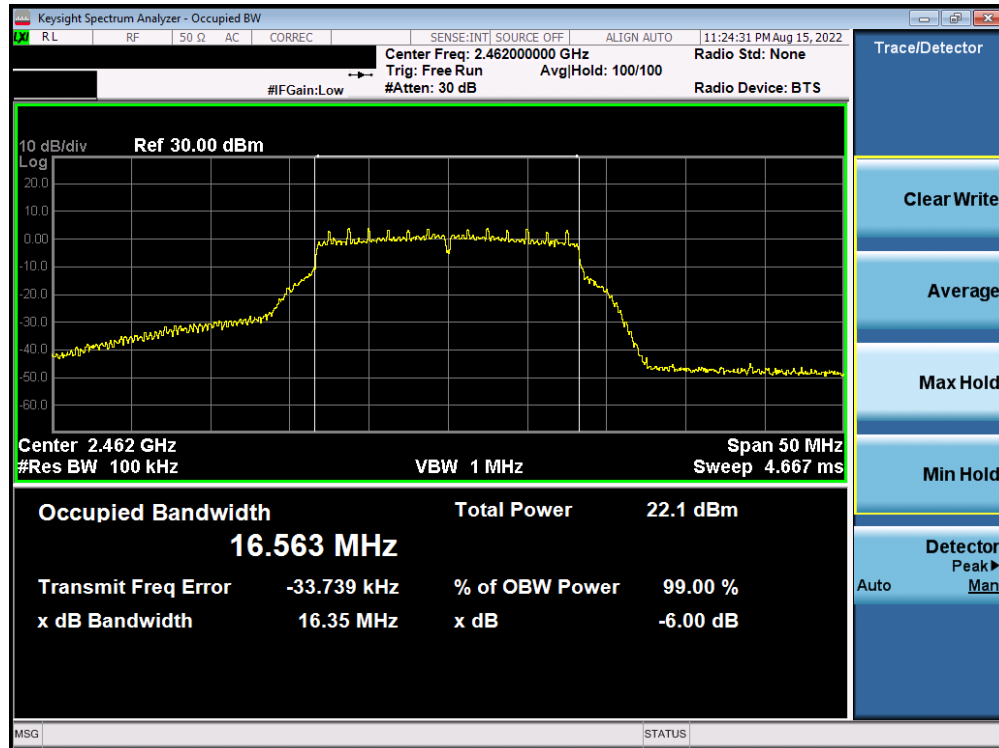
Plot 7-12. 6dB BW and 99% OBW Plot Antenna WF8 (802.11g – Ch. 11) – 18Mbps
