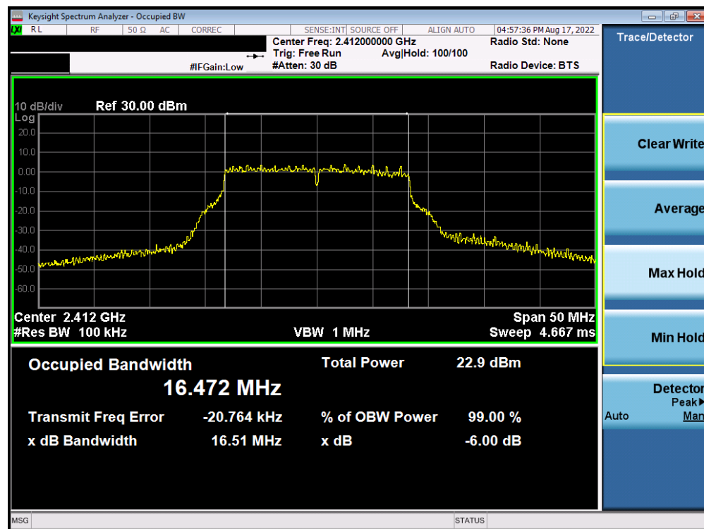
Plot 7-52. 6dB BW and 99% OBW Plot Antenna WF7 (802.11g – Ch. 1) – 36Mbps
