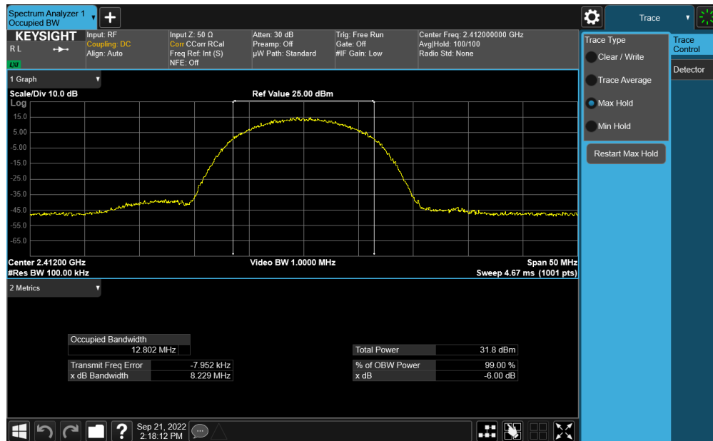
Plot 7-49. 6dB BW and 99% OBW Plot Antenna WF7 (802.11b – Ch. 1) – 11Mbps
