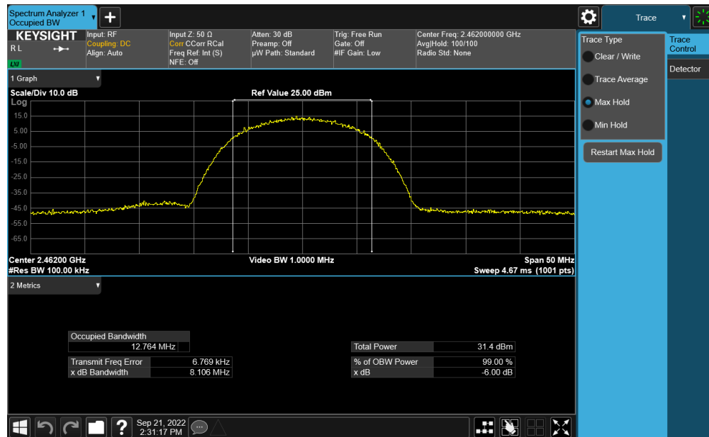
Plot 7-21. 6dB BW and 99% OBW Plot Antenna WF8 (802.11b – Ch. 11) – 11Mbps
