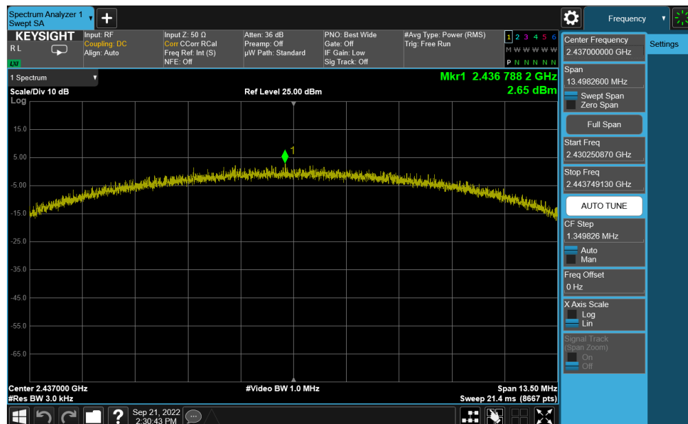
Plot 7-80. Power Spectral Density Plot Antenna WF8 (802.11b – Ch. 6) – 11Mbps
