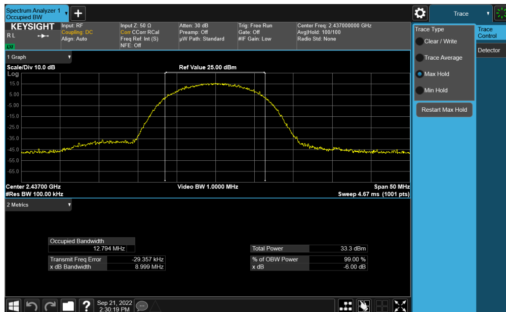
Plot 7-20. 6dB BW and 99% OBW Plot Antenna WF8 (802.11b – Ch. 6) – 11Mbps
