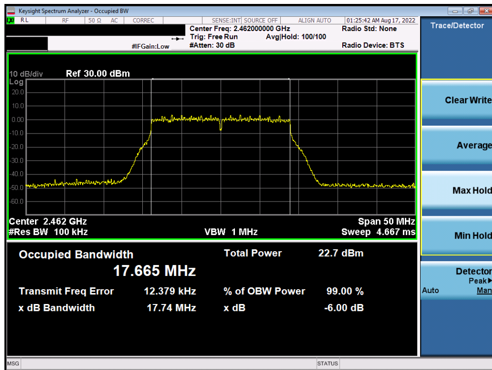
Plot 7-57. 6dB BW and 99% OBW Plot Antenna WF7 (802.11n (2.4GHz) – Ch. 11) – MCS5
