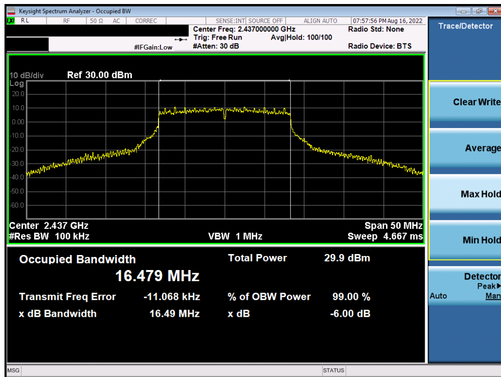
Plot 7-23. 6dB BW and 99% OBW Plot Antenna WF8 (802.11g – Ch. 6) – 36Mbps
