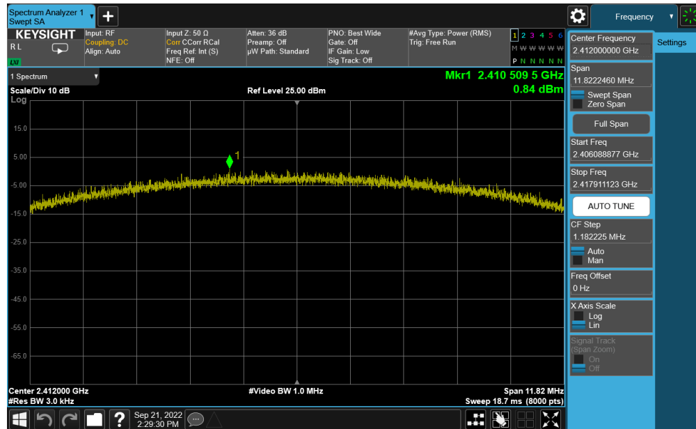
Plot 7-79. Power Spectral Density Plot Antenna WF8 (802.11b – Ch. 1) – 11Mbps
