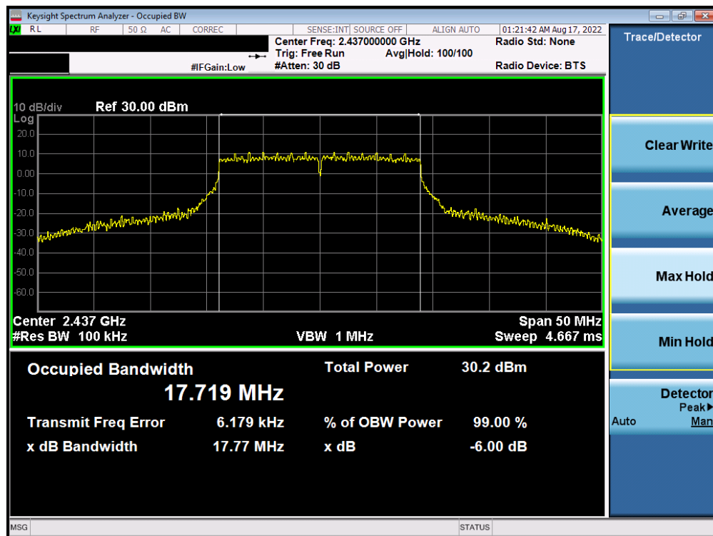
Plot 7-56. 6dB BW and 99% OBW Plot Antenna WF7 (802.11n (2.4GHz) – Ch. 6) – MCS5
