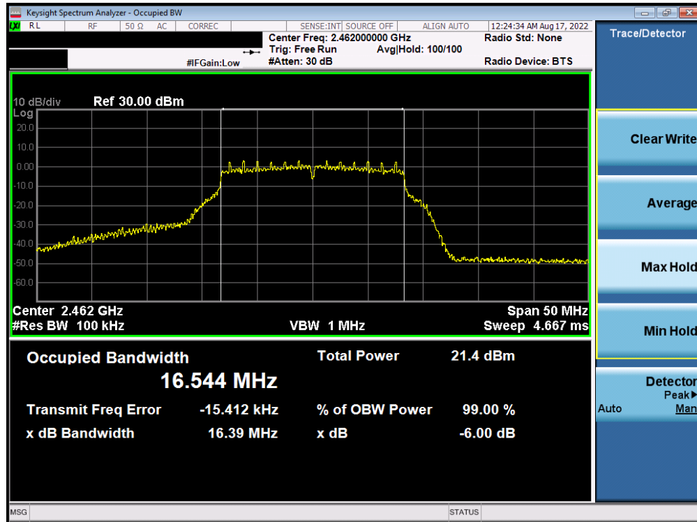
Plot 7-42. 6dB BW and 99% OBW Plot Antenna WF7 (802.11g – Ch. 11) – 18Mbps
