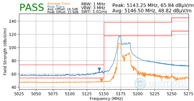
Plot 7-538. Antenna WF5T (Pk & Avg, RU52, Index 37, Ch.50, MCS11)
