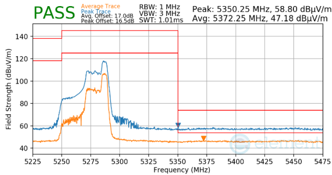
Plot 7-564. Antenna WF5B (Pk & Avg, RU52, Index 44, Ch.54, MCS11)
