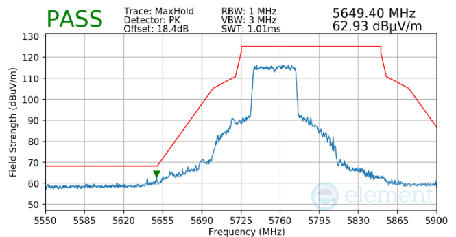
Plot 7-581. Antenna WF5B (Pk, RU484, Index 65, Ch.151, MCS11)
