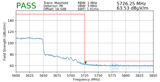
Plot 7-535. (FCC Only) Antenna WF5T (Pk, RU996, Index 67, Ch.122, MCS11)
