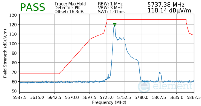
Plot 7-569. Antenna WF5B (Pk, RU26, Index 0, Ch.151, MCS11)
