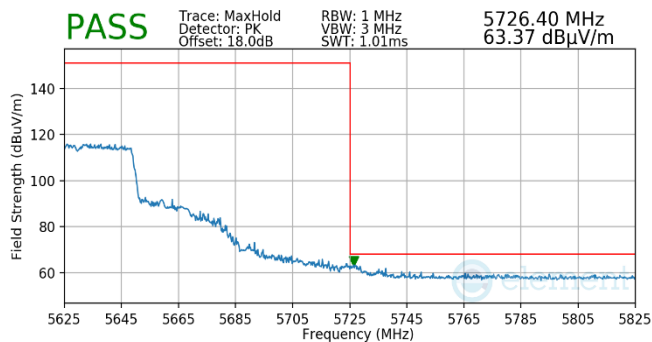
Plot 7-520. (FCC Only) Antenna WF5T (Pk, RU484, Index 65, Ch.126, MCS11)
