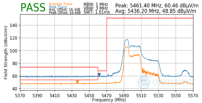
Plot 7-566. Antenna WF5B (Pk & Avg, RU52, Index 37, Ch.102, MCS11)
