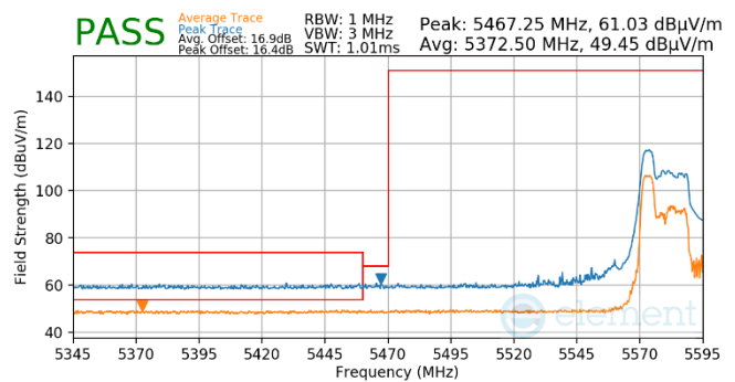
Plot 7-527. (FCC Only) Antenna WF5T (Pk & Avg, RU52, Index 37, Ch.122, MCS11)
