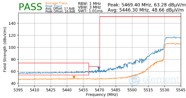
Plot 7-557. Antenna WF5B (Pk & Avg, RU242, Index 61, Ch.108, MCS11)
