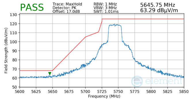
Plot 7-561. Antenna WF5B (Pk, RU242, Index 61, Ch.149, MCS11)
