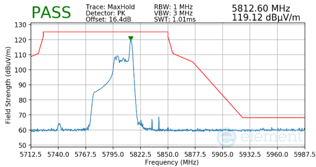
Plot 7-570. Antenna WF5B (Pk, RU26, Index 17, Ch.159, MCS11)
