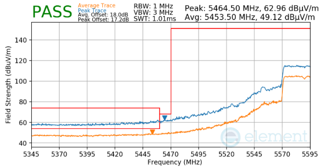
Plot 7-577. (FCC Only) Antenna WF5B (Pk & Avg, RU484, Index 65, Ch.118, MCS11)
