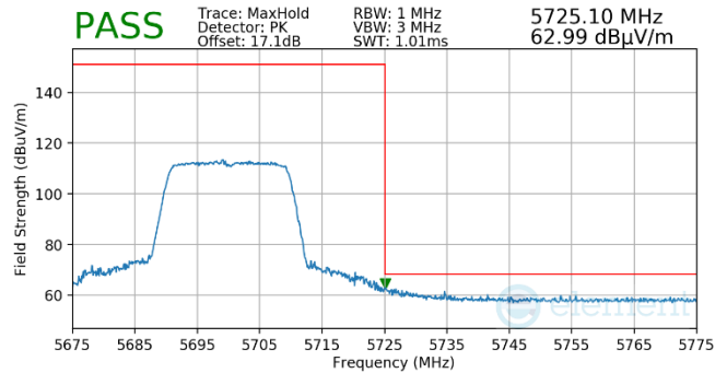
Plot 7-501. Antenna WF5T (Pk, RU242, Index 61, Ch.140, MCS11)
