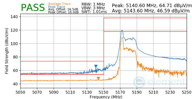
Plot 7-524. Antenna WF5T (Pk & Avg, RU26, Index 0, Ch.42, MCS11)
