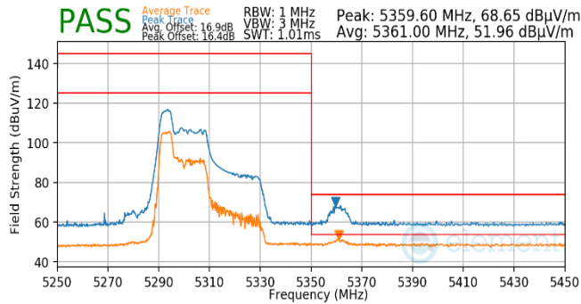
Plot 7-565. Antenna WF5B (Pk & Avg, RU52, Index 37, Ch.62, MCS11)
