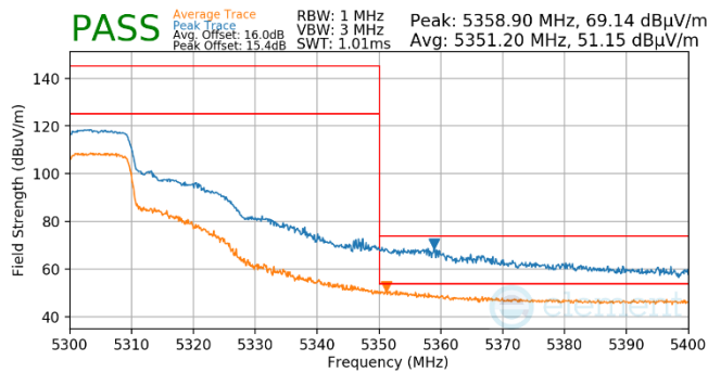
Plot 7-553. Antenna WF5B (Pk & Avg, RU242, Index 61, Ch.60, MCS11)
