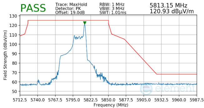
Plot 7-511. Antenna WF5T (Pk, RU26, Index 17, Ch.159, MCS11)
