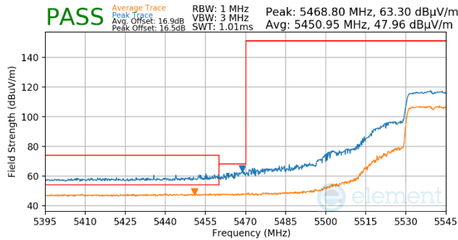
Plot 7-498. Antenna WF5T (Pk & Avg, RU242, Index 61, Ch.108, MCS11)
