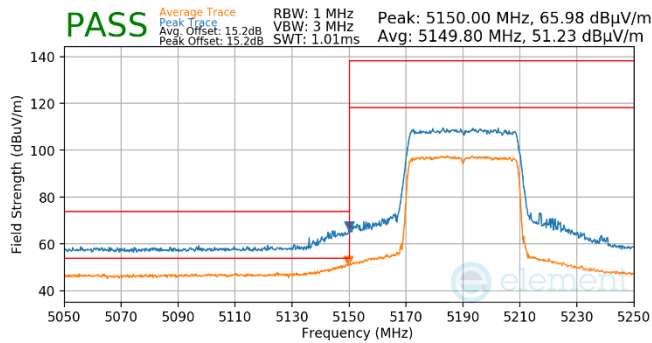
Plot 7-571. Antenna WF5B (Pk & Avg, RU484, Index 65, Ch.38, MCS11)
