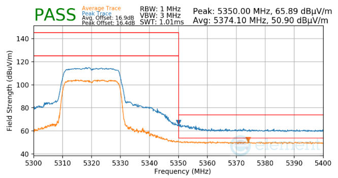
Plot 7-554. Antenna WF5B (Pk & Avg, RU242, Index 61, Ch.64, MCS11)
