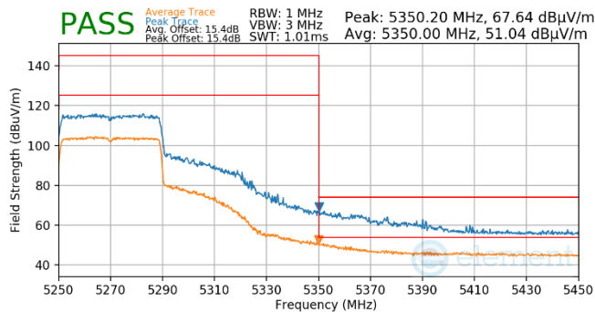
Plot 7-573. Antenna WF5B (Pk & Avg, RU484, Index 65, Ch.54, MCS11)
