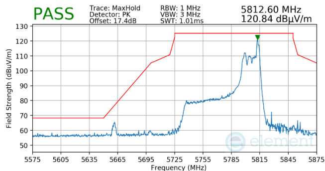
Plot 7-530. Antenna WF5T (Pk, RU26, Index 36, Ch.155, MCS11)
