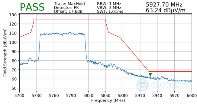
Plot 7-537. Antenna WF5T (Pk, RU996, Index 67, Ch.155, MCS11)
