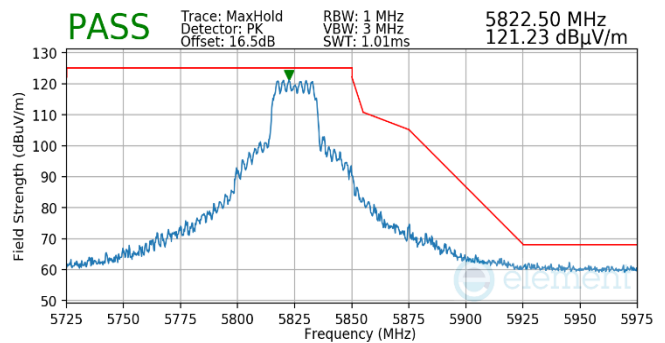
Plot 7-503. Antenna WF5T (Pk, RU242, Index 61, Ch.165, MCS11)
