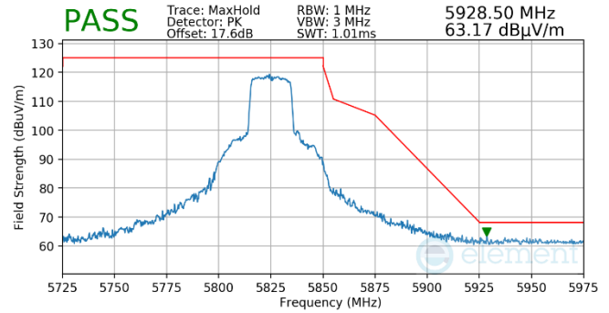
Plot 7-562. Antenna WF5B (Pk, RU242, Index 61, Ch.165, MCS11)
