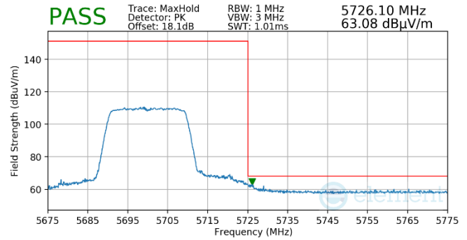
Plot 7-560. Antenna WF5B (Pk, RU242, Index 61, Ch.140, MCS11)
