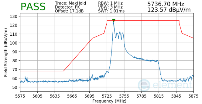
Plot 7-529. Antenna WF5T (Pk, RU26, Index 0, Ch.155, MCS11)
