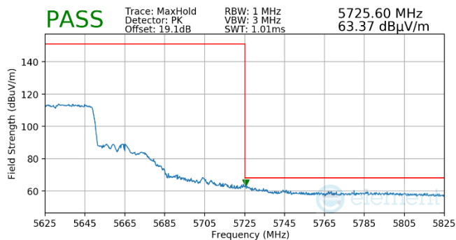
Plot 7-579. (FCC Only) Antenna WF5B (Pk, RU484, Index 65, Ch.126, MCS11)
