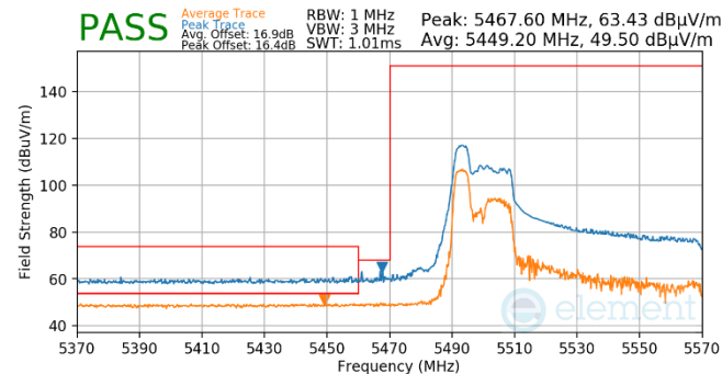
Plot 7-526. Antenna WF5T (Pk & Avg, RU52, Index 37, Ch.106, MCS11)
