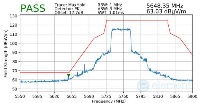
Plot 7-522. Antenna WF5T (Pk, RU484, Index 65, Ch.151, MCS11)
