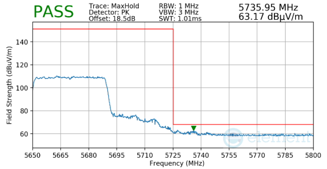
Plot 7-580. Antenna WF5B (Pk, RU484, Index 65, Ch.134, MCS11)
