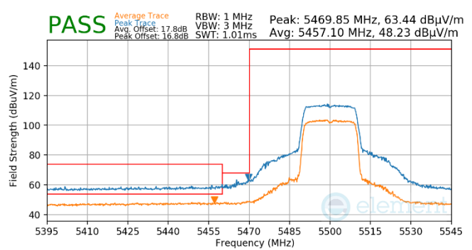
Plot 7-555. Antenna WF5B (Pk & Avg, RU242, Index 61, Ch.100, MCS11)
