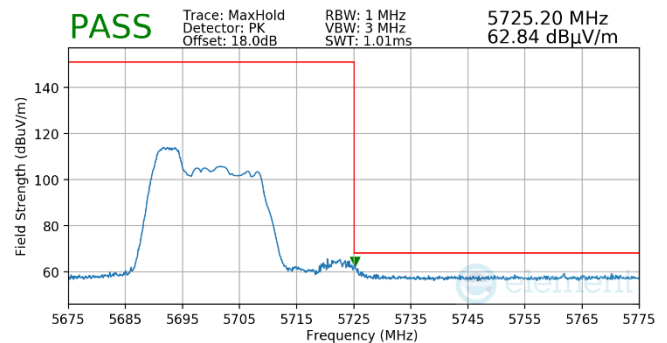
Plot 7-548. Antenna WF5B (Pk, RU52, Index 37, Ch.140, MCS11)
