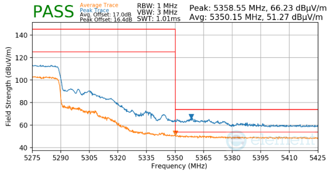
Plot 7-514. Antenna WF5T (Pk & Avg, RU484, Index 65, Ch.54, MCS11)
