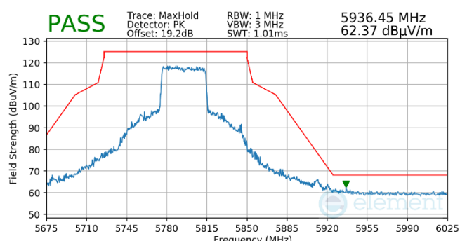
Plot 7-582. Antenna WF5B (Pk, RU484, Index 65, Ch.159, MCS11)
