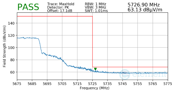
Plot 7-500. Antenna WF5T (Pk, RU242, Index 61, Ch.136, MCS11)
