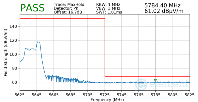
Plot 7-528. (FCC Only) Antenna WF5T (Pk, RU52, Index 52, Ch.122, MCS11)
