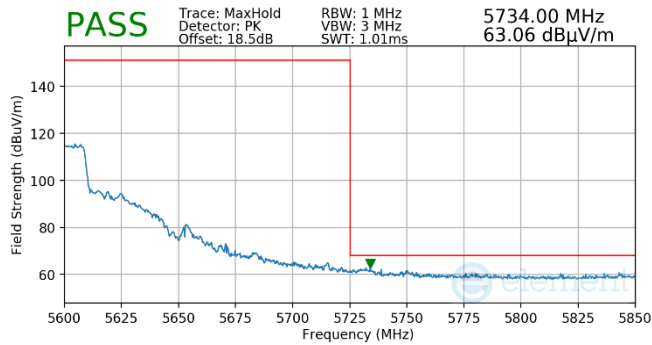
Plot 7-578. (FCC Only) Antenna WF5B (Pk, RU484, Index 65, Ch.118, MCS11)
