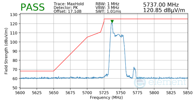
Plot 7-549. Antenna WF5B (Pk, RU26, Index 0, Ch.149, MCS11)
