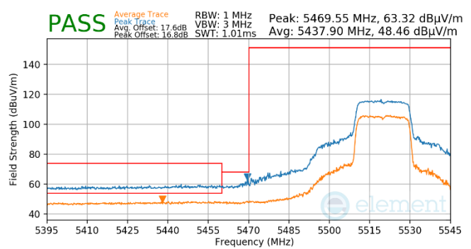
Plot 7-556. Antenna WF5B (Pk & Avg, RU242, Index 61, Ch.104, MCS11)
