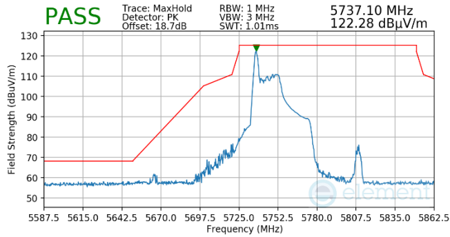
Plot 7-510. Antenna WF5T (Pk, RU26, Index 0, Ch.151, MCS11)
