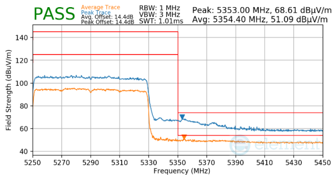
Plot 7-532. Antenna WF5T (Pk & Avg, RU996, Index 67, Ch.58, MCS11)
