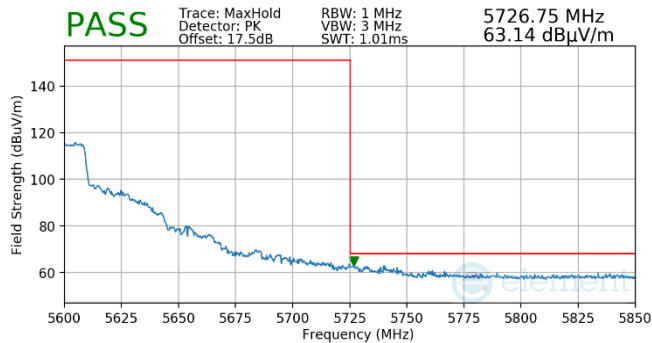
Plot 7-519. (FCC Only) Antenna WF5T (Pk, RU484, Index 65, Ch.118, MCS11)
