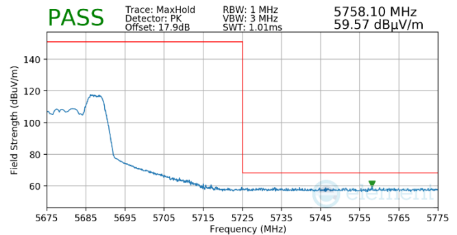
Plot 7-547. Antenna WF5B (Pk, RU52, Index 40, Ch.136, MCS11)
