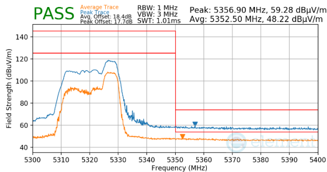
Plot 7-545. Antenna WF5B (Pk & Avg, RU52, Index 40, Ch.64, MCS11)
