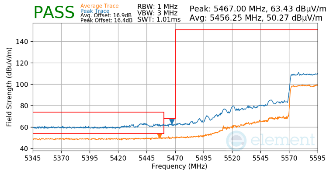
Plot 7-534. (FCC Only) Antenna WF5T (Pk & Avg, RU996, Index 67, Ch.122, MCS11)
