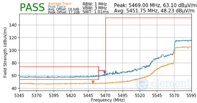
Plot 7-518. (FCC Only) Antenna WF5T (Pk & Avg, RU484, Index 65, Ch.118, MCS11)
