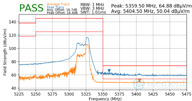
Plot 7-539. Antenna WF5T (Pk & Avg, RU52, Index 52, Ch.50, MCS11)
