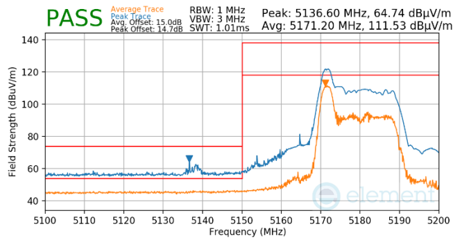
Plot 7-544. Antenna WF5B (Pk & Avg, RU26, Index 0, Ch.36, MCS11)
