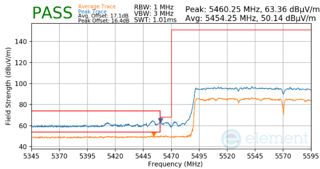
Plot 7-543. (FCC Only) Antenna WF5T (Pk & Avg, RU996x2, Index 68, Ch.114, MCS11)
