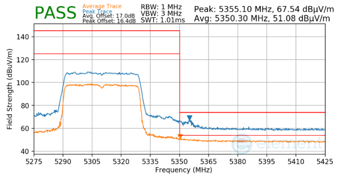
Plot 7-515. Antenna WF5T (Pk & Avg, RU484, Index 65, Ch.62, MCS11)
