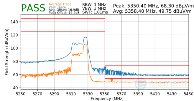
Plot 7-525. Antenna WF5T (Pk & Avg, RU52, Index 52, Ch.58, MCS11)
