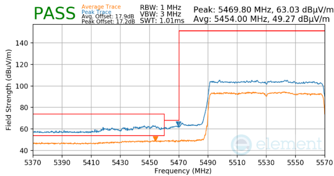
Plot 7-533. Antenna WF5T (Pk & Avg, RU996, Index 67, Ch.106, MCS11)
