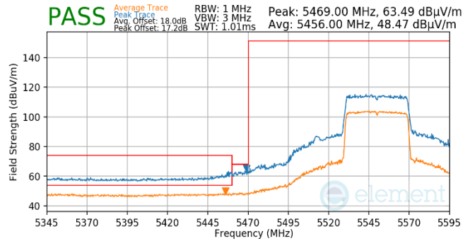
Plot 7-517. Antenna WF5T (Pk & Avg, RU484, Index 65, Ch.110, MCS11)
