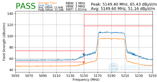
Plot 7-512. Antenna WF5T (Pk & Avg, RU484, Index 65, Ch.38, MCS11)
