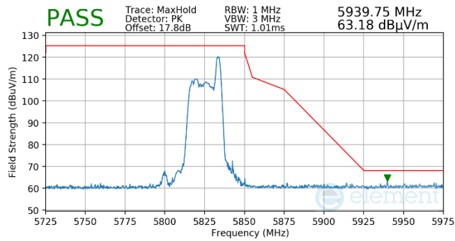
Plot 7-550. Antenna WF5B (Pk, RU26, Index 8, Ch.165, MCS11)
