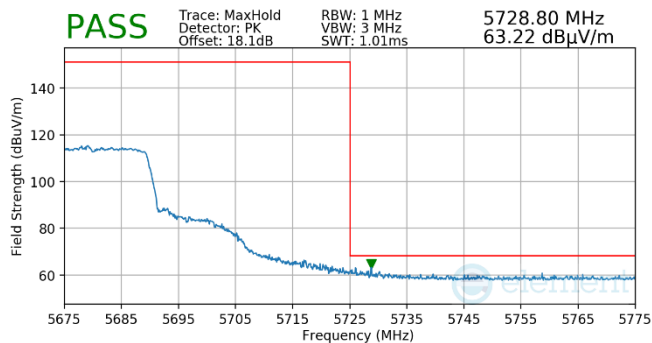
Plot 7-559. Antenna WF5B (Pk, RU242, Index 61, Ch.136, MCS11)
