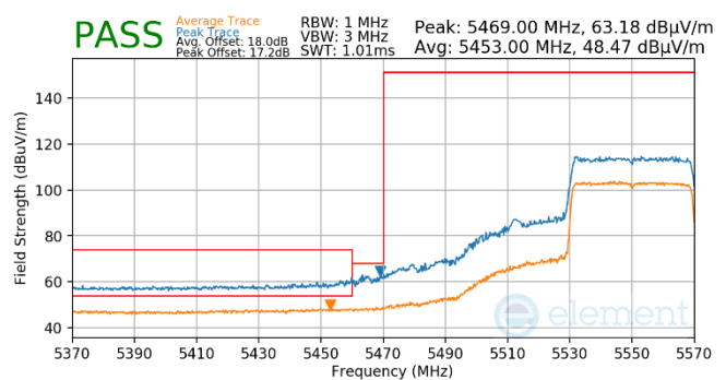
Plot 7-576. Antenna WF5B (Pk & Avg, RU484, Index 65, Ch.110, MCS11)
