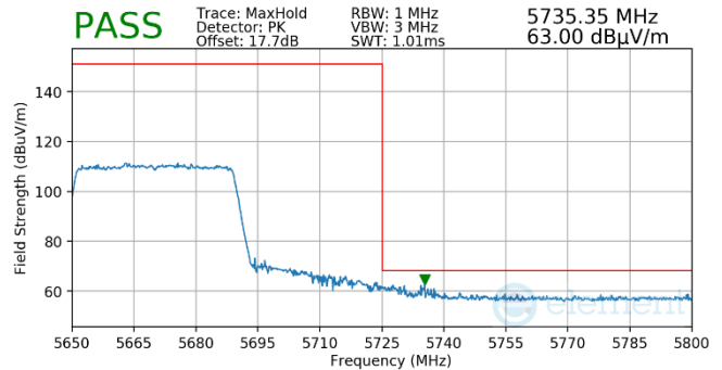
Plot 7-521. Antenna WF5T (Pk, RU484, Index 65, Ch.134, MCS11)
