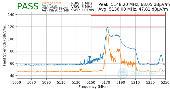
Plot 7-563. Antenna WF5B (Pk & Avg, RU26, Index 0, Ch.38, MCS11)
