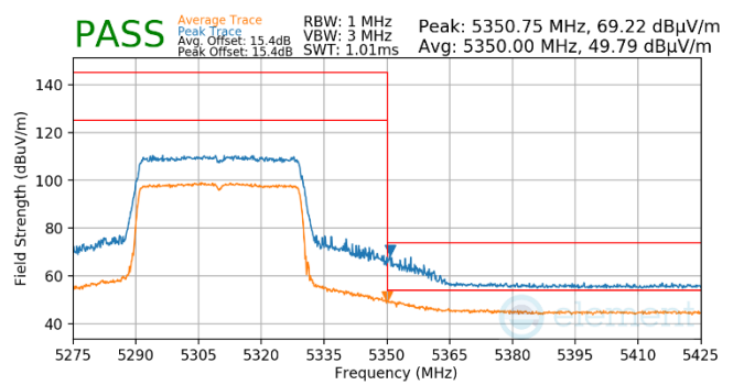
Plot 7-574. Antenna WF5B (Pk & Avg, RU484, Index 65, Ch.62, MCS11)
