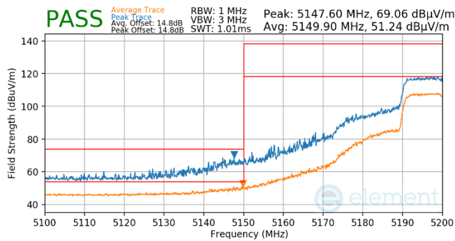
Plot 7-552. Antenna WF5B (Pk & Avg, RU242, Index 61, Ch.40, MCS11)
