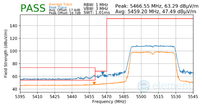
Plot 7-516. Antenna WF5T (Pk & Avg, RU484, Index 65, Ch.102, MCS11)
