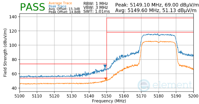
Plot 7-551. Antenna WF5B (Pk & Avg, RU242, Index 61, Ch.36, MCS11)
