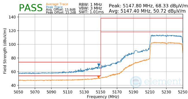
Plot 7-513. Antenna WF5T (Pk & Avg, RU484, Index 65, Ch.46, MCS11)
