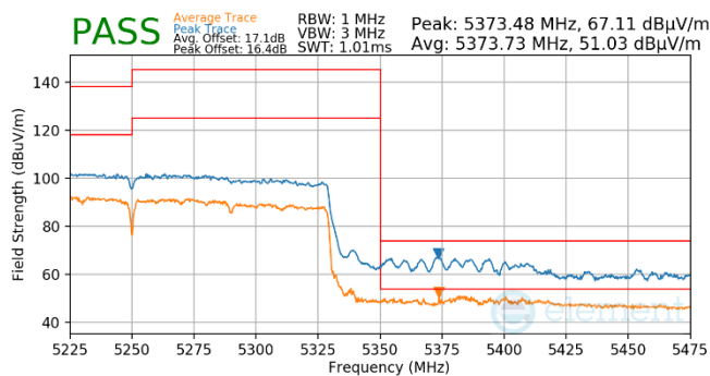
Plot 7-542. Antenna WF5T (Pk & Avg, RU996x2, Index 68, Ch.50, MCS11)
