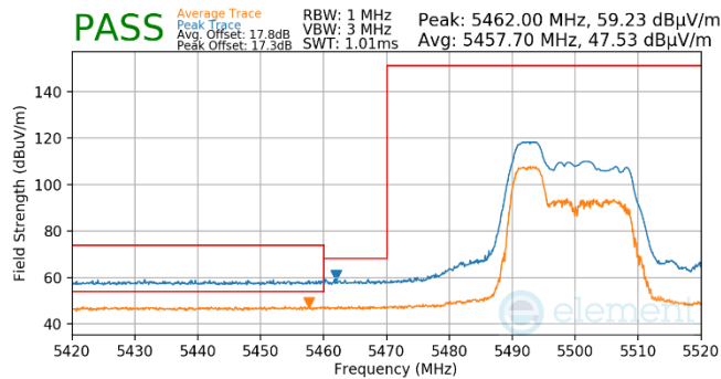
Plot 7-546. Antenna WF5B (Pk & Avg, RU52, Index 37, Ch.100, MCS11)
