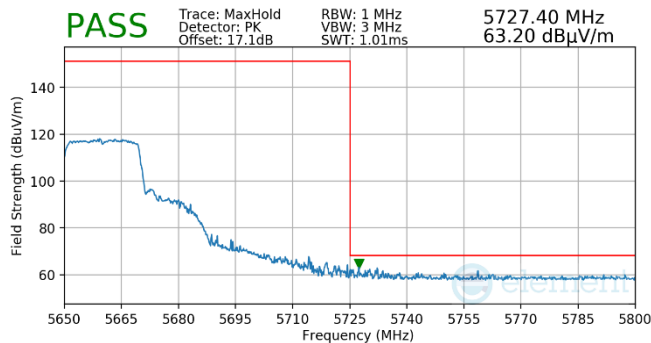
Plot 7-499. Antenna WF5T (Pk, RU242, Index 61, Ch.132, MCS11)
