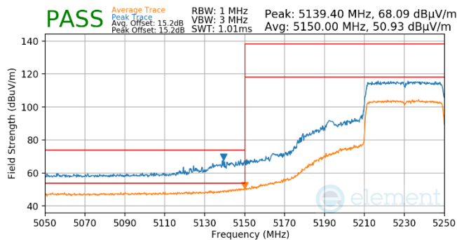
Plot 7-572. Antenna WF5B (Pk & Avg, RU484, Index 65, Ch.46, MCS11)
