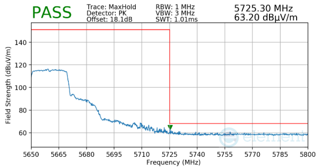
Plot 7-558. Antenna WF5B (Pk, RU242, Index 61, Ch.132, MCS11)
