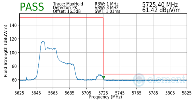
Plot 7-568. Antenna WF5B (Pk, RU52, Index 37, Ch.134, MCS11)
