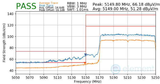
Plot 7-531. Antenna WF5T (Pk & Avg, RU996, Index 67, Ch.42, MCS11)
