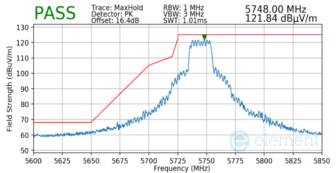
Plot 7-502. Antenna WF5T (Pk, RU242, Index 61, Ch.149, MCS11)
