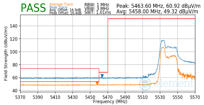
Plot 7-567. Antenna WF5B (Pk & Avg, RU52, Index 37, Ch.110, MCS11)
