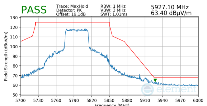
Plot 7-523. Antenna WF5T (Pk, RU484, Index 65, Ch.159, MCS11)
