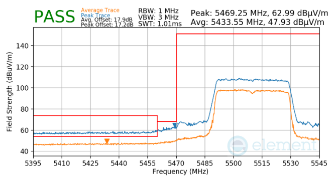
Plot 7-575. Antenna WF5B (Pk & Avg, RU484, Index 65, Ch.102, MCS11)
