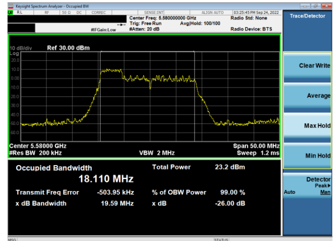
Plot 7-73. 26dB BW & 99% OBW Antenna WF5B (20MHz BW 11ax Index 37 - RU52 - Ch.116)
