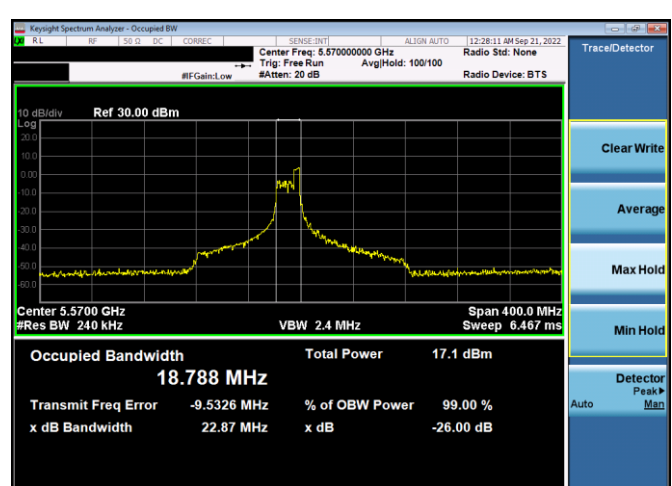
Plot 7-86. 26dB BW & 99% OBW Antenna WF5B (160MHz BW 11ax Index 52 - RU52 - Ch.114(L))
