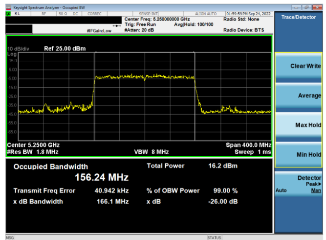
Plot 7-60. 26dB BW & 99% OBW Antenna WF5B (160MHz BW 11ax – RU996x2 – Ch.50)
