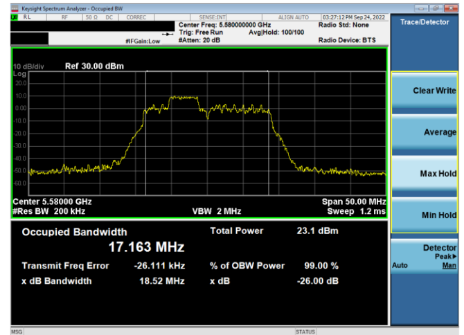
Plot 7-74. 26dB BW & 99% OBW Antenna WF5B (20MHz BW 11ax Index 38 - RU52 - Ch.116)
