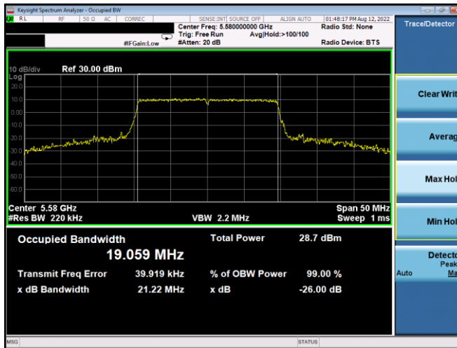
Plot 7-76. 26dB BW & 99% OBW Antenna WF5B (20MHz BW 11ax – RU242 – Ch.116)
