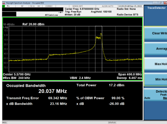
Plot 7-87. 26dB BW & 99% OBW Antenna WF5B (160MHz BW 11ax Index 52 – RU52 – Ch.114(U))
