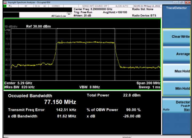
Plot 7-72. 26dB BW & 99% OBW Antenna WF5B (80MHz BW 11ax - RU996 - Ch.58)
