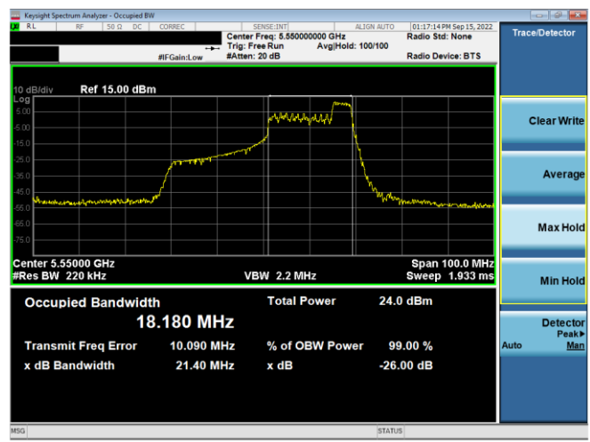
Plot 7-79. 26dB BW & 99% OBW Antenna WF5B (40MHz BW 11ax Index 44 – RU52 – Ch.110)
