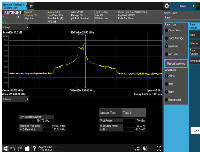
Plot 7-58. 26dB BW & 99% OBW Antenna WF5B (160MHz BW 11ax Index 52 – RU52 – Ch.50(L))
