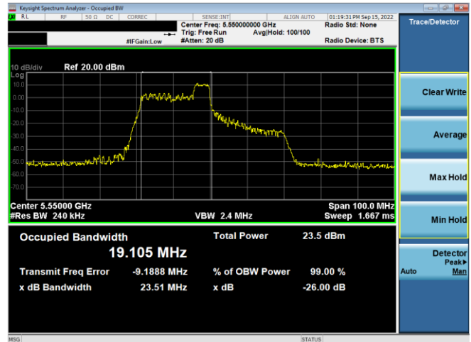
Plot 7-78. 26dB BW & 99% OBW Antenna WF5B (40MHz BW 11ax Index 40 – RU52 – Ch.110)
