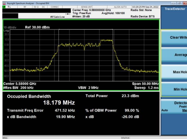
Plot 7-75. 26dB BW & 99% OBW Antenna WF5B (20MHz BW 11ax Index 40 – RU52 – Ch.116)
