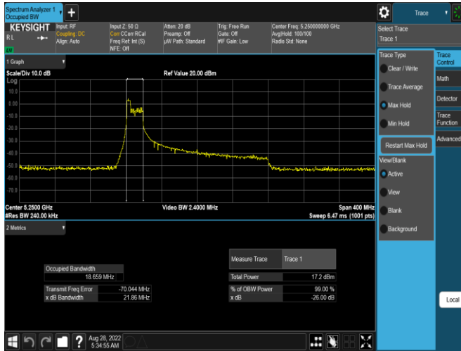
Plot 7-57. 26dB BW & 99% OBW Antenna WF5B (160MHz BW 11ax Index 37 – RU52 – Ch.50(L))
