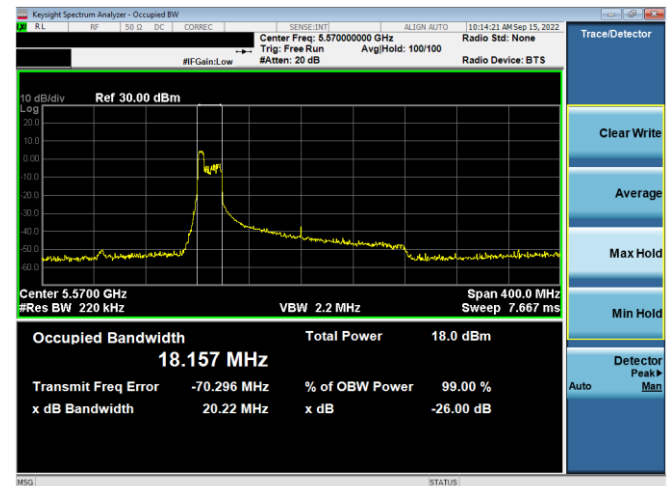
Plot 7-85. 26dB BW & 99% OBW Antenna WF5B (160MHz BW 11ax Index 37 - RU52 - Ch.114(L))
