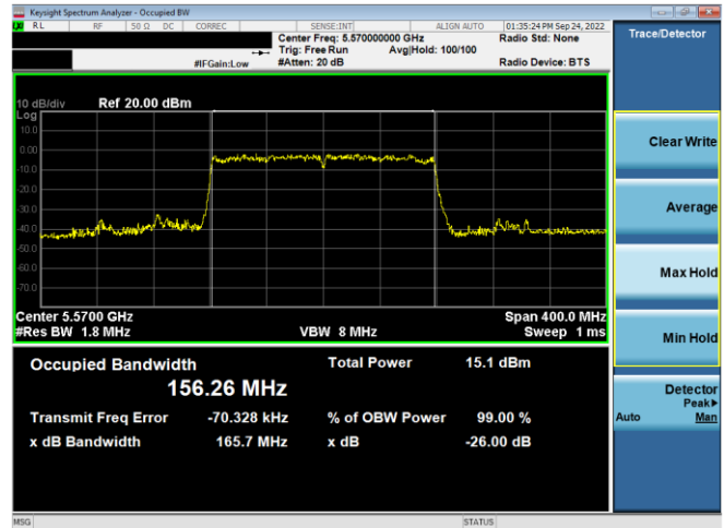
Plot 7-88. 26dB BW & 99% OBW Antenna WF5B (160MHz BW 11ax – RU996x2 – Ch.114)
