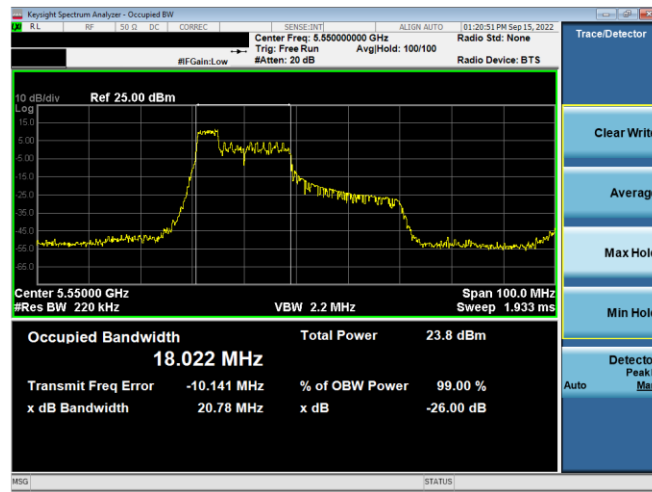
Plot 7-77. 26dB BW & 99% OBW Antenna WF5B (40MHz BW 11ax Index 37 – RU52 – Ch.110)
