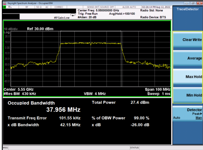
Plot 7-80. 26dB BW & 99% OBW Antenna WF5B (40MHz BW 11ax – RU484 – Ch.110)
