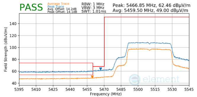
Plot 7-984. Antenna WF5b (Pk & Avg, Ch.102, 80.11ax(SU), MCS2)
