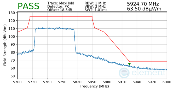
Plot 7-1048. Antenna WF5b (Pk, Ch.155, 802.11ax(SU), MCS4)
