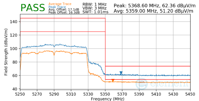
Plot 7-1012. Antenna WF5b (Pk & Avg, Ch.58, 802.11ac, MCS4)
