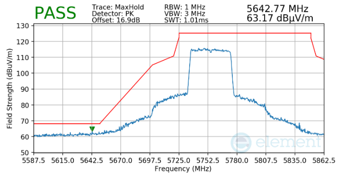
Plot 7-1002. Antenna WF5b (Pk, Ch.151, 80.11ax(SU), MCS2)
