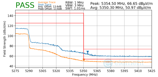
Plot 7-978. Antenna WF5b (Pk & Avg, Ch.54, 80.11ax(SU), MCS2)
