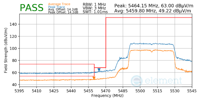
Plot 7-985. Antenna WF5b (Pk & Avg, Ch.102, 80.11ax(SU), MCS4)
