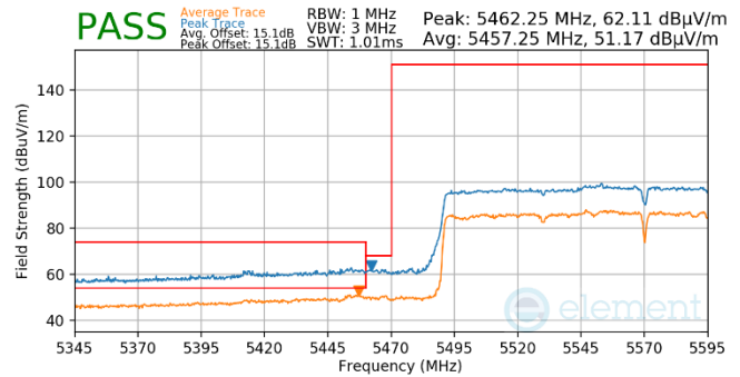
Plot 7-1065. (FCC Only) Antenna WF5b (Pk & Avg, Ch.114, 802.11ax(SU), MCS2)
