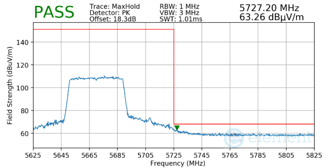
Plot 7-1001. Antenna WF5b (Pk, Ch.134, 80.11ax(SU), MCS11)
