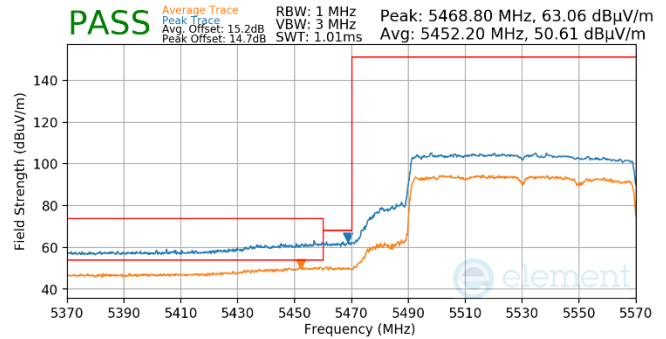
Plot 7-1035. Antenna WF5b (Pk & Avg, Ch.106, 802.11ax(SU), MCS2)
