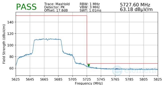
Plot 7-999. Antenna WF5b (Pk, Ch.134, 80.11ax(SU), MCS2)
