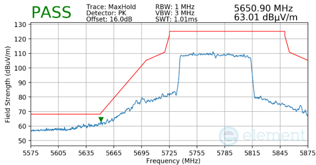
Plot 7-1025. Antenna WF5b (Pk, Ch.155, 802.11ac, MCS9)
