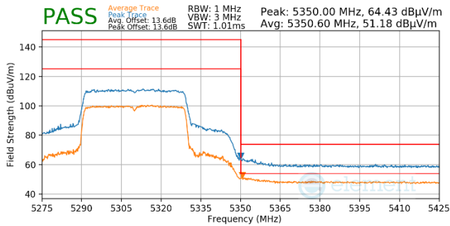
Plot 7-982. Antenna WF5b (Pk & Avg, Ch.62, 80.11ax(SU), MCS4)
