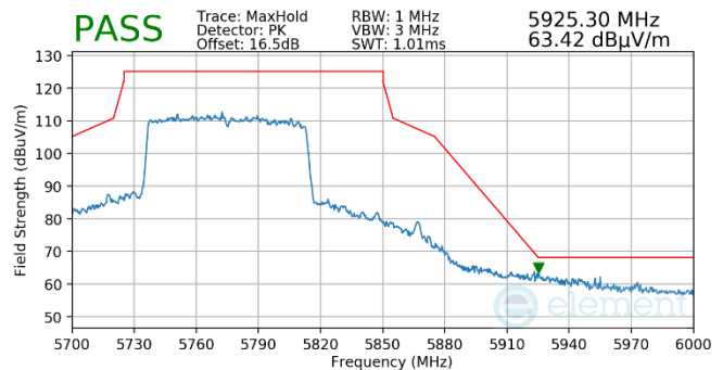
Plot 7-1028. Antenna WF5b (Pk, Ch.155, 802.11ac, MCS9)
