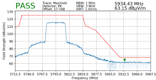
Plot 7-1005. Antenna WF5b (Pk, Ch.159, 80.11ax(SU), MCS2)
