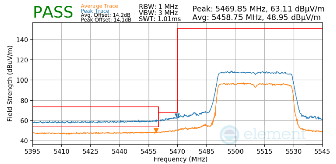
Plot 7-986. Antenna WF5b (Pk & Avg, Ch.102, 80.11ax(SU), MCS11)
