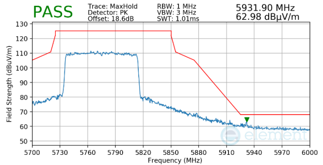
Plot 7-1049. Antenna WF5b (Pk, Ch.155, 802.11ax(SU), MCS11)
