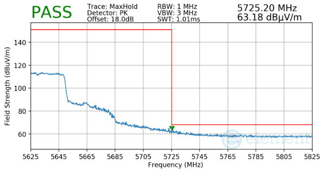
Plot 7-997. (FCC Only) Antenna WF5b (Pk, Ch.126, 80.11ax(SU), MCS4)
