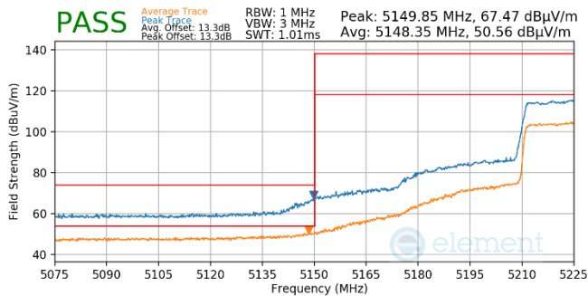
Plot 7-975. Antenna WF5b (Pk & Avg, Ch.46, 80.11ax(SU), MCS2)
