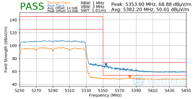
Plot 7-1034. Antenna WF5b (Pk & Avg, Ch.58, 802.11ax(SU), MCS11)
