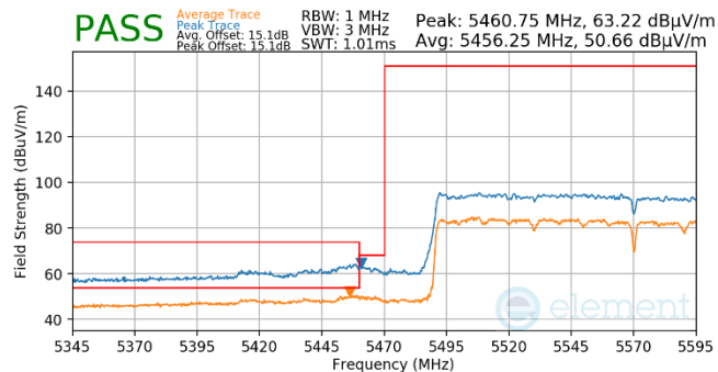
Plot 7-1067. (FCC Only) Antenna WF5b (Pk & Avg, Ch.114, 802.11ax(SU), MCS11)
