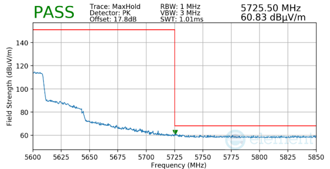
Plot 7-993. (FCC Only) Antenna WF5b (Pk, Ch.118, 80.11ax(SU), MCS2)
