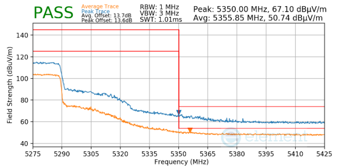
Plot 7-979. Antenna WF5b (Pk & Avg, Ch.54, 80.11ax(SU), MCS4)
