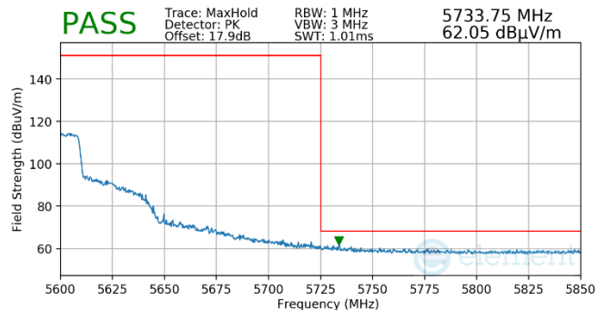
Plot 7-994. (FCC Only) Antenna WF5b (Pk, Ch.118, 80.11ax(SU), MCS4)
