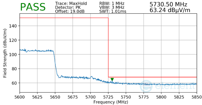
Plot 7-1022. (FCC Only) Antenna WF5b (Pk, Ch.122, 802.11ac, MCS9)
