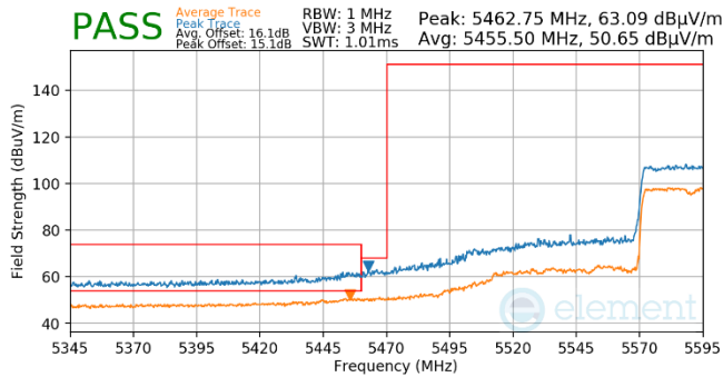
Plot 7-1040. (FCC Only) Antenna WF5b (Pk & Avg, Ch.122, 802.11ax(SU), MCS11)
