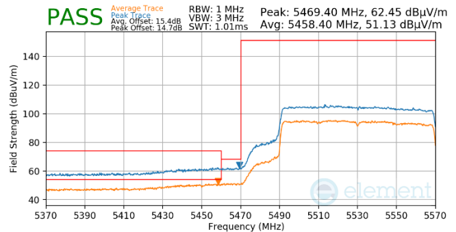
Plot 7-1036. Antenna WF5b (Pk & Avg, Ch.106, 802.11ax(SU), MCS4)
