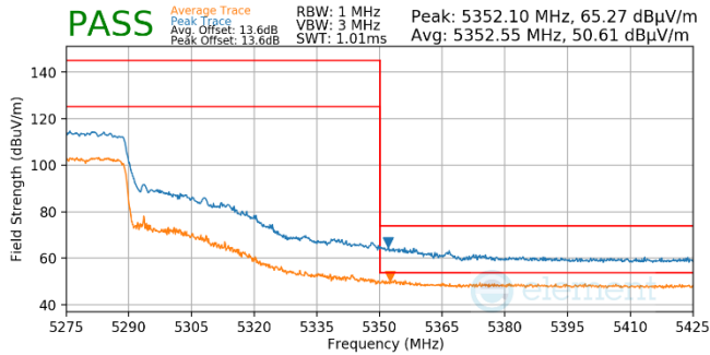
Plot 7-980. Antenna WF5b (Pk & Avg, Ch.54, 80.11ax(SU), MCS11)
