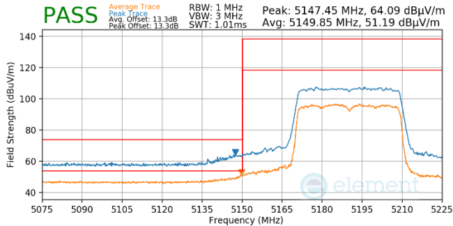
Plot 7-974. Antenna WF5b (Pk & Avg, Ch.38, 80.11ax(SU), MCS11)
