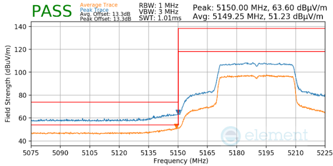
Plot 7-972. Antenna WF5b (Pk & Avg, Ch.38, 80.11ax(SU), MCS2)
