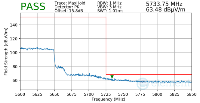
Plot 7-1042. (FCC Only) Antenna WF5b (Pk, Ch.122, 802.11ax(SU), MCS4)
