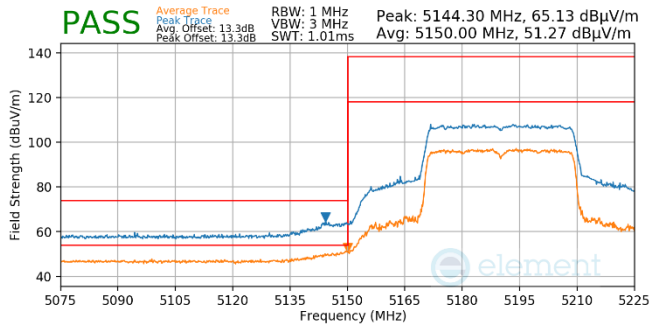
Plot 7-973. Antenna WF5b (Pk & Avg, Ch.38, 80.11ax(SU), MCS4)
