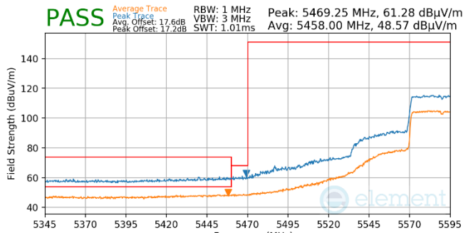
Plot 7-990. (FCC Only) Antenna WF5b (Pk, Ch.118, 80.11ax(SU), MCS2)
