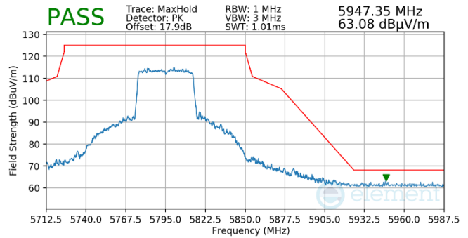
Plot 7-1007. Antenna WF5b (Pk, Ch.159, 80.11ax(SU), MCS11)
