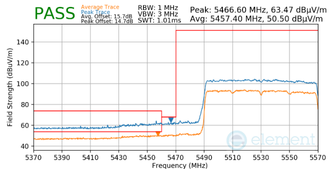
Plot 7-1037. Antenna WF5b (Pk & Avg, Ch.106, 802.11ax(SU), MCS11)
