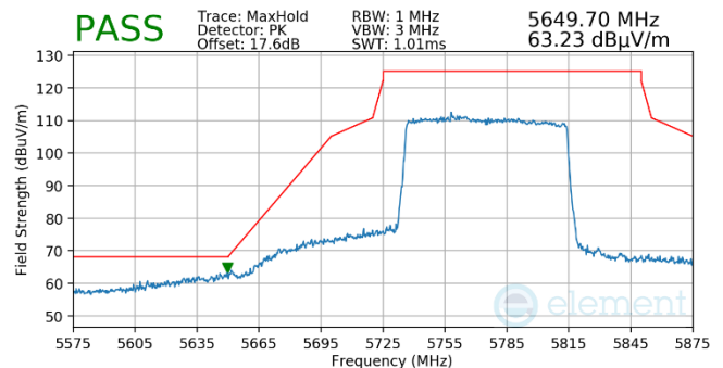
Plot 7-1044. Antenna WF5b (Pk, Ch.155, 802.11ax(SU), MCS2)
