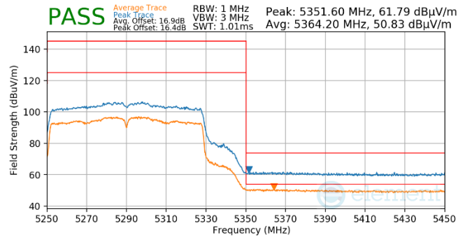
Plot 7-1011. Antenna WF5b (Pk & Avg, Ch.58, 802.11ac, MCS2)
