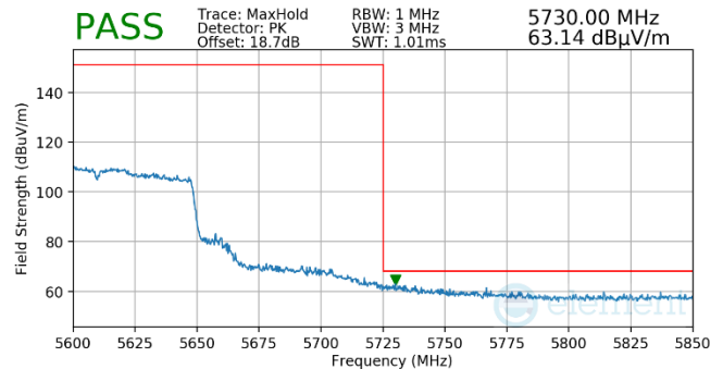
Plot 7-1021. (FCC Only) Antenna WF5b (Pk, Ch.122, 802.11ac, MCS4)
