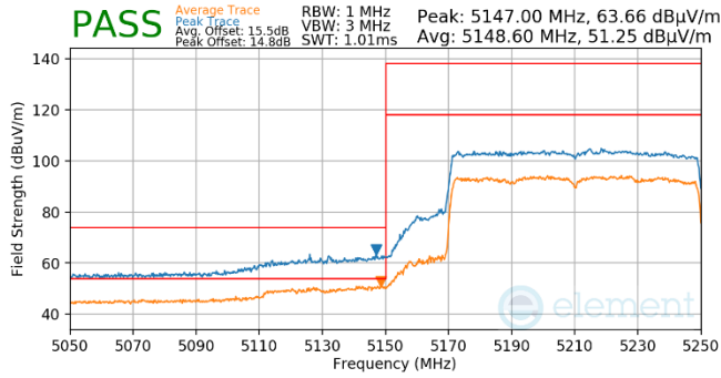
Plot 7-1030. Antenna WF5b (Pk & Avg, Ch.42, 802.11ax(SU), MCS4)
