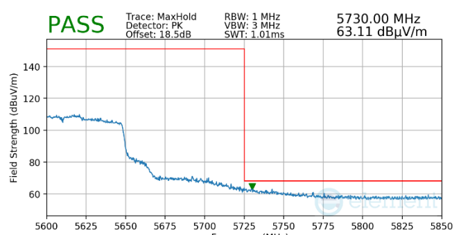
Plot 7-1020. (FCC Only) Antenna WF5b (Pk, Ch.122, 802.11ac, MCS2)
