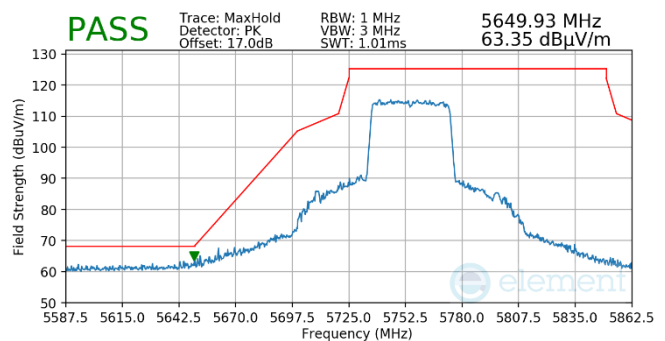
Plot 7-1003. Antenna WF5b (Pk, Ch.151, 80.11ax(SU), MCS4)
