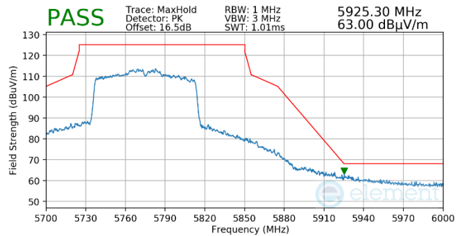
Plot 7-1026. Antenna WF5b (Pk, Ch.155, 802.11ac, MCS2)
