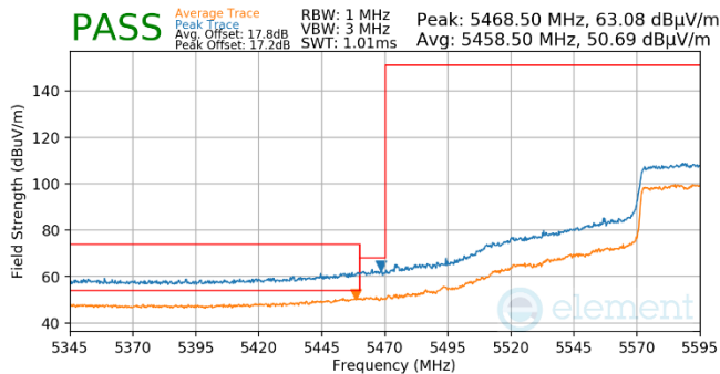
Plot 7-1017. (FCC Only) Antenna WF5b (Pk & Avg, Ch.122, 802.11ac, MCS2)
