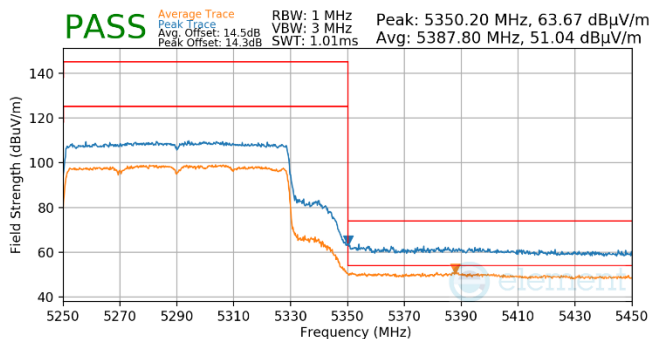
Plot 7-1033. Antenna WF5b (Pk & Avg, Ch.58, 802.11ax(SU), MCS4)
