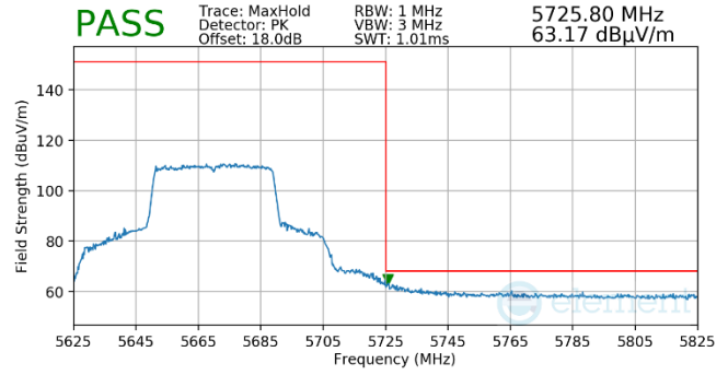
Plot 7-1000. Antenna WF5b (Pk, Ch.134, 80.11ax(SU), MCS4)
