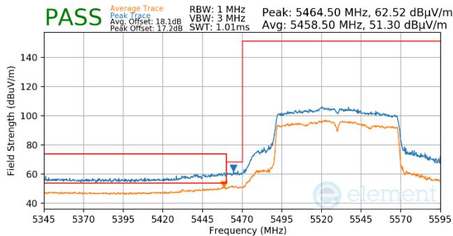
Plot 7-1015. Antenna WF5b (Pk & Avg, Ch.106, 802.11ac, MCS4)
