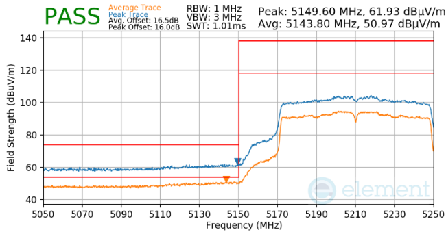
Plot 7-1008. Antenna WF5b (Pk & Avg, Ch.42, 802.11ac, MCS2)
