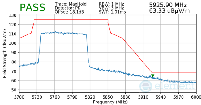
Plot 7-1047. Antenna WF5b (Pk, Ch.155, 802.11ax(SU), MCS2)
