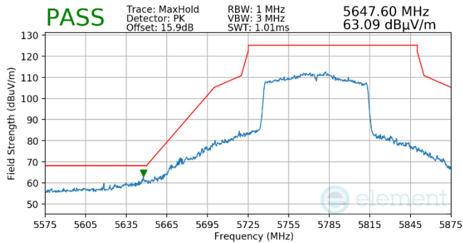
Plot 7-1024. Antenna WF5b (Pk, Ch.155, 802.11ac, MCS4)
