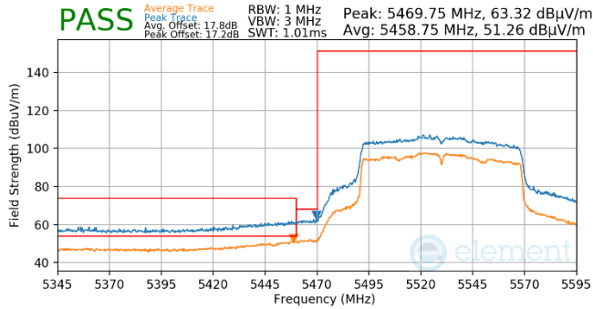
Plot 7-1014. Antenna WF5b (Pk & Avg, Ch.106, 802.11ac, MCS2)
