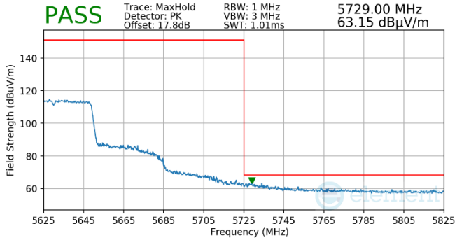
Plot 7-996. (FCC Only) Antenna WF5b (Pk, Ch.126, 80.11ax(SU), MCS2)
