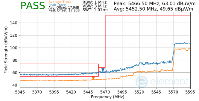
Plot 7-1019. (FCC Only) Antenna WF5b (Pk & Avg, Ch.122, 802.11ac, MCS9)
