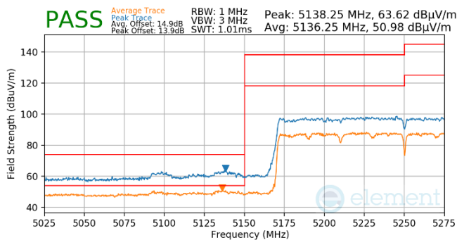
Plot 7-1061 Antenna WF5b (Pk & Avg, Ch.50, 802.11ax(SU), MCS11)
