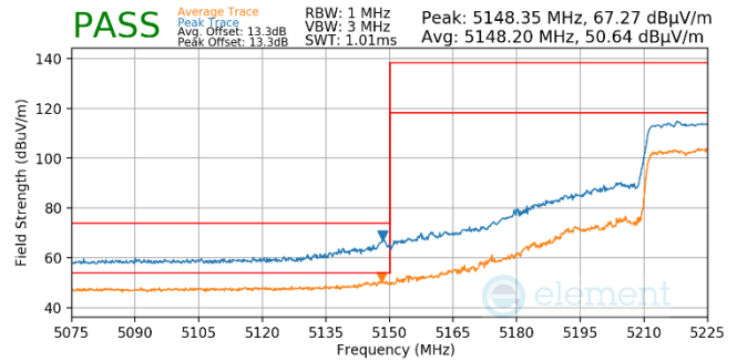
Plot 7-977. Antenna WF5b (Pk & Avg, Ch.46, 80.11ax(SU), MCS11)
