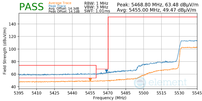
Plot 7-988. Antenna WF5b (Pk & Avg, Ch.110, 80.11ax(SU), MCS4)
