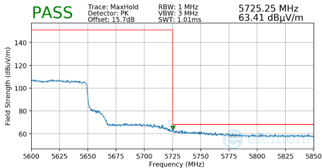
Plot 7-1041. (FCC Only) Antenna WF5b (Pk, Ch.122, 802.11ax(SU), MCS2)
