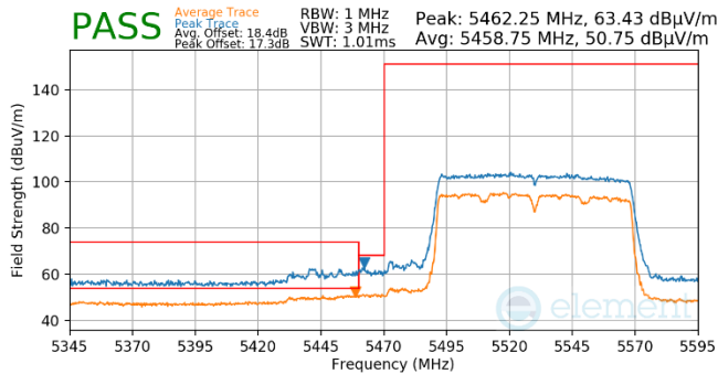
Plot 7-1016. Antenna WF5b (Pk & Avg, Ch.106, 802.11ac, MCS9)
