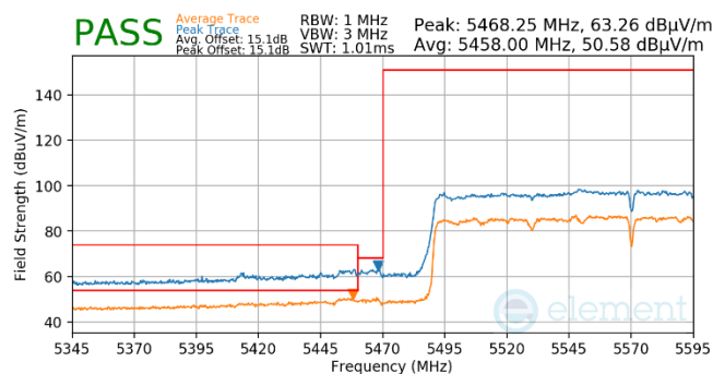
Plot 7-1066. (FCC Only) Antenna WF5b (Pk & Avg, Ch.114, 802.11ax(SU), MCS4) (Pk & Avg, Ch.114)
