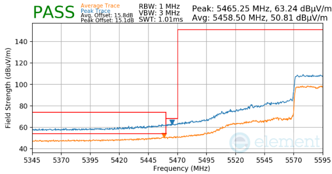
Plot 7-1039. (FCC Only) Antenna WF5b (Pk & Avg, Ch.122, 802.11ax(SU), MCS3)
