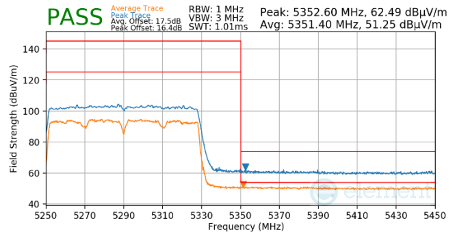
Plot 7-1013. Antenna WF5b (Pk & Avg, Ch.58, 802.11ac, MCS9)
