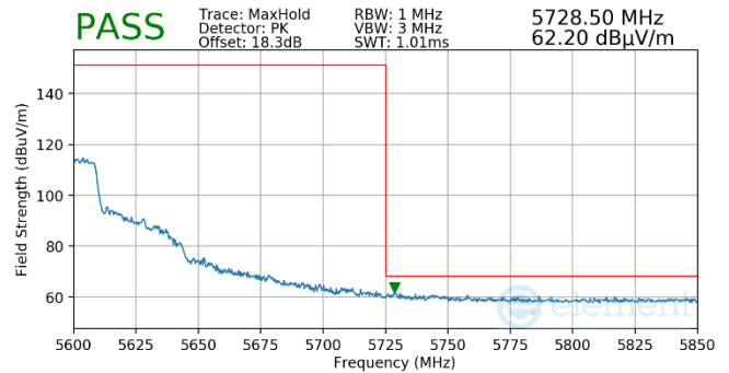
Plot 7-995. (FCC Only) Antenna WF5b (Pk, Ch.118, 80.11ax(SU), MCS11)
