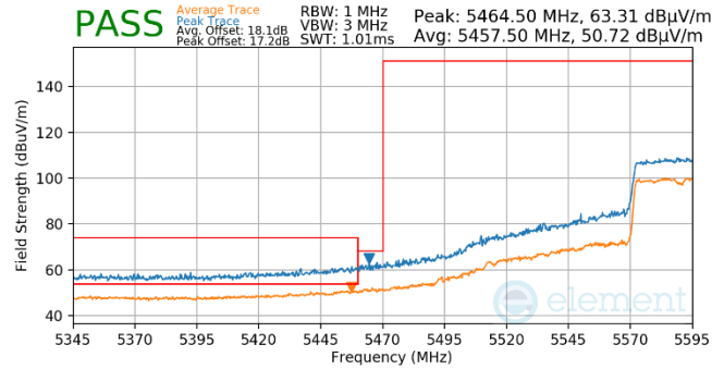
Plot 7-1018. (FCC Only) Antenna WF5b (Pk & Avg, Ch.122, 802.11ac, MCS4)
