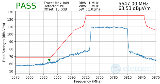
Plot 7-1046. Antenna WF5b (Pk, Ch.155, 802.11ax(SU), MCS11)
