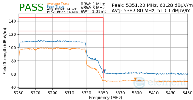
Plot 7-1032. Antenna WF5b (Pk & Avg, Ch.58, 802.11ax(SU), MCS2)
