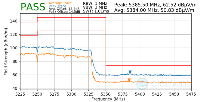
Plot 7-1063. Antenna WF5b (Pk & Avg, Ch.50, 802.11ax(SU), MCS4)
