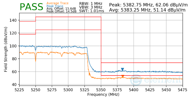
Plot 7-1064. Antenna WF5b (Pk & Avg, Ch.50, 802.11ax(SU), MCS11)
