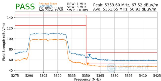
Plot 7-983. Antenna WF5b (Pk & Avg, Ch.62, 80.11ax(SU), MCS11)
