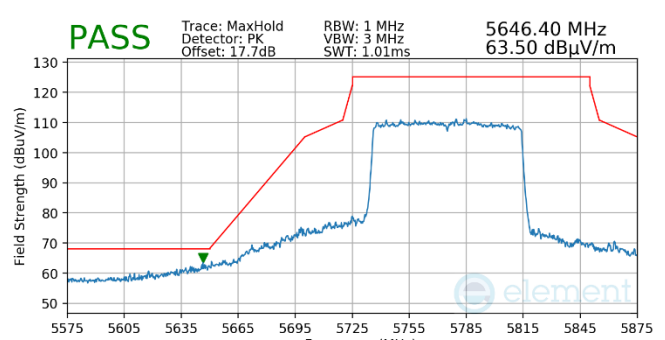
Plot 7-1045. Antenna WF5b (Pk, Ch.155, 802.11ax(SU), MCS4)
