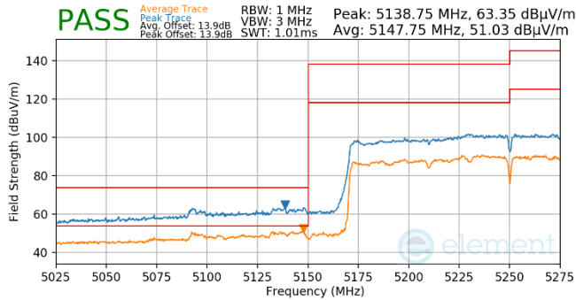
Plot 7-1060. Antenna WF5b (Pk & Avg, Ch.50, 802.11ax(SU), MCS4)
