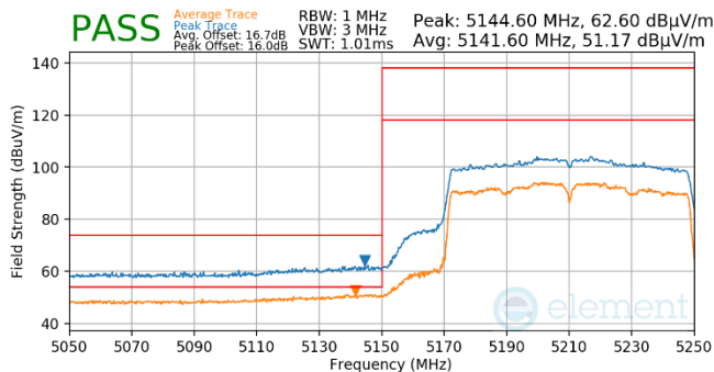
Plot 7-1009. Antenna WF5b (Pk & Avg, Ch.42, 802.11ac, MCS4)
