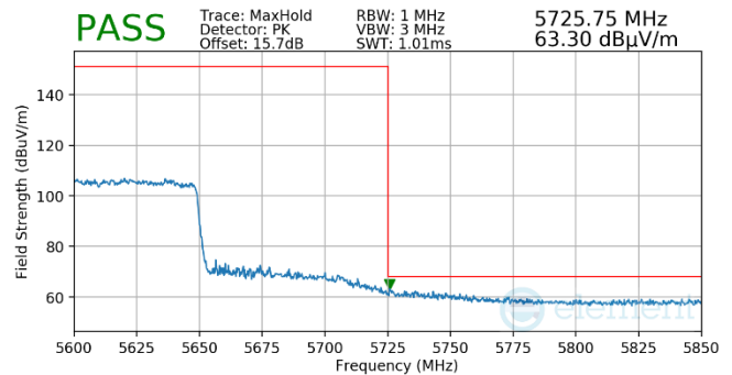
Plot 7-1043. (FCC Only) Antenna WF5b (Pk, Ch.122, 802.11ax(SU), MCS11)
