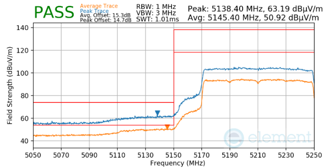
Plot 7-1029. Antenna WF5b (Pk & Avg, Ch.42, 802.11ax(SU), MCS2)
