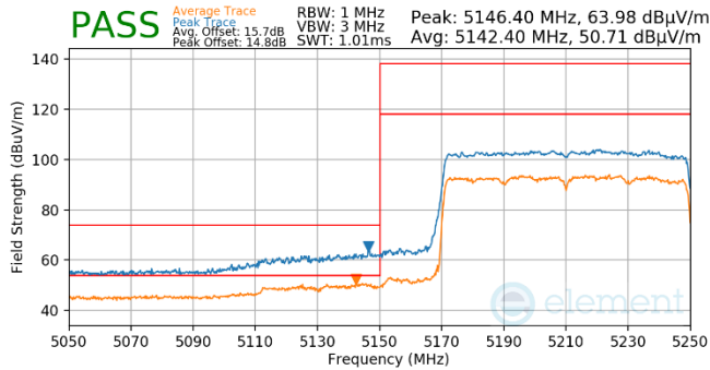
Plot 7-1031. Antenna WF5b (Pk & Avg, Ch.42, 802.11ax(SU), MCS11)
