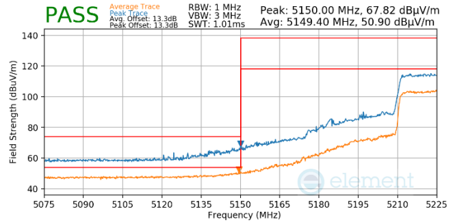
Plot 7-976. Antenna WF5b (Pk & Avg, Ch.46, 80.11ax(SU), MCS4)
