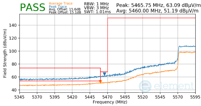
Plot 7-1038. (FCC Only) Antenna WF5b (Pk & Avg, Ch.122, 802.11ax(SU), MCS0)
