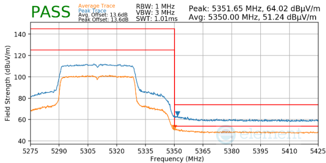
Plot 7-981. Antenna WF5b (Pk & Avg, Ch.62, 80.11ax(SU), MCS2)
