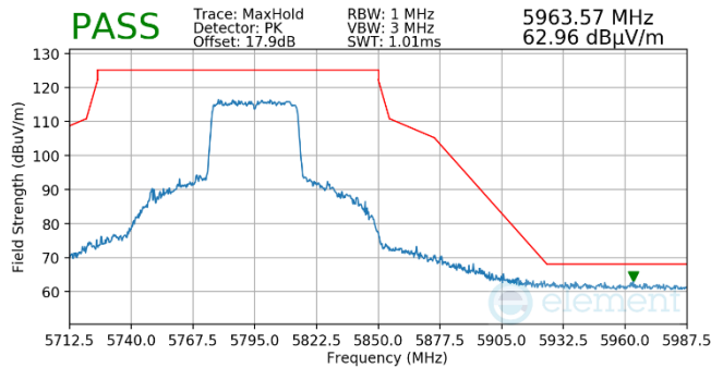
Plot 7-1006. Antenna WF5b (Pk, Ch.159, 80.11ax(SU), MCS4)
