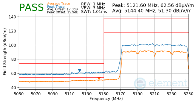
Plot 7-1010. Antenna WF5b (Pk & Avg, Ch.42, 802.11ac, MCS9)
