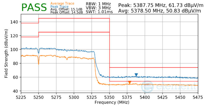
Plot 7-1062. Antenna WF5b (Pk & Avg, Ch.50, 802.11ax(SU), MCS2)
