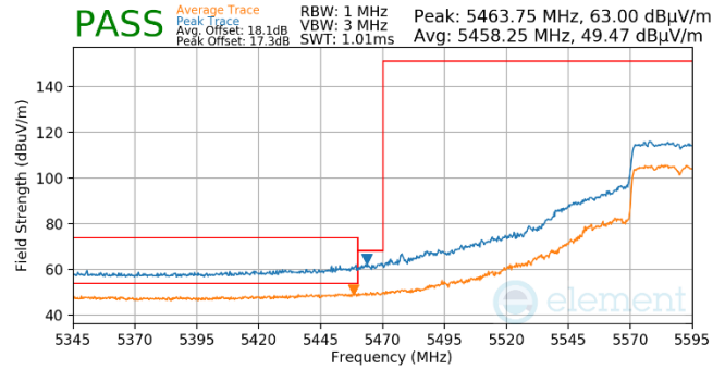
Plot 7-992. (FCC Only) Antenna WF5b (Pk & Avg, Ch.118, 80.11ax(SU), MCS11)
