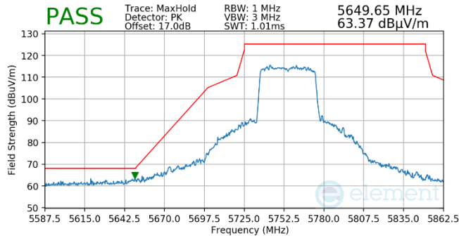
Plot 7-1004. Antenna WF5b (Pk, Ch.151, 80.11ax(SU), MCS11)
