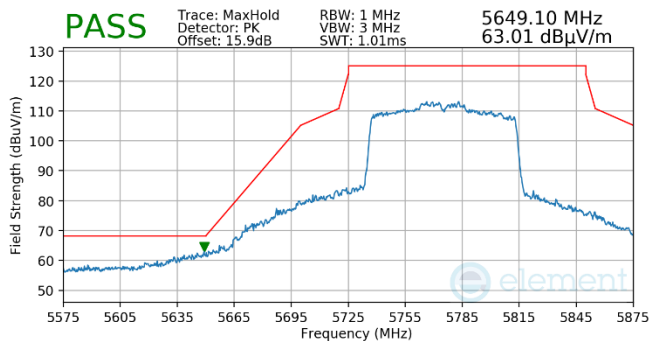
Plot 7-1023. Antenna WF5b (Pk, Ch.155, 802.11ac, MCS2)
