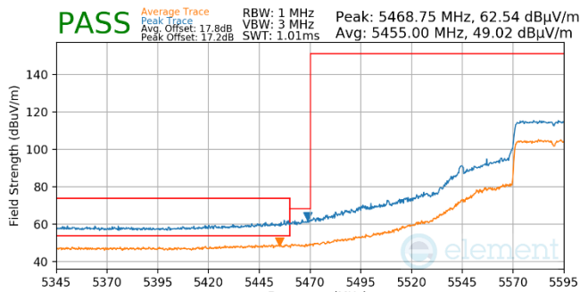
Plot 7-991. (FCC Only) Antenna WF5b (Pk, Ch.118, 80.11ax(SU), MCS4)
