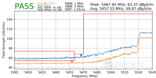
Plot 7-989. Antenna WF5b (Pk & Avg, Ch.110, 80.11ax(SU), MCS11)
