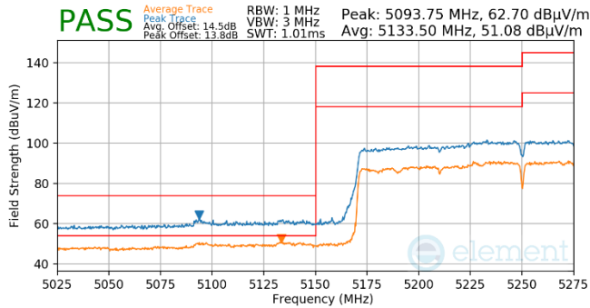
Plot 7-1059. Antenna WF5b (Pk & Avg, Ch.50, 802.11ax(SU), MCS2)
