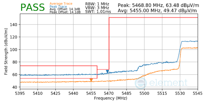
Plot 7-987. Antenna WF5b (Pk & Avg, Ch.110, 80.11ax(SU), MCS2)
