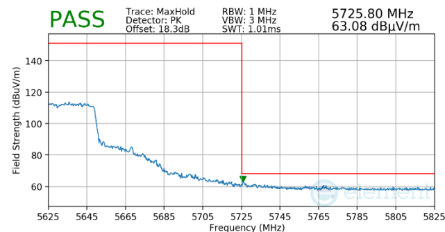
Plot 7-998. (FCC Only) Antenna WF5b (Pk, Ch.126, 80.11ax(SU), MCS2)
