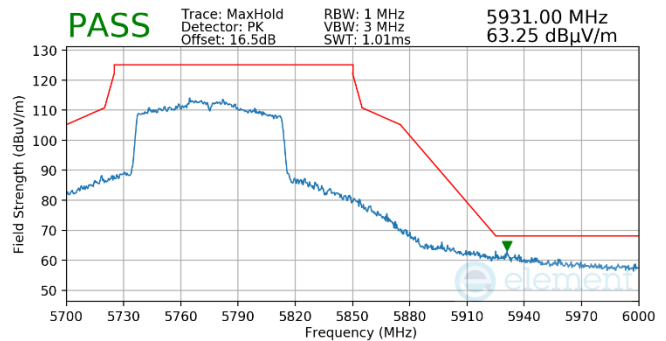
Plot 7-1027. Antenna WF5b (Pk, Ch.155, 802.11ac, MCS4)
