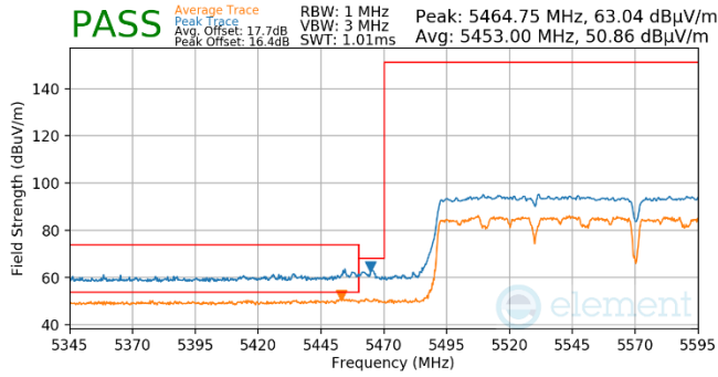
Plot 7-1058. Antenna WF5b (FCC Only) (Pk & Avg. CH. 114, 802.11ac, MCS9)
