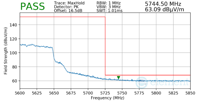
Plot 7-829. (FCC Only) Antenna WF5t (Pk, Ch.122, 802.11ac, MCS2)
