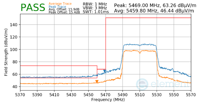
Plot 7-798. Antenna WF5t (Pk & Avg, Ch.102, 80.11ax(SU), MCS11)
