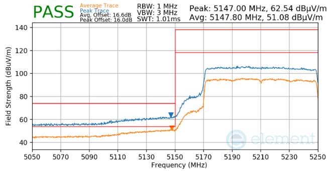
Plot 7-838. Antenna WF5t (Pk & Avg, Ch.42, 802.11ax(SU), MCS2)
