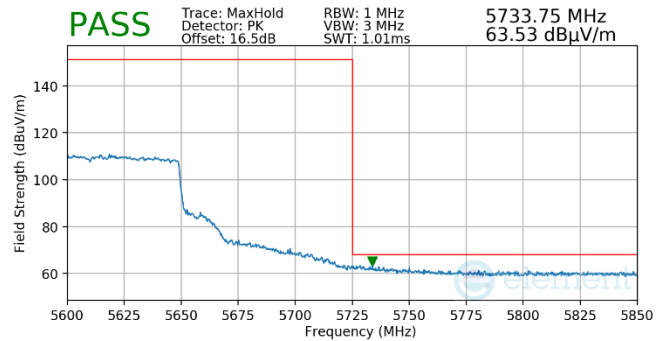
Plot 7-851. (FCC Only) Antenna WF5t (Pk, Ch.122, 802.11ax(SU), MCS4)
