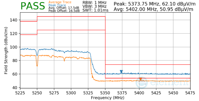
Plot 7-862. Antenna WF5t (Pk & Avg, Ch.50, 802.11ac, MCS2)
