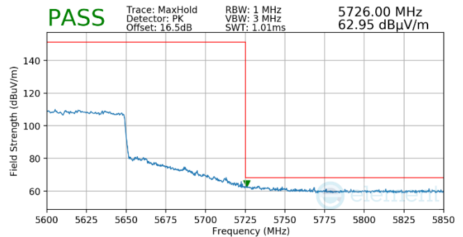
Plot 7-852. (FCC Only) Antenna WF5t (Pk, Ch.122, 802.11ax(SU), MCS11)
