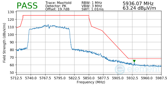
Plot 7-835. Antenna WF5t (Pk, Ch.155, 802.11ac, MCS2)
