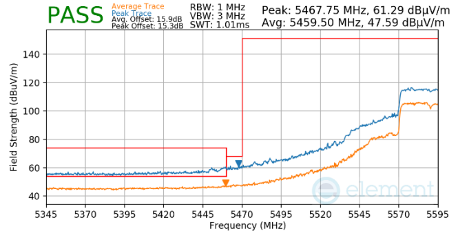
Plot 7-804. (FCC Only) Antenna WF5t (Pk & Avg, Ch.118, 80.11ax(SU),MCS11)
