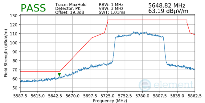
Plot 7-832. Antenna WF5t (Pk, Ch.155, 802.11ac, MCS2)
