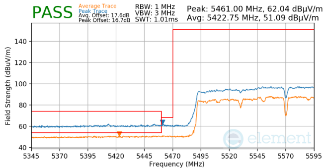
Plot 7-866. (FCC Only) Antenna WF5t (Pk & Avg, Ch.114, 802.11n, MCS4)
