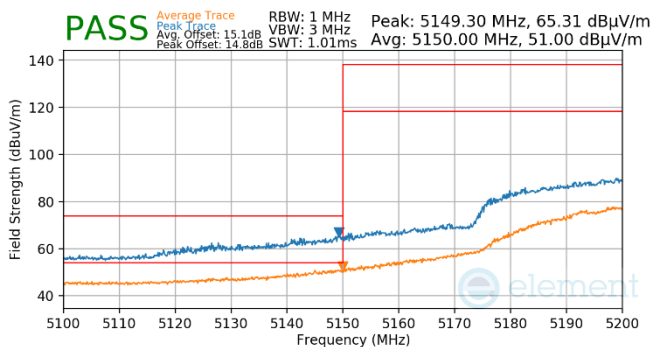
Plot 7-787. Antenna WF5t (Pk & Avg, Ch.46, 80.11ax(SU), MCS2)
