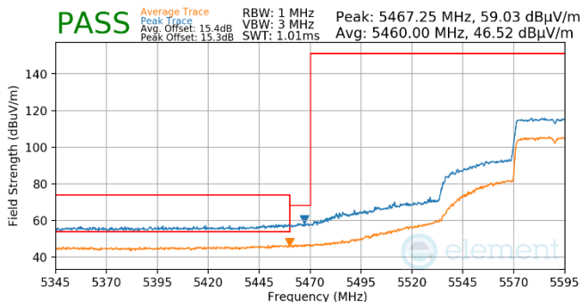
Plot 7-802. (FCC Only) Antenna WF5t (Pk & Avg, Ch.118, 80.11ax(SU),MCS2)
