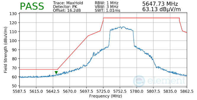
Plot 7-812. Antenna WF5t (Pk, Ch.151, 80.11ax(SU), MCS4)
