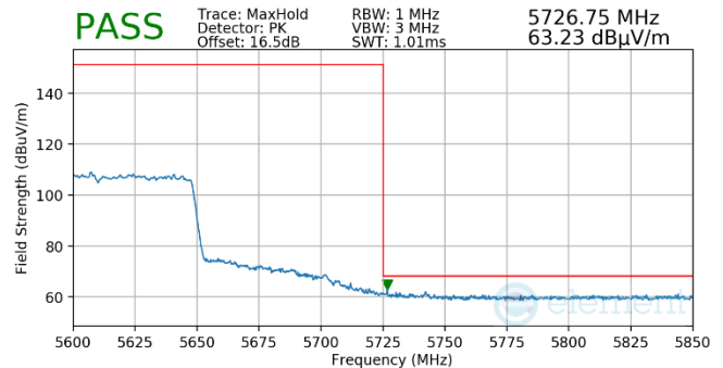
Plot 7-831. (FCC Only) Antenna WF5t (Pk, Ch.122, 802.11ac, MCS9)
