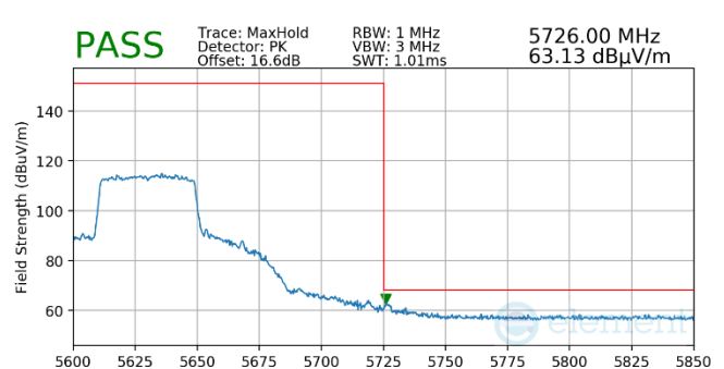
Plot 7-807. (FCC Only) Antenna WF5t (Pk, Ch.126, 80.11ax(SU), MCS11)
