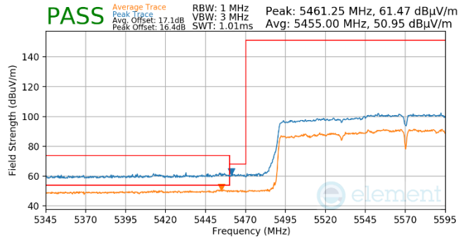
Plot 7-874. (FCC Only) Antenna WF5t (Pk & Avg, Ch.114, 802.11ax(SU), MCS2)
