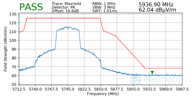
Plot 7-814. Antenna WF5t (Pk, Ch.159, 80.11ax(SU), MCS2)
