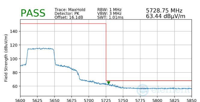
Plot 7-805. (FCC Only) Antenna WF5t (Pk, Ch.126, 80.11ax(SU), MCS2)
