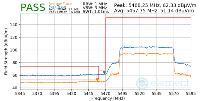
Plot 7-845. Antenna WF5t (Pk & Avg, Ch.106, 802.11ax(SU), MCS4)
