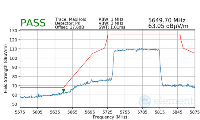
Plot 7-854. Antenna WF5t (Pk, Ch.155, 802.11ax(SU), MCS4)
