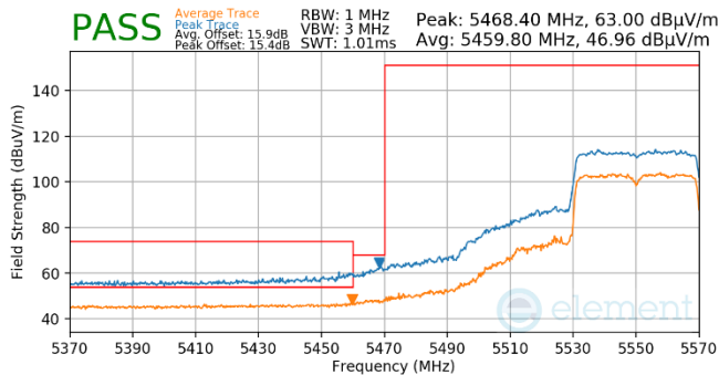
Plot 7-801. Antenna WF5t (Pk & Avg, Ch.110, 80.11ax(SU), MCS11)
