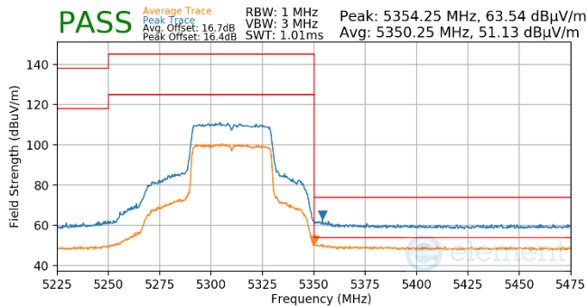
Plot 7-793. Antenna WF5t (Pk & Avg, Ch.62, 80.11ax(SU), MCS2)
