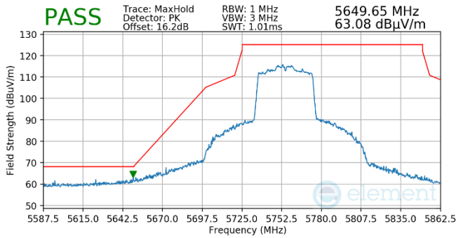
Plot 7-811. Antenna WF5t (Pk, Ch.151, 80.11ax(SU), MCS2)
