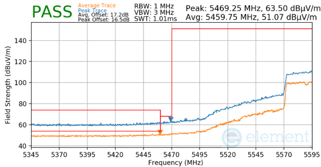
Plot 7-827. (FCC Only) Antenna WF5t (Pk & Avg, Ch.122, 802.11ac, MCS4)
