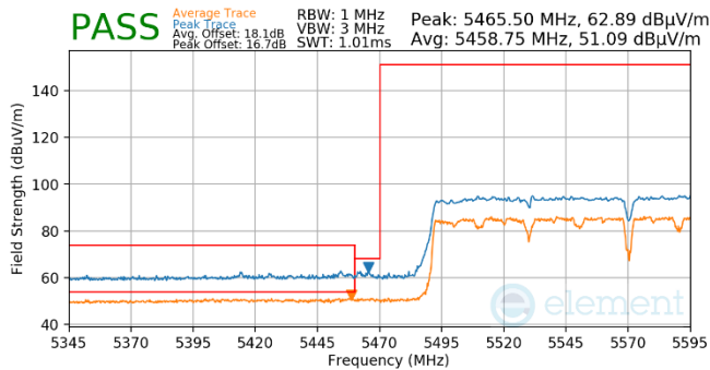
Plot 7-867. (FCC Only) Antenna WF5t (Pk & Avg, Ch.114, 802.11n, MCS11)
