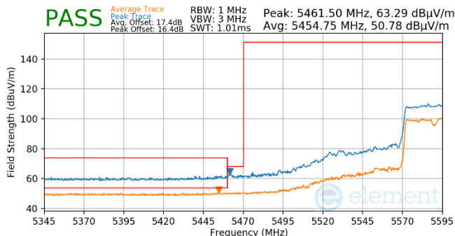
Plot 7-828. (FCC Only) Antenna WF5t (Pk & Avg, Ch.122, 802.11ac, MCS9)
