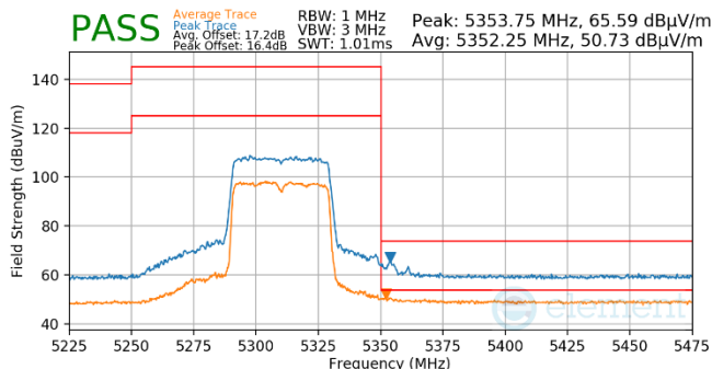
Plot 7-795. Antenna WF5t (Pk & Avg, Ch.62, 80.11ax(SU), MCS11)
