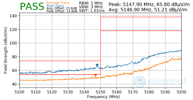
Plot 7-789. Antenna WF5t (Pk & Avg, Ch.46, 80.11ax(SU), MCS11)
