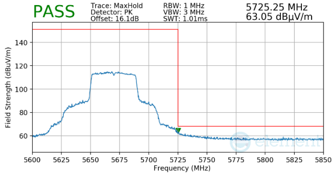
Plot 7-808. Antenna WF5t (Pk, Ch.134, 80.11ax(SU), MCS2)
