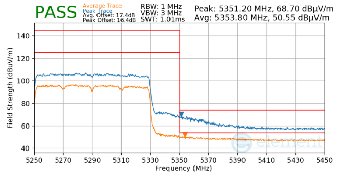
Plot 7-843. Antenna WF5t (Pk & Avg, Ch.58, 802.11ax(SU), MCS11)
