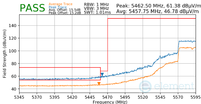
Plot 7-803. (FCC Only) Antenna WF5t (Pk & Avg, Ch.118, 80.11ax(SU),MCS4)
