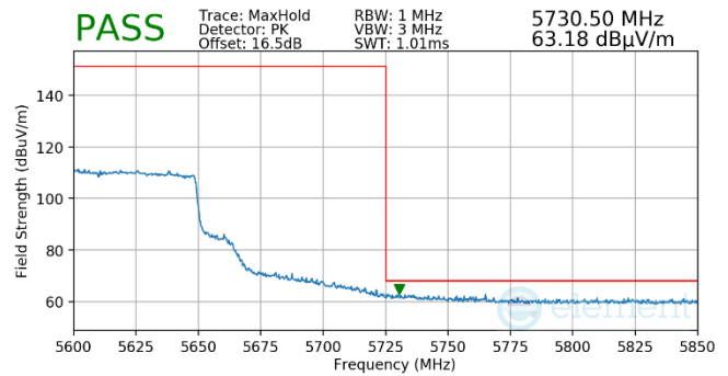
Plot 7-850. (FCC Only) Antenna WF5t (Pk, Ch.122, 802.11ax(SU), MCS2)
