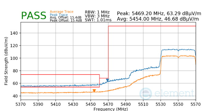
Plot 7-799. Antenna WF5t (Pk & Avg, Ch.110, 80.11ax(SU), MCS2)
