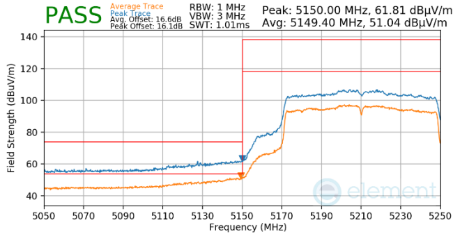
Plot 7-817. Antenna WF5t (Pk & Avg, Ch.42, 802.11ac, MCS2)
