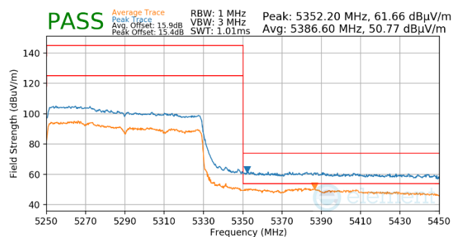
Plot 7-871. Antenna WF5t (Pk & Avg, Ch.50, 802.11ax(SU), MCS2)
