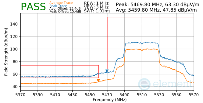
Plot 7-796. Antenna WF5t (Pk & Avg, Ch.102, 80.11ax(SU), MCS2)
