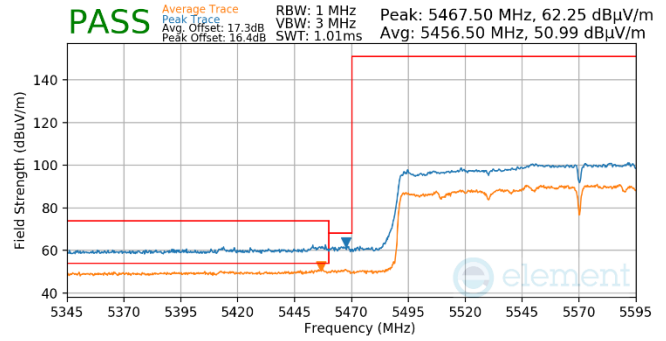
Plot 7-875. Antenna WF5t (FCC Only) (Pk & Avg. CH. 114, 802.11ax(SU), MCS4)
