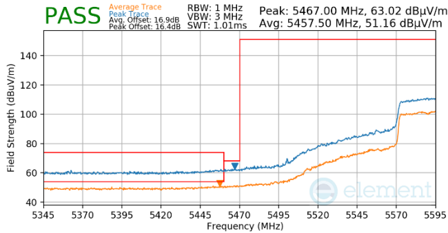
Plot 7-826. (FCC Only) Antenna WF5t (Pk & Avg, Ch.122, 802.11ac, MCS2)
