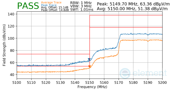
Plot 7-784. Antenna WF5t (Pk & Avg, Ch.38, 80.11ax(SU), MCS2)
