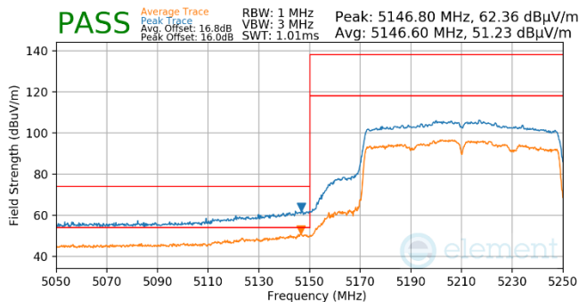
Plot 7-818. Antenna WF5t (Pk & Avg, Ch.42, 802.11ac, MCS4)
