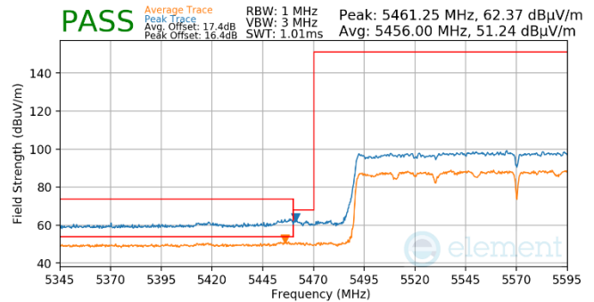
Plot 7-876. Antenna WF5t (FCC Only) (Pk & Avg. CH. 114, 802.11ax(SU), MCS11)
