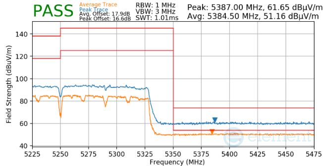
Plot 7-861. Antenna WF5t (Pk & Avg, Ch.50, 802.11ac, MCS9)
