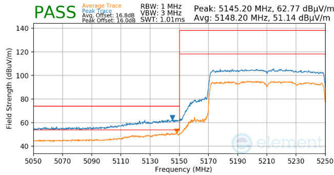
Plot 7-839. Antenna WF5t (Pk & Avg, Ch.42, 802.11ax(SU), MCS4)
