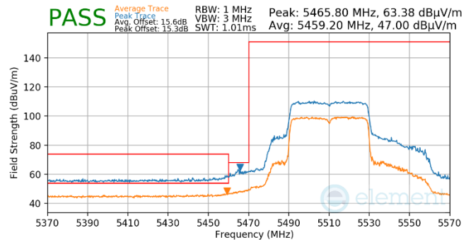
Plot 7-797. Antenna WF5t (Pk & Avg, Ch.102, 80.11ax(SU), MCS4)
