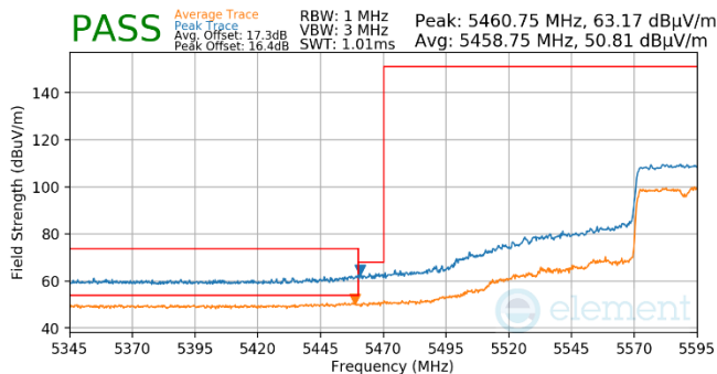
Plot 7-849. (FCC Only) Antenna WF5t (Pk & Avg, Ch.122, 802.11ax(SU), MCS11)
