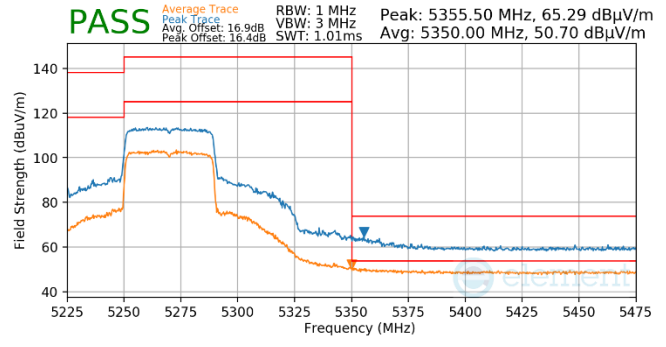
Plot 7-791. Antenna WF5t (Pk & Avg, Ch.54, 80.11ax(SU), MCS4)
