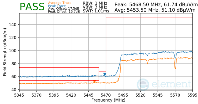
Plot 7-865. (FCC Only) Antenna WF5t (Pk & Avg, Ch.114, 802.11n, MCS2)
