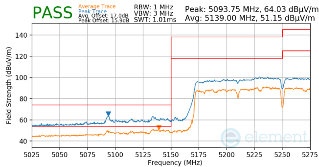
Plot 7-860. Antenna WF5t (Pk & Avg, Ch.50, 802.11ac, MCS4)
