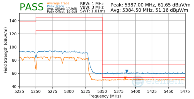
Plot 7-864. Antenna WF5t (Pk & Avg, Ch.50, 802.11ac, MCS9)
