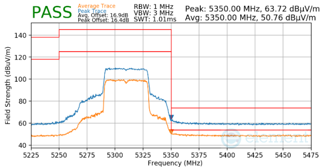
Plot 7-794. Antenna WF5t (Pk & Avg, Ch.62, 80.11ax(SU), MCS4)
