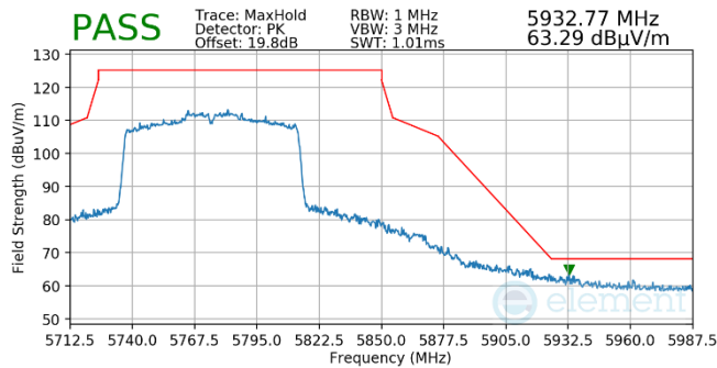
Plot 7-836. Antenna WF5t (Pk, Ch.155, 802.11ac, MCS4)
