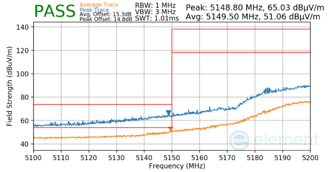
Plot 7-788. Antenna WF5t (Pk & Avg, Ch.46, 80.11ax(SU), MCS4)
