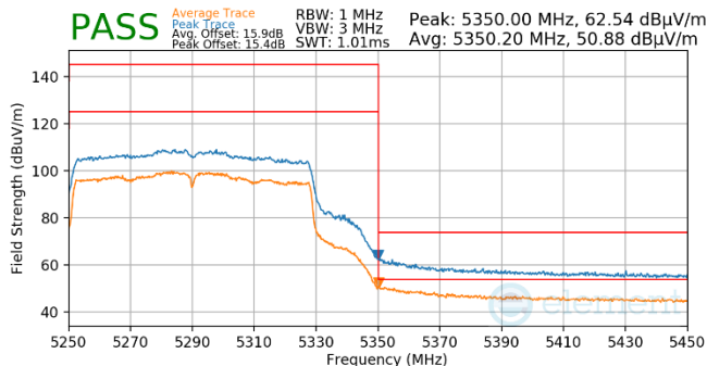
Plot 7-820. Antenna WF5t (Pk & Avg, Ch.58, 802.11ac, MCS2)
