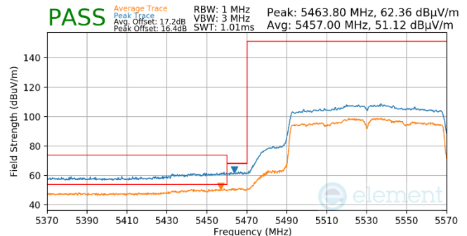
Plot 7-824. Antenna WF5t (Pk & Avg, Ch.106, 802.11ac, MCS4)
