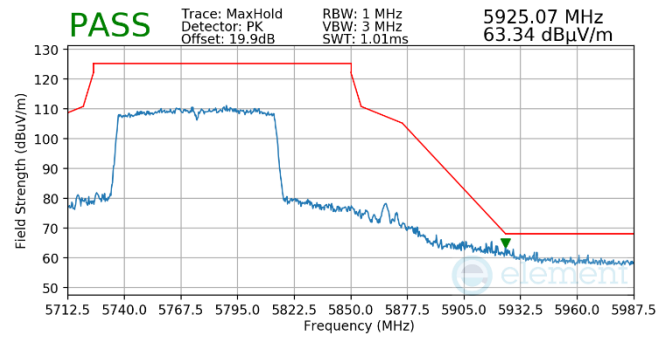
Plot 7-837. Antenna WF5t (Pk, Ch.155, 802.11ac, MCS9)
