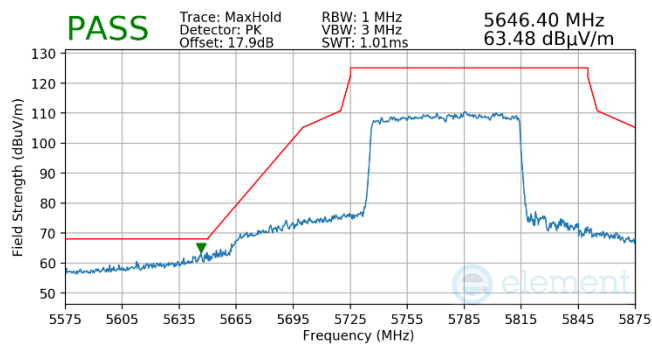
Plot 7-855. Antenna WF5t (Pk, Ch.155, 802.11ax(SU), MCS11)
