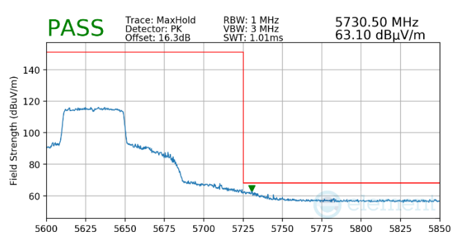
Plot 7-806. (FCC Only) Antenna WF5t (Pk, Ch.126, 80.11ax(SU), MCS4)
