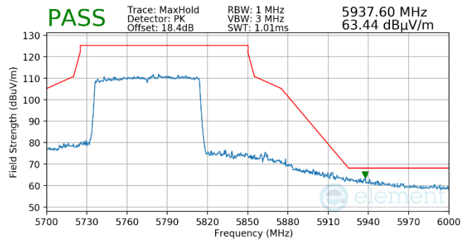
Plot 7-857. Antenna WF5t (Pk, Ch.155, 802.11ax(SU), MCS4)
