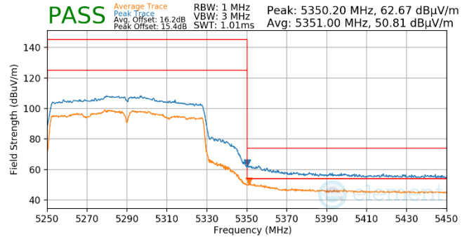
Plot 7-821. Antenna WF5t (Pk & Avg, Ch.58, 802.11ac, MCS4)
