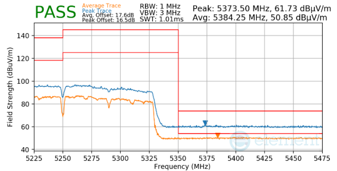
Plot 7-863. Antenna WF5t (Pk & Avg, Ch.50, 802.11ac, MCS4)
