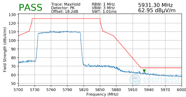
Plot 7-856. Antenna WF5t (Pk, Ch.155, 802.11ax(SU), MCS2)
