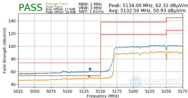
Plot 7-868. Antenna WF5t (Pk & Avg, Ch.50, 802.11ax(SU), MCS2)
