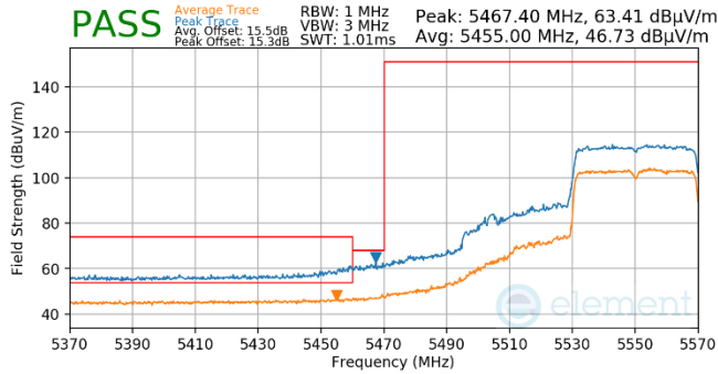
Plot 7-800. Antenna WF5t (Pk & Avg, Ch.110, 80.11ax(SU), MCS4)
