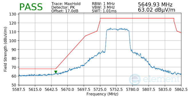
Plot 7-813. Antenna WF5t (Pk, Ch.151, 80.11ax(SU), MCS11)
