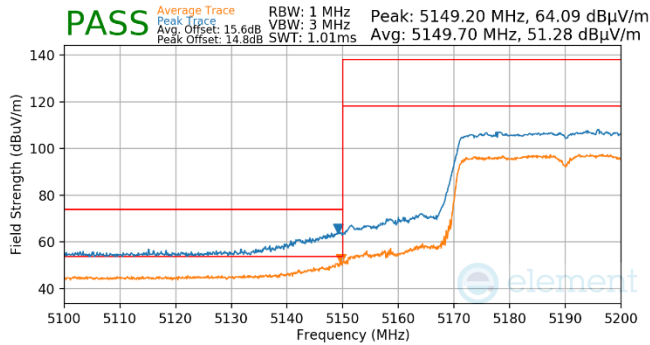
Plot 7-786. Antenna WF5t (Pk & Avg, Ch.38, 80.11ax(SU), MCS11)
