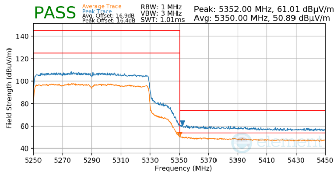
Plot 7-841. Antenna WF5t (Pk & Avg, Ch.58, 802.11ax(SU), MCS2)
