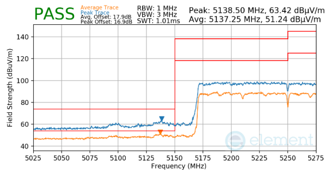
Plot 7-870. Antenna WF5t (Pk & Avg, Ch.50, 802.11ax(SU), MCS11)
