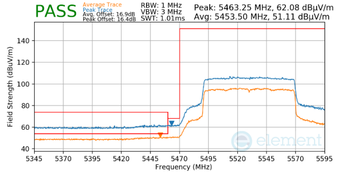
Plot 7-844. Antenna WF5t (Pk & Avg, Ch.106, 802.11ax(SU), MCS2)
