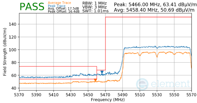
Plot 7-825. Antenna WF5t (Pk & Avg, Ch.106, 802.11ac, MCS9)
