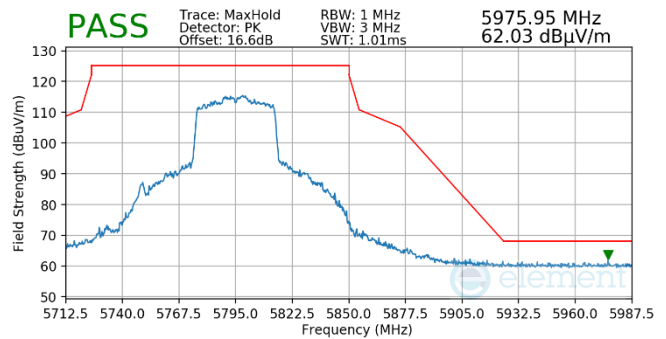
Plot 7-815. Antenna WF5t (Pk, Ch.159, 80.11ax(SU), MCS4)
