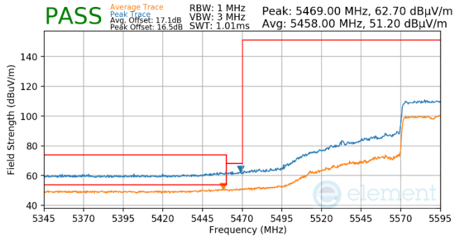
Plot 7-848. (FCC Only) Antenna WF5t (Pk & Avg, Ch.122, 802.11ax(SU), MCS4)
