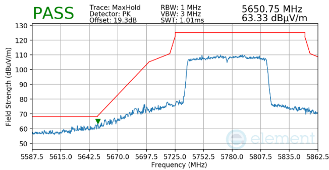
Plot 7-834. Antenna WF5t (Pk, Ch.155, 802.11ac, MCS9)
