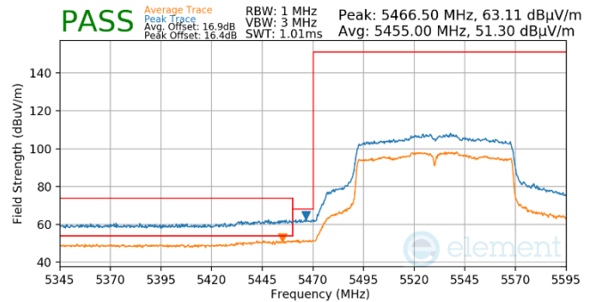
Plot 7-823. Antenna WF5t (Pk & Avg, Ch.106, 802.11ac, MCS2)
