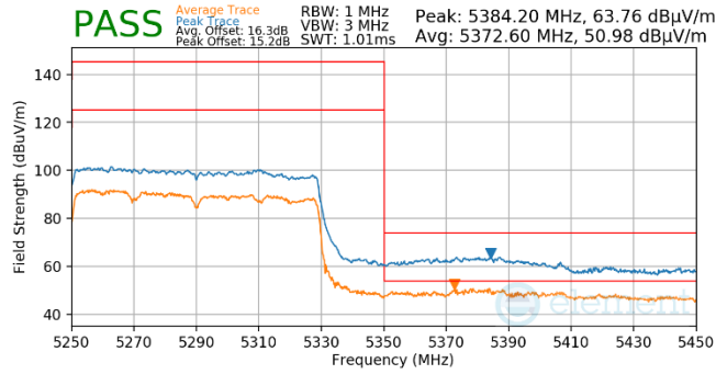
Plot 7-873. Antenna WF5t (Pk & Avg, Ch.50, 802.11ax(SU), MCS11)
