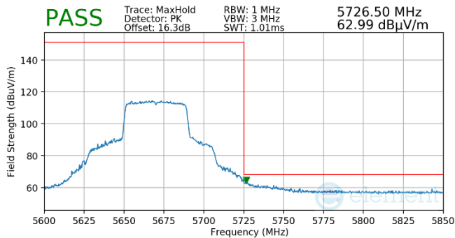
Plot 7-809. Antenna WF5t (Pk, Ch.134, 80.11ax(SU), MCS4)
