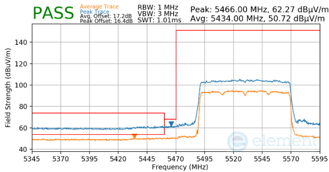
Plot 7-846. Antenna WF5t (Pk & Avg, Ch.106, 802.11ax(SU), MCS11)
