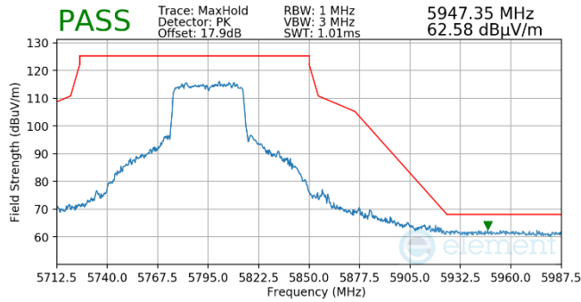
Plot 7-816. Antenna WF5t (Pk, Ch.159, 80.11ax(SU), MCS11)
