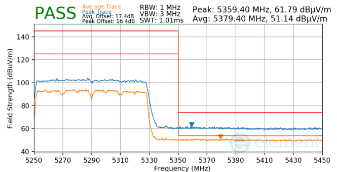
Plot 7-822. Antenna WF5t (Pk & Avg, Ch.58, 802.11ac, MCS9)
