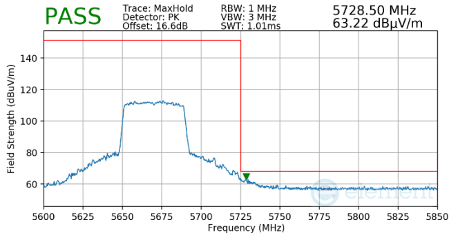
Plot 7-810. Antenna WF5t (Pk, Ch.134, 80.11ax(SU), MCS11)
