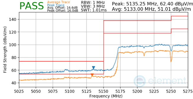
Plot 7-859. Antenna WF5t (Pk & Avg, Ch.50, 802.11ac, MCS2)
