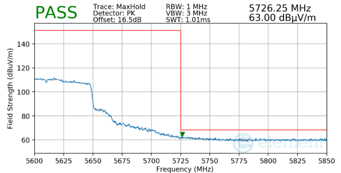
Plot 7-830. (FCC Only) Antenna WF5t (Pk, Ch.122, 802.11ac, MCS4)
