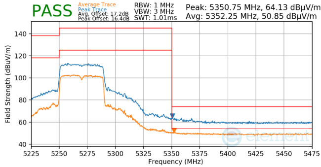
Plot 7-792. Antenna WF5t (Pk & Avg, Ch.54, 80.11ax(SU), MCS11)
