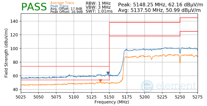
Plot 7-869. Antenna WF5t (Pk & Avg, Ch.50, 802.11ax(SU), MCS4)
