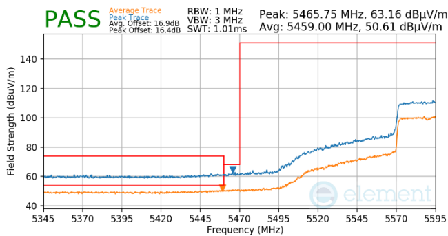
Plot 7-847. (FCC Only) Antenna WF5t (Pk & Avg, Ch.122, 802.11ax(SU), MCS2)
