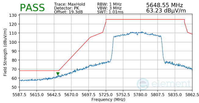
Plot 7-833. Antenna WF5t (Pk, Ch.155, 802.11ac, MCS4)
