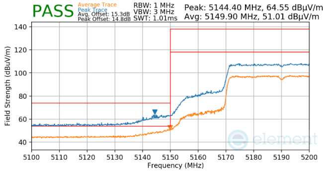
Plot 7-785. Antenna WF5t (Pk & Avg, Ch.38, 80.11ax(SU), MCS4)
