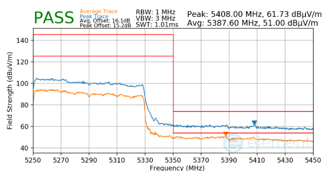
Plot 7-872. Antenna WF5t (Pk & Avg, Ch.50, 802.11ax(SU), MCS4)
