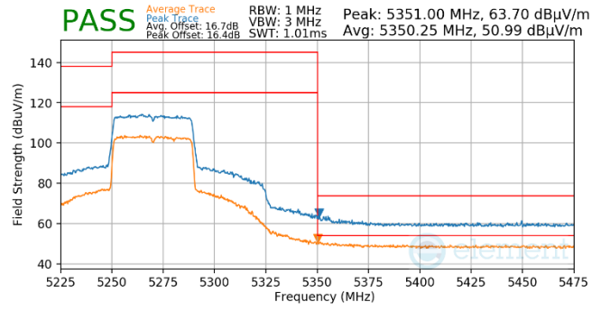
Plot 7-790. Antenna WF5t (Pk & Avg, Ch.54, 80.11ax(SU), MCS2)
