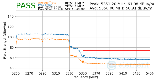
Plot 7-842. Antenna WF5t (Pk & Avg, Ch.58, 802.11ax(SU), MCS4)
