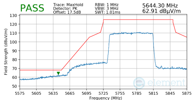
Plot 7-853. Antenna WF5t (Pk, Ch.155, 802.11ax(SU), MCS2)
