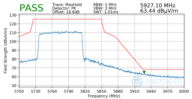
Plot 7-858. Antenna WF5t (Pk, Ch.155, 802.11ax(SU), MCS11)
