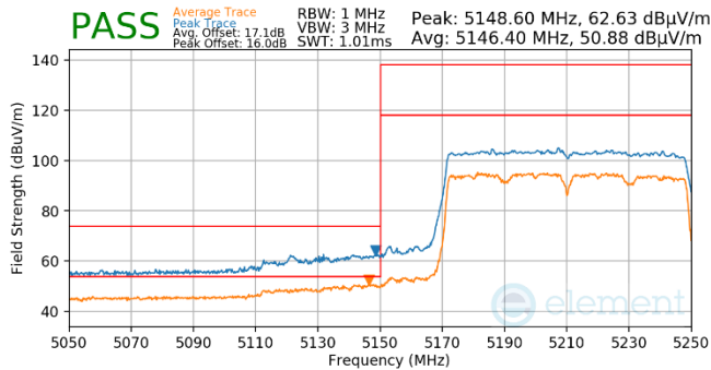
Plot 7-819. Antenna WF5t (Pk & Avg, Ch.42, 802.11ac, MCS9)
