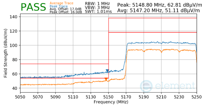
Plot 7-840. Antenna WF5t (Pk & Avg, Ch.42, 802.11ax(SU), MCS11)
