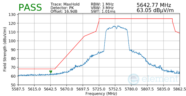
Plot 7-778. Antenna WF5t (Pk, Ch.151, 802.11n, MCS2)
