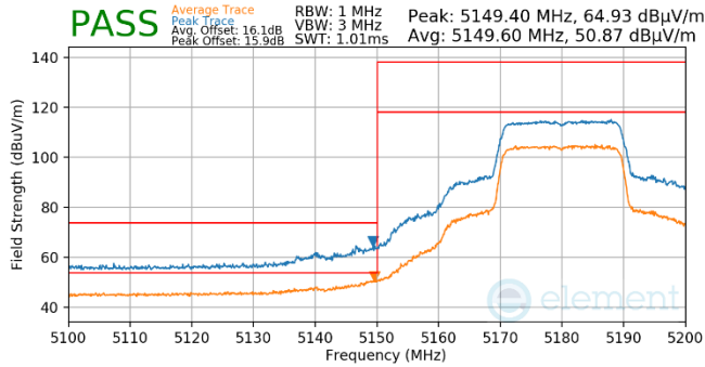
Plot 7-719. Antenna WF5t (Pk & Avg, Ch.36, 802.11ax(SU), MCS2)
