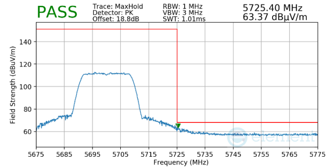
Plot 7-712. Antenna WF5t (Pk, Ch.140, 802.11n, MCS7)
