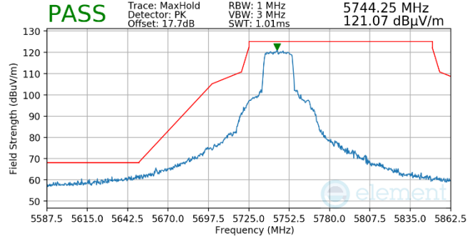
Plot 7-748. Antenna WF5t (Pk, Ch.149, 802.11ax(SU), MCS11)
