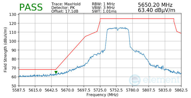
Plot 7-780. Antenna WF5t (Pk, Ch.151, 802.11n, MCS7)
