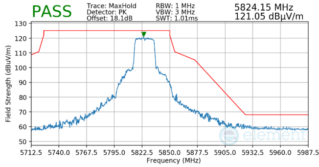
Plot 7-751. Antenna WF5t (Pk, Ch.165, 802.11ax(SU), MCS11)
