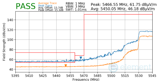
Plot 7-737. Antenna WF5t (Pk & Avg, Ch.108, 802.11ax(SU), MCS11)
