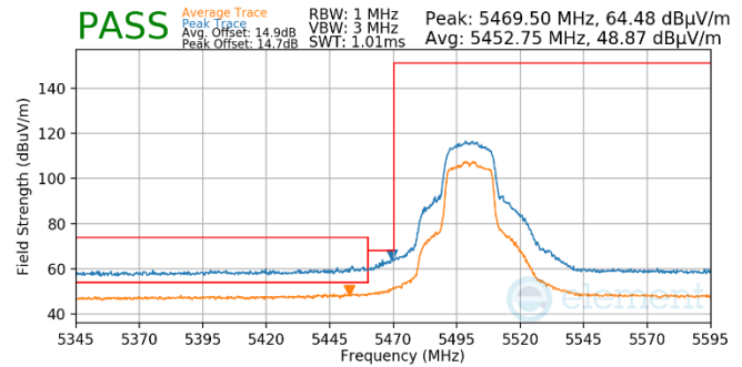
Plot 7-701. Antenna WF5t (Pk & Avg, Ch.100, 802.11n, MCS2)
