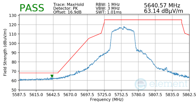
Plot 7-779. Antenna WF5t (Pk, Ch.151, 802.11n, MCS4)
