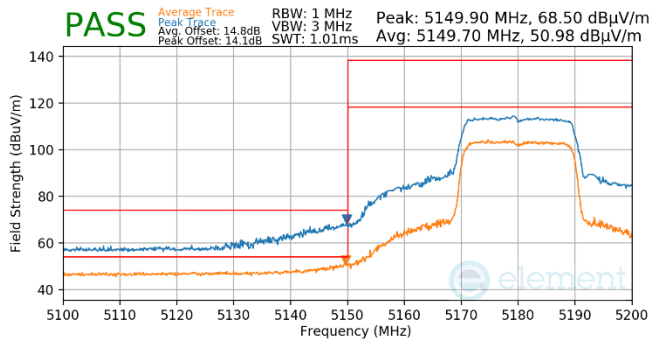
Plot 7-721. Antenna WF5t (Pk & Avg, Ch.36, 802.11ax(SU), MCS11)
