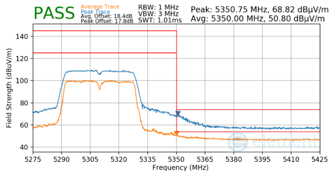
Plot 7-763. Antenna WF5t (Pk & Avg, Ch.62, 802.11n, MCS7)
