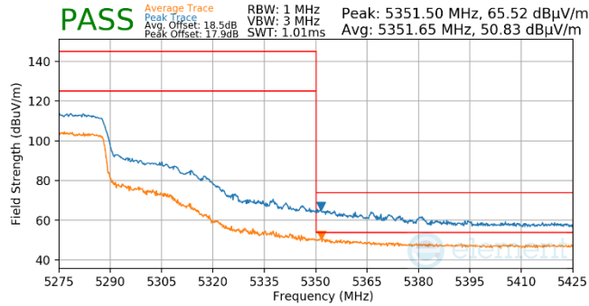
Plot 7-760. Antenna WF5t (Pk & Avg, Ch.54, 802.11n, MCS7)
