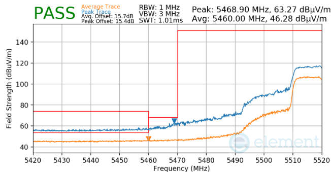
Plot 7-736. Antenna WF5t (Pk & Avg, Ch.104, 802.11ax(SU), MCS11)
