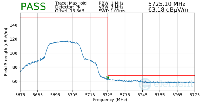
Plot 7-710. Antenna WF5t (Pk, Ch.140, 802.11n, MCS2)
