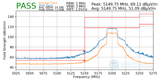
Plot 7-694. Antenna WF5t (Pk & Avg, Ch.40, 802.11n, MCS7)
