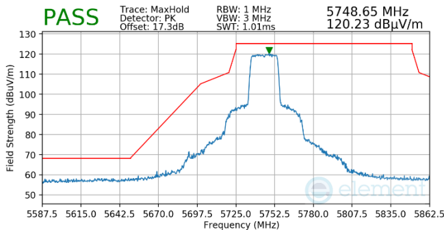
Plot 7-746. Antenna WF5t (Pk, Ch.149, 802.11ax(SU), MCS2)
