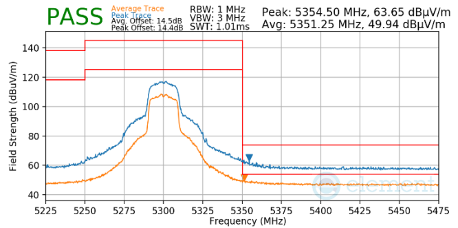
Plot 7-695. Antenna WF5t (Pk & Avg, Ch.60, 802.11n, MCS2)
