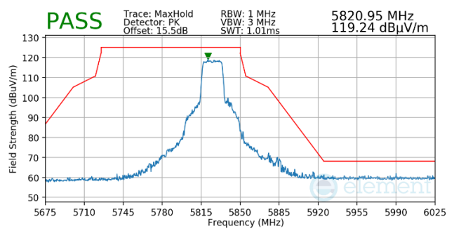
Plot 7-718. Antenna WF5t (Pk, Ch.165, 802.11n, MCS7)
