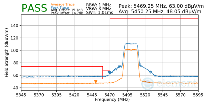
Plot 7-703. Antenna WF5t (Pk & Avg, Ch.100, 802.11n, MCS7)
