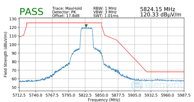
Plot 7-750. Antenna WF5t (Pk, Ch.165, 802.11ax(SU), MCS4)
