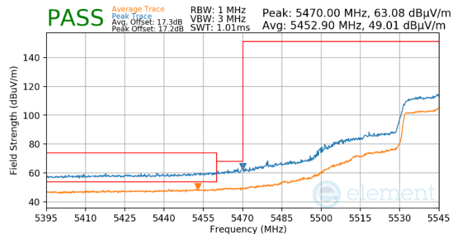
Plot 7-767. Antenna WF5t (Pk & Avg, Ch.110, 802.11n, MCS2)
