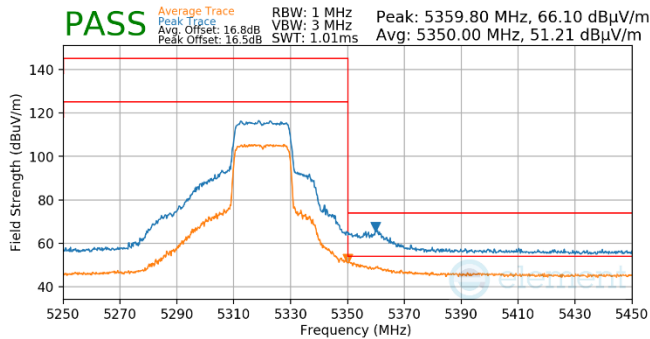
Plot 7-729. Antenna WF5t (Pk & Avg, Ch.64, 802.11ax(SU), MCS4)
