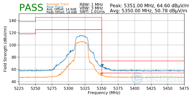
Plot 7-699. Antenna WF5t (Pk & Avg, Ch.64, 802.11n, MCS4)
