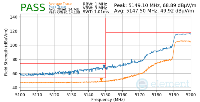
Plot 7-724. Antenna WF5t (Pk & Avg, Ch.40, 802.11ax(SU), MCS11)
