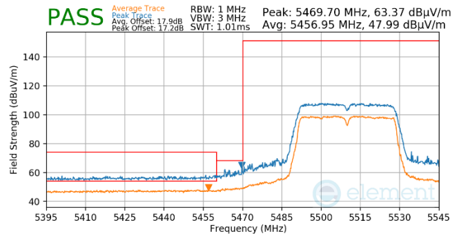
Plot 7-766. Antenna WF5t (Pk & Avg, Ch.102, 802.11n, MCS7)
