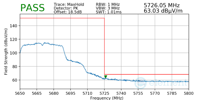
Plot 7-775. Antenna WF5t (Pk, Ch.134, 802.11n, MCS2)
