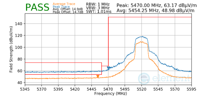
Plot 7-704. Antenna WF5t (Pk & Avg, Ch.104, 802.11n, MCS2)
