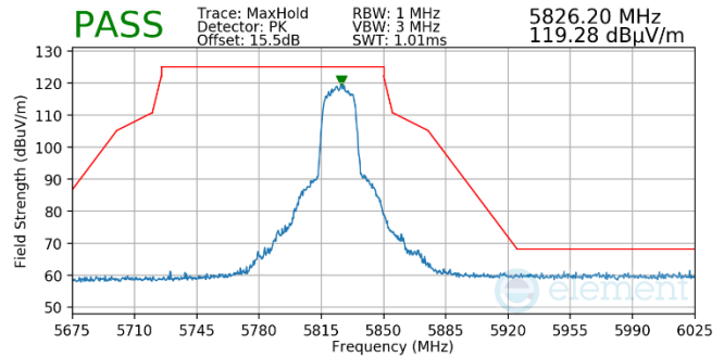
Plot 7-716. Antenna WF5t (Pk, Ch.165, 802.11n, MCS2)
