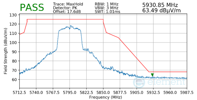
Plot 7-782. Antenna WF5t (Pk, Ch.159, 802.11n, MCS4)
