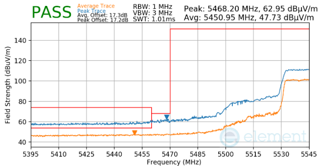
Plot 7-769. Antenna WF5t (Pk & Avg, Ch.110, 802.11n, MCS7)
