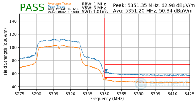
Plot 7-761. Antenna WF5t (Pk & Avg, Ch.62, 802.11n, MCS2)
