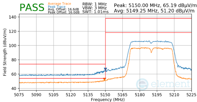
Plot 7-754. Antenna WF5t (Pk & Avg, Ch.38, 802.11n, MCS7)
