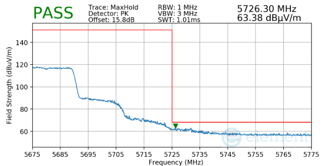
Plot 7-740. Antenna WF5t (Pk, Ch.136, 802.11ax(SU), MCS2)
