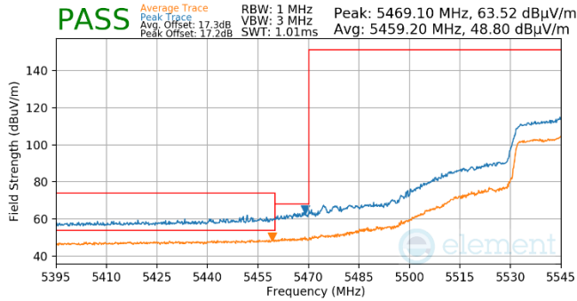
Plot 7-768. Antenna WF5t (Pk & Avg, Ch.110, 802.11n, MCS4)
