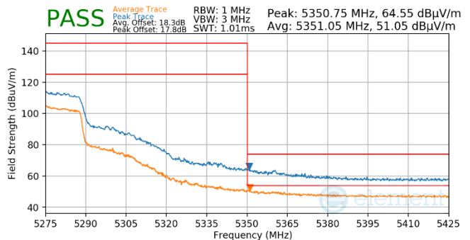
Plot 7-759. Antenna WF5t (Pk & Avg, Ch.54, 802.11n, MCS4)
