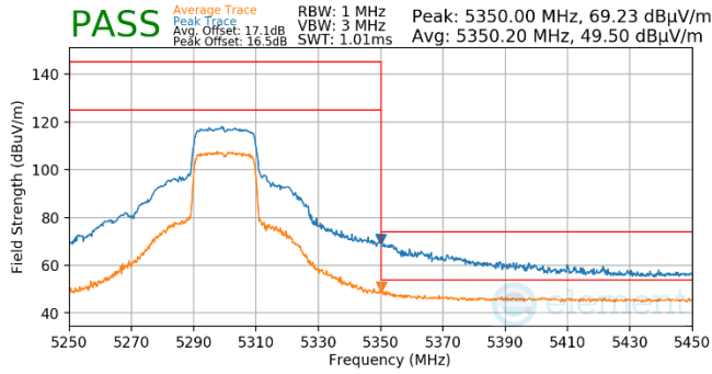
Plot 7-727. Antenna WF5t (Pk & Avg, Ch.60, 802.11ax(SU), MCS11)
