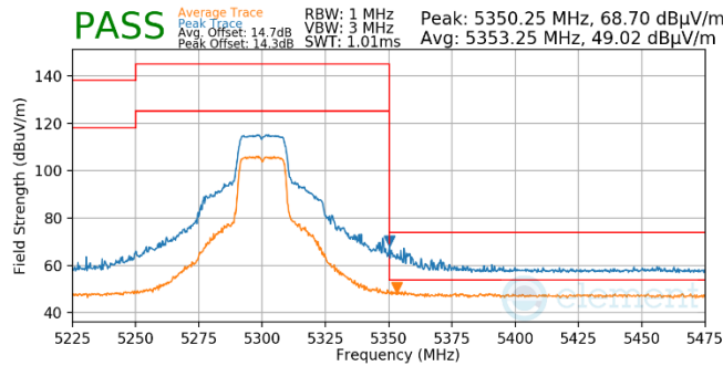
Plot 7-697. Antenna WF5t (Pk & Avg, Ch.60, 802.11n, MCS7)
