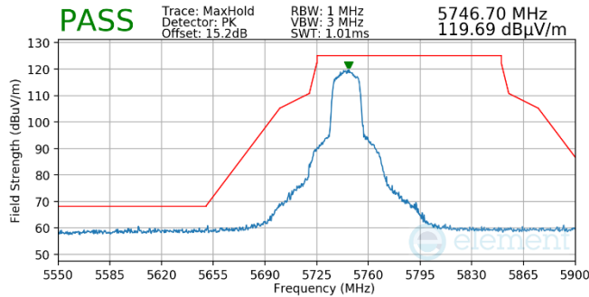
Plot 7-713. Antenna WF5t (Pk, Ch.149, 802.11n, MCS2)
