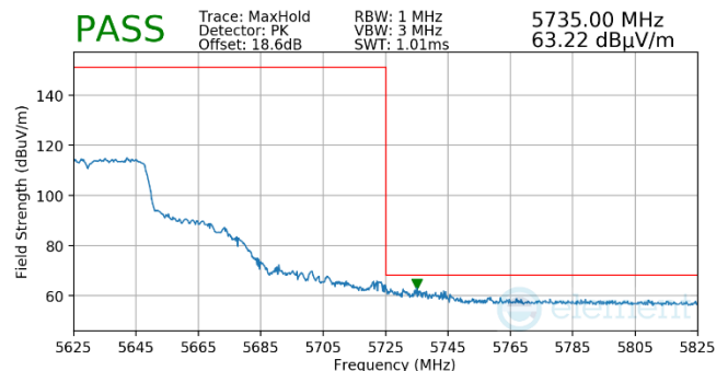
Plot 7-774. (FCC Only) Antenna WF5t (Pk, Ch.126, 802.11n, MCS7)
