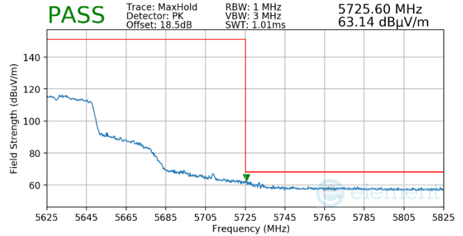
Plot 7-772. (FCC Only) Antenna WF5t (Pk, Ch.126, 802.11n, MCS2)
