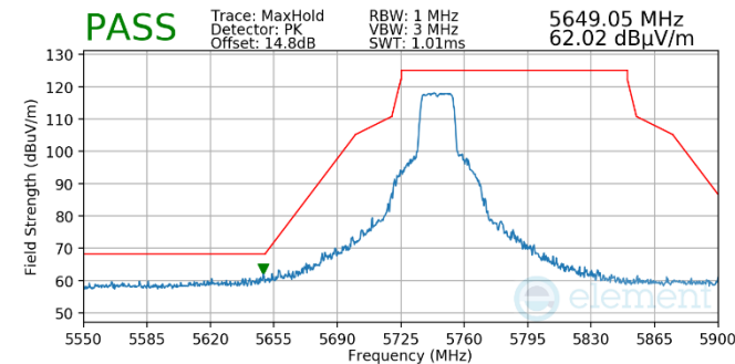
Plot 7-715. Antenna WF5t (Pk, Ch.149, 802.11n, MCS7)
