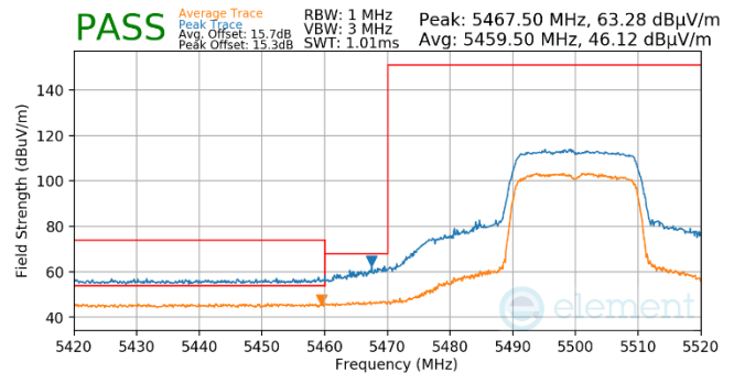
Plot 7-733. Antenna WF5t (Pk & Avg, Ch.100, 802.11ax(SU), MCS11)
