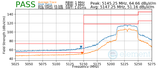
Plot 7-756. Antenna WF5t (Pk & Avg, Ch.46, 802.11n, MCS4)
