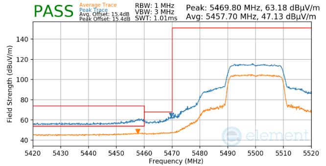
Plot 7-732. Antenna WF5t (Pk & Avg, Ch.100, 802.11ax(SU), MCS4)
