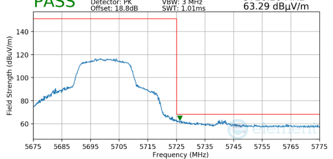
Plot 7-711. Antenna WF5t (Pk, Ch.140, 802.11n, MCS4)
