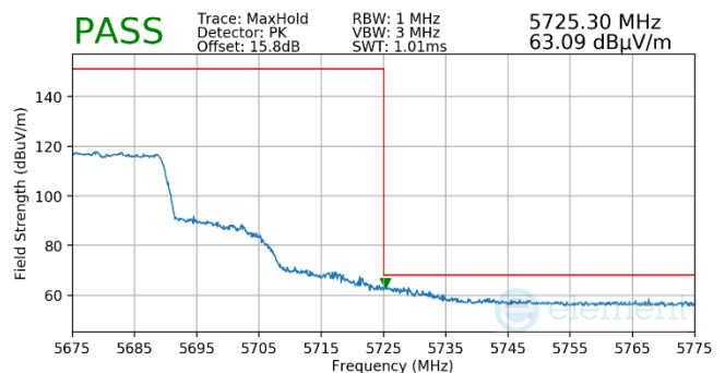
Plot 7-741. Antenna WF5t (Pk, Ch.136, 802.11ax(SU), MCS4)
