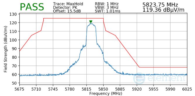
Plot 7-717. Antenna WF5t (Pk, Ch.165, 802.11n, MCS4)
