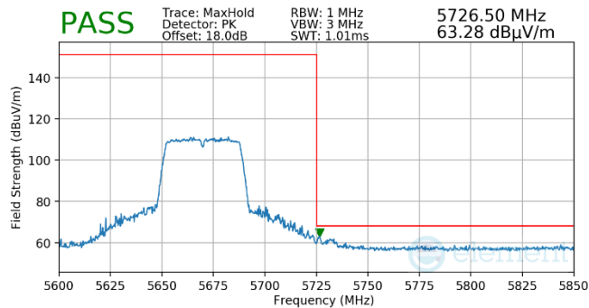
Plot 7-777. Antenna WF5t (Pk, Ch.134, 802.11n, MCS7)
