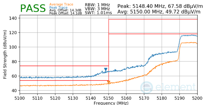
Plot 7-722. Antenna WF5t (Pk & Avg, Ch.40, 802.11ax(SU), MCS2)
