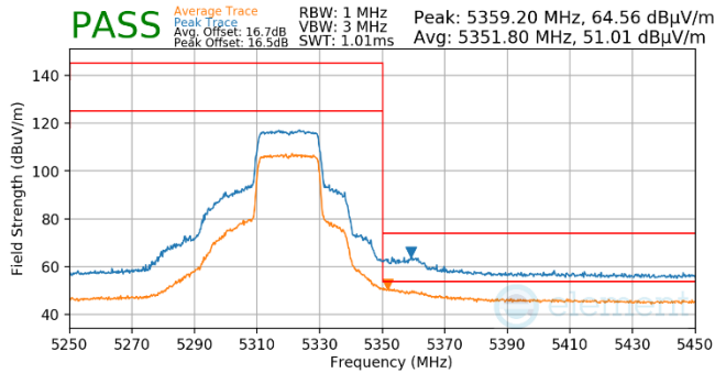
Plot 7-728. Antenna WF5t (Pk & Avg, Ch.64, 802.11ax(SU), MCS2)
