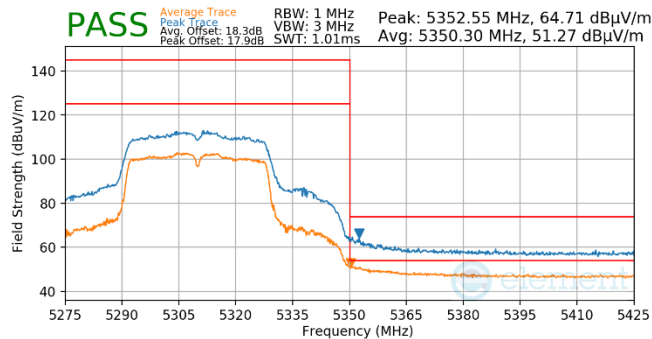
Plot 7-762. Antenna WF5t (Pk & Avg, Ch.62, 802.11n, MCS4)
