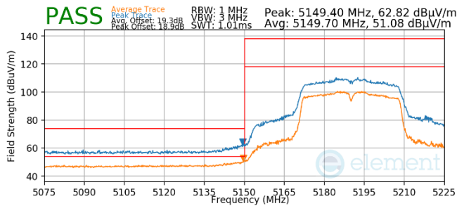
Plot 7-753. Antenna WF5t (Pk & Avg, Ch.38, 802.11n, MCS4)
