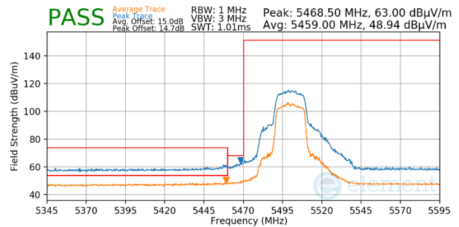
Plot 7-702. Antenna WF5t (Pk & Avg, Ch.100, 802.11n, MCS4)
