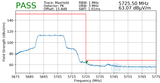
Plot 7-744. Antenna WF5t (Pk, Ch.140, 802.11ax(SU), MCS4)
