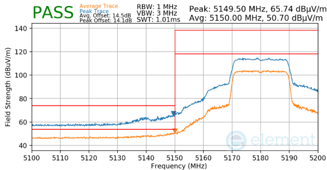
Plot 7-720. Antenna WF5t (Pk & Avg, Ch.36, 802.11ax(SU), MCS4)
