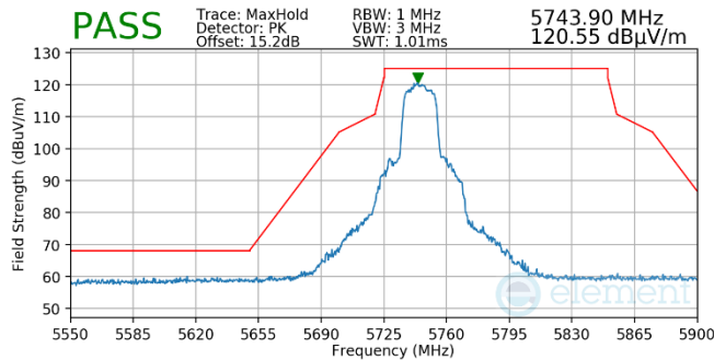
Plot 7-714. Antenna WF5t (Pk, Ch.149, 802.11n, MCS4)
