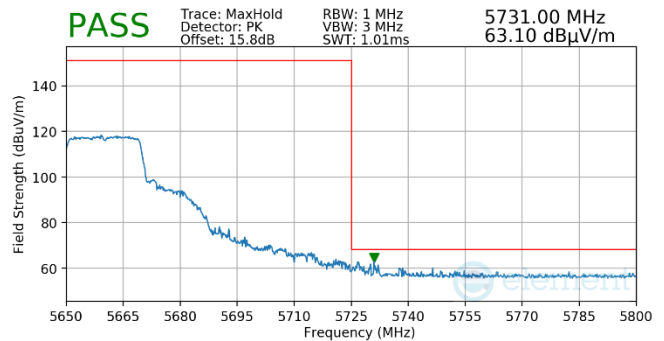
Plot 7-739. Antenna WF5t (Pk, Ch.132, 802.11ax(SU), MCS11)
