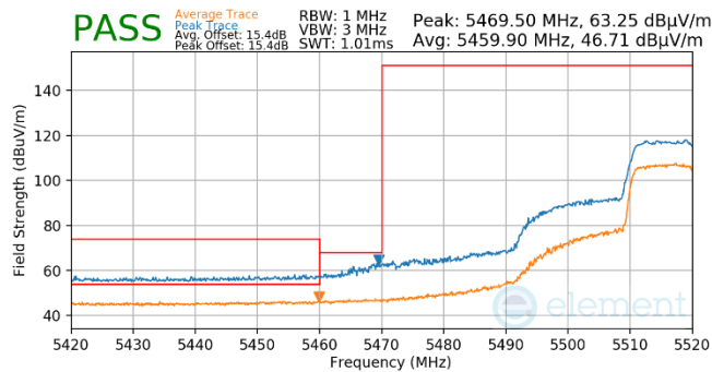
Plot 7-735. Antenna WF5t (Pk & Avg, Ch.104, 802.11ax(SU), MCS4)
