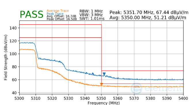
Plot 7-725. Antenna WF5t (Pk & Avg, Ch.60, 802.11ax(SU), MCS2)
