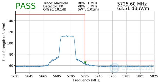
Plot 7-745. Antenna WF5t (Pk, Ch.140, 802.11ax(SU), MCS11)
