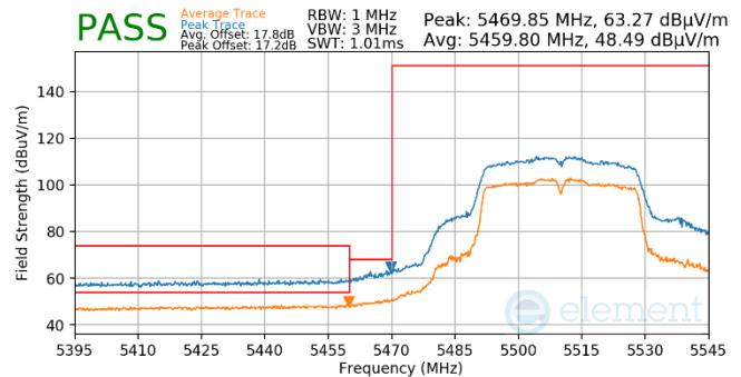
Plot 7-765. Antenna WF5t (Pk & Avg, Ch.102, 802.11n, MCS4)
