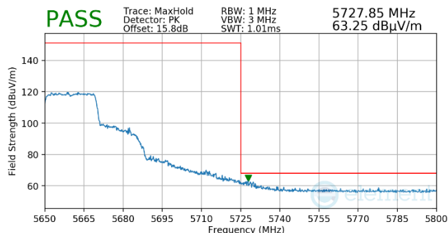
Plot 7-738. Antenna WF5t (Pk, Ch.132, 802.11ax(SU), MCS4)
