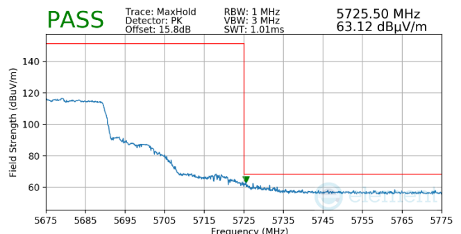
Plot 7-742. Antenna WF5t (Pk, Ch.136, 802.11ax(SU), MCS11)
