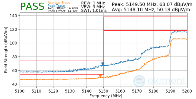
Plot 7-723. Antenna WF5t (Pk & Avg, Ch.40, 802.11ax(SU), MCS4)
