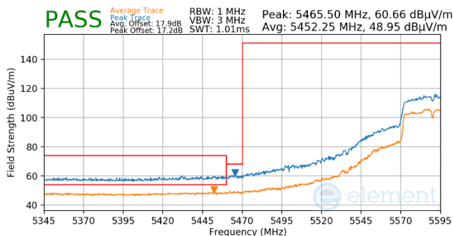
Plot 7-771. (FCC Only) Antenna WF5t (Pk & Avg, Ch.118, 802.11n, MCS7)
