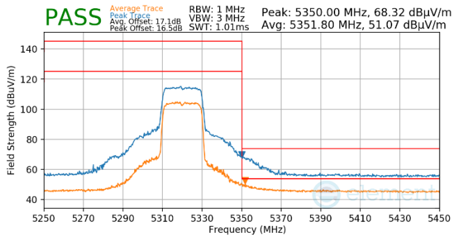
Plot 7-730. Antenna WF5t (Pk & Avg, Ch.64, 802.11ax(SU), MCS11)
