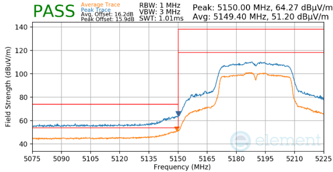
Plot 7-752. Antenna WF5t (Pk & Avg, Ch.38, 802.11n, MCS2)
