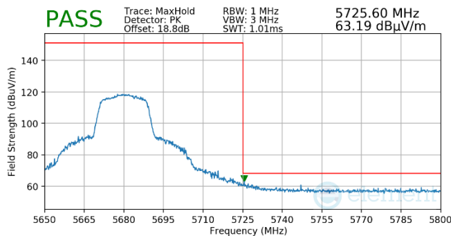
Plot 7-707. Antenna WF5t (Pk, Ch.136, 802.11n, MCS2)
