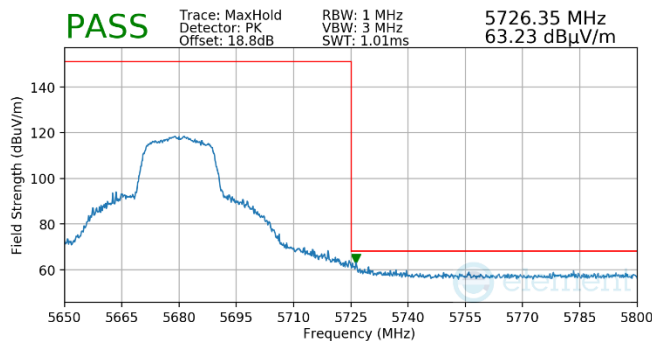
Plot 7-708. Antenna WF5t (Pk, Ch.136, 802.11n, MCS4)
