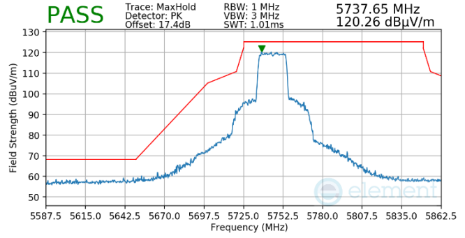
Plot 7-747. Antenna WF5t (Pk, Ch.149, 802.11ax(SU), MCS4)
