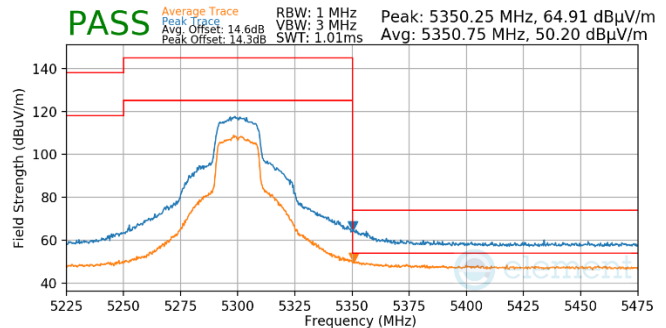
Plot 7-696. Antenna WF5t (Pk & Avg, Ch.60, 802.11n, MCS4)
