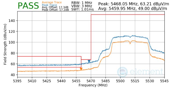
Plot 7-764. Antenna WF5t (Pk & Avg, Ch.102, 802.11n, MCS2)
