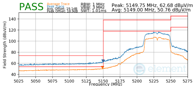
Plot 7-755. Antenna WF5t (Pk & Avg, Ch.46, 802.11n, MCS2)
