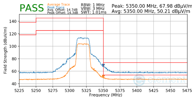
Plot 7-700. Antenna WF5t (Pk & Avg, Ch.64, 802.11n, MCS7)
