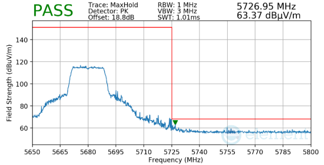
Plot 7-709. Antenna WF5t (Pk, Ch.136, 802.11n, MCS7)
