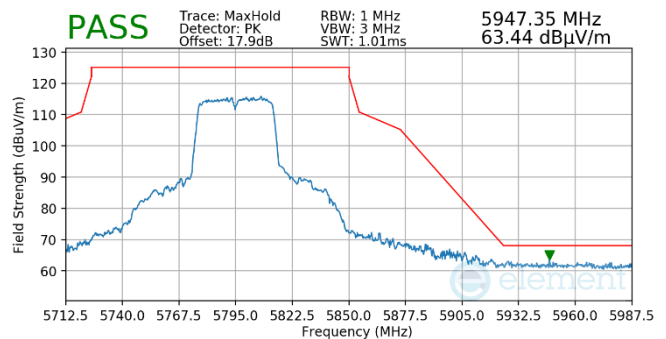
Plot 7-783. Antenna WF5t (Pk, Ch.159, 802.11n, MCS7)
