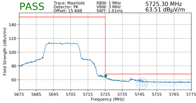
Plot 7-743. Antenna WF5t (Pk, Ch.140, 802.11ax(SU), MCS2)
