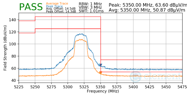
Plot 7-698. Antenna WF5t (Pk & Avg, Ch.64, 802.11n, MCS2)
