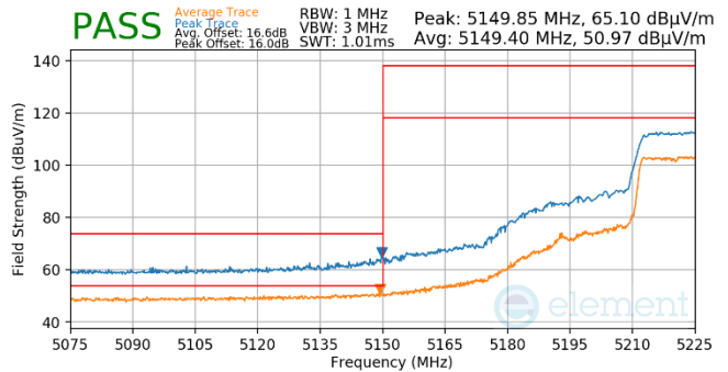
Plot 7-757. Antenna WF5t (Pk & Avg, Ch.46, 802.11n, MCS7)
