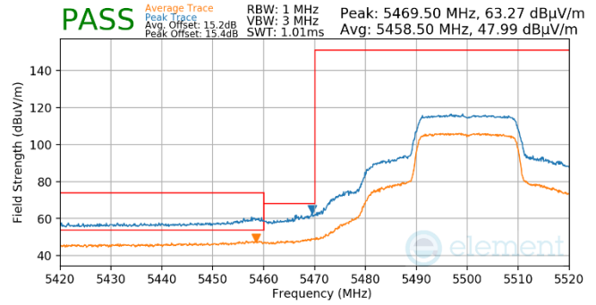
Plot 7-731. Antenna WF5t (Pk & Avg, Ch.100, 802.11ax(SU), MCS2)
