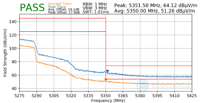
Plot 7-758. Antenna WF5t (Pk & Avg, Ch.54, 802.11n, MCS2)
