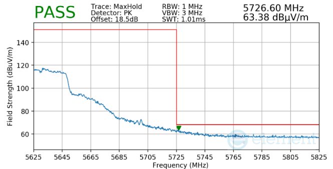
Plot 7-773. (FCC Only) Antenna WF5t (Pk, Ch.126, 802.11n, MCS4)
