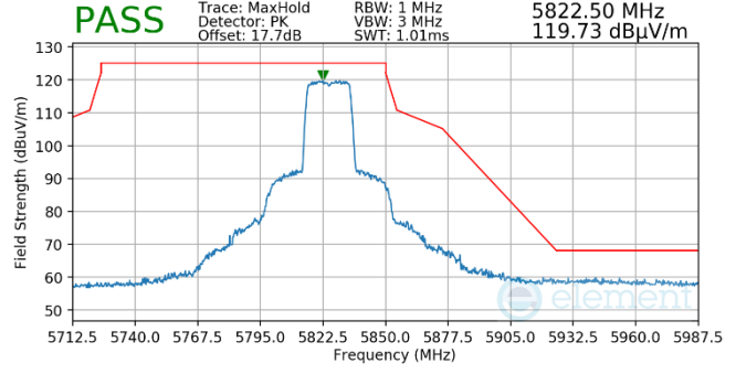
Plot 7-749. Antenna WF5t (Pk, Ch.165, 802.11ax(SU), MCS2)
