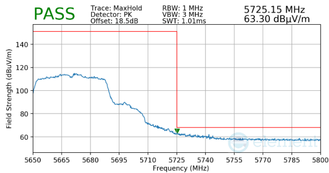
Plot 7-776. Antenna WF5t (Pk, Ch.134, 802.11n, MCS4)
