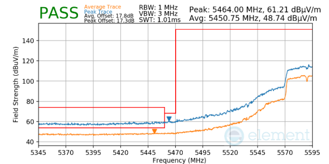
Plot 7-770. (FCC Only) Antenna WF5t (Pk & Avg, Ch.118, 802.11n, MCS4)
