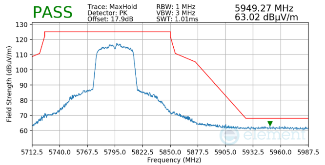
Plot 7-781. Antenna WF5t (Pk, Ch.159, 802.11n, MCS2)
