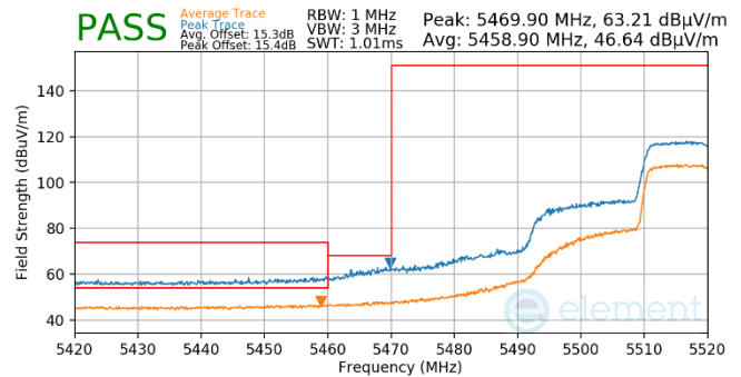
Plot 7-734. Antenna WF5t (Pk & Avg, Ch.104, 802.11ax(SU), MCS2)
