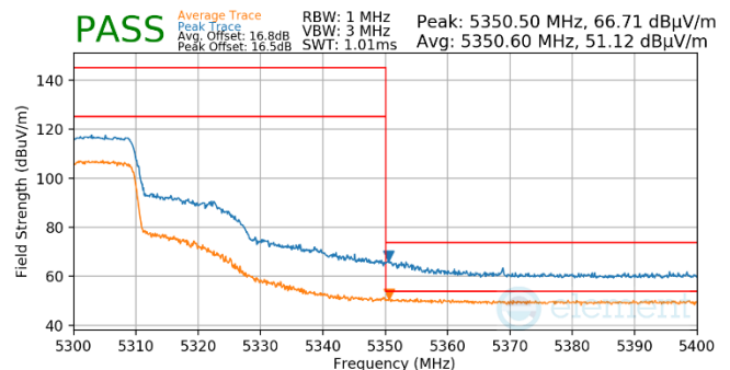
Plot 7-726. Antenna WF5t (Pk & Avg, Ch.60, 802.11ax(SU), MCS4)
