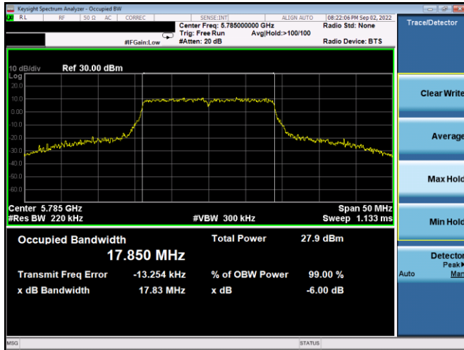
Plot 7-145. 6dB BW & 99% OBW Antenna WF5t (20MHz BW 802.11n – Ch. 157, MCS7)
