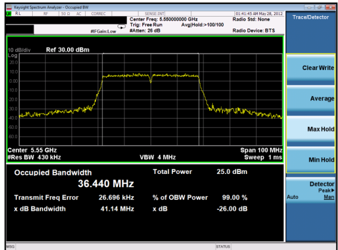
Plot 7-127. 26dB BW & 99% OBW Antenna WF5b (40MHz BW 802.11n – Ch. 110, MCS9)
