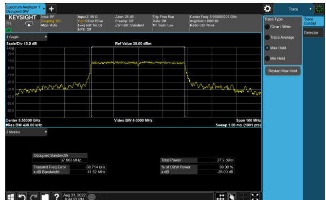
Plot 7-128. 26dB BW & 99% OBW Antenna WF5b (40MHz BW 802.11ax(SU) – Ch. 110, MCS11)
