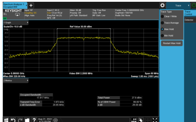
Plot 7-125. 26dB BW & 99% OBW Antenna WF5b (20MHz BW 802.11n – Ch. 116, MCS9)
