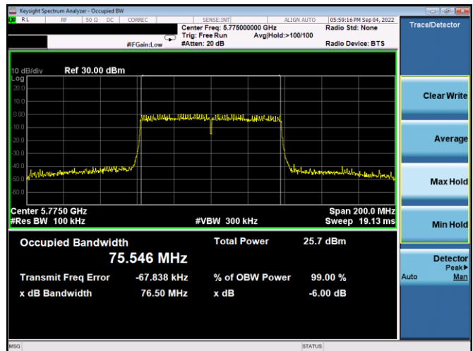
Plot 7-167. 6dB BW & 99% OBW Antenna WF5b (80MHz BW 802.11ac – Ch. 155, MCS9)
