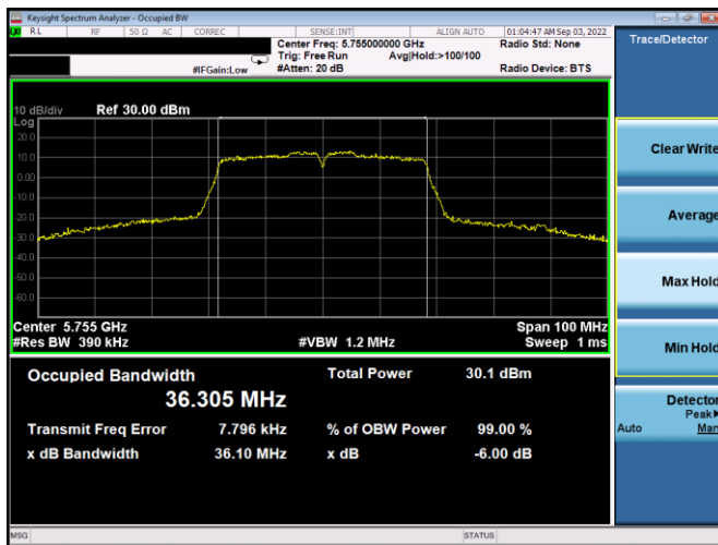
Plot 7-135. 6dB BW & 99% OBW Antenna WF5t (40MHz BW 802.11n – Ch. 151, MCS2)
