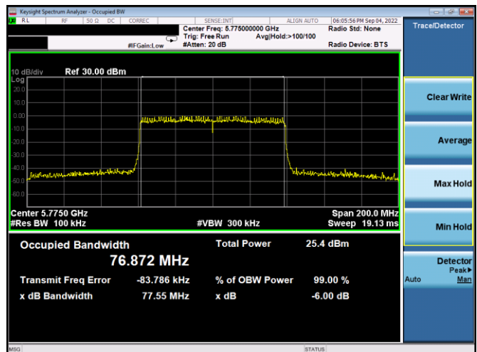
Plot 7-168. 6dB BW & 99% OBW Antenna WF5b (80MHz BW 802.11ax(SU) – Ch. 155, MCS11)
