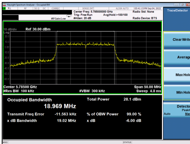
Plot 7-164. 6dB BW & 99% OBW Antenna WF5b (20MHz BW 802.11ax(SU) – Ch. 157, MCS11)
