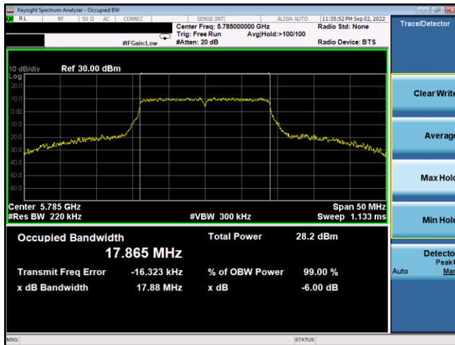
Plot 7-163. 6dB BW & 99% OBW Antenna WF5b (20MHz BW 802.11n – Ch. 157, MCS7)
