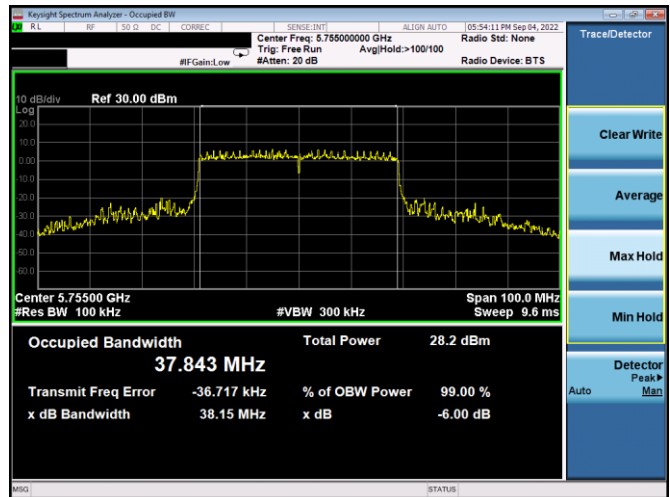
Plot 7-166. 6dB BW & 99% OBW Antenna WF5b (40MHz BW 802.11ax(SU) – Ch. 151, MCS11)
