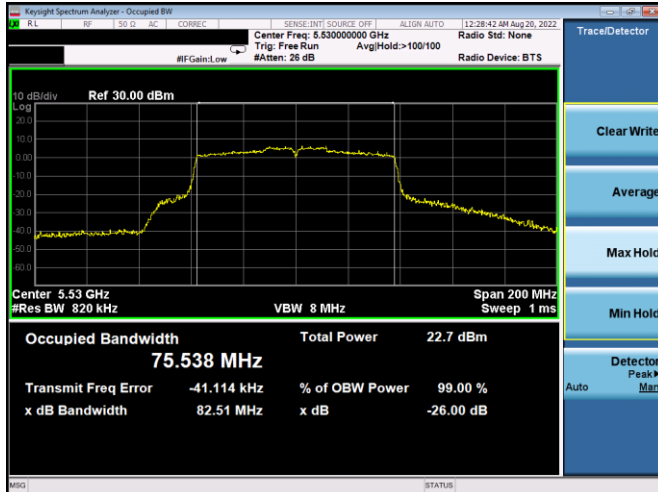
Plot 7-19. 26dB BW & 99% OBW Antenna WF5t (80MHz BW 802.11ac – Ch. 106, MCS2)
