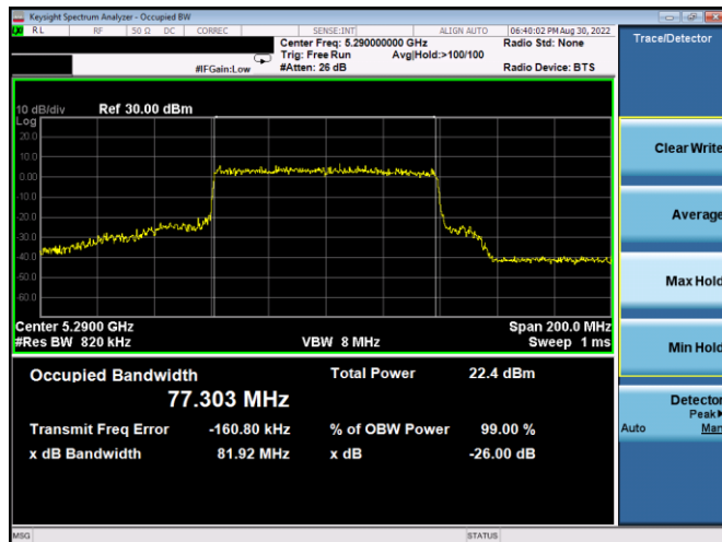
Plot 7-36. 26dB BW & 99% OBW Antenna WF5t (80MHz BW 802.11ax(SU) – Ch. 58, MCS4)
