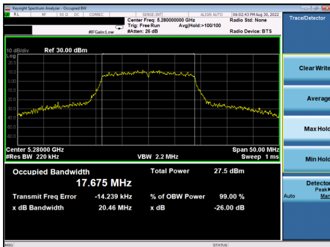
Plot 7-31. 26dB BW & 99% OBW Antenna WF5t (20MHz BW 802.11n – Ch. 56, MCS4)
