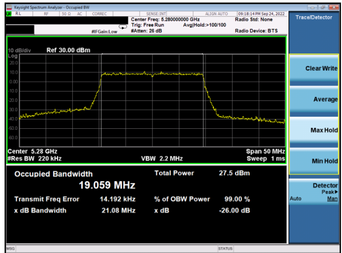
Plot 7-10. 26dB BW & 99% OBW Antenna WF5t (20MHz BW 802.11ax(SU) – Ch. 56, MCS2)
