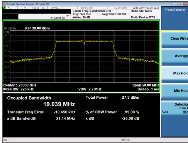
Plot 7-24. 26dB BW & 99% OBW Antenna WF5t (20MHz BW 802.11ax(SU) – Ch. 40, MCS4)
