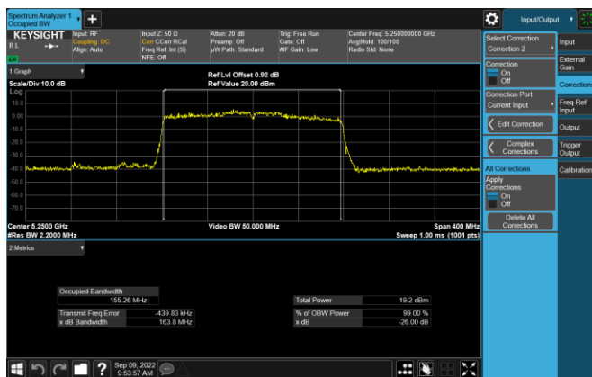
Plot 7-30. 26dB BW & 99% OBW Antenna WF5t (160MHz BW 802.11ax – Ch. 50, MCS4)
