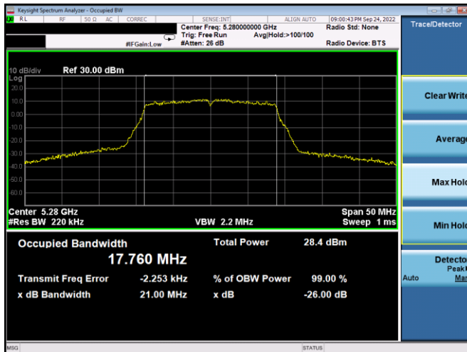
Plot 7-9. 26dB BW & 99% OBW Antenna WF5t (20MHz BW 802.11n – Ch. 56, MCS2)
