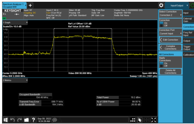
Plot 7-29. 26dB BW & 99% OBW Antenna WF5t (160MHz BW 802.11ac – Ch. 50, MCS4)
