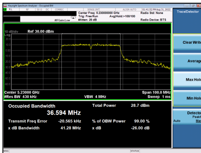
Plot 7-47. 26dB BW & 99% OBW Antenna WF5t (40MHz BW 802.11n – Ch. 46, MCS7)
