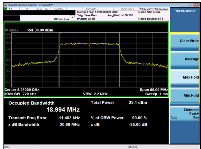
Plot 7-32. 26dB BW & 99% OBW Antenna WF5t (20MHz BW 802.11ax(SU) – Ch. 56, MCS4)
