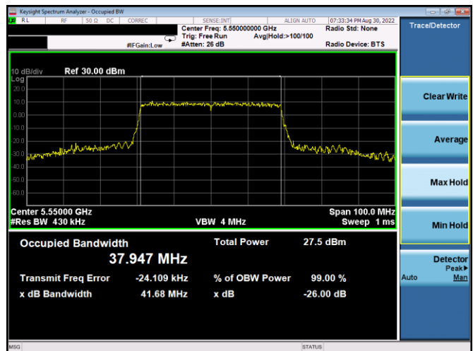
Plot 7-40. 26dB BW & 99% OBW Antenna WF5t (40MHz BW 802.11ax(SU) – Ch. 110, MCS4)
