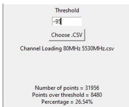
Figure 9-6. 5530MHz - Channel Loading Calculation - Mode 2 (80MHz)
