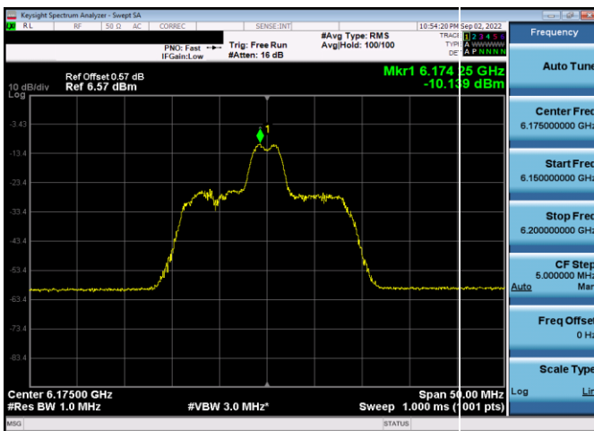
Plot 7-259. Power Spectral Density Plot SDM Antenna 4a (20MHz 802.11ax RU26 (UNII Band 5) – Ch. 45)
