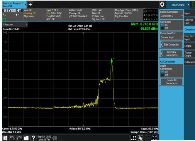
Plot 7-235. Power Spectral Density Plot Antenna 4a (80MHz 802.11ax RU26 (UNII Band 7) – Ch. 151)
