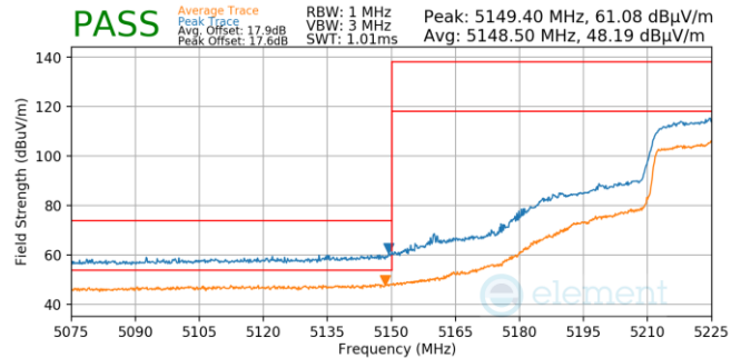
Plot 7-759. Antenna 5b (Pk & Avg, Ch.46, 802.11n, MCS2)
