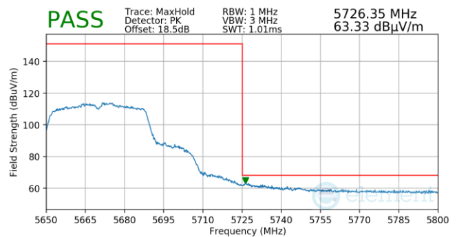
Plot 7-778. Antenna 5b (Pk, Ch.134, 802.11n, MCS2)
