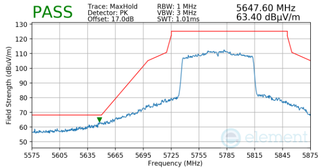
Plot 7-834. Antenna 5b (Pk, Ch.155, 802.11ac, MCS4)
