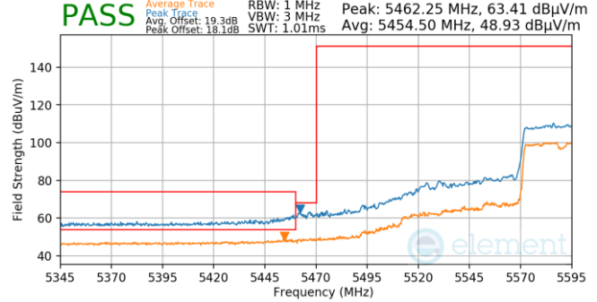
Plot 7-829. (FCC Only) Antenna 5b (Pk & Avg, Ch.122, 802.11ac, MCS9)
