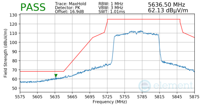
Plot 7-833. Antenna 5b (Pk, Ch.155, 802.11ac, MCS2)
