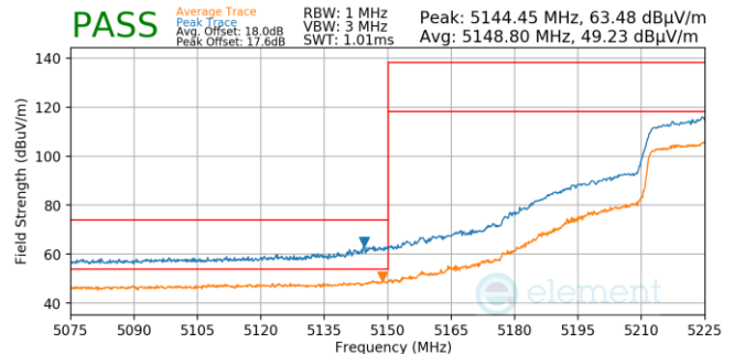
Plot 7-760. Antenna 5b (Pk & Avg, Ch.46, 802.11n, MCS4)
