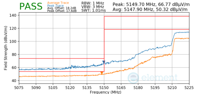
Plot 7-761. Antenna 5b (Pk & Avg, Ch.46, 802.11n, MCS7)
