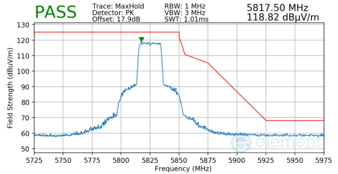
Plot 7-754. Antenna 5b (Pk, Ch.165, 802.11ax(SU), MCS4)
