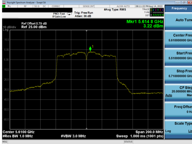
Plot 7-419. PSD CDD Antenna 5b (80MHz BW 802.11ac – Ch. 122, MCS2)
