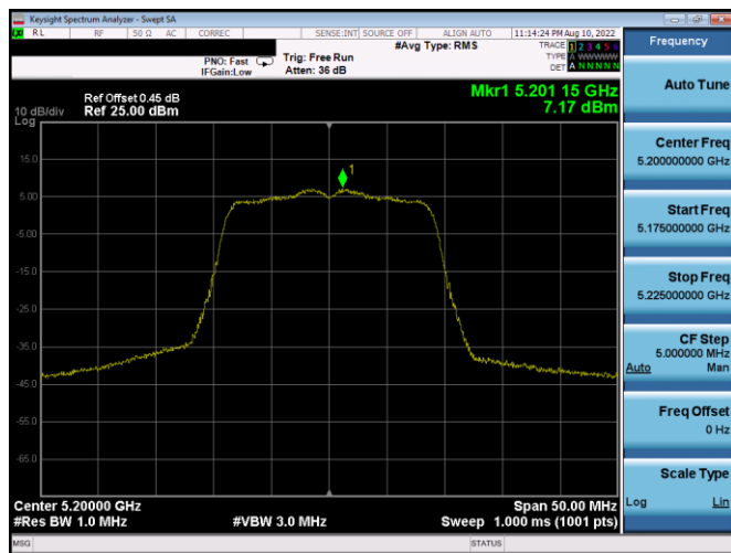
Plot 7-427. PSD SDM Antenna 5b (20MHz BW 802.11n - Ch. 40, MCS12)
