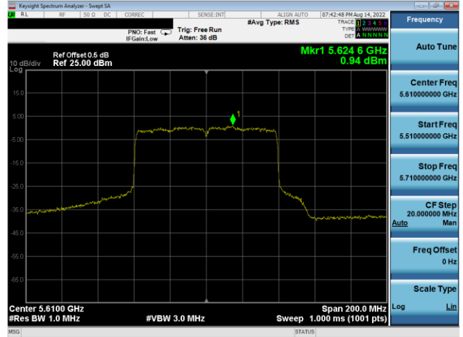
Plot 7-422. PSD CDD Antenna 4a (80MHz BW 802.11ax(SU) – Ch. 122, MCS2)
