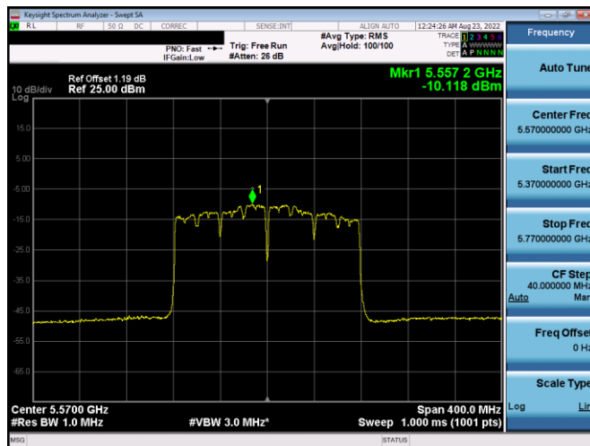
Plot 7-469. PSD CDD Antenna 5b (160MHz BW 802.11ac – Ch. 114, MCS4)
