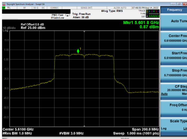
Plot 7-421. PSD CDD Antenna 5b (80MHz BW 802.11ax(SU) – Ch. 122, MCS2)
