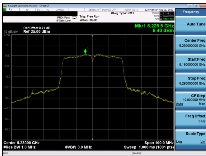
Plot 7-431. PSD SDM Antenna 5b (40MHz BW 802.11n - Ch. 46, MCS4)
