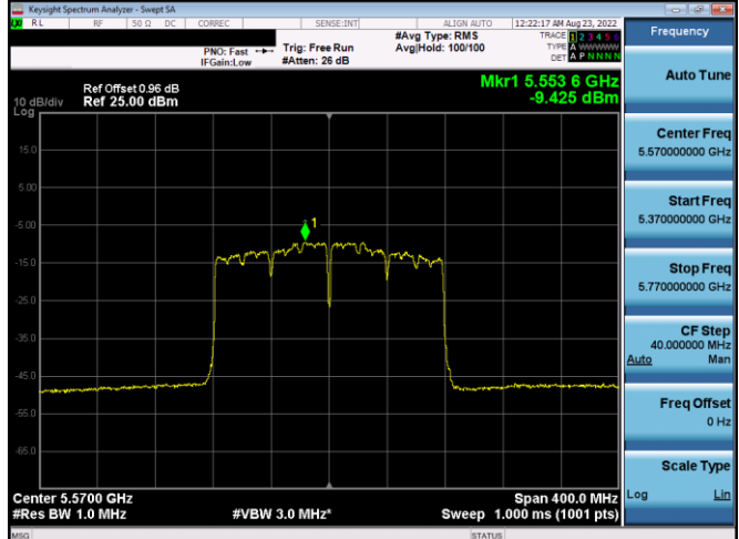
Plot 7-423. PSD CDD Antenna 5b (160MHz BW 802.11ax(SU)– Ch. 114, MCS2)
