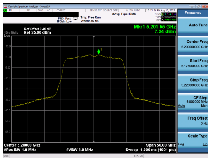
Plot 7-428. PSD SDM Antenna 4a (20MHz BW 802.11n - Ch. 40, MCS4)
