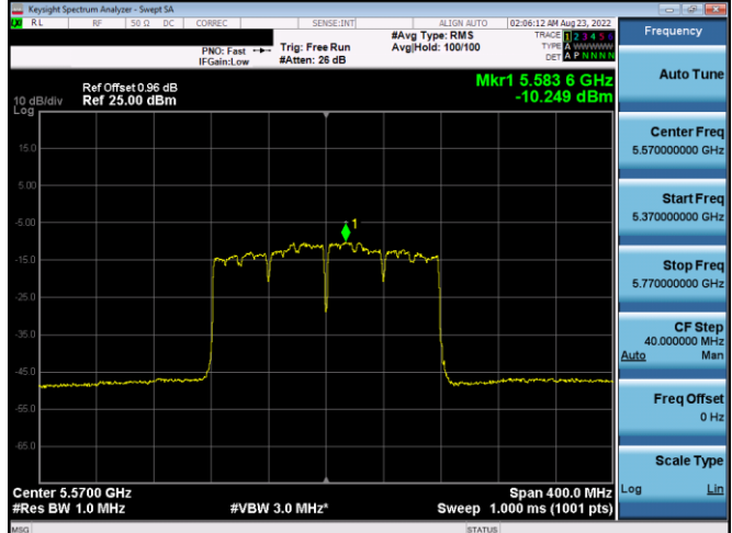
Plot 7-424. PSD CDD Antenna 4a (160MHz BW 802.11ax(SU)– Ch. 114, MCS2)
