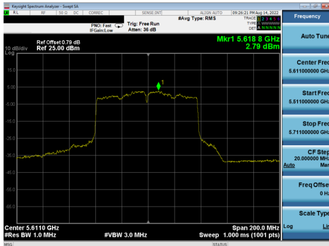
Plot 7-420. PSD CDD Antenna 4a (80MHz BW 802.11ac – Ch. 122, MCS2)
