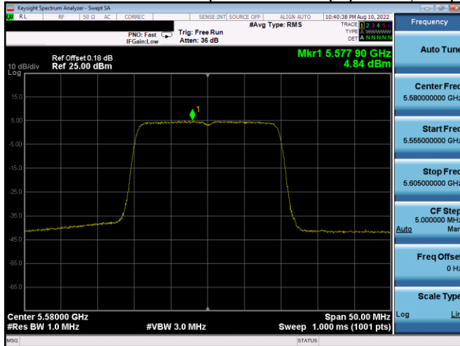
Plot 7-414. PSD CDD Antenna 4a (20MHz BW 802.11ax(SU) – Ch. 116, MCS2)
