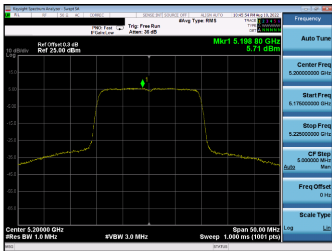
Plot 7-430. PSD CDD Antenna 4a (20MHz BW 802.11ax(SU) - Ch. 40, MCS4)
