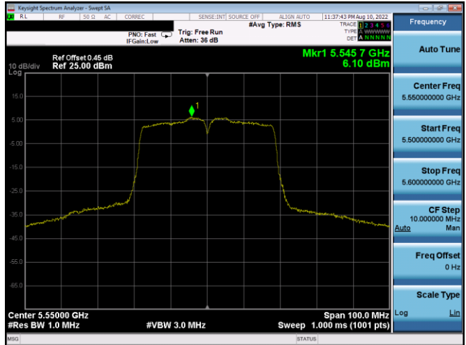
Plot 7-416. PSD CDD Antenna 4a (40MHz BW 802.11n – Ch. 110, MCS10)
