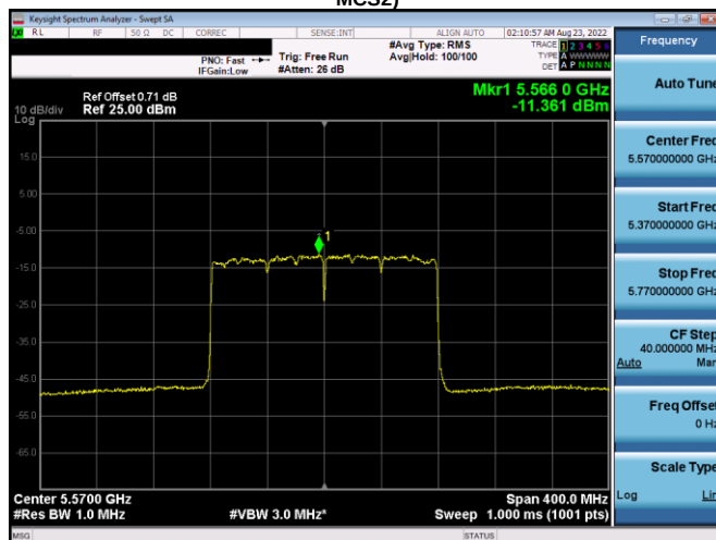
Plot 7-426. PSD CDD Antenna 4a (160MHz BW 802.11ac - Ch. 114, MCS2)
