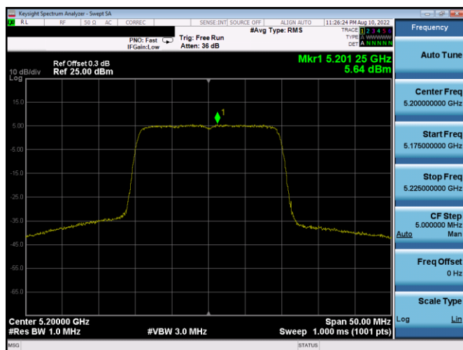
Plot 7-429. PSD CDD Antenna 5b (20MHz BW 802.11ax(SU) - Ch. 40, MCS4)
