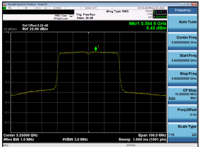
Plot 7-418. PSD CDD Antenna 4a (40MHz BW 802.11ax(SU) – Ch. 110, MCS2)
