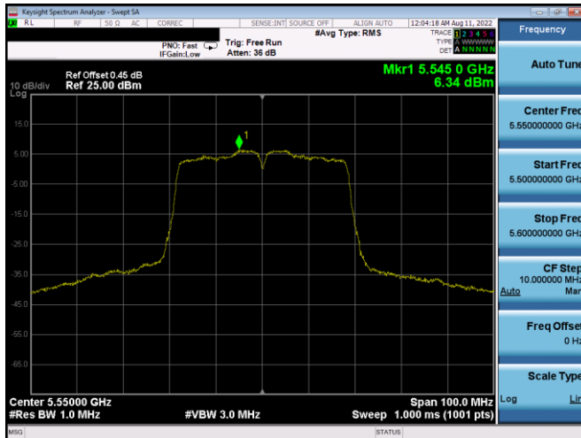
Plot 7-415. PSD CDD Antenna 5b (40MHz BW 802.11n – Ch. 110, MCS10)
