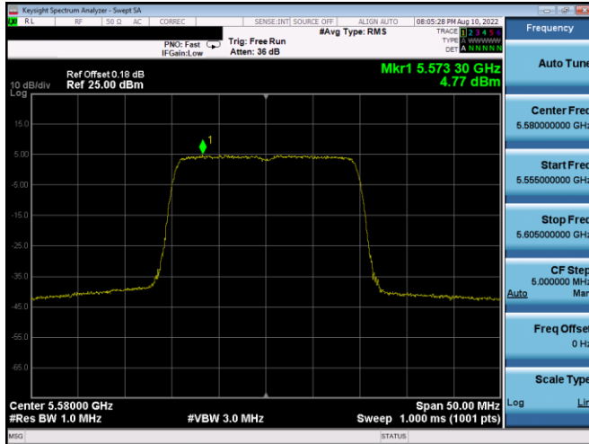
Plot 7-413. PSD CDD Antenna 5b (20MHz BW 802.11ax(SU) – Ch. 116, MCS2)
