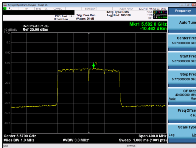
Plot 7-425. PSD CDD Antenna 5b (160MHz BW 802.11ax(SU)- Ch. 114, MCS2)
