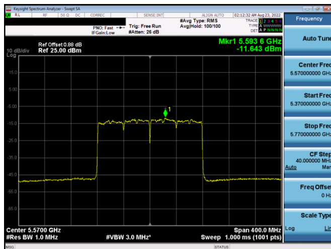
Plot 7-470. PSD CDD Antenna 4a (160MHz BW 802.11ac – Ch. 114, MCS4)
