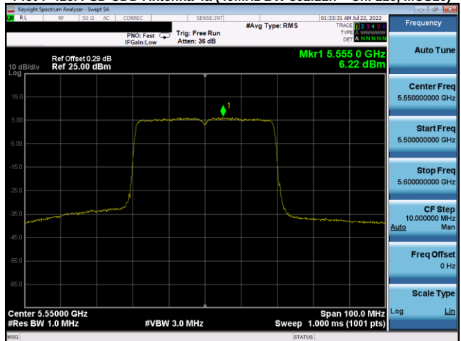
Plot 7-417. PSD CDD Antenna 5b (40MHz BW 802.11ax(SU) – Ch. 110, MCS2)
