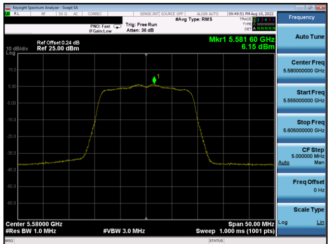
Plot 7-412. PSD CDD Antenna 4a (20MHz BW 802.11n - Ch. 116, MCS10)
