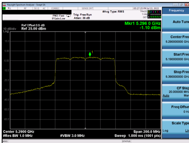
Plot 7-409. PSD CDD Antenna 5b (80MHz BW 802.11ax(SU) - Ch. 58, MCS2)
