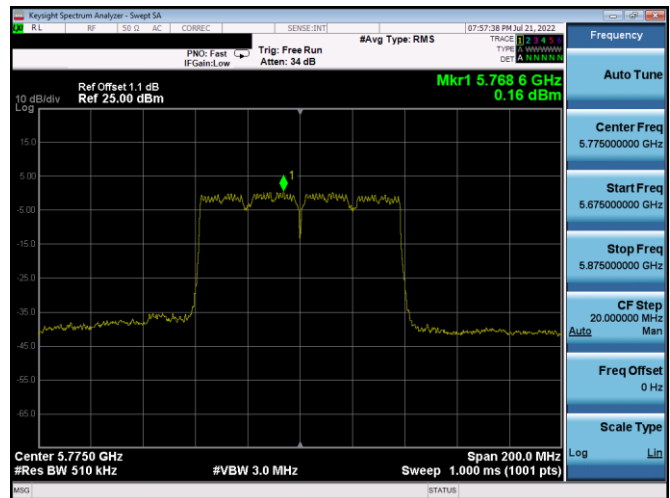
Plot 7-357. PSD Antenna 4a (80MHz BW 802.11ac – Ch. 155, MCS9)
