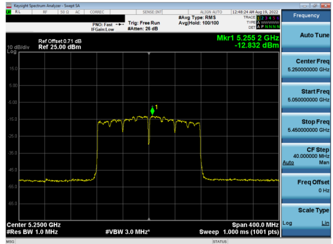
Plot 7-398. PSD CDD Antenna 4a (MHz BW 802.11ac – Ch. 50, MCS2)
