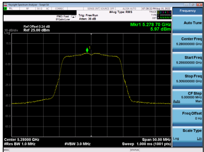
Plot 7-399. PSD SDM Antenna 5b (20MHz BW 802.11n – Ch. 56, MCS10)
