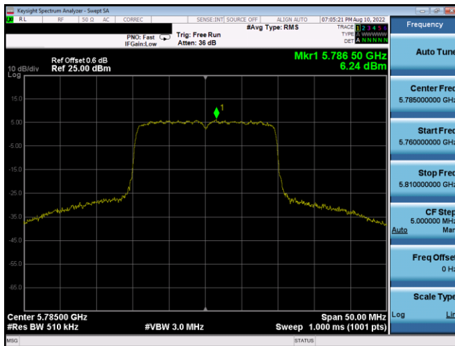
Plot 7-354. PSD Antenna 4a (20MHz BW 802.11ax(SU) – Ch. 157, MCS11)
