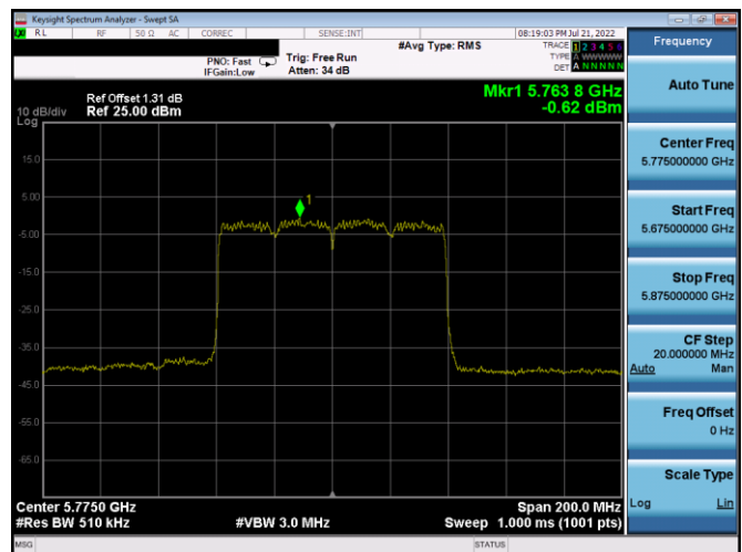
Plot 7-358. PSD Antenna 4a (80MHz BW 802.11ax(SU) – Ch. 155, MCS11)
