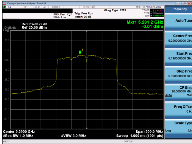
Plot 7-407. PSD CDD Antenna 5b (80MHz BW 802.11ac - Ch. 58, MCS2)
