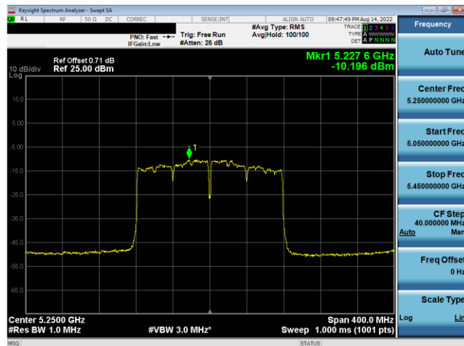
Plot 7-365. ISED PSD Antenna 4a (160MHz BW 11ac- Ch.50 MCS2)
