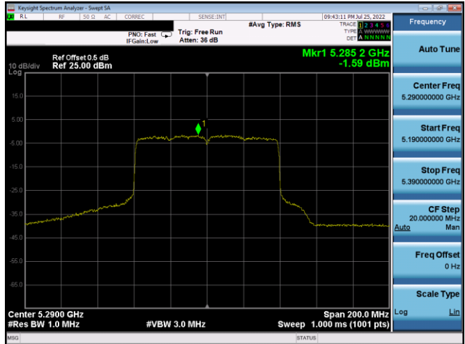
Plot 7-410. PSD CDD Antenna 4a (80MHz BW 802.11ax(SU) - Ch. 58, MCS2)
