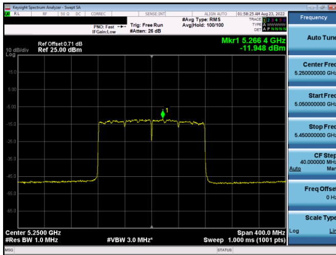
Plot 7-396. PSD CDD Antenna 4a (160MHz BW 802.11ax(SU) – Ch. 50, MCS2)
