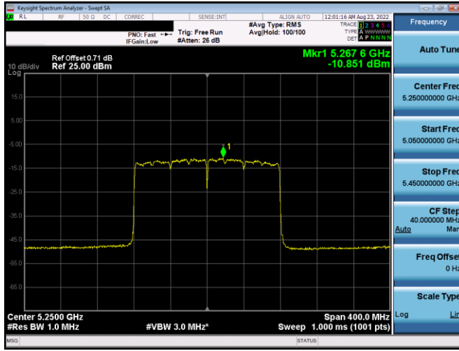
Plot 7-395. PSD CDD Antenna 5b (160MHz BW 802.11ax(SU) – Ch. 50, MCS2)
