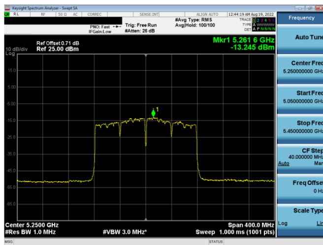
Plot 7-397. PSD CDD Antenna 5b (160MHz BW 802.11ac – Ch. 50, MCS2)
