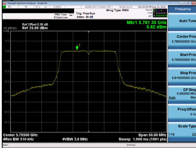
Plot 7-353. PSD Antenna 4a (20MHz BW 802.11n – Ch. 157, MCS7)
