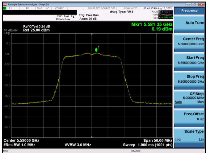
Plot 7-411. PSD CDD Antenna 5b (20MHz BW 802.11n - Ch. 116, MCS10)
