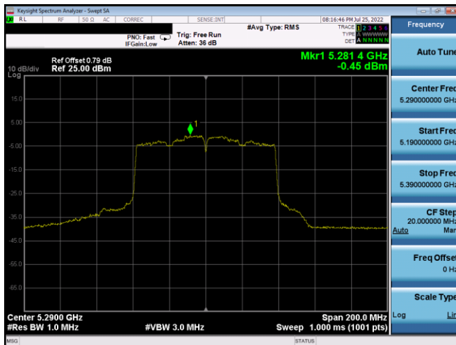
Plot 7-408. PSD CDD Antenna 4a (80MHz BW 802.11ac - Ch. 58, MCS2)
