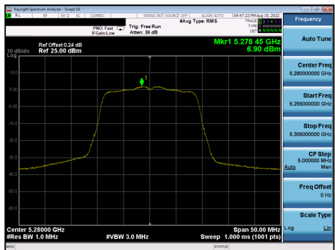
Plot 7-400. PSD SDM Antenna 4a (20MHz BW 802.11n – Ch. 56, MCS10)
