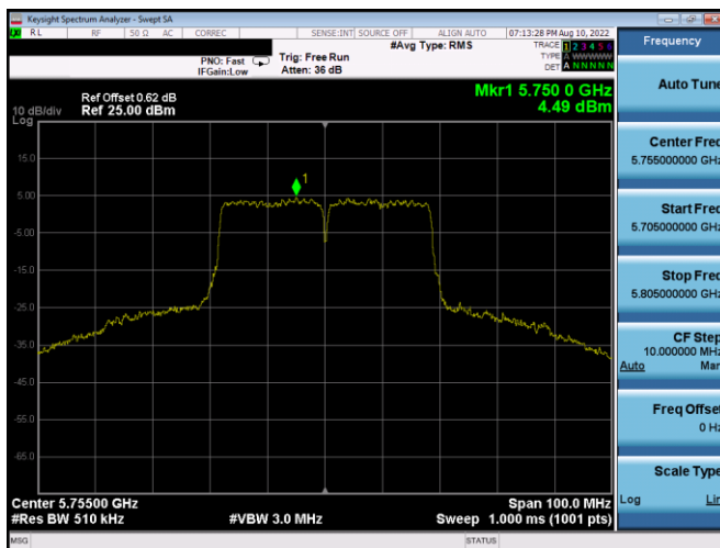
Plot 7-355. PSD Antenna 4a (40MHz BW 802.11n – Ch. 151, MCS7)
