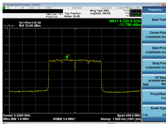
Plot 7-366. ISED PSD Antenna 4a (160MHz BW 11ax(SU) – Ch.50 MCS2)
