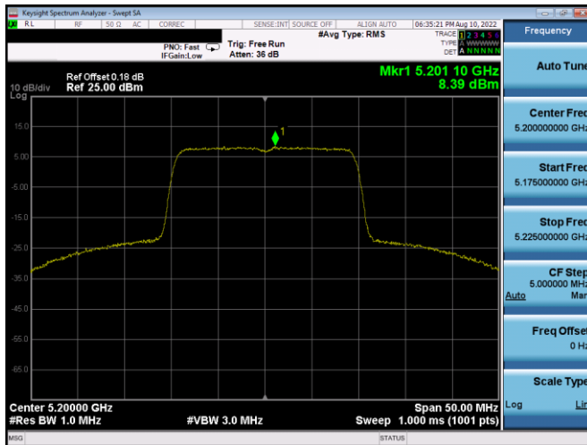
Plot 7-276. PSD Antenna 4a (20MHz BW 802.11ax(SU) - Ch. 40, MCS2)
