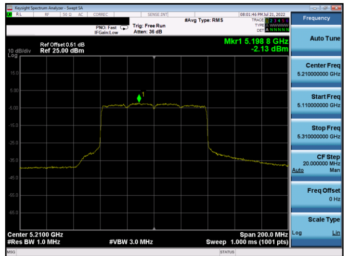
Plot 7-280. PSD Antenna 4a (80MHz BW 802.11ax(SU) - Ch. 42, MCS2)
