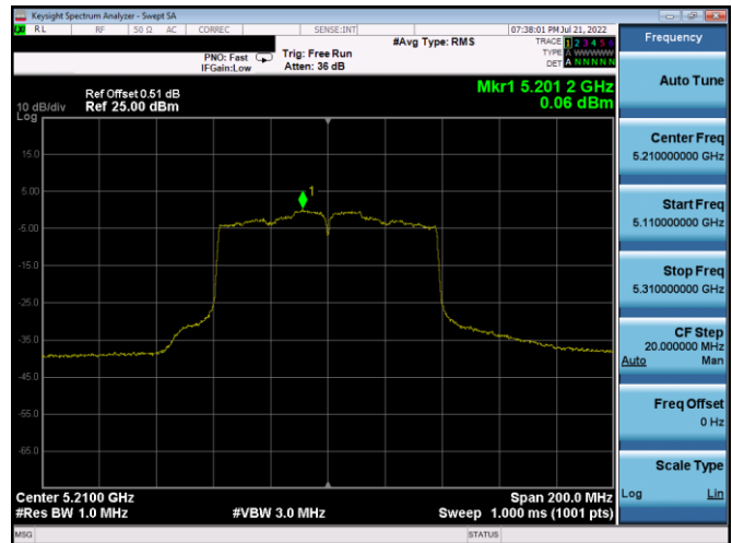
Plot 7-279. PSD Antenna 4a (80MHz BW 802.11ac - Ch. 42, MCS2)
