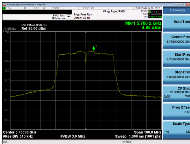
Plot 7-235. PSD Antenna 5b (40MHz BW 802.11n – Ch. 151, MCS4)
