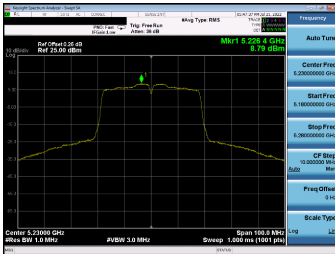
Plot 7-277. PSD Antenna 4a (40MHz BW 802.11n - Ch. 46, MCS2)
