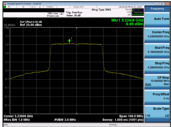
Plot 7-278. PSD Antenna 4a (40MHz BW 802.11ax(SU) - Ch. 46, MCS2)
