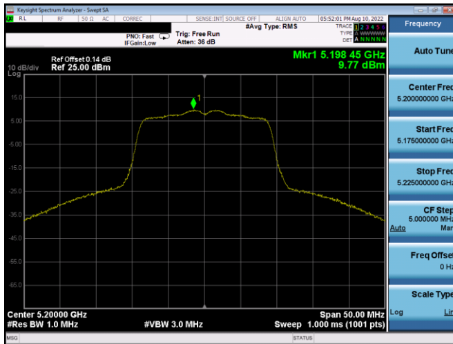
Plot 7-275. PSD Antenna 4a (20MHz BW 802.11n - Ch. 40, MCS2)
