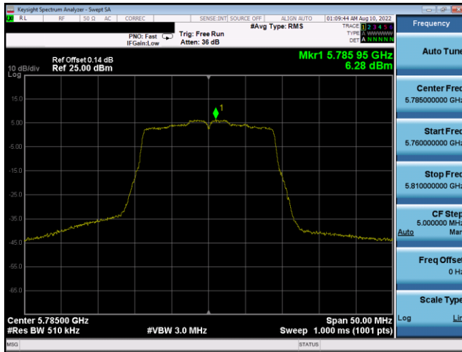
Plot 7-233. PSD Antenna 5b (20MHz BW 802.11n – Ch. 157, MCS2)
