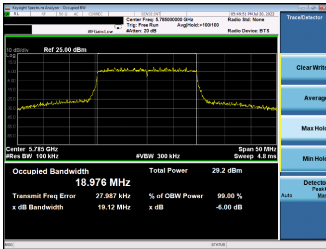
Plot 7-140. 6dB BW & 99% OBW Antenna 5b (20MHz BW 802.11ax(SU) – Ch. 157, MCS4)
