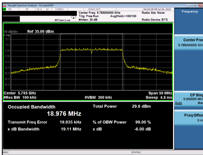
Plot 7-146. 6dB BW & 99% OBW Antenna 5b (20MHz BW 802.11ax(SU) – Ch. 157, MCS11)
