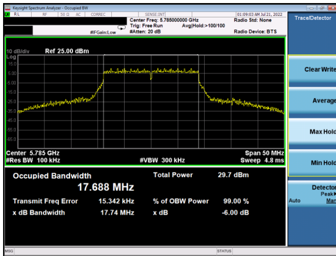
Plot 7-163. 6dB BW & 99% OBW Antenna 4a (20MHz BW 802.11n – Ch. 157, MCS7)
