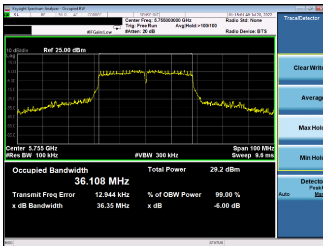
Plot 7-141. 6dB BW & 99% OBW Antenna 5b (40MHz BW 802.11n – Ch. 151, MCS4)
