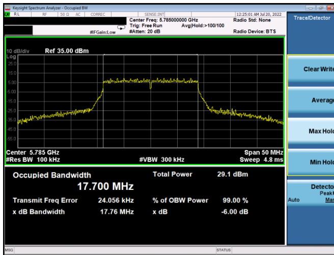
Plot 7-145. 6dB BW & 99% OBW Antenna 5b (20MHz BW 802.11n – Ch. 157, MCS7)
