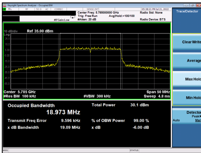
Plot 7-164. 6dB BW & 99% OBW Antenna 4a (20MHz BW 802.11ax(SU) – Ch. 157, MCS11)
