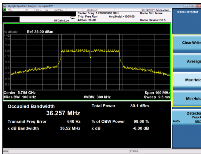
Plot 7-165. 6dB BW & 99% OBW Antenna 4a (40MHz BW 802.11n – Ch. 151, MCS9)
