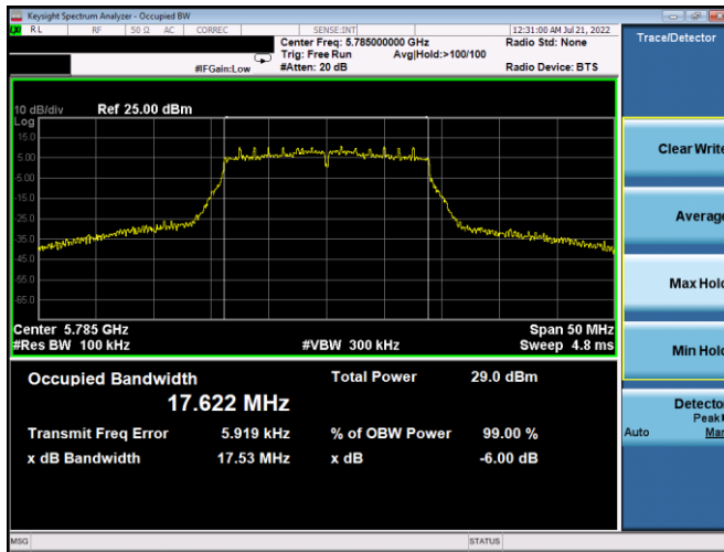
Plot 7-151. 6dB BW & 99% OBW Antenna 4a (20MHz BW 802.11n – Ch. 157, MCS2)
