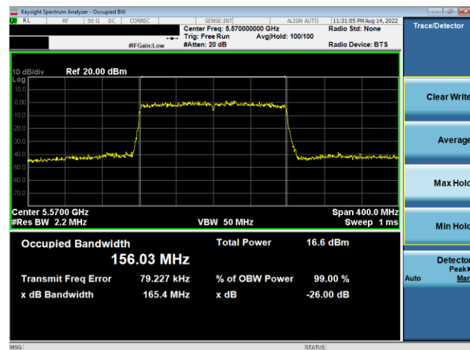
Plot 7-43. 26dB BW & 99% OBW Antenna 5b (160MHz BW 802.11ac – Ch. 114, MCS0)
