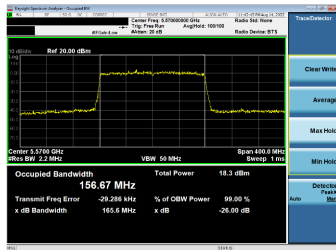
Plot 7-21. 26dB BW & 99% OBW Antenna 5b (160MHz BW 802.11ac – Ch. 114, MCS2)
