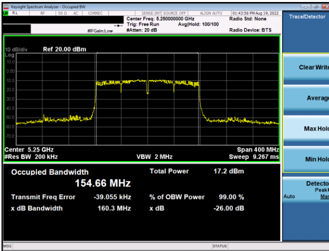
Plot 7-8. 26dB BW & 99% OBW Antenna 5b (160MHz BW 802.11ac – Ch. 50, MCS2)
