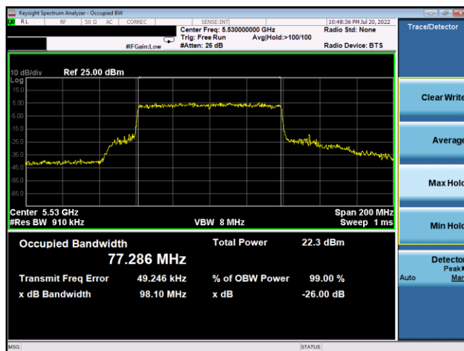
Plot 7-42. 26dB BW & 99% OBW Antenna 5b (80MHz BW 802.11ax(SU) – Ch. 106, MCS4)
