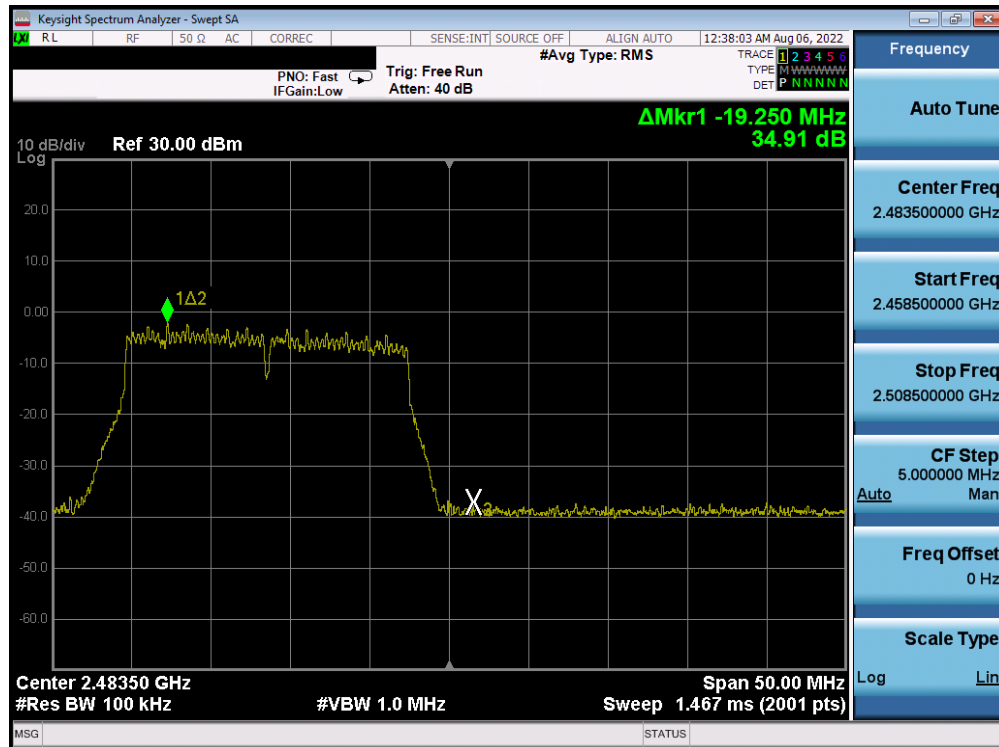
Plot 7-287. Band Edge Plot Antenna 4a (802.11n (2.4GHz) – Ch. 13) – MCS5
