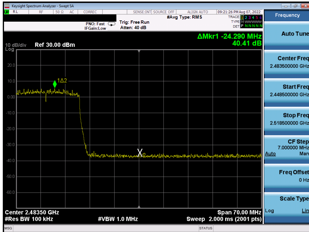
Plot 7-298. Band Edge Plot Antenna 4a (802.11ax (SU - 2.4GHz) – Ch. 10) – MCS5
