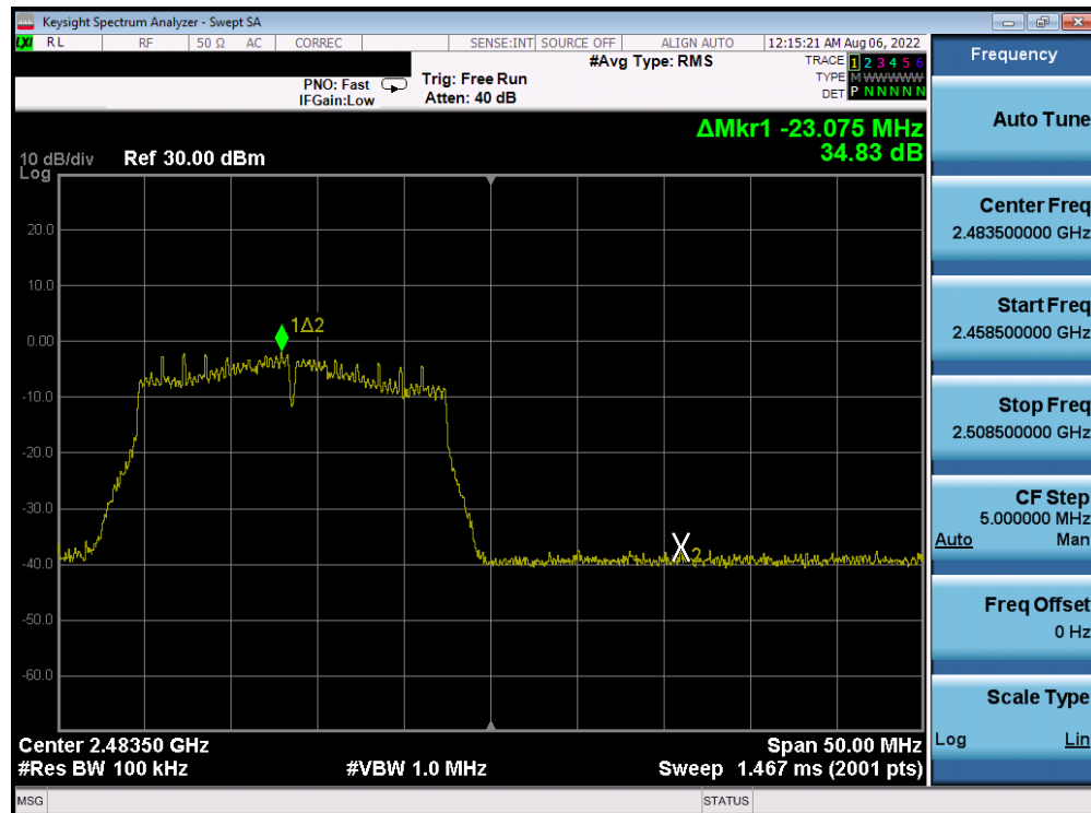
Plot 7-240. Band Edge Plot Antenna 4a (802.11n (2.4GHz) - Ch. 13) - MCS3
