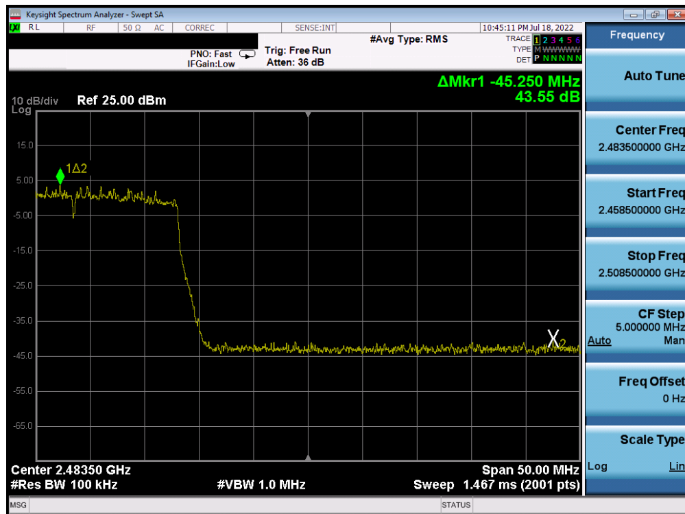
Plot 7-299. Band Edge Plot Antenna 4a (802.11ax (SU - 2.4GHz) – Ch. 11) – MCS5
