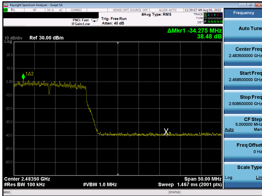
Plot 7-286. Band Edge Plot Antenna 4a (802.11n (2.4GHz) – Ch. 12) – MCS5
