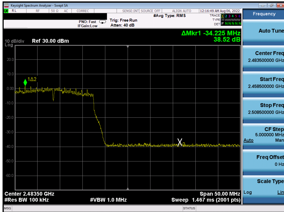
Plot 7-239. Band Edge Plot Antenna 4a (802.11n (2.4GHz) - Ch. 12) - MCS3
