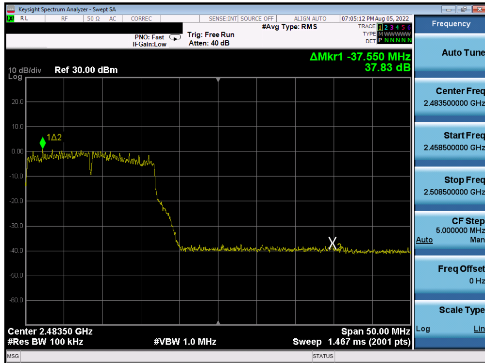
Plot 7-272. Band Edge Plot Antenna 4a (802.11g – Ch. 12) – 36Mbps
