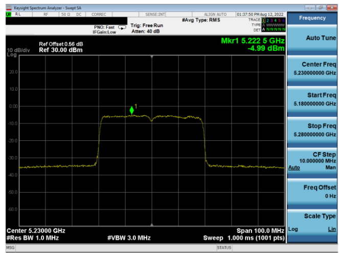
Plot 7-382. ISED PSD CDD Antenna WF4a (40MHz BW 11ax - RU484 - Ch.46)
