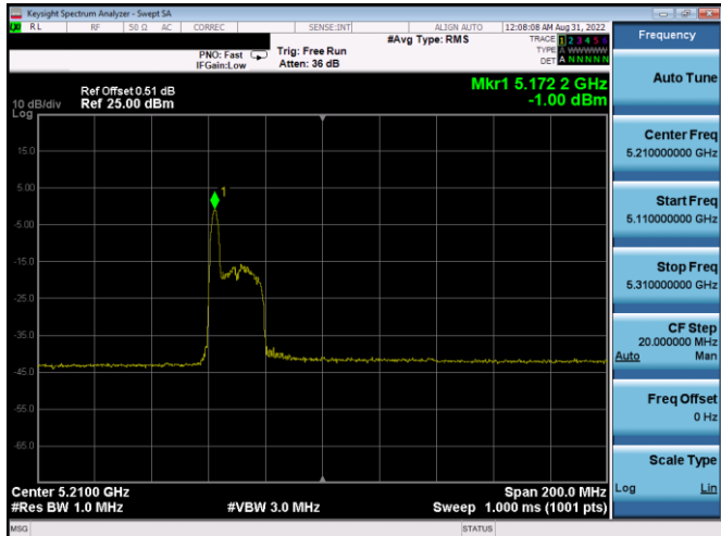
Plot 7-384. ISED PSD SDM Antenna WF4a (80MHz BW 11ax Index 0 - RU26 - Ch.42)
