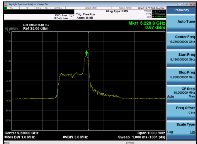
Plot 7-377. ISSED PSD SDM Antenna WF5b (40MHz BW 11ax Index 8 - RU26 - Ch.46)
