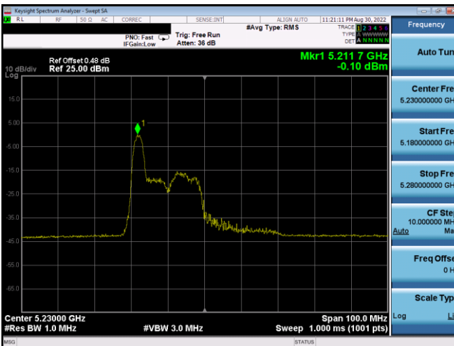
Plot 7-375. ISSED PSD SDM Antenna WF5b (40MHz BW 11ax Index 0 - RU26 - Ch.46)
