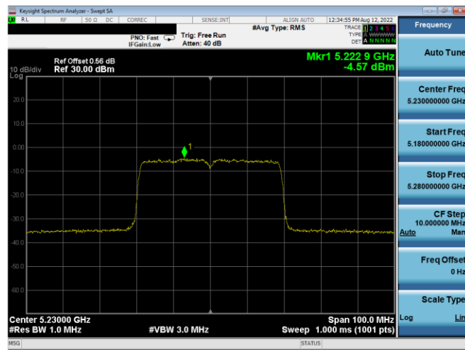
Plot 7-381. ISED PSD SDM Antenna WF5b (40MHz BW 11ax - RU484 - Ch.46)
