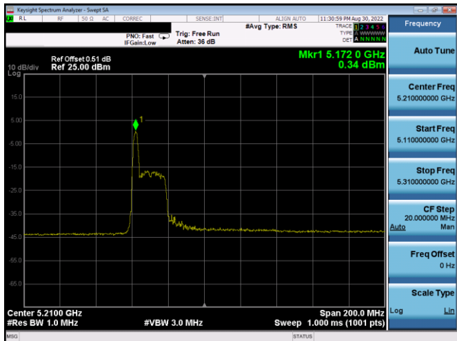
Plot 7-383. ISED PSD SDM Antenna WF5b (80MHz BW 11ax Index 0 - RU26 - Ch.42)
