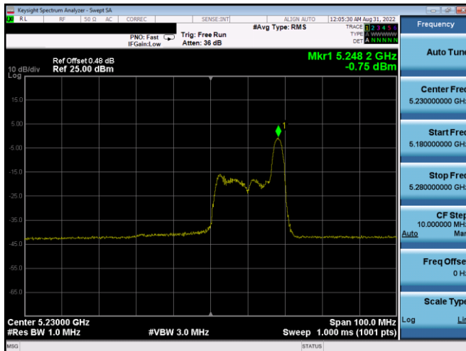
Plot 7-380. ISED PSD SDM Antenna WF4a (40MHz BW 11ax Index 17 - RU26 - Ch.46)
