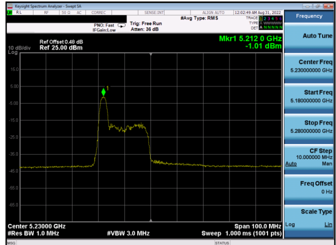
Plot 7-376. ISSED PSD SDM Antenna WF4a (40MHz BW 11ax Index 0 - RU26 - Ch.46)
