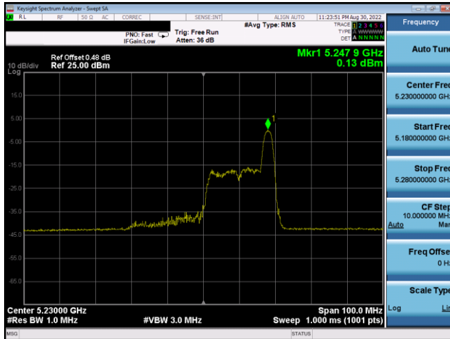
Plot 7-379. ISED PSD SDM Antenna WF5b (40MHz BW 11ax Index 17 - RU26 - Ch.46)
