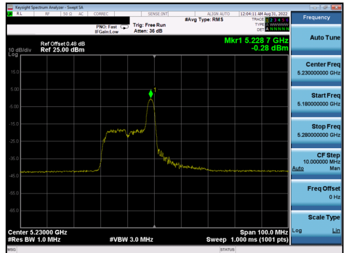
Plot 7-378. ISSED PSD SDM Antenna WF4a (40MHz BW 11ax Index 8 - RU26 - Ch.46)
