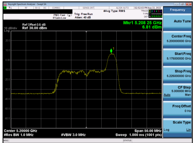
Plot 7-259. PSD SDM Antenna WF5b (20MHz BW 11ax Index 8– RU26 – Ch.40)
