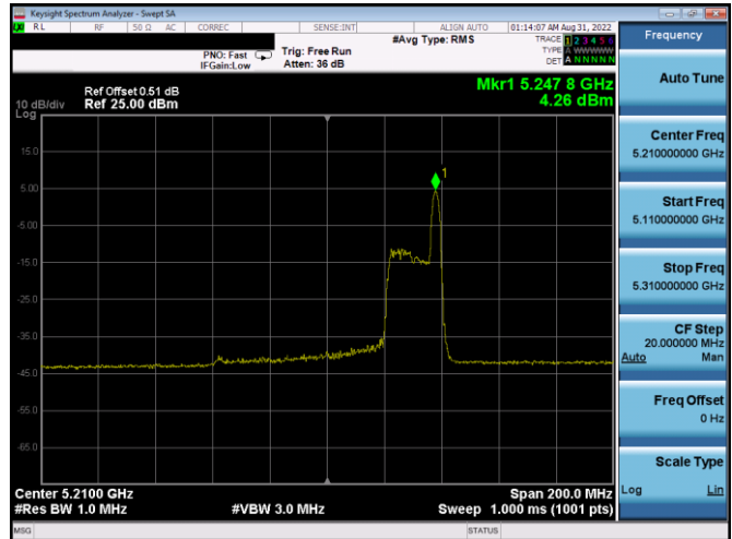
Plot 7-276. PSD SDM Antenna WF4a (80MHz BW 11ax Index 36 – RU26 – Ch.42)
