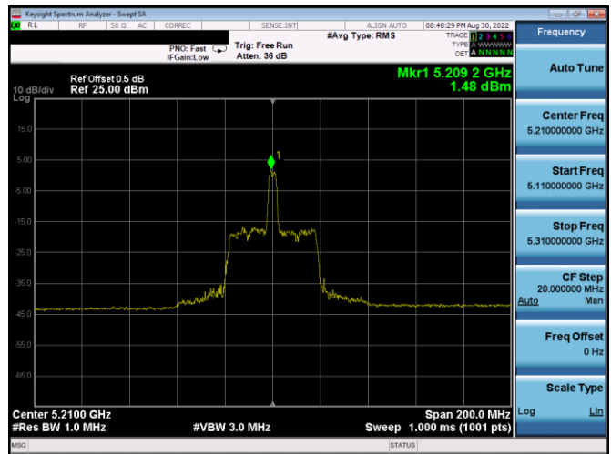
Plot 7-249. ISSED PSD Antenna WF4a (80MHz BW 11ax Index 18 - RU26 - Ch.42)
