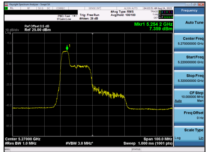
Plot 7-295. PSD SDM Antenna WF5b (40MHz BW 11ax Index 37 - RU52 - Ch.54)
