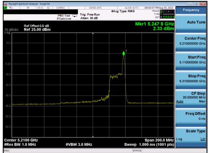
Plot 7-250. ISSED PSD Antenna WF4a (80MHz BW 11ax Index 36 - RU26 - Ch.42)
