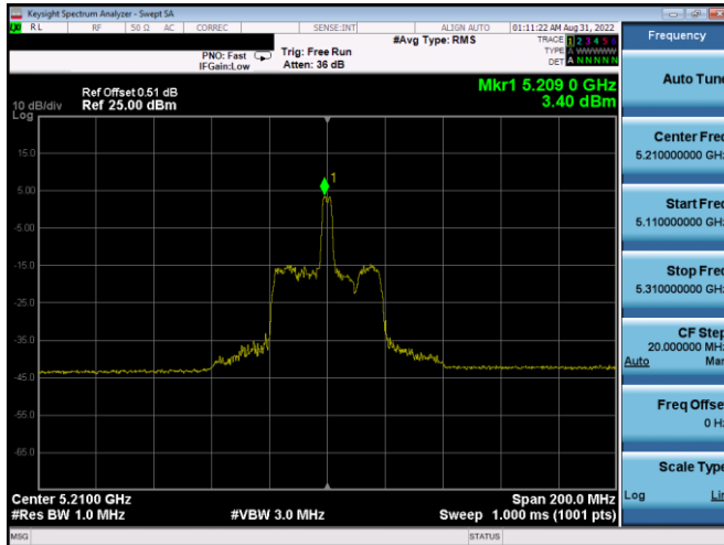
Plot 7-273. PSD SDM Antenna WF5b (80MHz BW 11ax Index 18 – RU26 – Ch.42)
