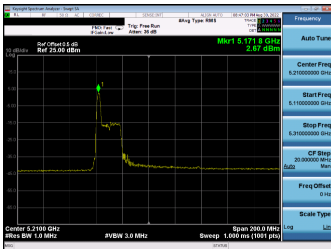
Plot 7-248. ISSED PSD Antenna WF4a (80MHz BW 11ax Index 0 - RU26 - Ch.42)
