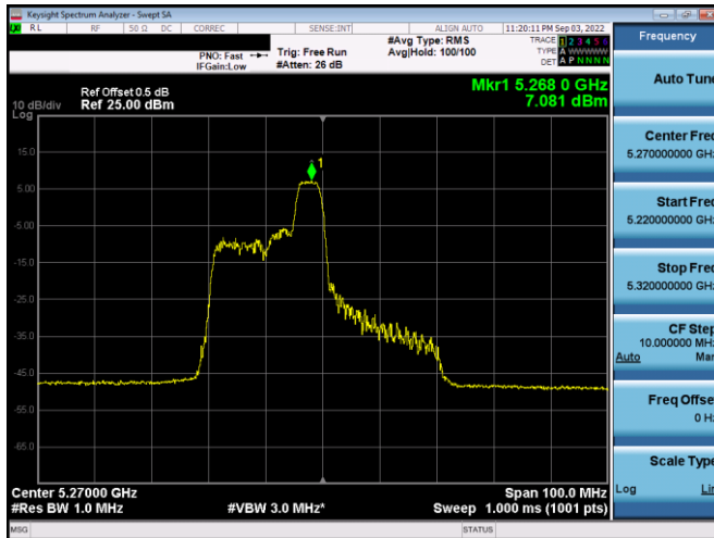
Plot 7-298. PSD SDM Antenna WF4a (40MHz BW 11ax Index 40 – RU52 – Ch.54)
