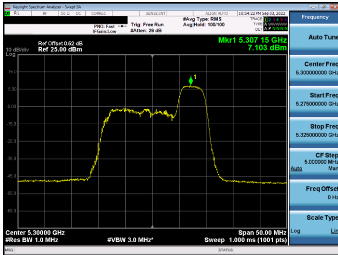
Plot 7-292. PSD SDM Antenna WF4a (20MHz BW 11ax Index 40- RU52 - Ch.60)
