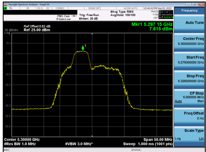
Plot 7-289. PSD SDM Antenna WF5b (20MHz BW 11ax Index 38 - RU52 - Ch.60)
