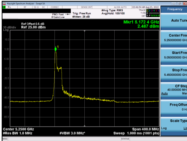
Plot 7-279. PSD CDD Antenna WF5b (20MHz BW 11ax Index 37 – RU52 – Ch.50)
