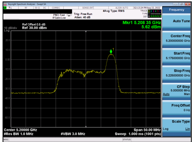
Plot 7-260. PSD SDM Antenna WF4a (20MHz BW 11ax Index 8– RU26 – Ch.40)
