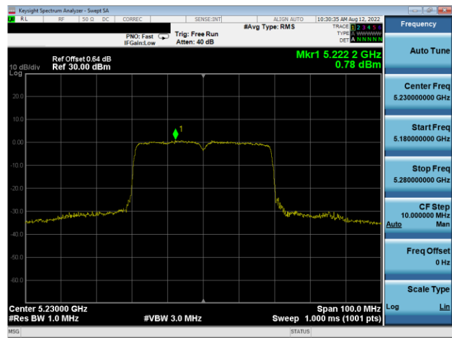
Plot 7-247. ISSED PSD Antenna WF4a (40MHz BW 11ax - RU484 - Ch.46)
