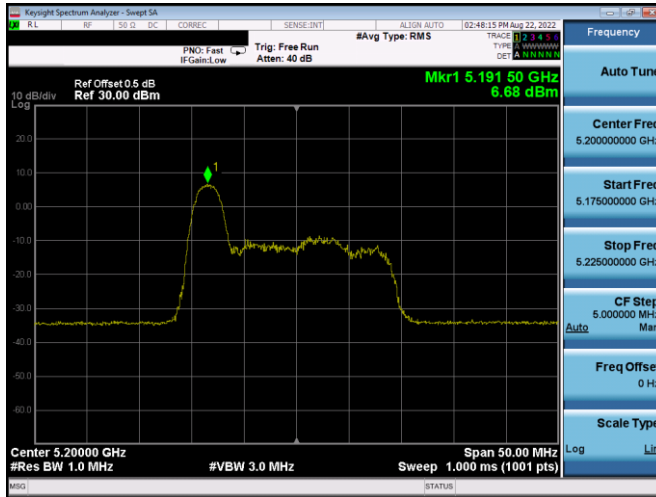
Plot 7-255. PSD SDM Antenna WF5b (20MHz BW 11ax Index 0 – RU26 – Ch.40)
