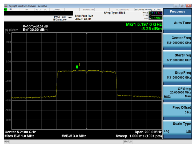
Plot 7-251. ISSED PSD Antenna WF4a (80MHz BW 11ax - RU996 - Ch.42)
