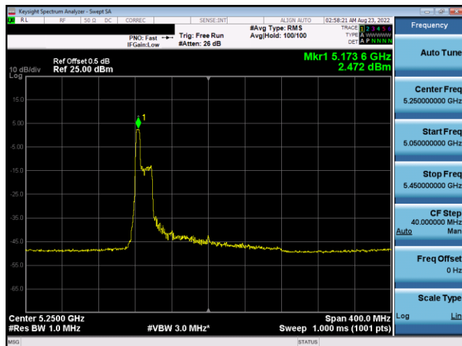
Plot 7-252. ISED PSD Antenna WF4a (160MHz BW 11ax Index 37 – RU52 – Ch.50(L))
