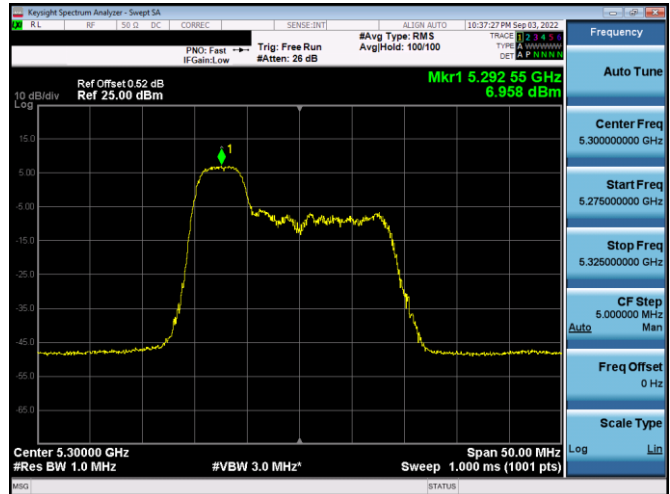
Plot 7-288. PSD SDM Antenna WF4a (20MHz BW 11ax Index 37 - RU52 - Ch.60)
