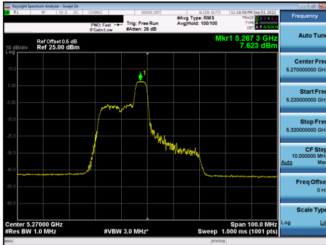
Plot 7-297. PSD SDM Antenna WF5b (40MHz BW 11ax Index 40 – RU52 – Ch.54)
