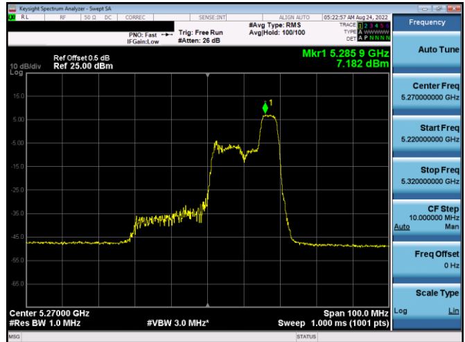
Plot 7-300. PSD SDM Antenna WF4a (40MHz BW 11ax Index 44 – RU52 – Ch.54)
