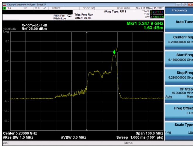
Plot 7-246. ISSED PSD Antenna WF4a (40MHz BW 11ax Index 17 - RU26 - Ch.46)
