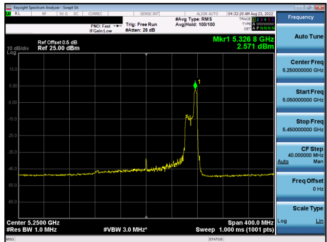
Plot 7-284. PSD CDD Antenna WF4a (20MHz BW 11ax Index 52– RU52 – Ch.50)
