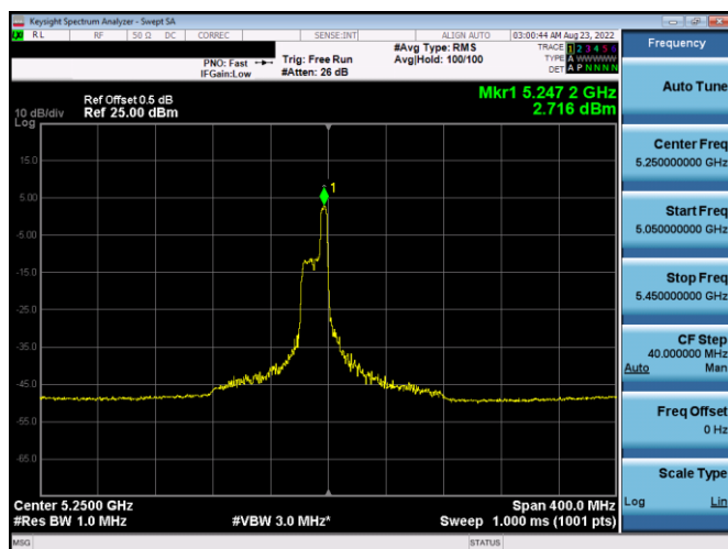
Plot 7-253. ISED PSD Antenna WF4a (160MHz BW 11ax Index 52 – RU52 – Ch.50(L))
