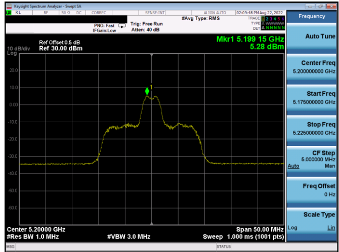
Plot 7-258. PSD SDM Antenna WF4a (20MHz BW 11ax Index 4 – RU26 – Ch.40)
