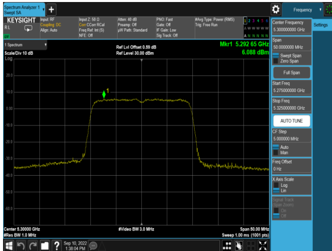
Plot 7-293. PSD SDM Antenna WF5b (20MHz BW 11ax- RU242 - Ch.60)
