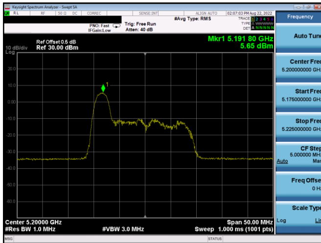
Plot 7-256. PSD SDM Antenna WF4a (20MHz BW 11ax Index 0 – RU26 – Ch.40)
