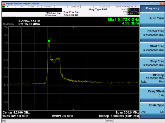
Plot 7-271. PSD SDM Antenna WF5b (80MHz BW 11ax Index 0 - RU26 - Ch.42)
