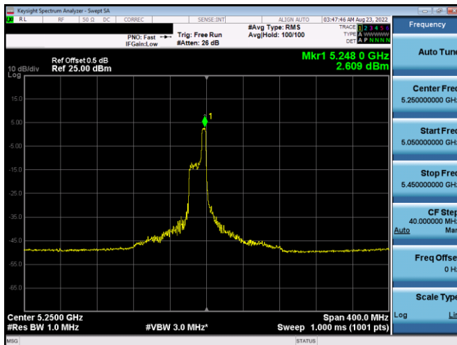
Plot 7-281. PSD CDD Antenna WF5b (20MHz BW 11ax Index 44 – RU52 – Ch.50)
