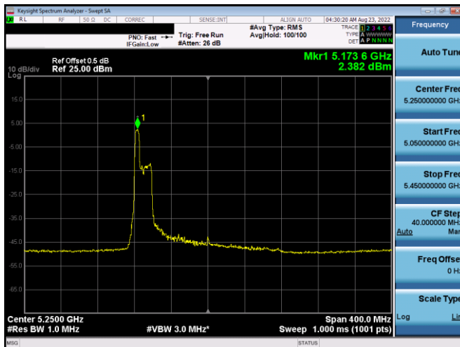
Plot 7-280. PSD CDD Antenna WF4a (20MHz BW 11ax Index 37 – RU52 – Ch.50)
