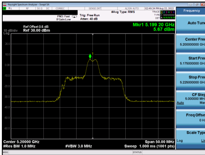
Plot 7-257. PSD SDM Antenna WF5b (20MHz BW 11ax Index 4 – RU26 – Ch.40)
