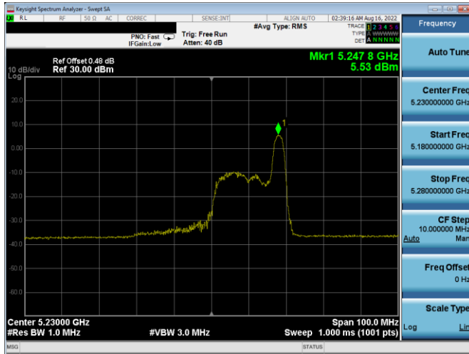
Plot 7-267. PSD SDM Antenna WF5b (40MHz BW 11ax Index 17 - RU26 - Ch.46)
