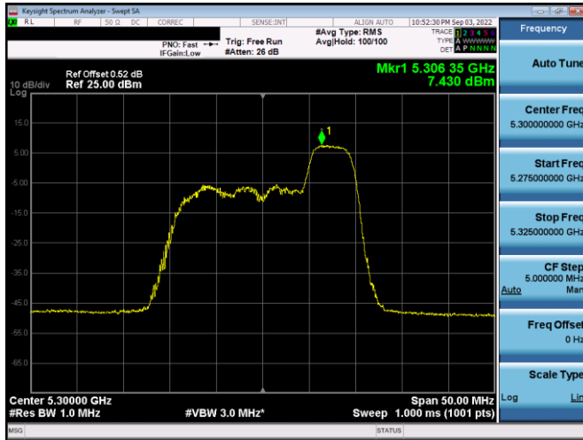
Plot 7-291. PSD SDM Antenna WF5b (20MHz BW 11ax Index 40- RU52 - Ch.60)
