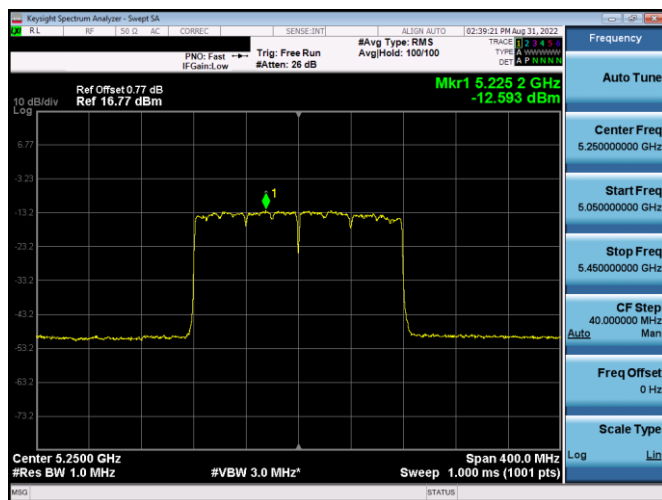
Plot 7-254. ISED PSD Antenna WF4a (160MHz BW 11ax – RU996x2 – Ch.50)
