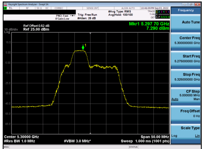
Plot 7-290. PSD SDM Antenna WF4a (20MHz BW 11ax Index 38 - RU52 - Ch.60)
