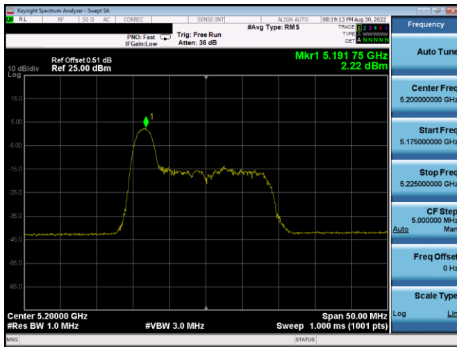
Plot 7-240. ISED PSD Antenna WF4a (20MHz BW 11ax Index 0 – RU26 – Ch.40)
