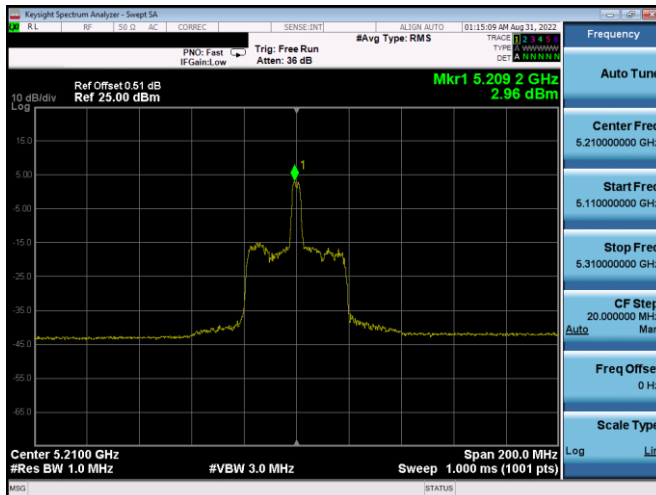
Plot 7-274. PSD SDM Antenna WF4a (80MHz BW 11ax Index 18 – RU26 – Ch.42)
