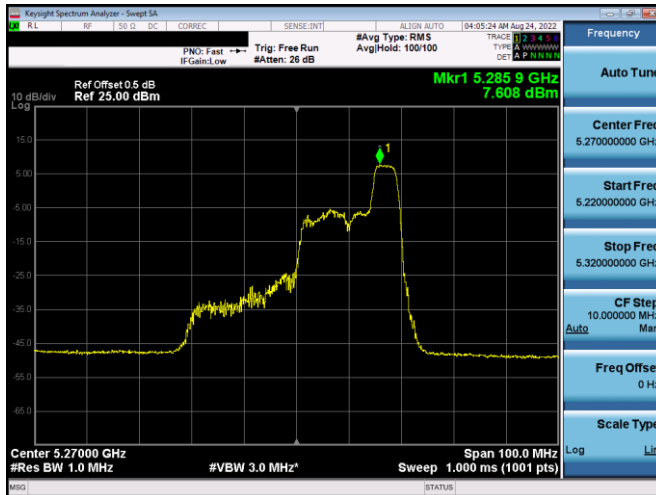
Plot 7-299. PSD SDM Antenna WF5b (40MHz BW 11ax Index 44 – RU52 – Ch.54)
