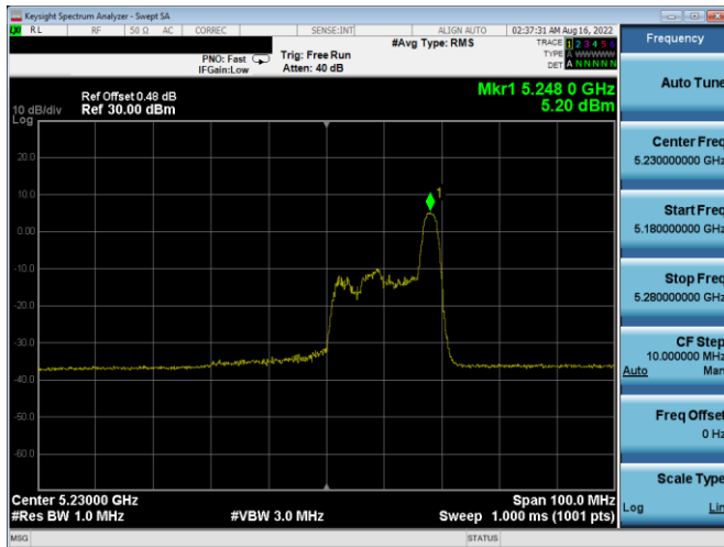
Plot 7-268. PSD SDM Antenna WF4a (40MHz BW 11ax Index 17 - RU26 - Ch.46)
