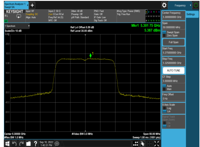
Plot 7-294. PSD SDM Antenna WF4a (20MHz BW 11ax- RU242 - Ch.60)
