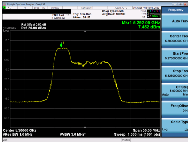
Plot 7-287. PSD SDM Antenna WF5b (20MHz BW 11ax Index 37 - RU52 - Ch.60)
