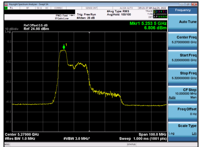
Plot 7-296. PSD SDM Antenna WF4a (40MHz BW 11ax Index 37 - RU52 - Ch.54)
