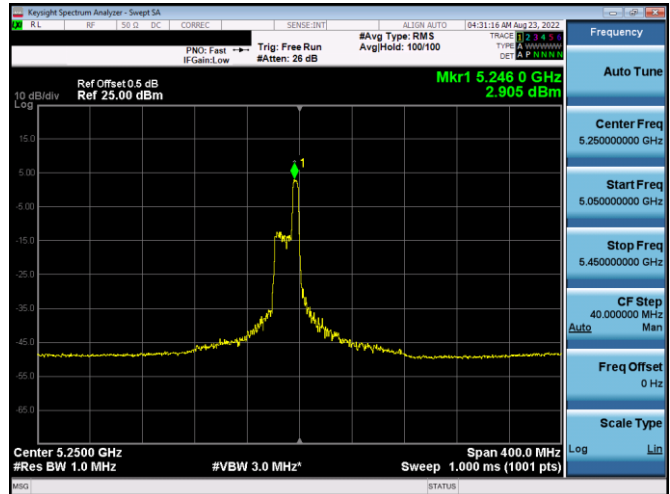
Plot 7-282. PSD CDD Antenna WF4a (20MHz BW 11ax Index 44 – RU52 – Ch.50)
