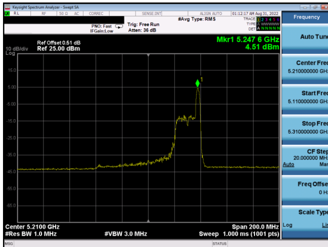
Plot 7-275. PSD SDM Antenna WF5b (80MHz BW 11ax Index 36 – RU26 – Ch.42)
