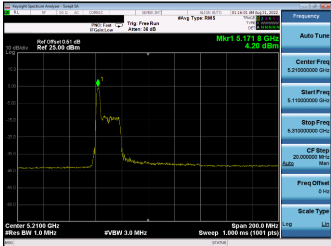
Plot 7-272. PSD SDM Antenna WF4a (80MHz BW 11ax Index 0 - RU26 - Ch.42)
