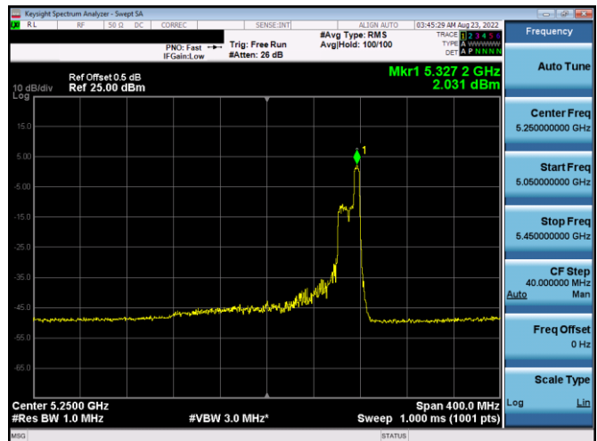
Plot 7-283. PSD CDD Antenna WF5b (20MHz BW 11ax Index 52– RU52 – Ch.50)
