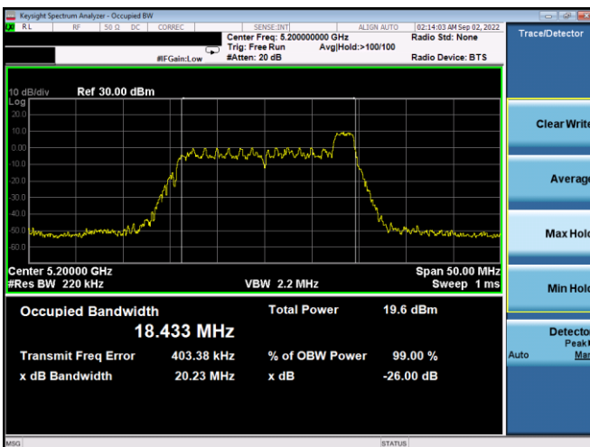
Plot 7-47. 26dB BW & 99% OBW Antenna WF4a (20MHz BW 11ax Index 8 – RU26 – Ch.40)
