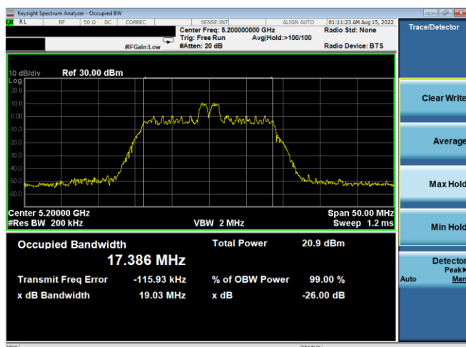
Plot 7-46. 26dB BW & 99% OBW Antenna WF4a (20MHz BW 11ax Index 4 – RU26 – Ch.40)
