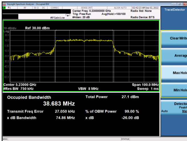
Plot 7-52. 26dB BW & 99% OBW Antenna WF4a (40MHz BW 11ax – RU484 – Ch.46)
