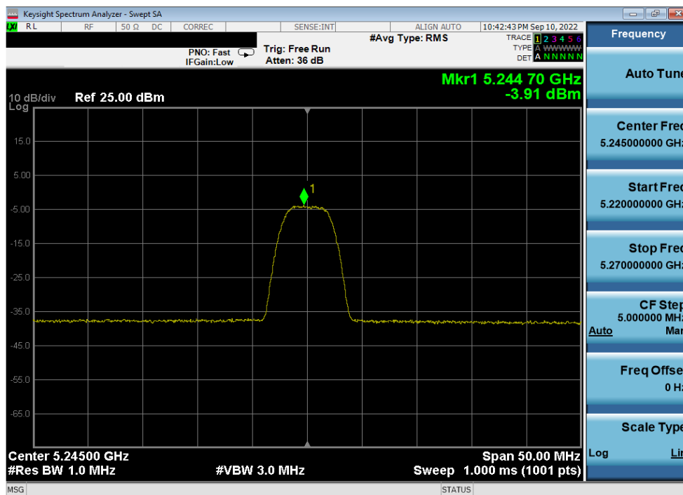
Plot 7-60. PSD Antenna 4a (HDR8, iPA, 5245MHz)
