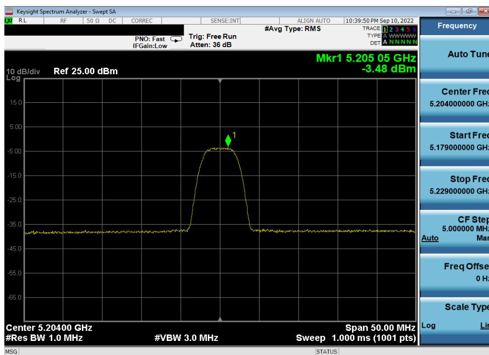
Plot 7-59. PSD Antenna 4a (HDR8, iPA, 5204MHz)
