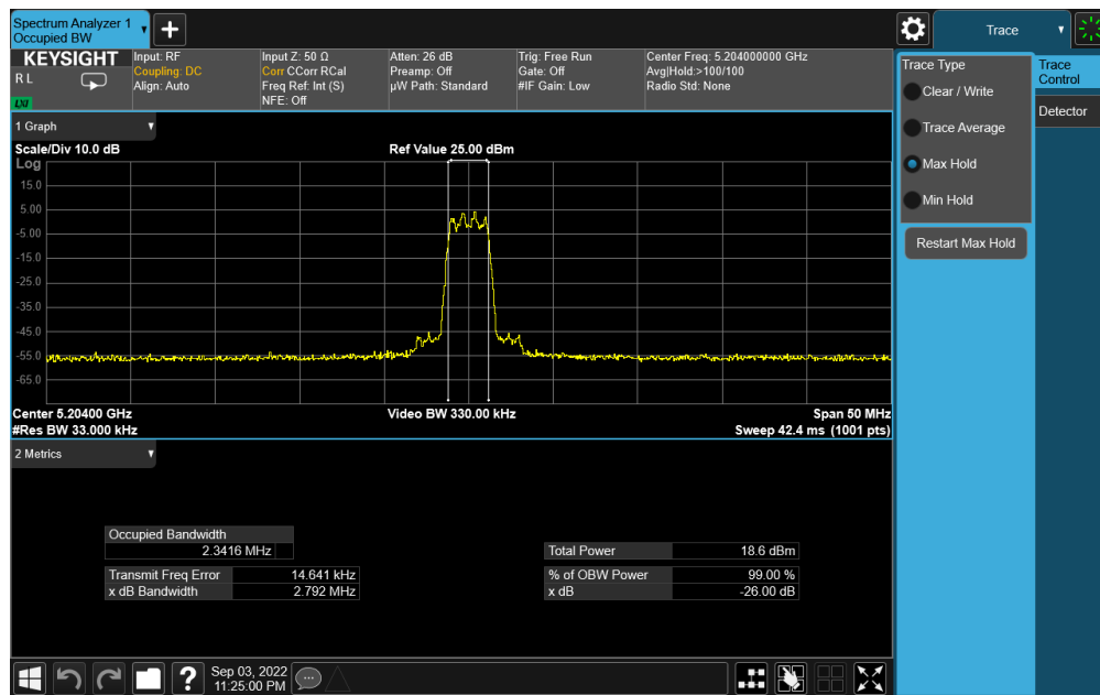
Plot 7-2. 26dB BW & 99% OBW Antenna 5b (HDR4, ePA, 5204MHz)
