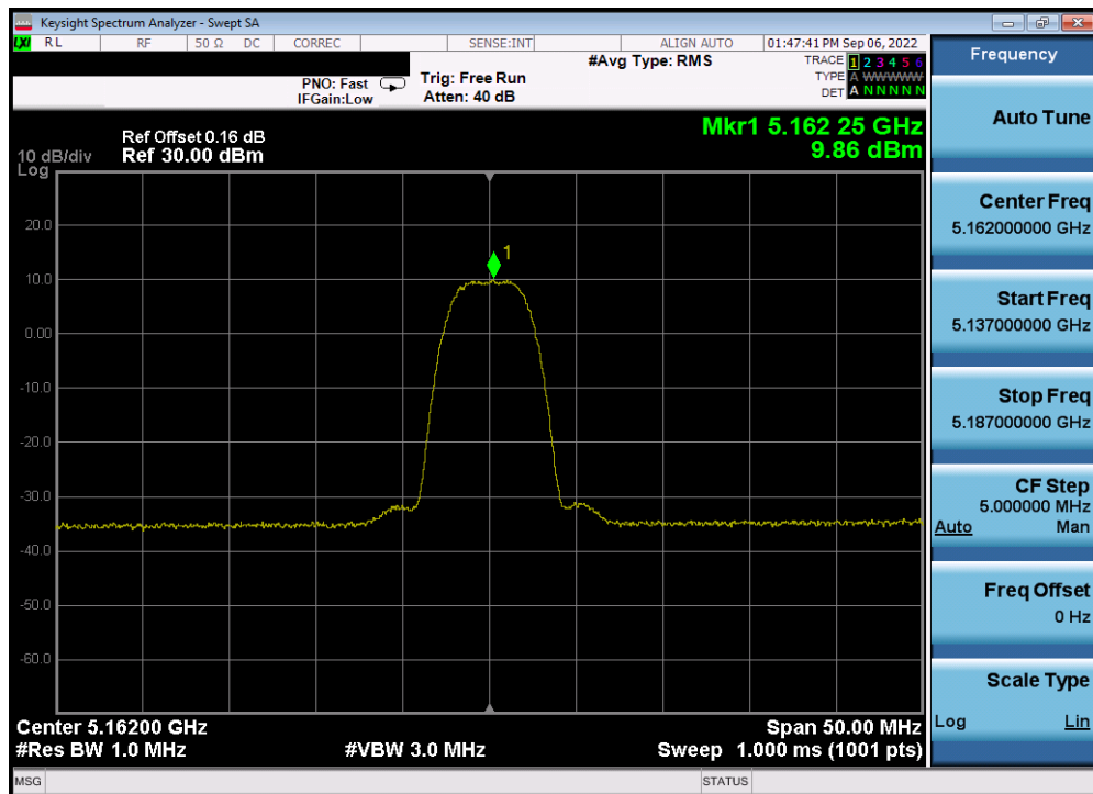
Plot 7-28. PSD Antenna 5b (HDR8, ePA, 5162MHz)
