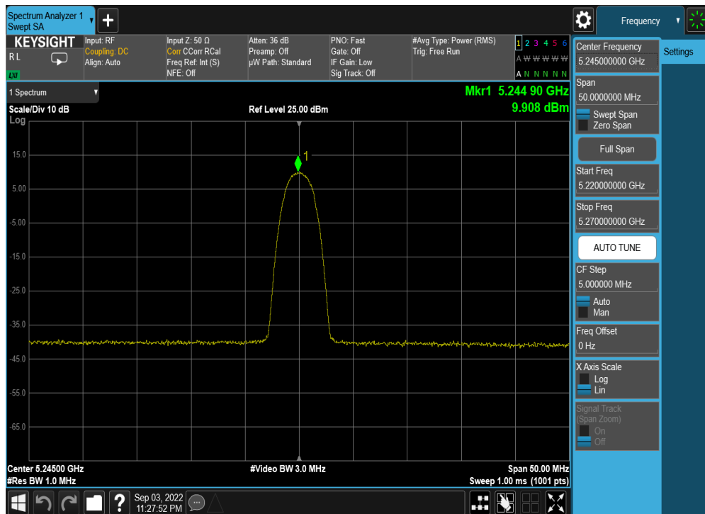
Plot 7-27. PSD Antenna 5b (HDR4, ePA, 5245MHz)
