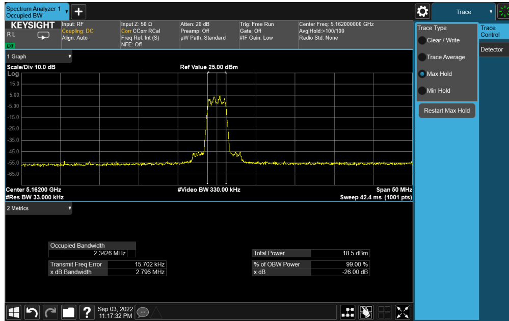
Plot 7-1. 26dB BW & 99% OBW Antenna 5b (HDR4, ePA, 5162MHz)
