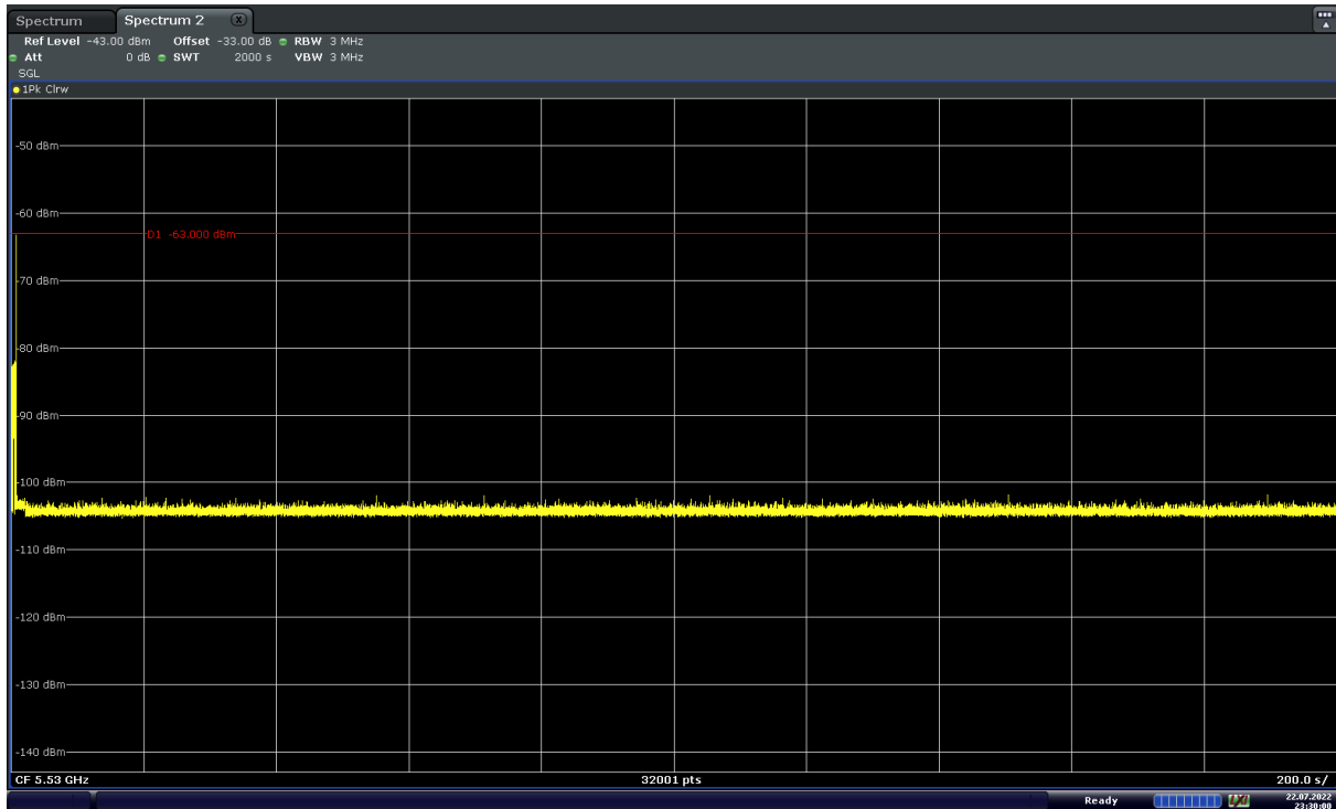
Figure 9-16. 5530MHz - Non-Occupancy Period (30 Minutes) - Mode 1 (80MHz)
