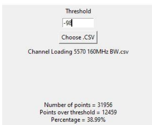
Figure 9-4. 5570MHz - Channel Loading Calculation - Mode 1 (160MHz)
