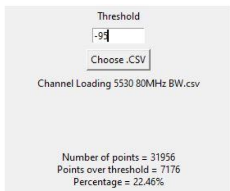
Figure 9-8. 5530MHz - Channel Loading Calculation - Mode 3 (80MHz)
