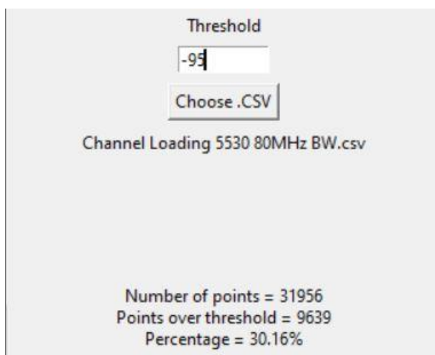
Figure 9-6. 5530MHz - Channel Loading Calculation - Mode 2 (80MHz)
