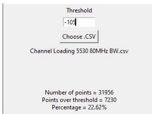
Figure 9-10. 5530MHz - Channel Loading Calculation - Mode 4 (80MHz)
