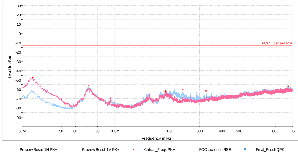
Plot 7-438. Ant M2 - RSE Plot (Band n258-R1-100MHz-1CC SISO Dual Pol – QPSK – Mid Channel)
