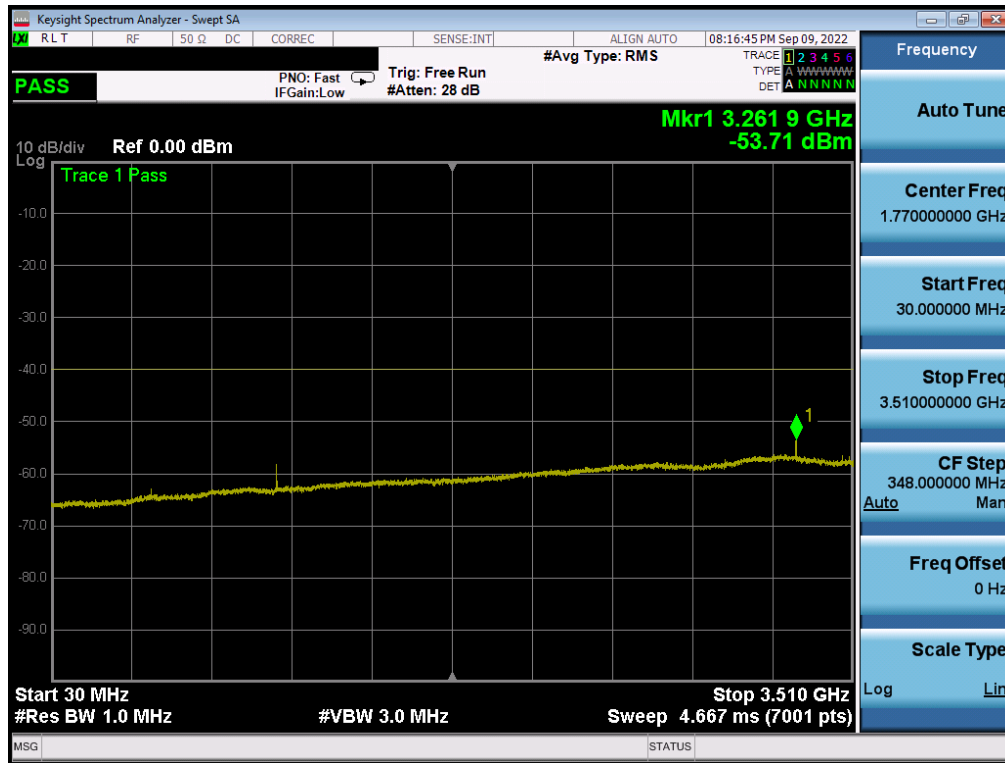
Plot 7-45. Conducted Spurious Plot (ULCA Band 48 - 20+20MHz QPSK - Low Channel)
