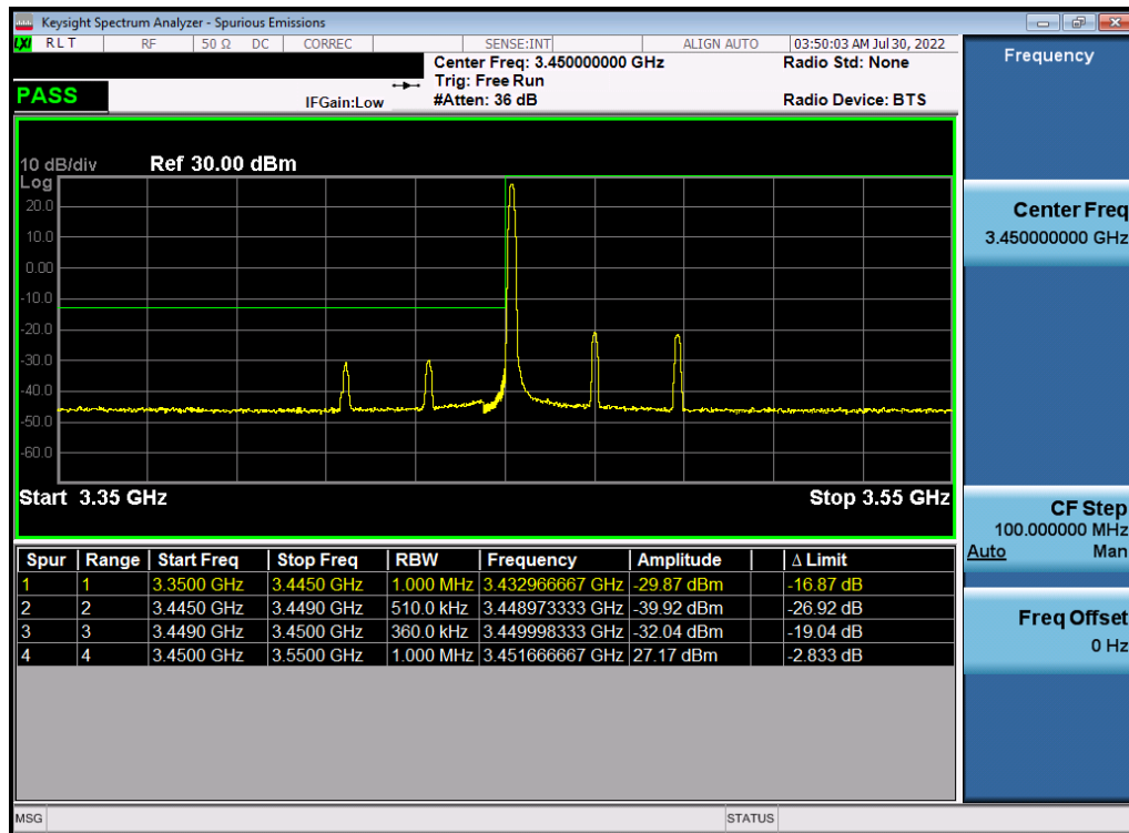
Plot 7-137. Lower ACP Plot (NR Band n77 - 40MHz DFT-s-OFDM \pi/2 BPSK - Full RB)
