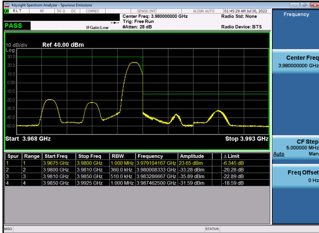
Plot 7-152. Upper ACP Plot (NR Band n77 - 10MHz DFT-s-OFDM \pi/2 BPSK – Full RB)
