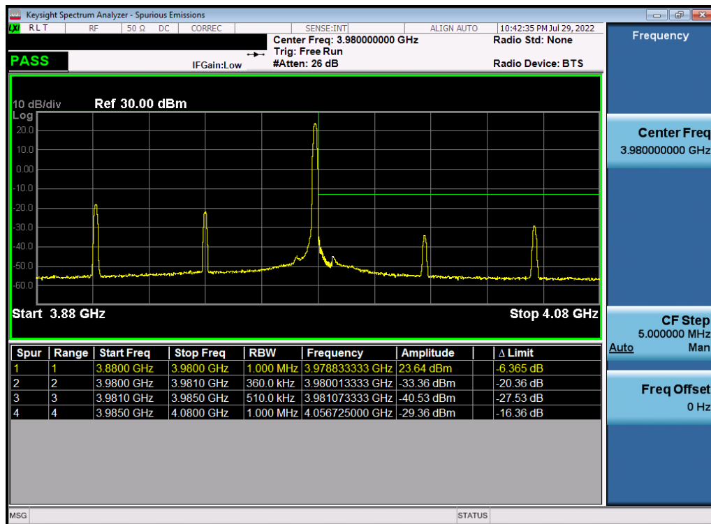
Plot 7-168. Upper ACP Plot (NR Band n77 - 80MHz DFT-s-OFDM \pi/2 BPSK - Full RB)
