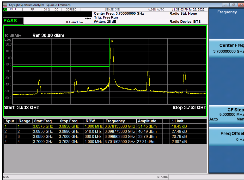
Plot 7-161. Lower ACP Plot (NR Band n77 - 50MHz DFT-s-OFDM \pi/2 BPSK - Full RB)
