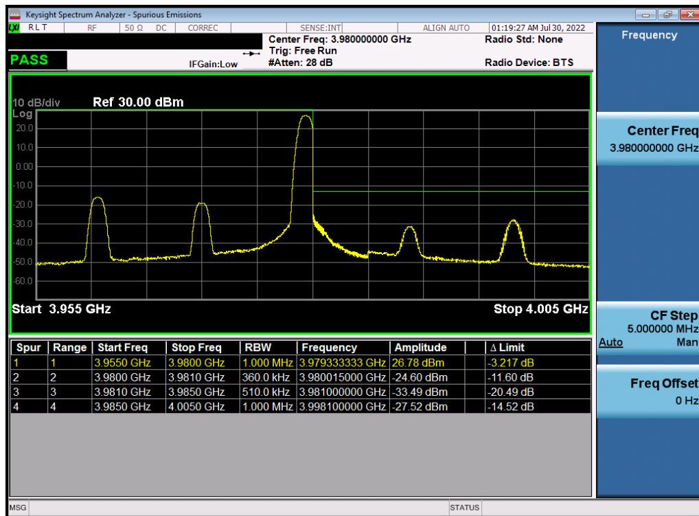
Plot 7-156. Upper ACP Plot (NR Band n77 - 20MHz DFT-s-OFDM \pi/2 BPSK - Full RB)
