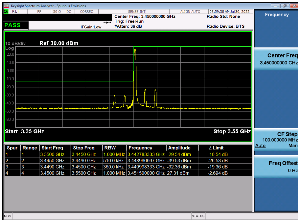
Plot 7-133. Lower ACP Plot (NR Band n77 - 20MHz DFT-s-OFDM \pi/2 BPSK - Full RB)
