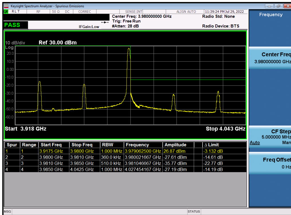
Plot 7-162. Upper ACP Plot (NR Band n77 - 50MHz DFT-s-OFDM \pi/2 BPSK - Full RB)
