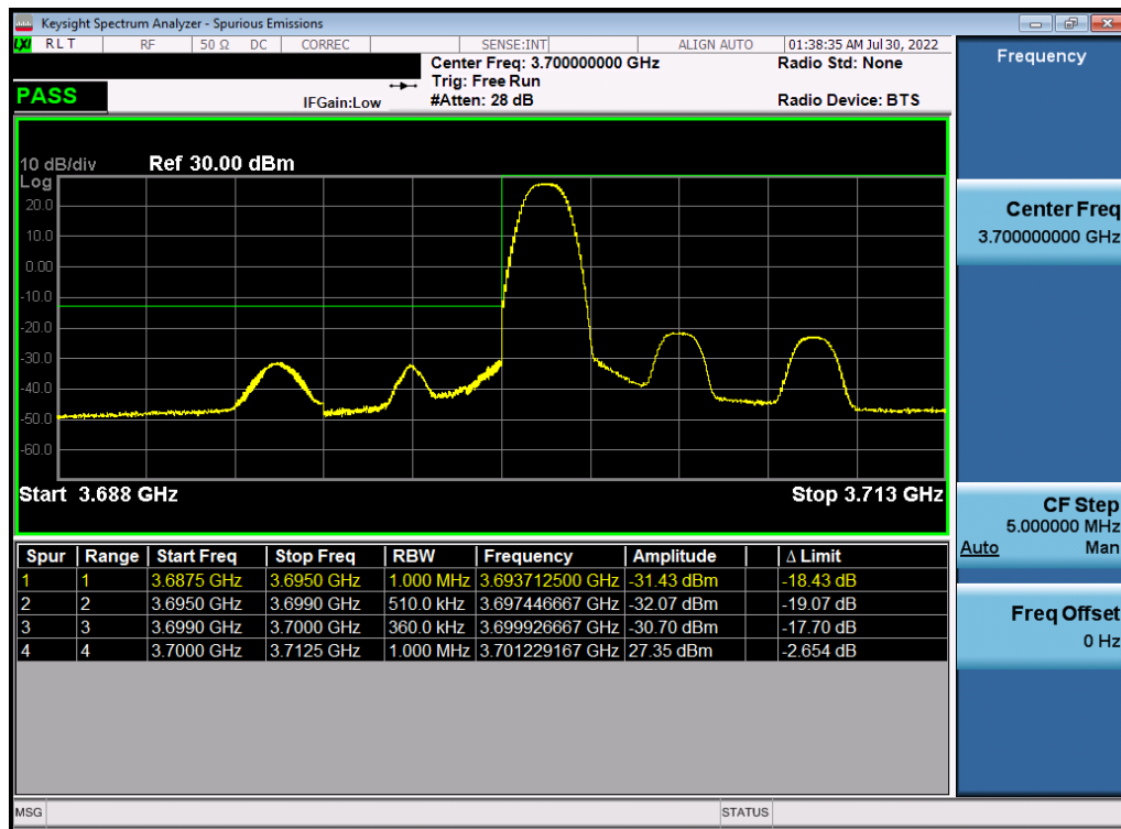
Plot 7-151. Lower ACP Plot (NR Band n77 - 10MHz DFT-s-OFDM \pi/2 BPSK – Full RB)
