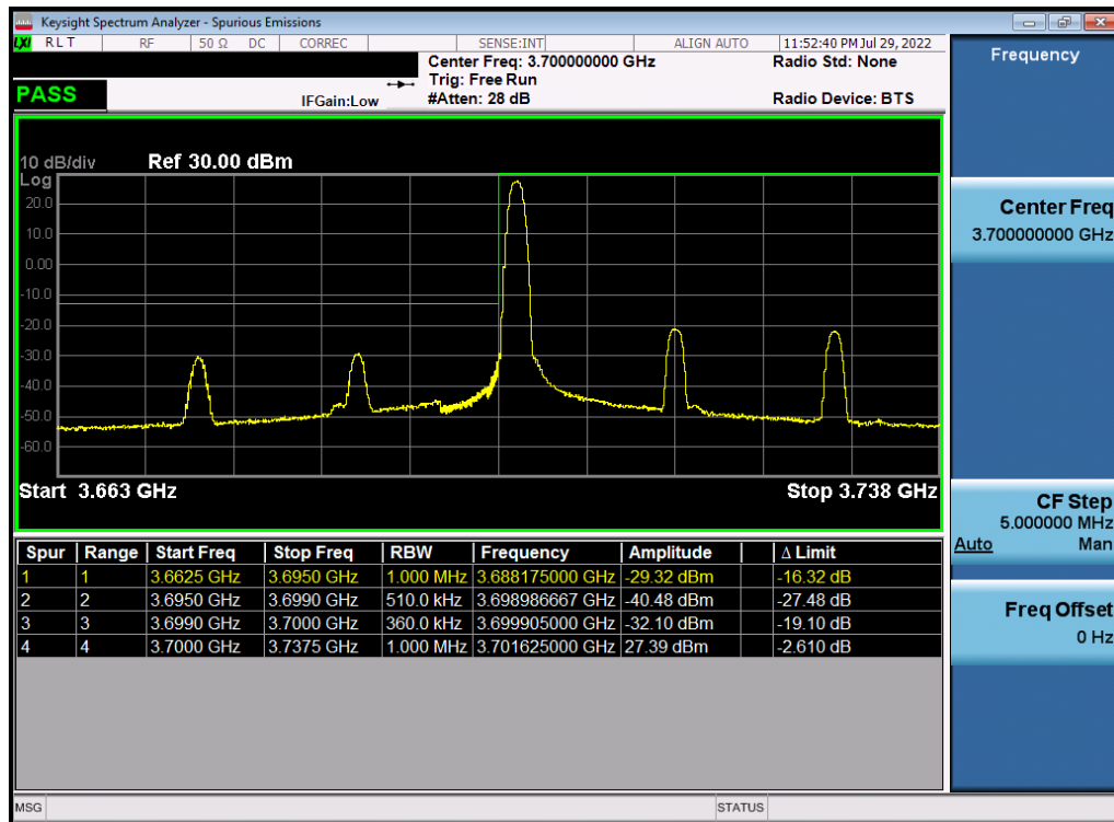
Plot 7-157. Lower ACP Plot (NR Band n77 - 30MHz DFT-s-OFDM \pi/2 BPSK - Full RB)
