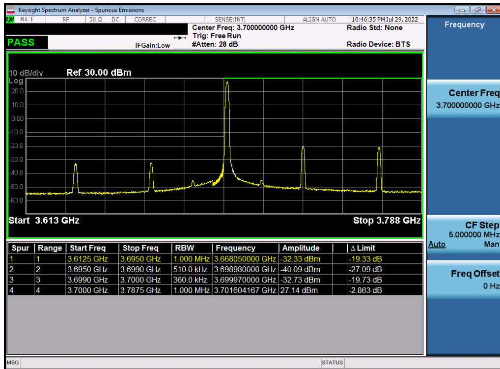
Plot 7-165. Lower ACP Plot (NR Band n77 - 70MHz DFT-s-OFDM \pi/2 BPSK - Full RB)
