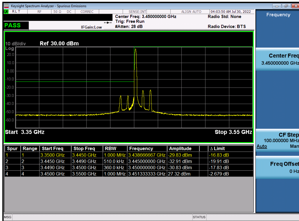
Plot 7-131. Lower ACP Plot (NR Band n77 - 15MHz DFT-s-OFDM \pi/2 BPSK - Full RB)
