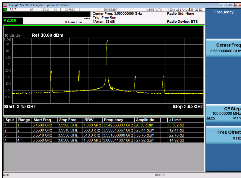
Plot 7-142. Upper ACP Plot (NR Band n77 - 60MHz DFT-s-OFDM \pi/2 BPSK - Full RB)
