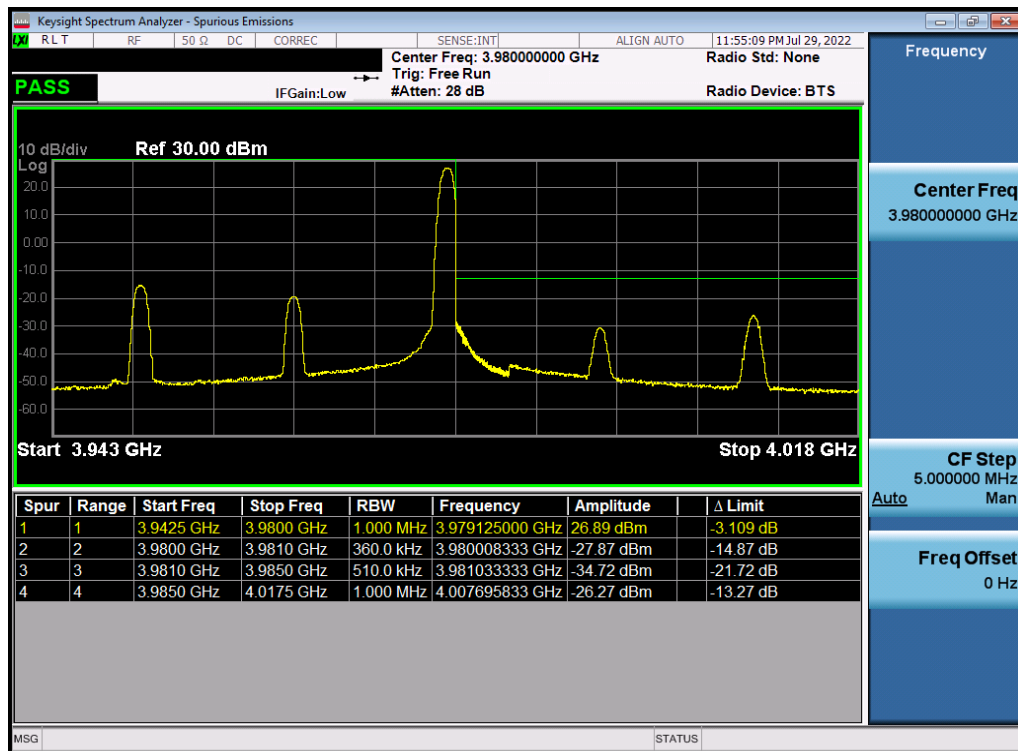
Plot 7-158. Upper ACP Plot (NR Band n77 - 30MHz DFT-s-OFDM \pi/2 BPSK - Full RB)
