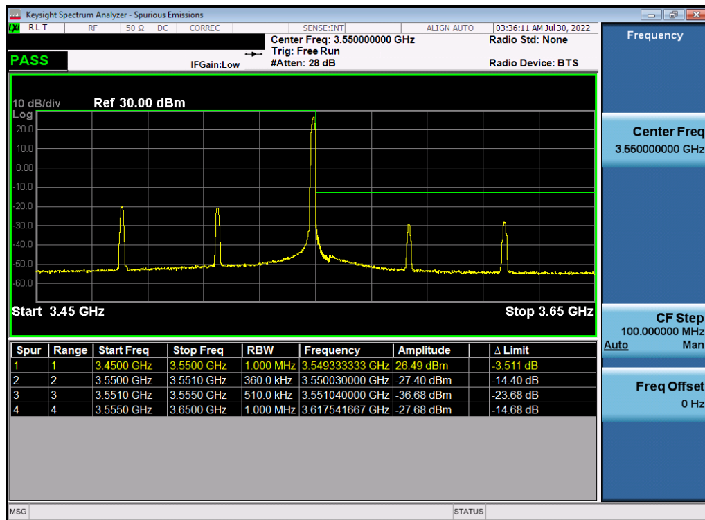
Plot 7-144. Upper ACP Plot (NR Band n77 - 70MHz DFT-s-OFDM \pi/2 BPSK - Full RB)
