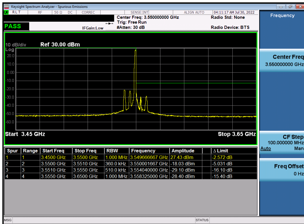
Plot 7-130. Upper ACP Plot (NR Band n77 - 10MHz DFT-s-OFDM \pi/2 BPSK – Full RB)
