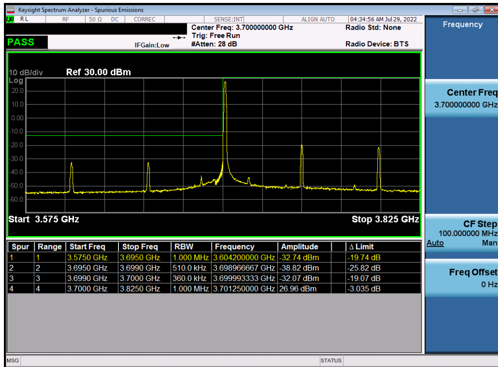
Plot 7-171. Lower ACP Plot (NR Band n77 - 100MHz DFT-s-OFDM \pi/2 BPSK - Full RB)
