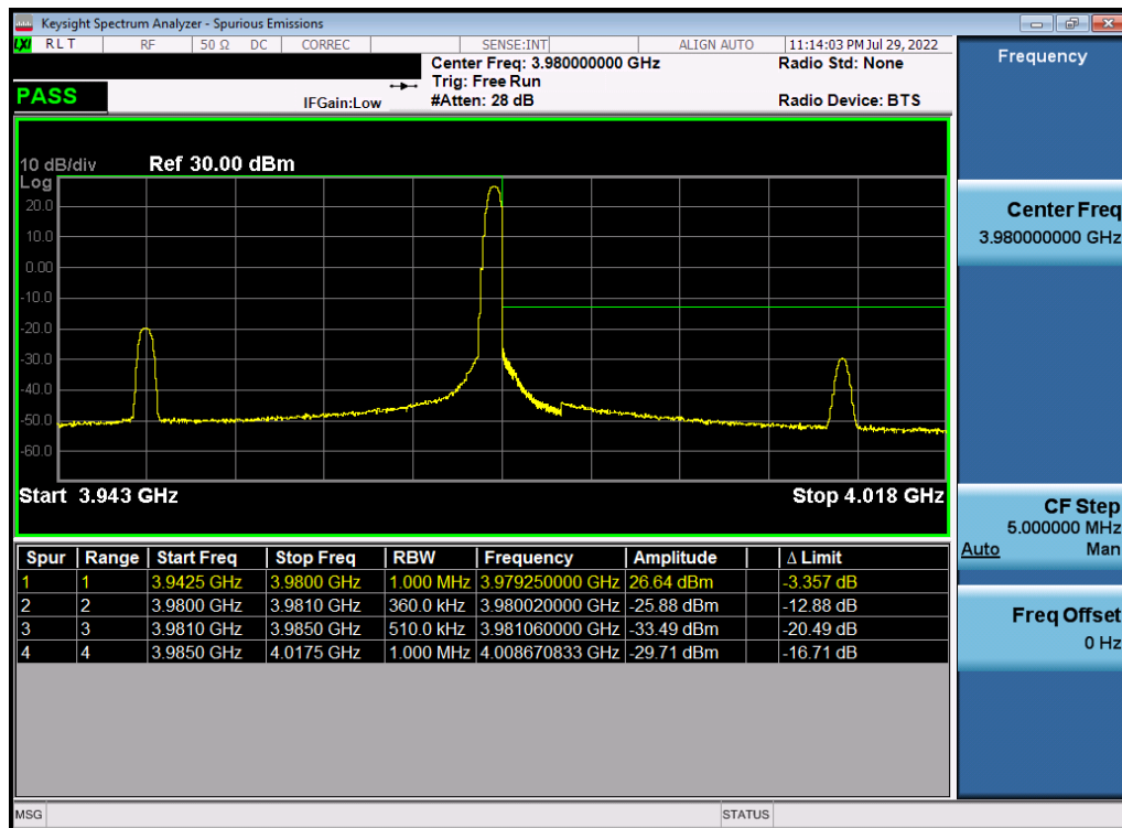
Plot 7-164. Upper ACP Plot (NR Band n77 - 60MHz DFT-s-OFDM \pi/2 BPSK - Full RB)
