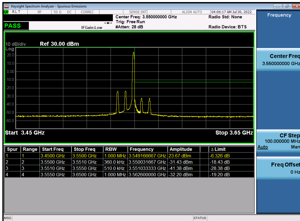
Plot 7-132. Upper ACP Plot (NR Band n77 - 15MHz DFT-s-OFDM \pi/2 BPSK - Full RB)
