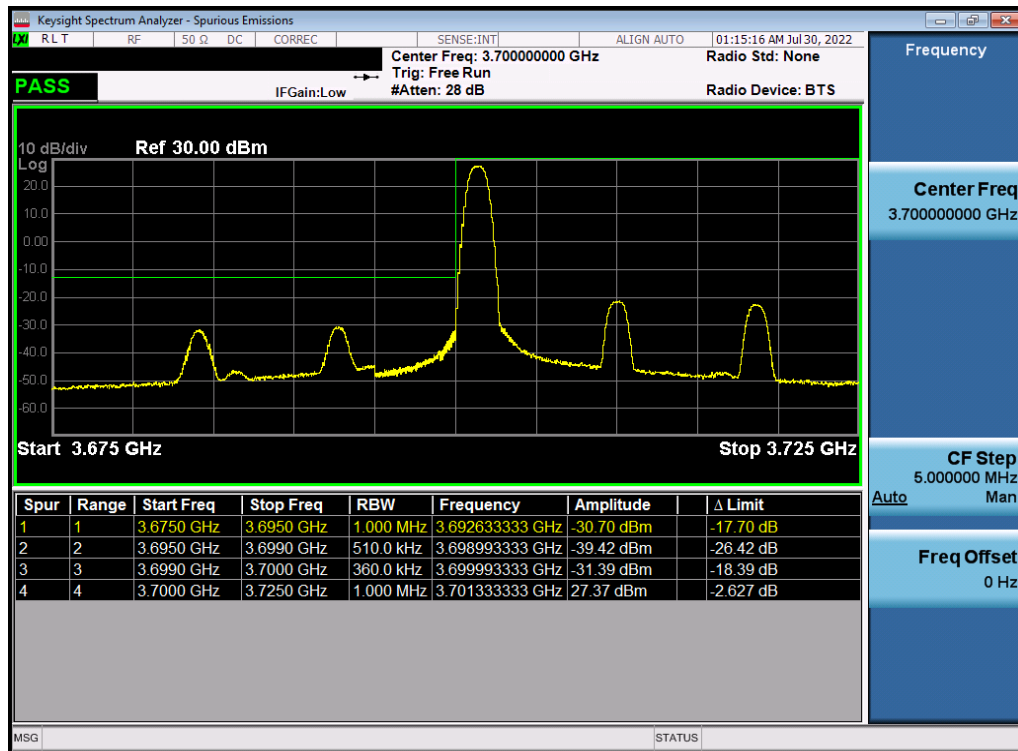
Plot 7-155. Lower ACP Plot (NR Band n77 - 20MHz DFT-s-OFDM \pi/2 BPSK - Full RB)
