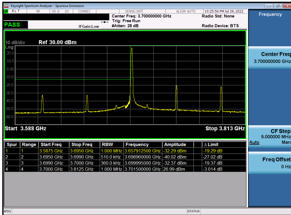
Plot 7-169. Lower ACP Plot (NR Band n77 - 90MHz DFT-s-OFDM \pi/2 BPSK - Full RB)
