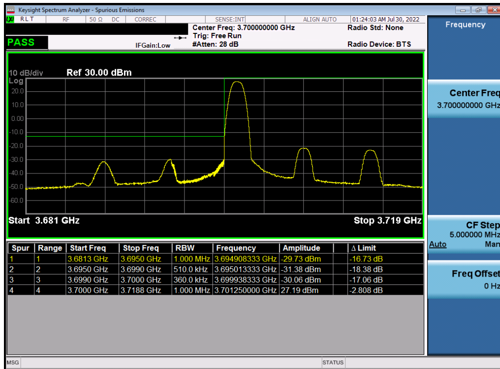
Plot 7-153. Lower ACP Plot (NR Band n77 - 15MHz DFT-s-OFDM \pi/2 BPSK - Full RB)
