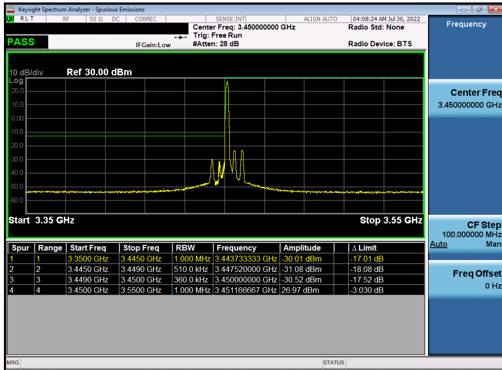
Plot 7-129. Lower ACP Plot (NR Band n77 - 10MHz DFT-s-OFDM \pi/2 BPSK – Full RB)
