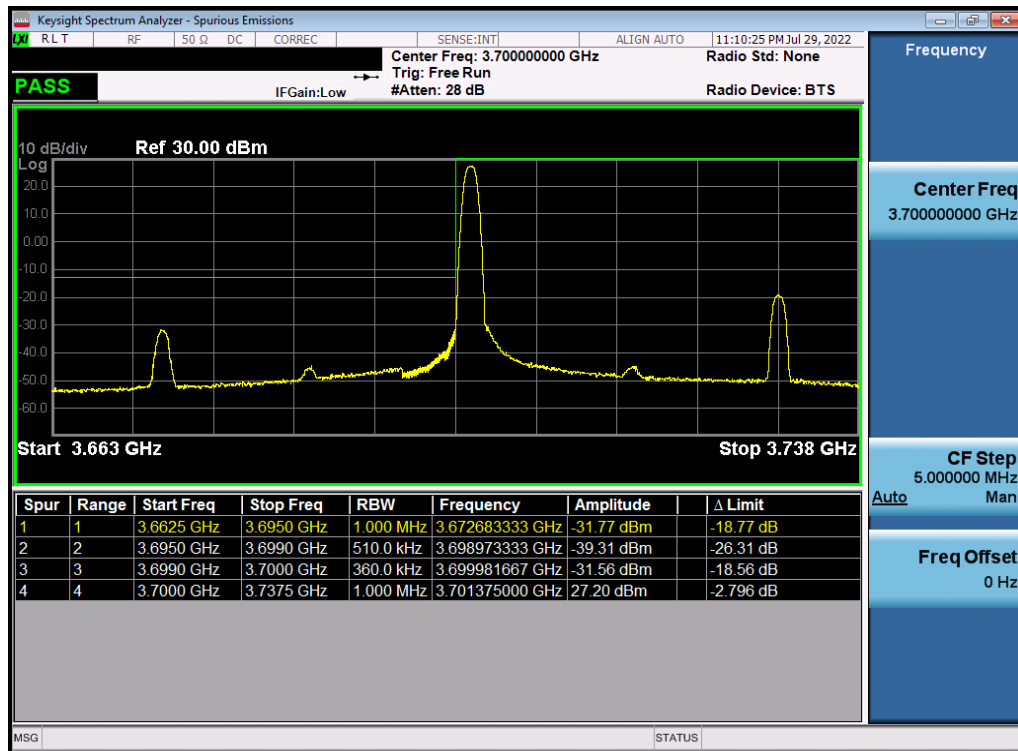
Plot 7-163. Lower ACP Plot (NR Band n77 - 60MHz DFT-s-OFDM \pi/2 BPSK - Full RB)
