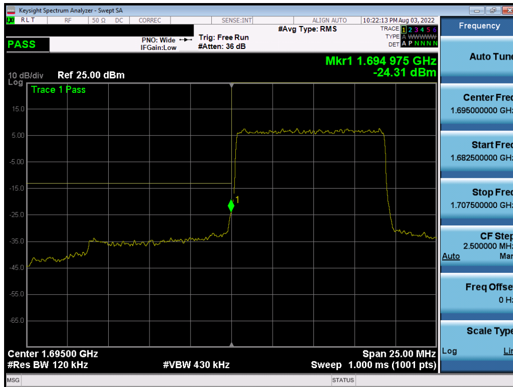
Plot 7-325. Lower Band Edge Plot (NR Band n70 – 10.0MHz DFT-s-OFDM \pi/2 BPSK - Full RB)
