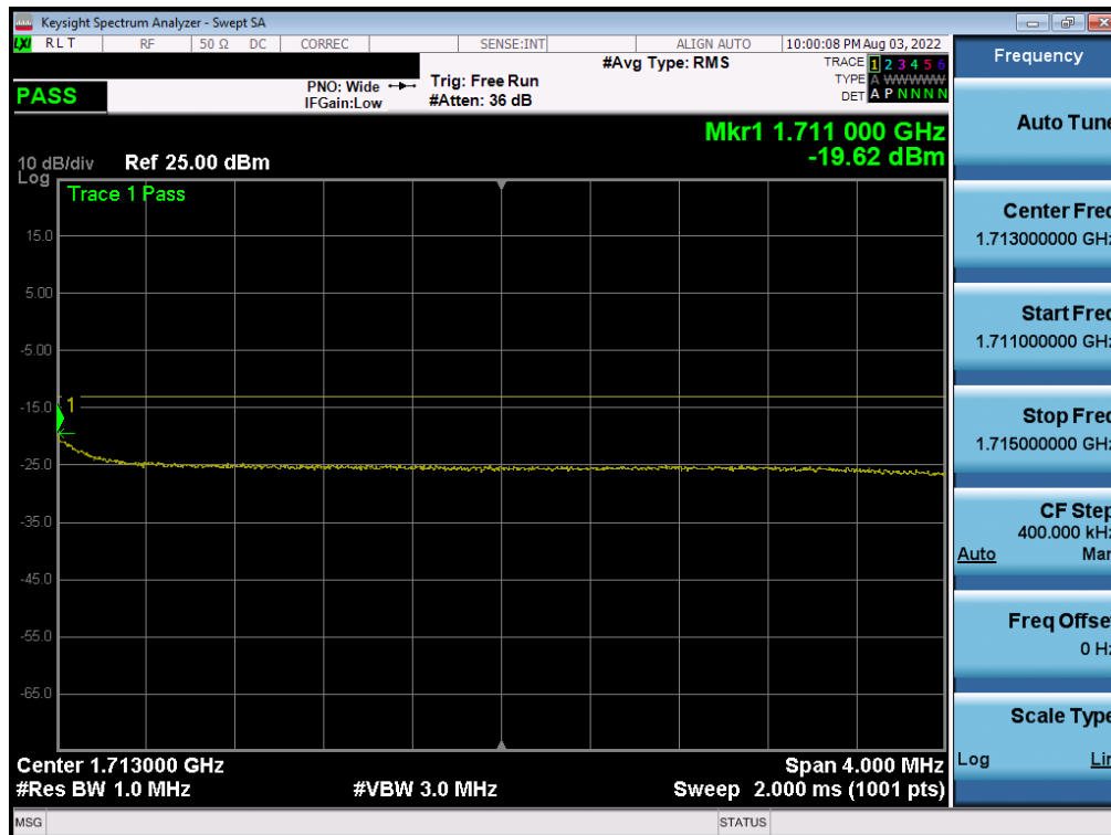
Plot 7-332. Upper Extended Band Edge Plot (NR Band n70 – 15.0MHz DFT-s-OFDM \pi/2 BPSK - Full RB)
