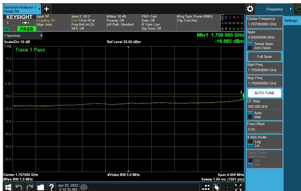
Plot 7-306. Lower Extended Band Edge Plot (NR Band n66 – 15.0MHz DFT-s-OFDM \pi/2 BPSK - Full RB)
