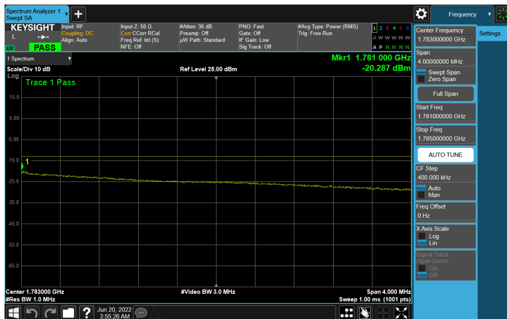
Plot 7-312. Upper Extended Band Edge Plot (NR Band n66 – 20.0MHz DFT-s-OFDM \pi/2 BPSK - Full RB)
