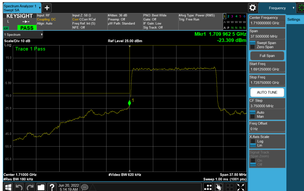
Plot 7-305. Lower Band Edge Plot (NR Band n66 – 15.0MHz DFT-s-OFDM \pi/2 BPSK - Full RB)
