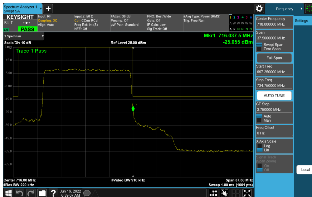
Plot 7-346. Upper Band Edge Plot (NR Band n12 – 15.0MHz DFT-s-OFDM \pi/2 BPSK - Full RB)
