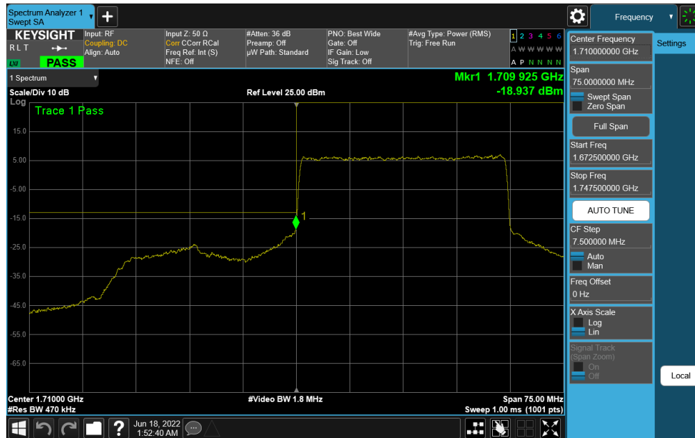
Plot 7-313. Lower Band Edge Plot (NR Band n66 – 30.0MHz DFT-s-OFDM \pi/2 BPSK - Full RB)
