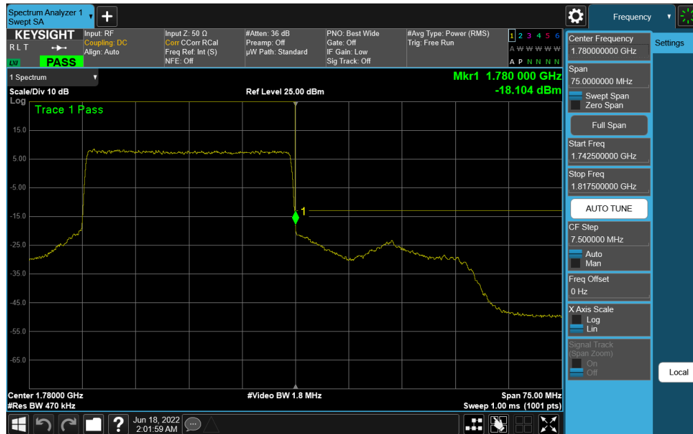
Plot 7-315. Upper Band Edge Plot (NR Band n66 – 30.0MHz DFT-s-OFDM \pi/2 BPSK - Full RB)
