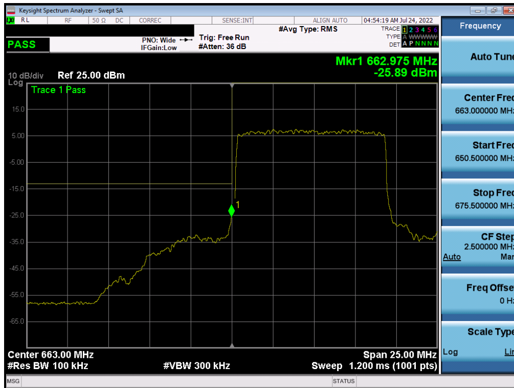
Plot 7-335. Lower Band Edge Plot (NR Band n71 – 10.0MHz DFT-s-OFDM \pi/2 BPSK - Full RB)
