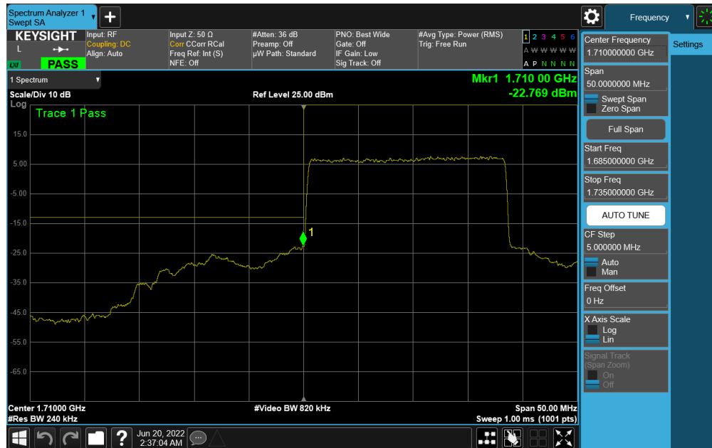
Plot 7-309. Lower Band Edge Plot (NR Band n66 – 20.0MHz DFT-s-OFDM \pi/2 BPSK - Full RB)
