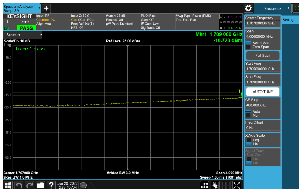
Plot 7-310. Lower Extended Band Edge Plot (NR Band n66 – 20.0MHz DFT-s-OFDM \pi/2 BPSK - Full RB)
