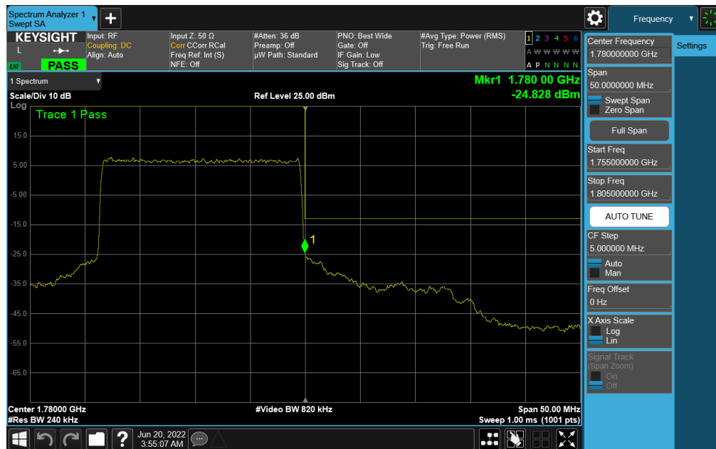
Plot 7-311. Upper Band Edge Plot (NR Band n66 – 20.0MHz DFT-s-OFDM \pi/2 BPSK - Full RB)
