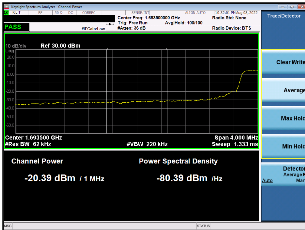
Plot 7-322. Lower Extended Band Edge Plot (NR Band n70 – 5.0MHz CP--OFDM \pi/2 BPSK - Full RB)
