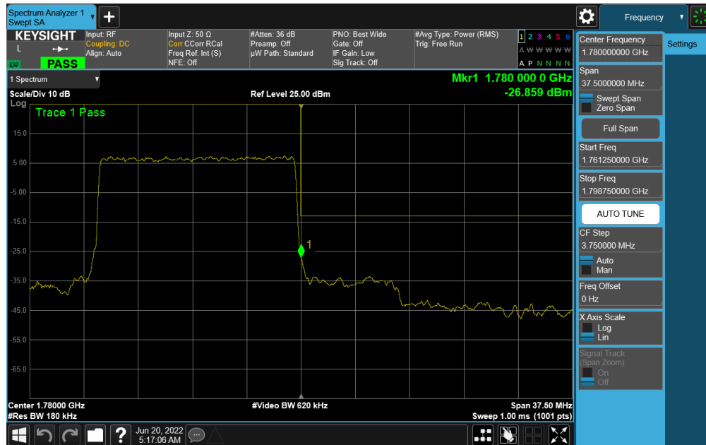
Plot 7-307. Upper Band Edge Plot (NR Band n66 – 15.0MHz DFT-s-OFDM \pi/2 BPSK - Full RB)
