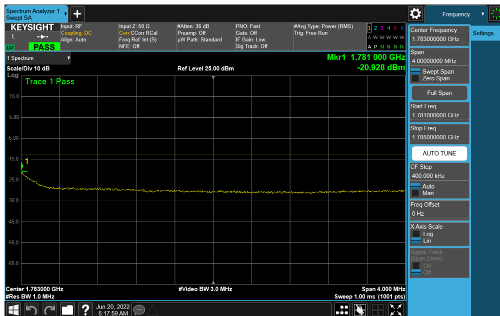
Plot 7-308. Upper Extended Band Edge Plot (NR Band n66 – 15.0MHz DFT-s-OFDM \pi/2 BPSK - Full RB)
