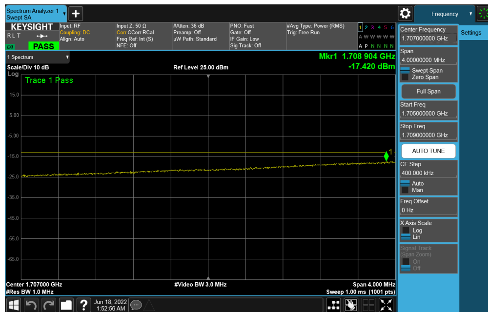
Plot 7-314. Lower Extended Band Edge Plot (NR Band n66 – 30.0MHz DFT-s-OFDM \pi/2 BPSK - Full RB)
