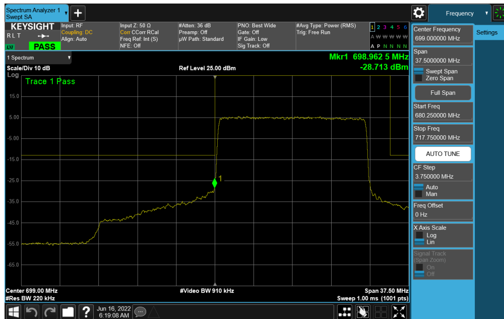
Plot 7-345. Lower Band Edge Plot (NR Band n12 – 15.0MHz DFT-s-OFDM \pi/2 BPSK - Full RB)
