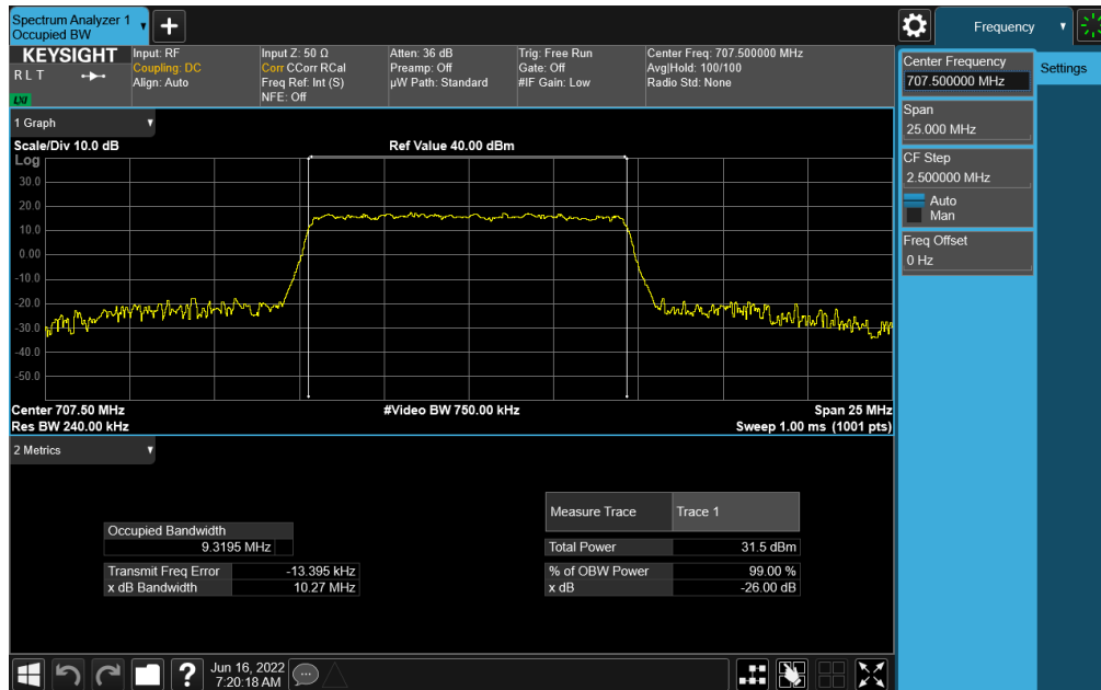
Plot 7-136. Occupied Bandwidth Plot (NR Band n12 - 10MHz CP-OFDM QPSK - Full RB)
