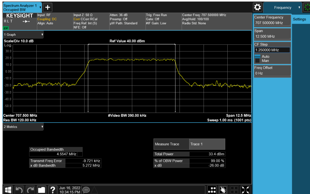
Plot 7-131. Occupied Bandwidth Plot (NR Band n12 - 5MHz DFT-s-OFDM QPSK - Full RB)
