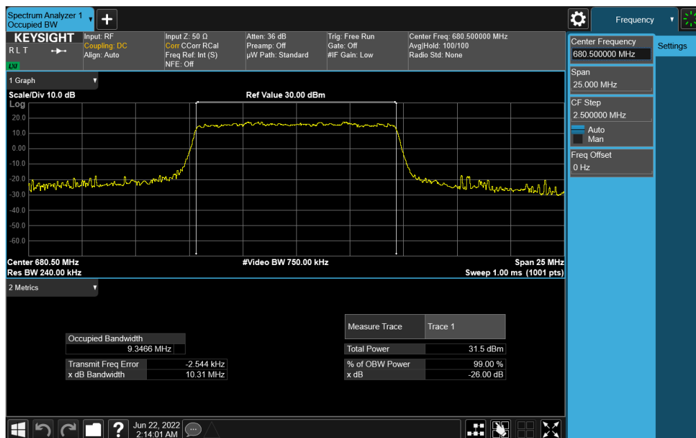
Plot 7-117. Occupied Bandwidth Plot (NR Band n71 - 10MHz CP-OFDM 16-QAM - Full RB)
