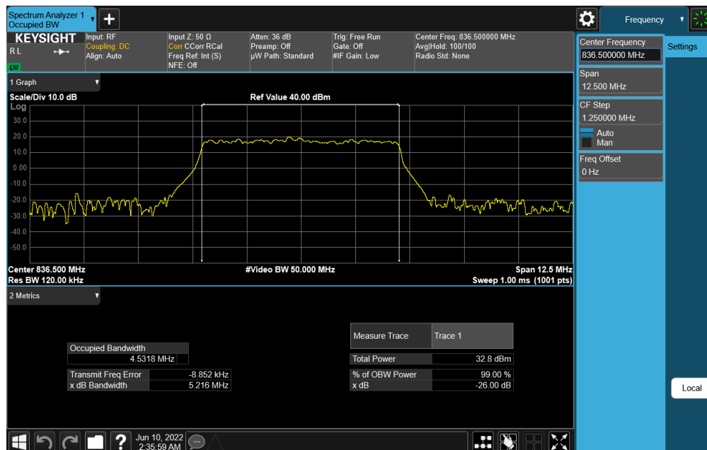
Plot 7-18. Occupied Bandwidth Plot (NR Band n26/n5 - 5MHz DFT-s-OFDM QPSK - Full RB Configuration)
