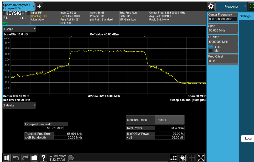
Plot 7-33. Occupied Bandwidth Plot (NR Band n5 - 20MHz CP-OFDM QPSK - Full RB Configuration)
