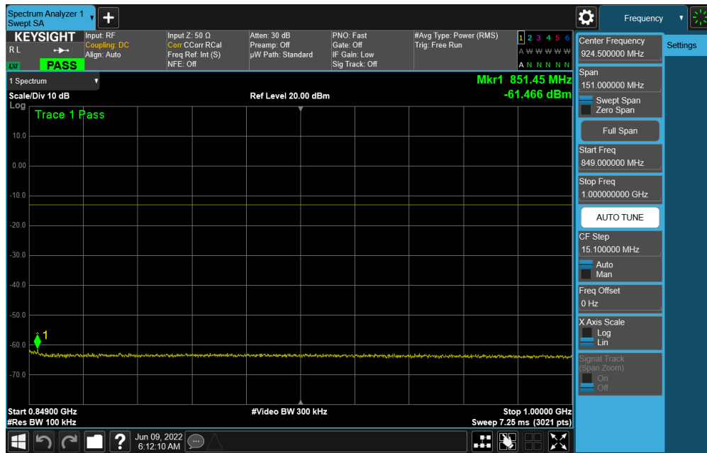
Plot 7-61. CSE (NR Band n5 - 20.0MHz DFT-s-OFDM QPSK - RB Size 1, RB Offset 0 - Mid Channel)
