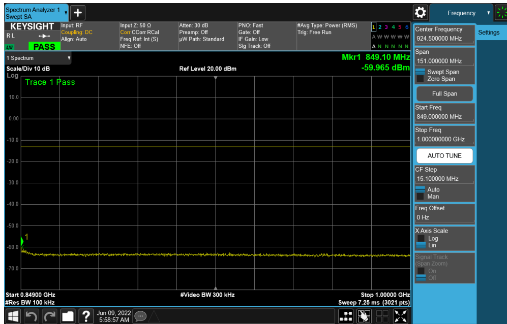
Plot 7-64. CSE (NR Band n5 - 20.0MHz DFT-s-OFDM QPSK - RB Size 1, RB Offset 0 - High Channel)
