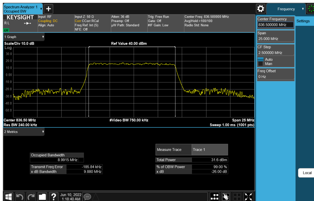
Plot 7-26. Occupied Bandwidth Plot (NR Band n26/n5 - 10MHz DFT-s-OFDM 256-QAM - Full RB Configuration)
