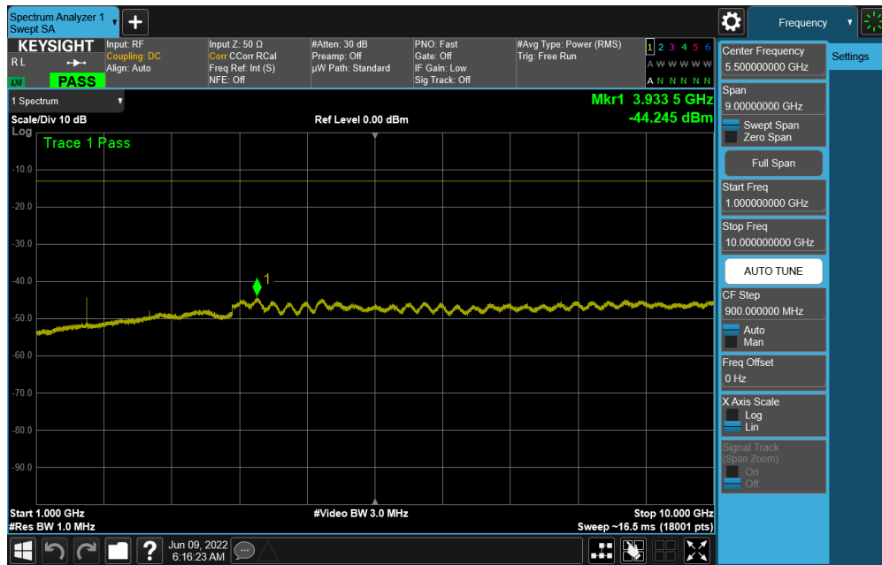
Plot 7-59. CSE (NR Band n5 - 20.0MHz DFT-s-OFDM QPSK - RB Size 1, RB Offset 0 - Low Channel)
