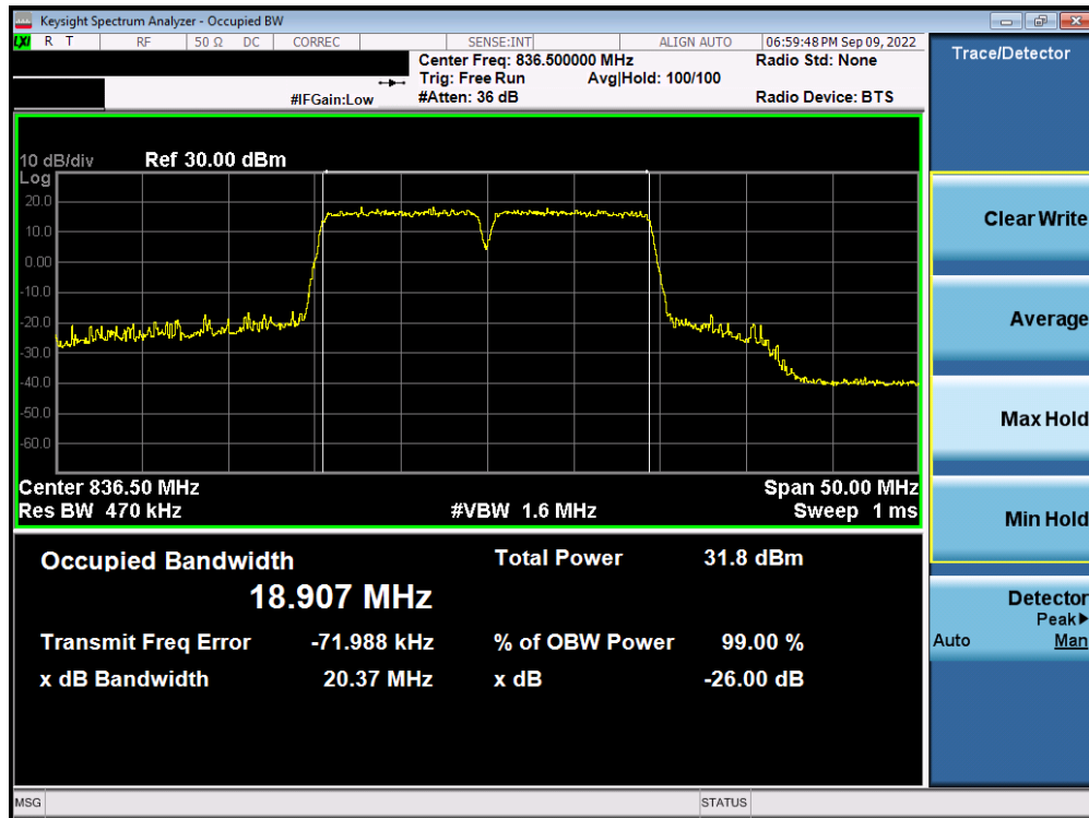
Plot 7-39. Occupied Bandwidth Plot (ULCA LTE Band – (10 + 10)MHz 64-QAM - Full RB Configuration)
