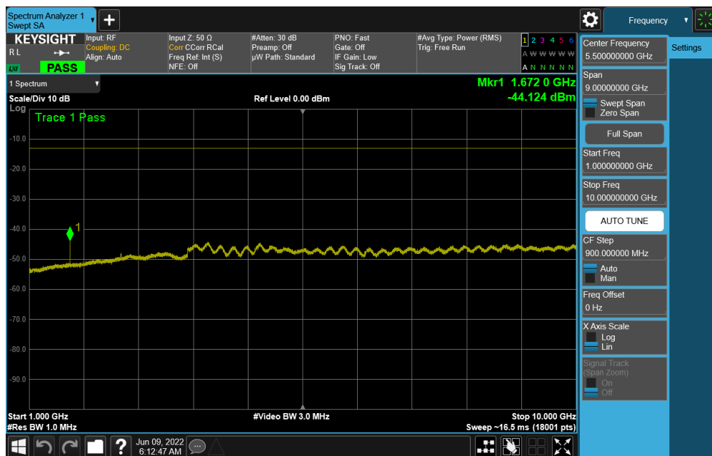
Plot 7-62. CSE (NR Band n5 - 20.0MHz DFT-s-OFDM QPSK - RB Size 1, RB Offset 0 - Mid Channel)
