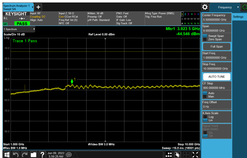
Plot 7-65. CSE (NR Band n5 - 20.0MHz DFT-s-OFDM QPSK - RB Size 1, RB Offset 0 - High Channel)
