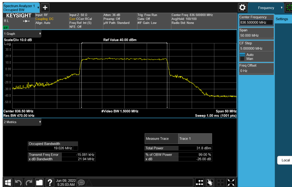
Plot 7-34. Occupied Bandwidth Plot (NR Band n5 - 20MHz CP-OFDM 16-QAM - Full RB Configuration)
