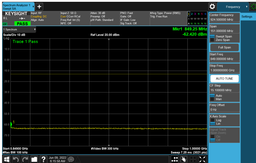
Plot 7-58. CSE (NR Band n5 - 20.0MHz DFT-s-OFDM QPSK - RB Size 1, RB Offset 0 - Low Channel)
