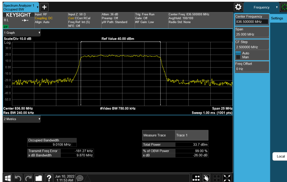
Plot 7-23. Occupied Bandwidth Plot (NR Band n26/n5 - 10MHz DFT-s-OFDM QPSK - Full RB Configuration)
