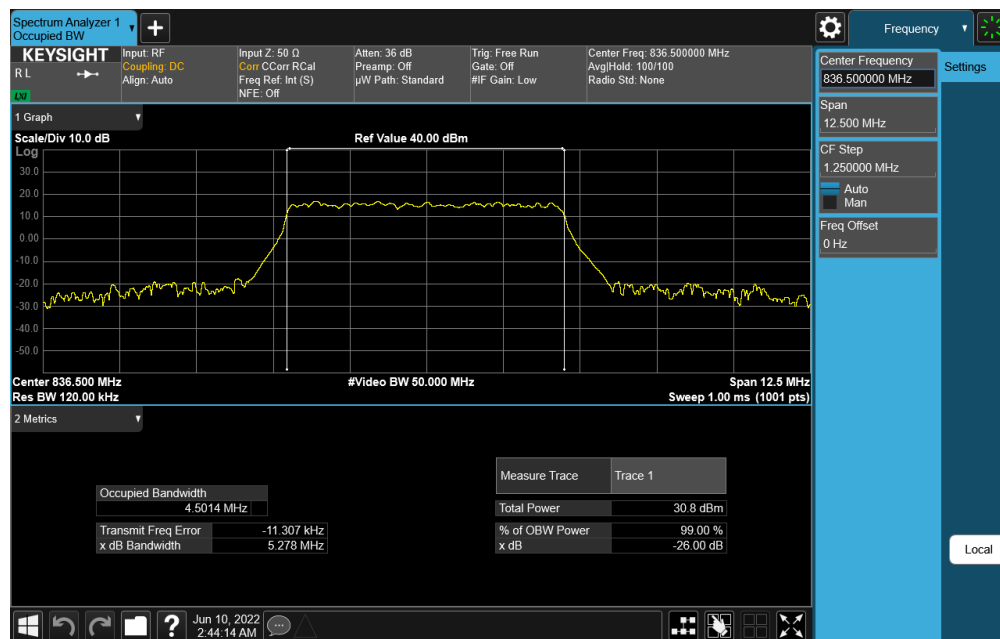
Plot 7-20. Occupied Bandwidth Plot (NR Band n26/n5 - 5MHz CP-OFDM 64-QAM - Full RB Configuration)
