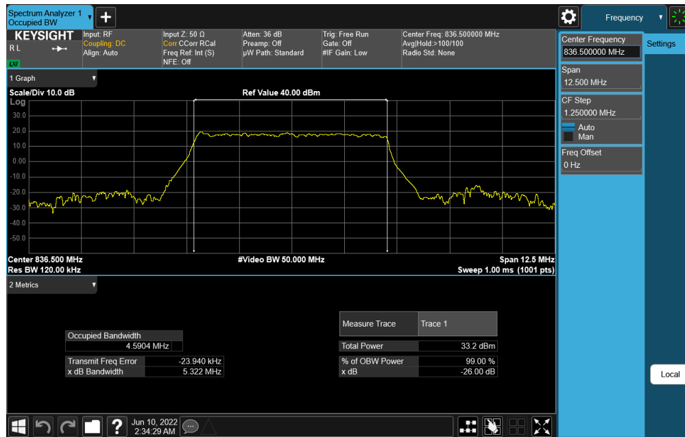
Plot 7-17. Occupied Bandwidth Plot (NR Band n26/n5 - 5MHz DFT-s-OFDM \pi/2 BPSK - Full RB Configuration)
