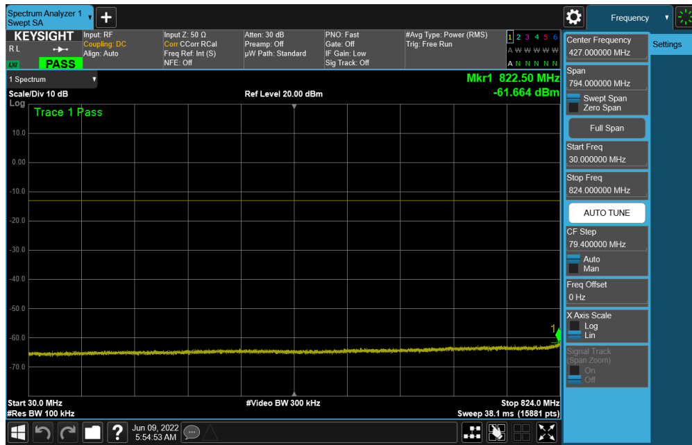
Plot 7-63. CSE (NR Band n5 - 20.0MHz DFT-s-OFDM QPSK - RB Size 1, RB Offset 0 - High Channel)
