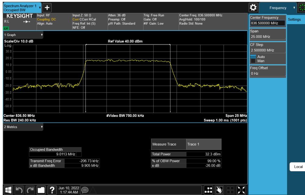
Plot 7-25. Occupied Bandwidth Plot (NR Band n26/n5 - 10MHz DFT-s-OFDM 64-QAM - Full RB Configuration)
