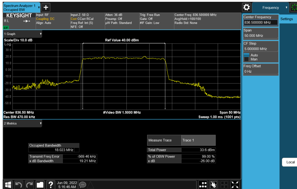
Plot 7-32. Occupied Bandwidth Plot (NR Band n5 - 20MHz DFT-s-OFDM \pi/2 BPSK - Full RB Configuration)
