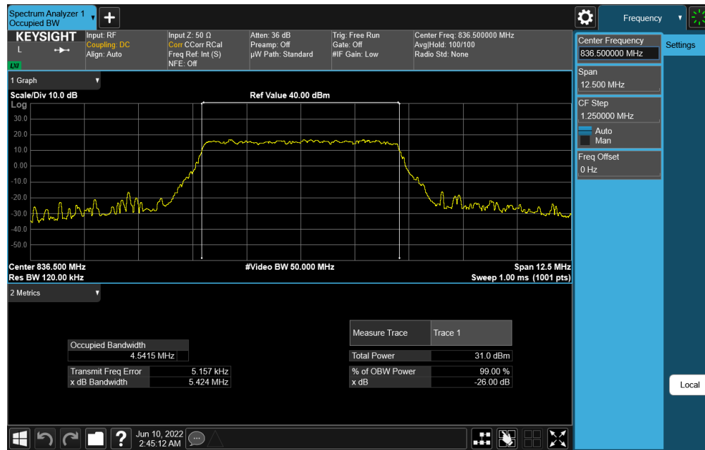
Plot 7-19. Occupied Bandwidth Plot (NR Band n26/n5 - 5MHz CP-OFDM 16-QAM - Full RB Configuration)
