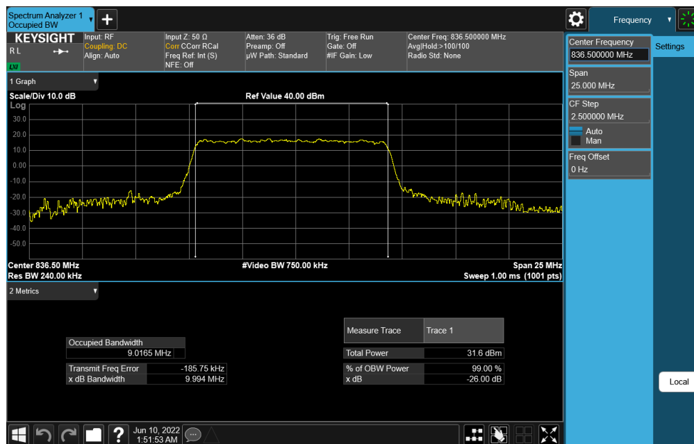
Plot 7-24. Occupied Bandwidth Plot (NR Band n26/n5 - 10MHz CP-OFDM 16-QAM - Full RB Configuration)
