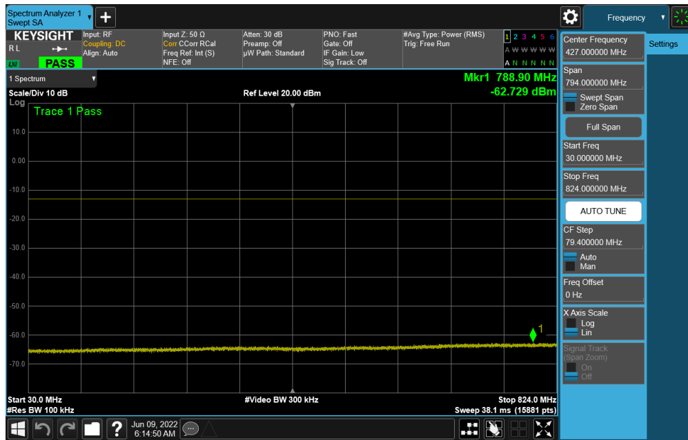
Plot 7-57. CSE (NR Band n5 - 20.0MHz DFT-s-OFDM QPSK - RB Size 1, RB Offset 0 - Low Channel)
