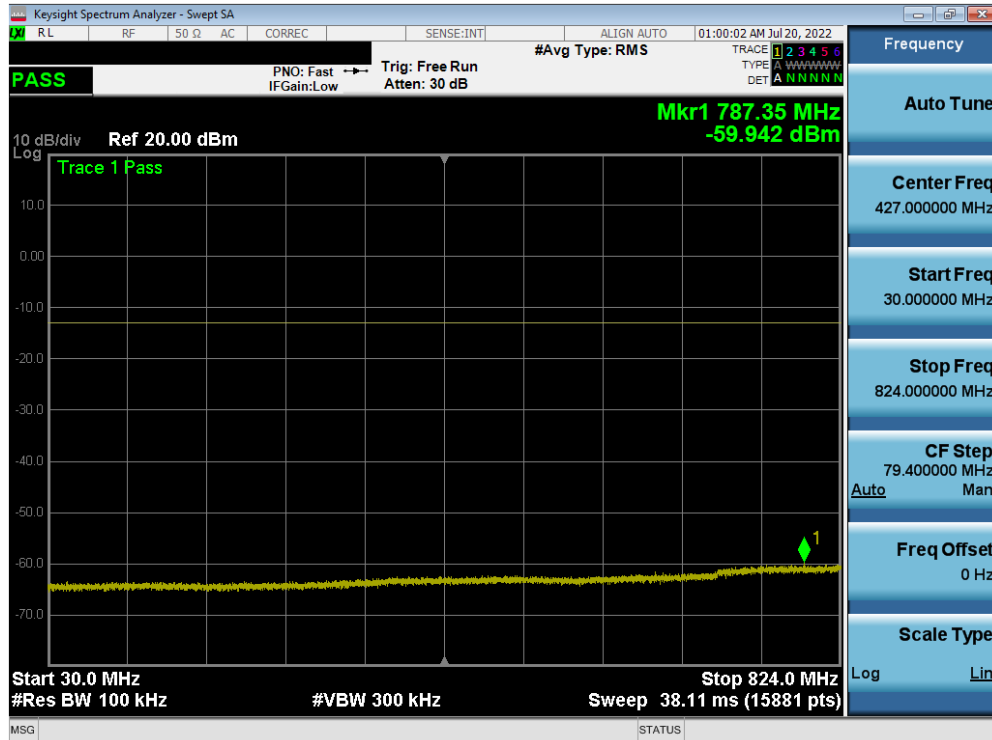
Plot 7-48. CSE (LTE Band 26/5 - 10MHz QPSK - RB Size 1, RB Offset 0 - High Channel)
