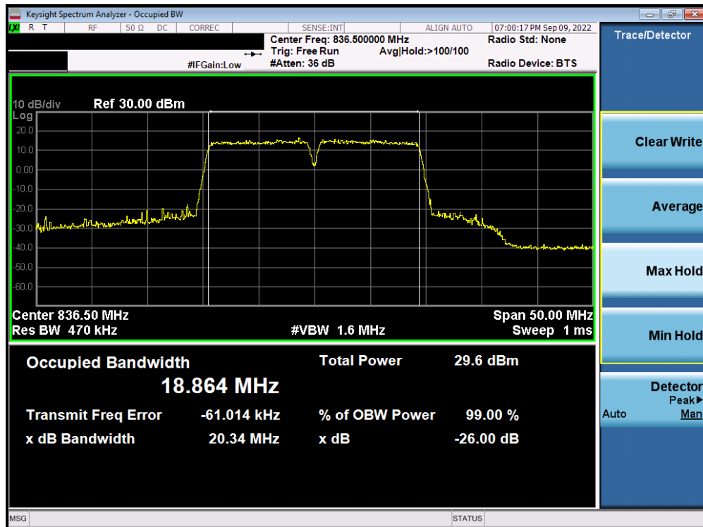
Plot 7-40. Occupied Bandwidth Plot (ULCA LTE Band – (10 + 10)MHz 256-QAM - Full RB Configuration)
