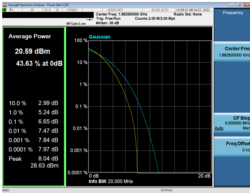
Plot 7-207. PAR Plot (LTE Band 25 - 20MHz 256-QAM - Full RB Configuration)
