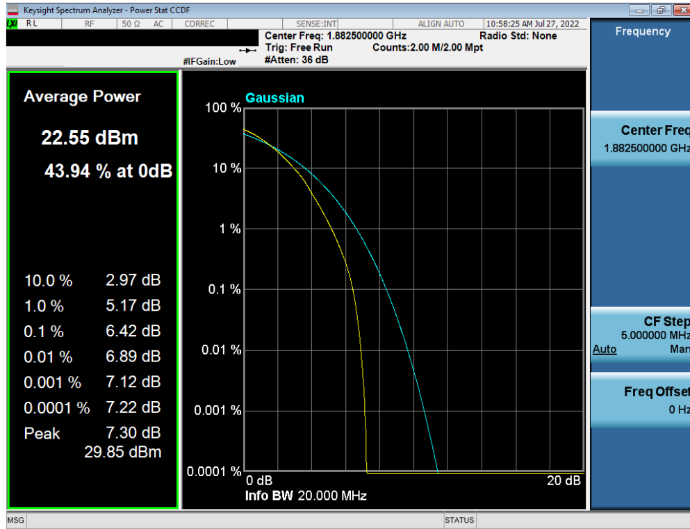
Plot 7-206. PAR Plot (LTE Band 25 - 20MHz 64-QAM - Full RB Configuration)
