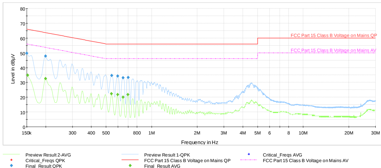
Plot 7-44. AC Line-Conducted Test Plot- Ch.39 (N, with AC/DC Adapter)
