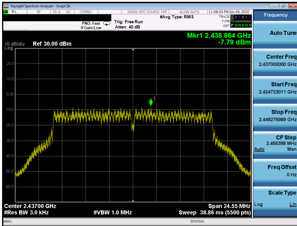
Plot 7-40. Power Spectral Density Plot CDD CORE 1 (802.11g – Ch. 6)
