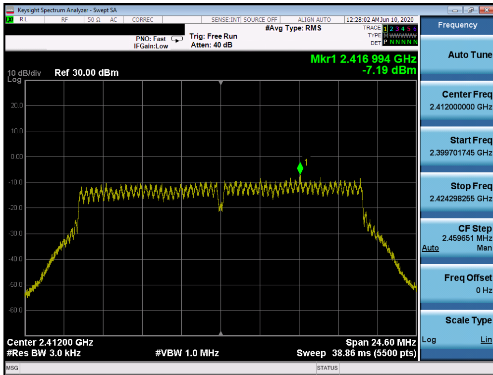
Plot 7-34. Power Spectral Density Plot SISO CORE 1 (802.11n (2.4GHz) – Ch. 1)
