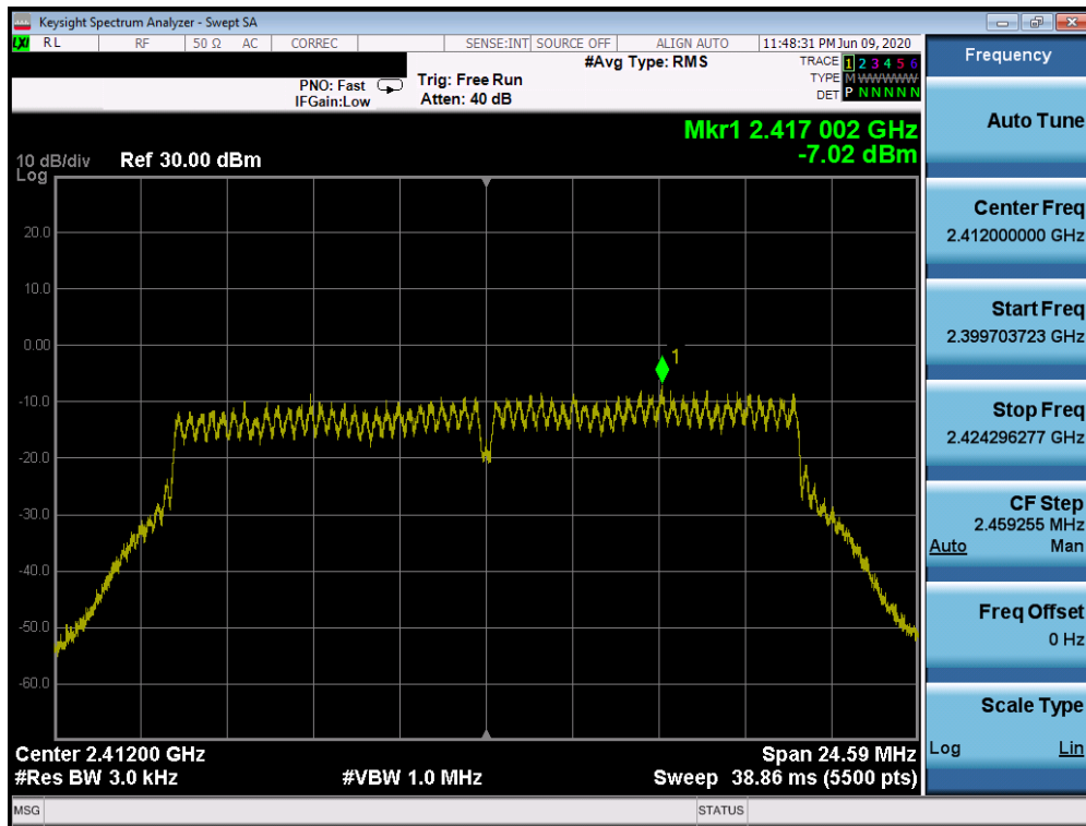
Plot 7-25. Power Spectral Density Plot SISO CORE 0 (802.11n (2.4GHz) - Ch. 1)
