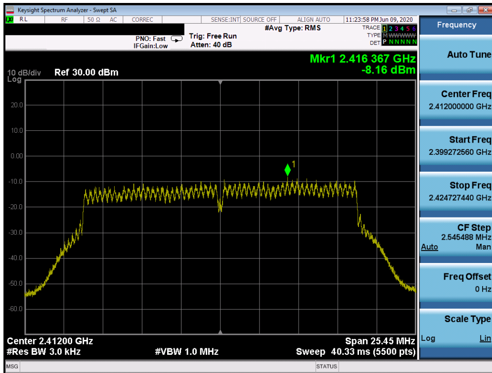
Plot 7-44. Power Spectral Density Plot CDD CORE 1 (802.11n (2.4GHz) – Ch. 1)
