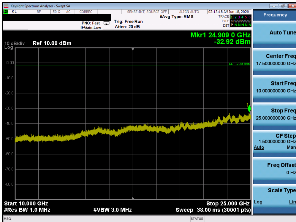
Plot 7-20. Conducted Spurious Plot (Bluetooth (LE), 1Mbps, ePA – Ch. 39)
