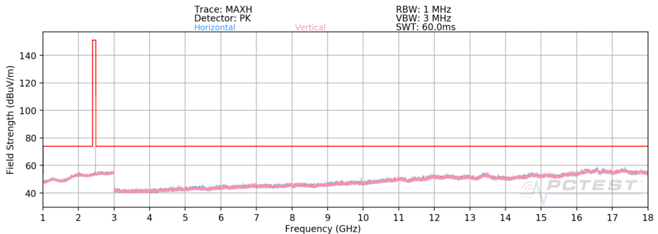
Plot 7-23. Radiated Spurious Emissions Above 1GHz (1Mbps, ePA – Ch. 39)
