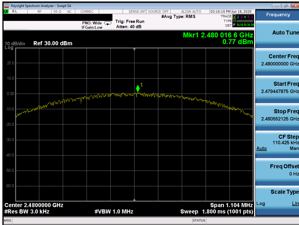
Plot 7-9. Power Spectral Density Plot (Bluetooth (LE), 1Mbps, ePA – Ch. 39)
