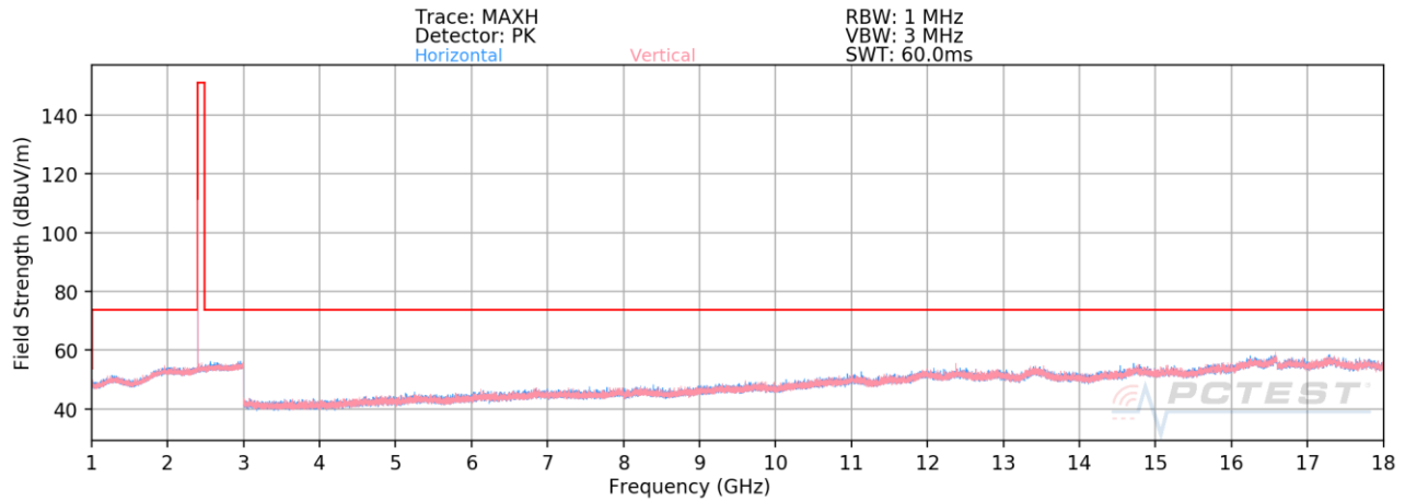
Plot 7-21. Radiated Spurious Emissions Above 1GHz (1Mbps, ePA – Ch. 0)
