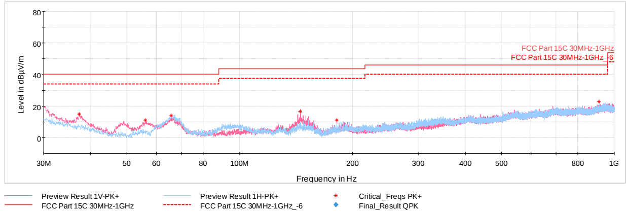
Plot 7-28. Radiated Spurious Emissions below 1GHz (1Mbps, ePA Ch.19 with AC/DC Adapter)
