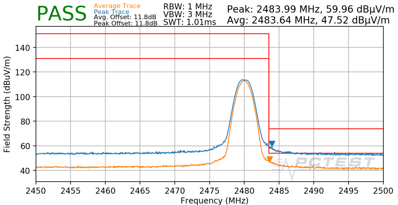
Plot 7-27. Radiated Restricted Upper Band Edge Measurement (Average & Peak)
