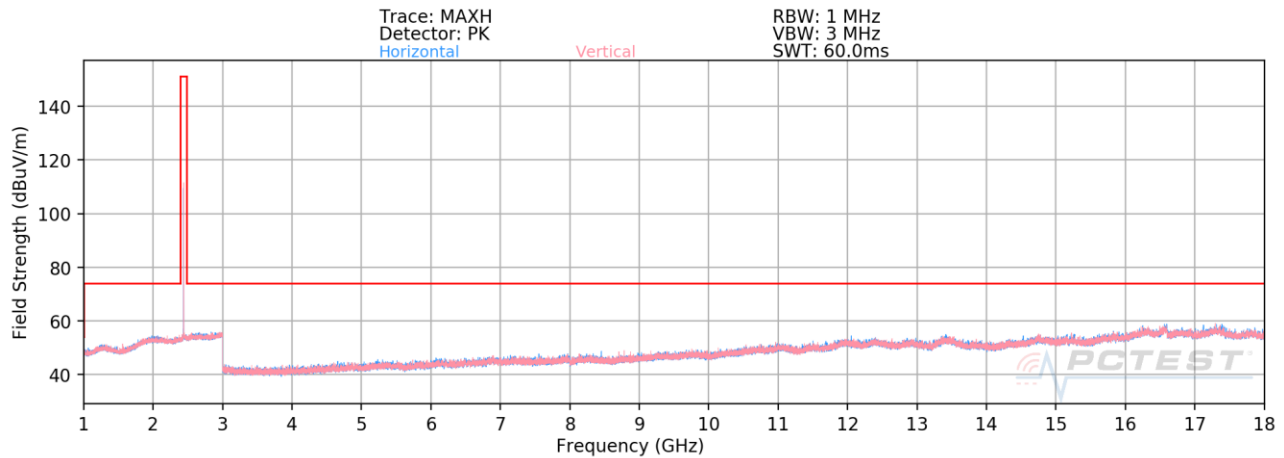
Plot 7-22. Radiated Spurious Emissions Above 1GHz (1Mbps, ePA – Ch. 19)
