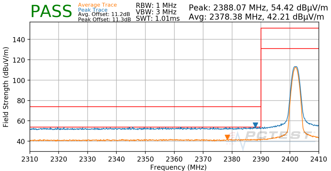
Plot 7-26. Radiated Restricted Lower Band Edge Measurement (Average & Peak)
