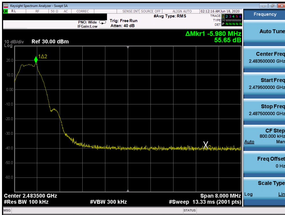
Plot 7-14. Band Edge Plot (Bluetooth (LE), ePA – Ch. 39)
