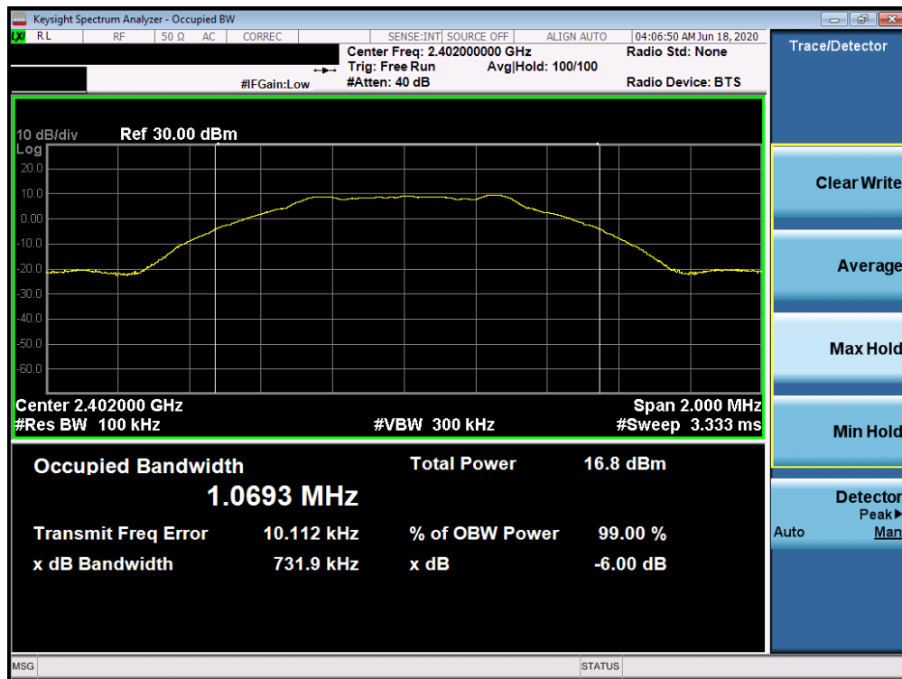
Plot 7-4. 6dB Bandwidth Plot (Bluetooth (LE), 1Mbps, iPA – Ch. 1)
