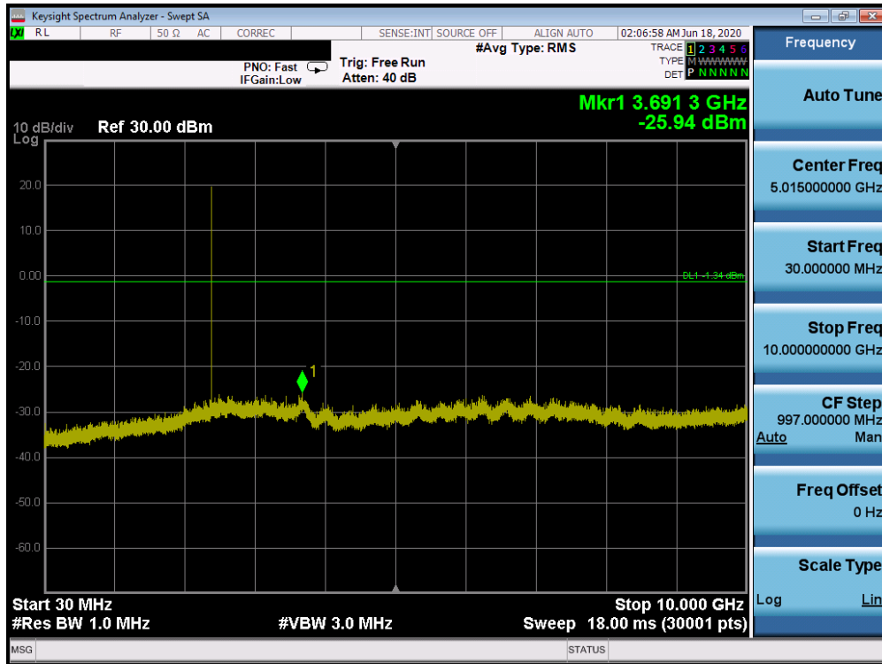
Plot 7-15. Conducted Spurious Plot (Bluetooth (LE), 1Mbps, ePA – Ch. 0)
