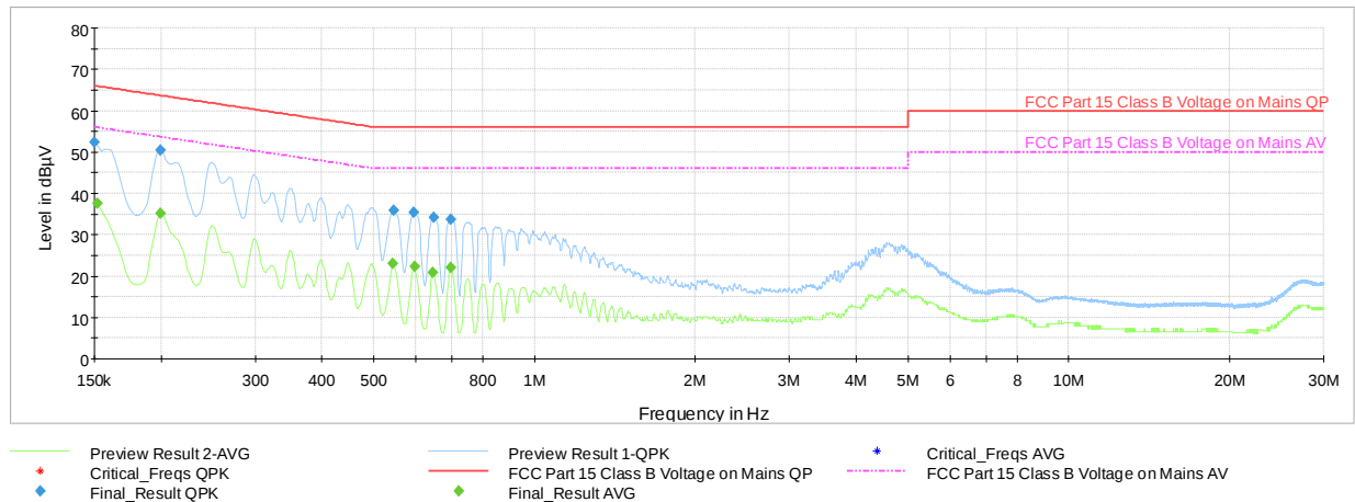
Plot 7-29. AC Line Conducted Plot with Bluetooth LE (L1 – 1Mbps, ePA, Ch.19, with AC/DC Adapter)
