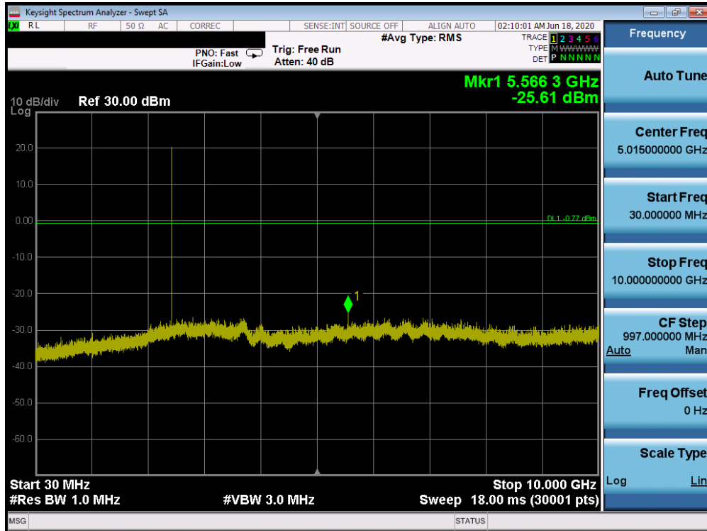
Plot 7-17. Conducted Spurious Plot (Bluetooth (LE), 1Mbps, ePA – Ch. 19)
