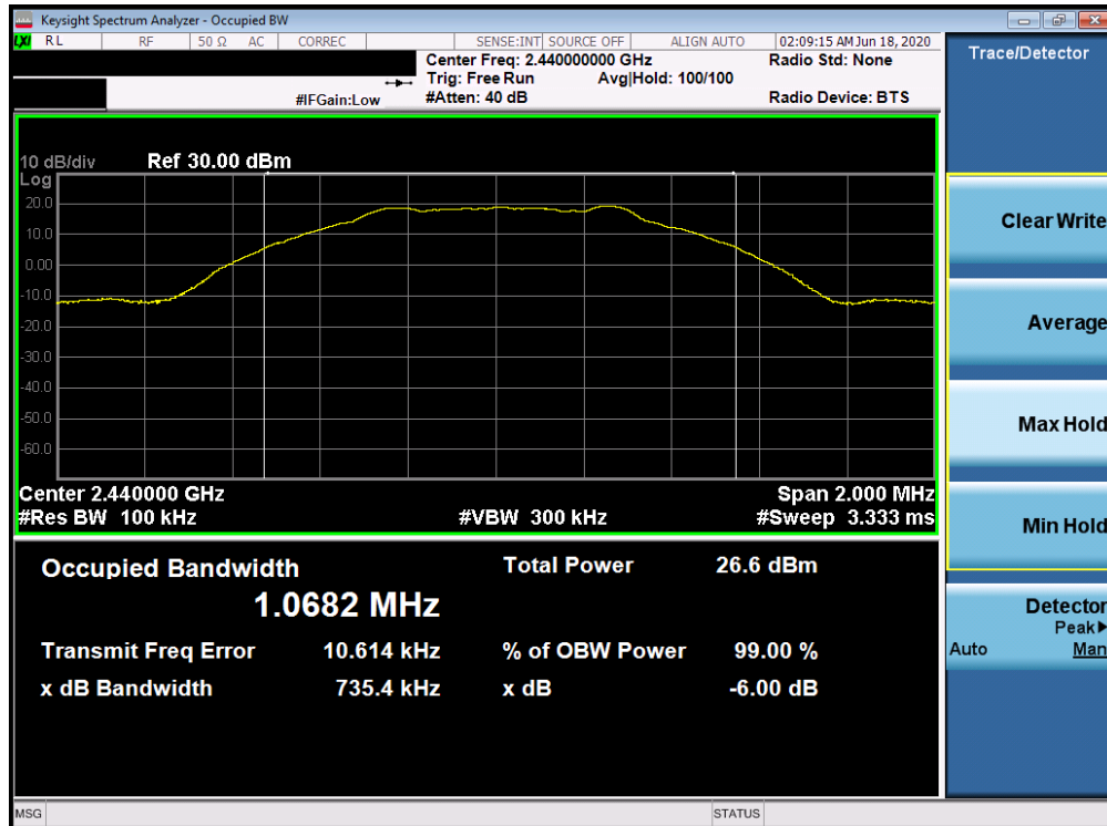
Plot 7-2. 6dB Bandwidth Plot (Bluetooth (LE), 1Mbps, ePA – Ch. 19)
