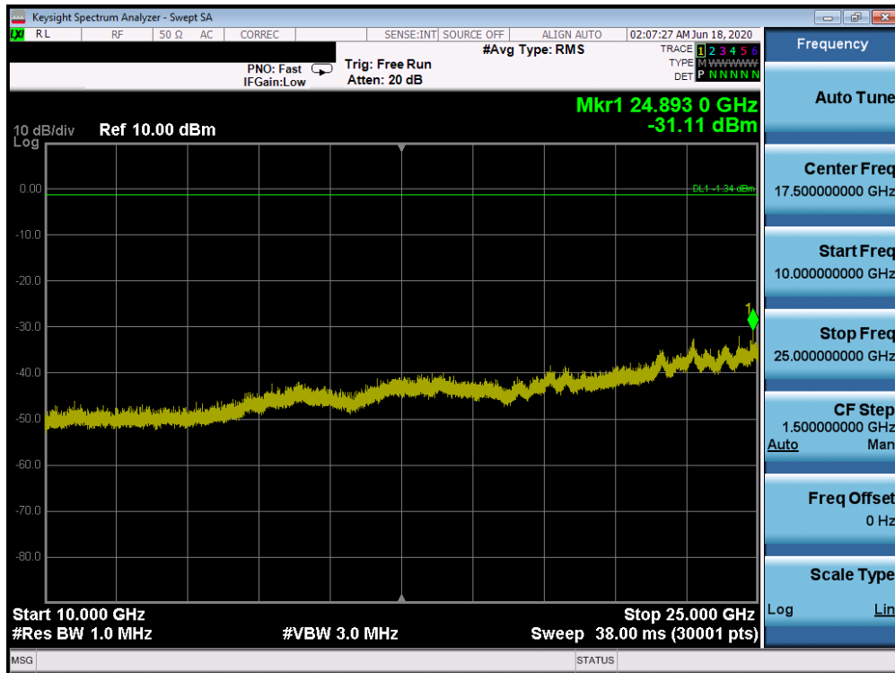
Plot 7-16. Conducted Spurious Plot (Bluetooth (LE), 1Mbps, ePA – Ch. 0)
