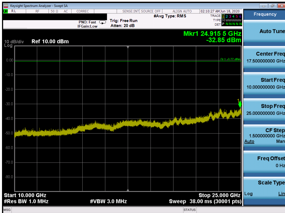
Plot 7-18. Conducted Spurious Plot (Bluetooth (LE), 1Mbps, ePA – Ch. 19)
