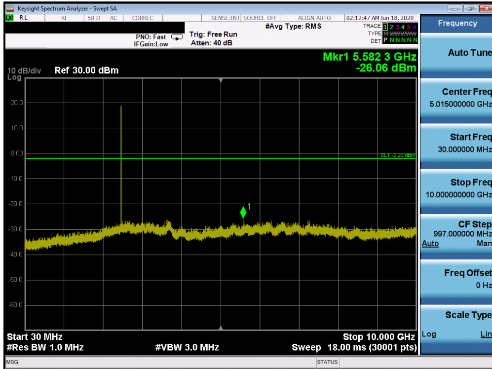
Plot 7-19. Conducted Spurious Plot (Bluetooth (LE), 1Mbps, ePA – Ch. 39)
