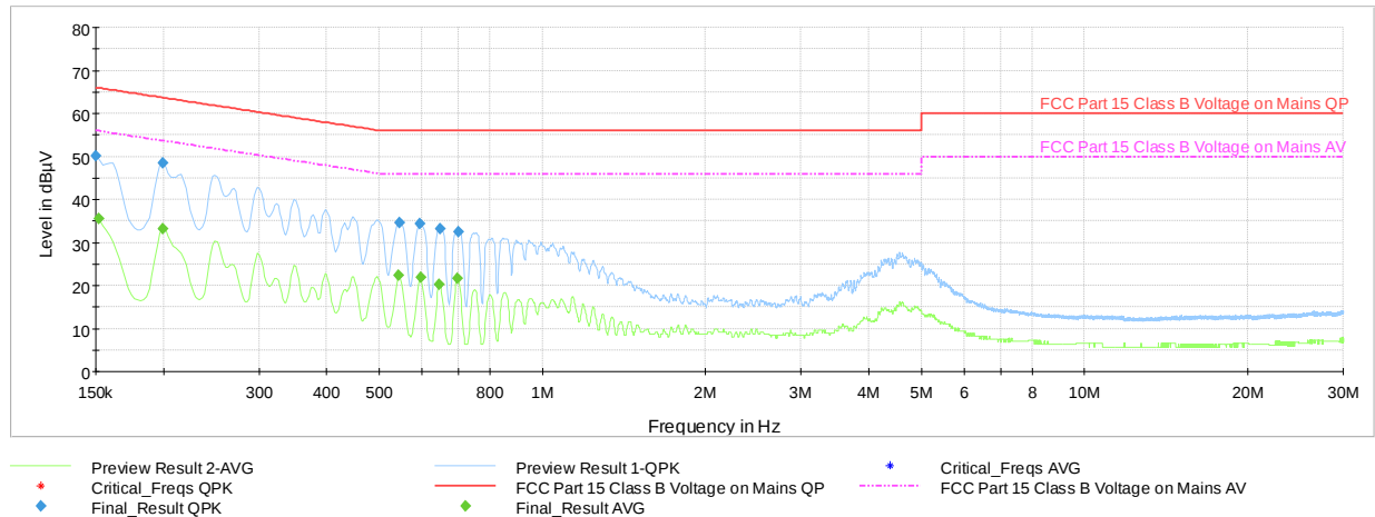
Plot 7-30. AC Line Conducted Plot with Bluetooth LE (N – 1Mbps, ePA, Ch.19 with AC/DC Adapter)
