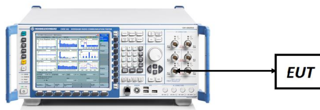
Figure 7-5. ERP/EIRP Measurement Setup
