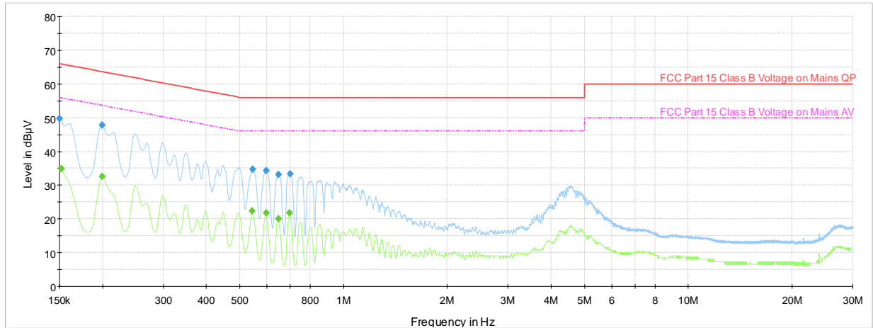
Plot 7-44. AC Line-Conducted Test Plot- Ch.39 (N, with AC/DC Adapter)
