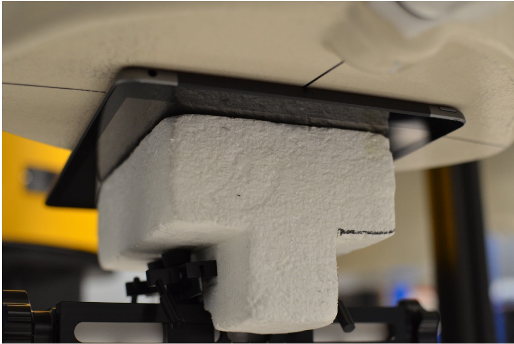
SAR Test Setup Photo 1: Back Side at 0.0 cm – Antenna C/Antenna D
