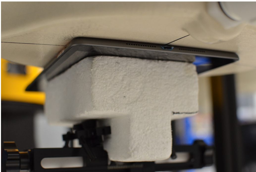
SAR Test Setup Photo 2: Back Side at 0.0 cm – Antenna A/Antenna B
