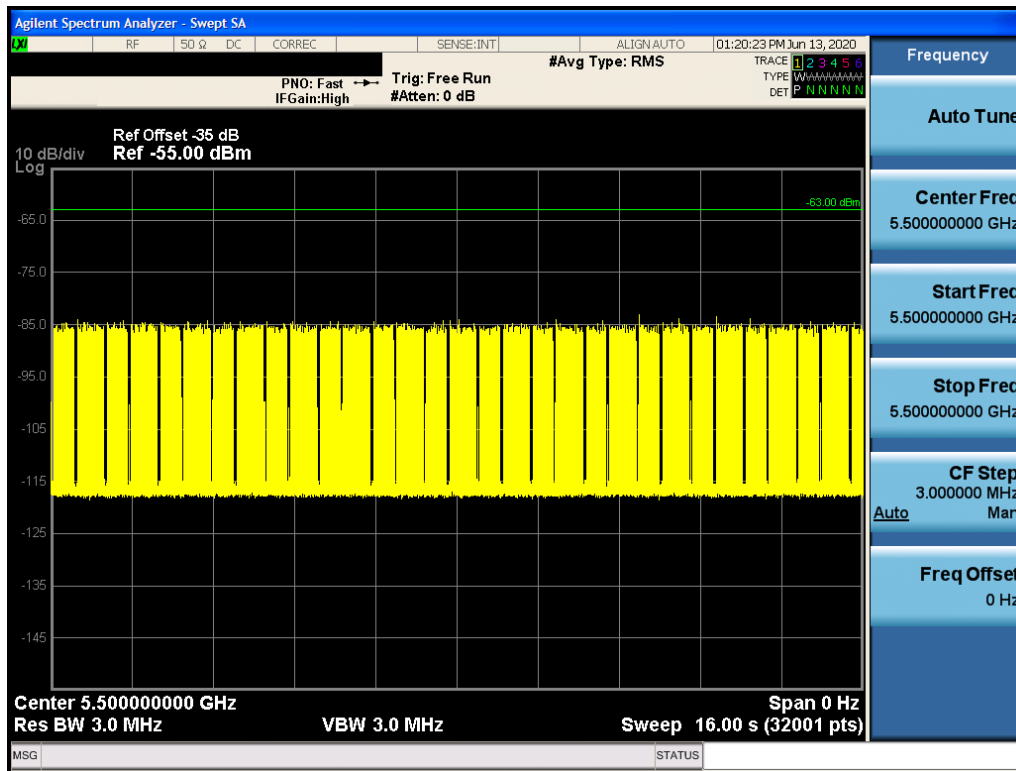
Figure 9-13. 5500MHz - Channel Loading - Mode 3 (20MHz)
