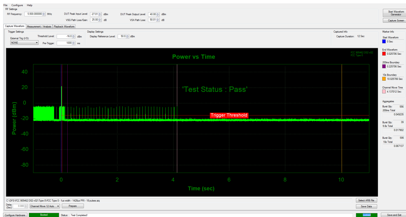
Figure 9-25. 5500MHz - Channel Move/ Closing Transmission Time - Mode 1 (20 MHz)
