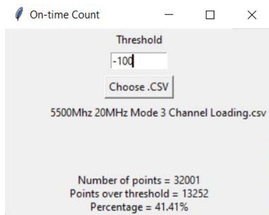
Figure 9-14. 5500MHz - Channel Loading Calculation - Mode 3 (20MHz)
