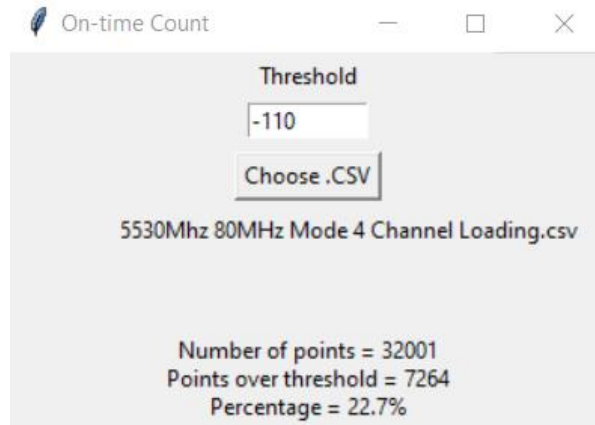
Figure 9-24. 5530MHz - Channel Loading Calculation - Mode 4 (80MHz)
