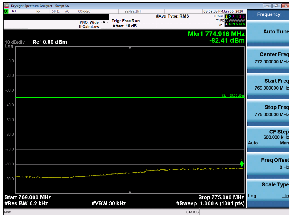
Plot 7-36. Lower Extended Band Edge Plot (Band 14 - 10MHz QPSK - Full RB Configuration)
