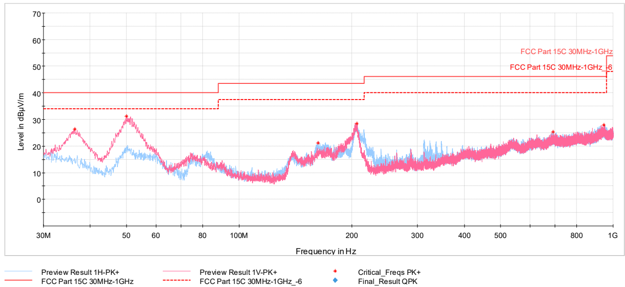
Plot 7-80. Radiated Spurious Emissions below 1GHz TxBF (GFSK ePA – Ch.0, with AC/DC Adapter)
