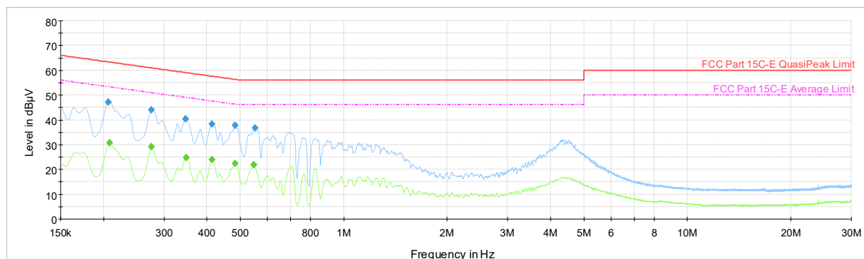
Plot 7-81. AC Line-Conducted Test Plot TxBF (L1, GFSK ePA – Ch.0, with AC/DC Adapter)
