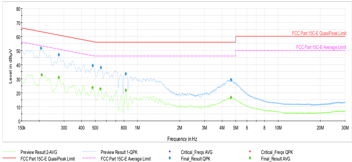
Plot 7-106. AC Line Conducted Plot with Bluetooth HDR (N, 4Mbps ePA - Ch.38 with Laptop)
