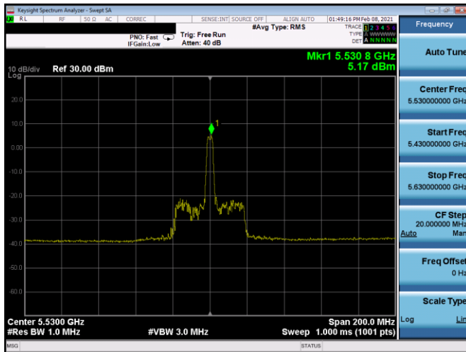
Plot 7-283. PSD CDD Antenna 5b (80MHz BW 11ax Index 18 – RU26 – Ch.106)
