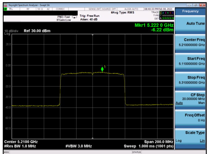
Plot 7-336. ISED PSD CDD Antenna 4b (80MHz BW 11ax – RU996 – Ch.42)
