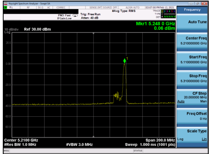
Plot 7-334. ISED PSD SDM Antenna 4b (80MHz BW 11ax Index 36 – RU26 – Ch.42)
