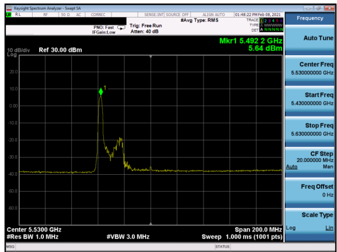
Plot 7-281. PSD CDD Antenna 5b (80MHz BW 11ax Index 0 – RU26 – Ch.106)
