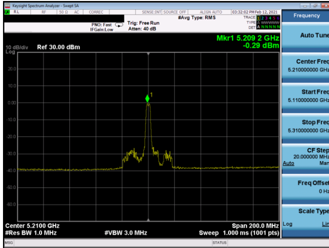
Plot 7-331. ISED PSD SDM Antenna 5b (80MHz BW 11ax Index 18 – RU26 – Ch.42)
