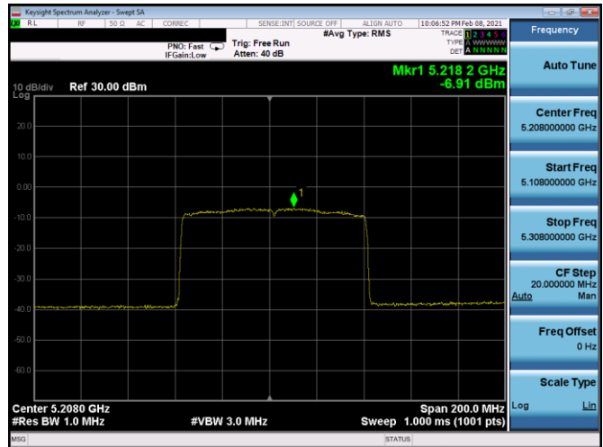
Plot 7-335. ISED PSD CDD Antenna 5b (80MHz BW 11ax – RU996 – Ch.42)
