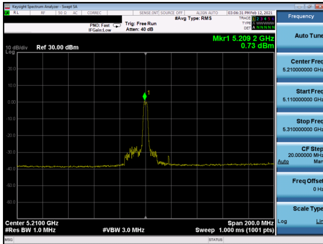
Plot 7-332. ISED PSD SDM Antenna 4b (80MHz BW 11ax Index 18 – RU26 – Ch.42)
