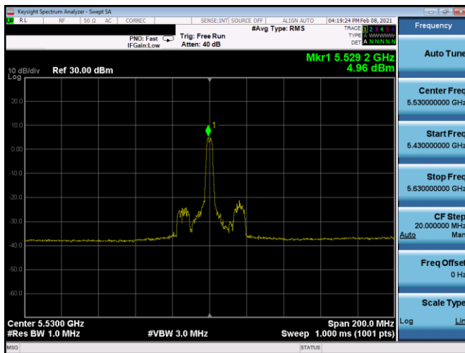
Plot 7-284. PSD CDD Antenna 4b (80MHz BW 11ax Index 18 – RU26 – Ch.106)
