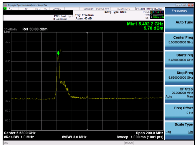
Plot 7-282. PSD CDD Antenna 4b (80MHz BW 11ax Index 0 – RU26 – Ch.106)
