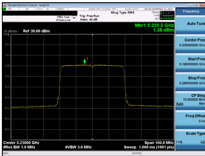
Plot 7-327. ISED PSD SDM Antenna 5b (40MHz BW 11ax - RU484 - Ch.46)
