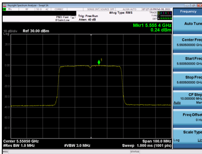
Plot 7-279. PSD CDD Antenna 5b (40MHz BW 11ax – RU484 – Ch.110)
