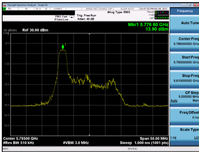
Plot 7-290. PSD CDD Antenna 4b (20MHz BW 11ax Index 0 – RU26 – Ch.157)
