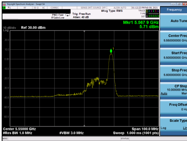
Plot 7-277. PSD CDD Antenna 5b (40MHz BW 11ax Index 17 – RU26 – Ch.110)
