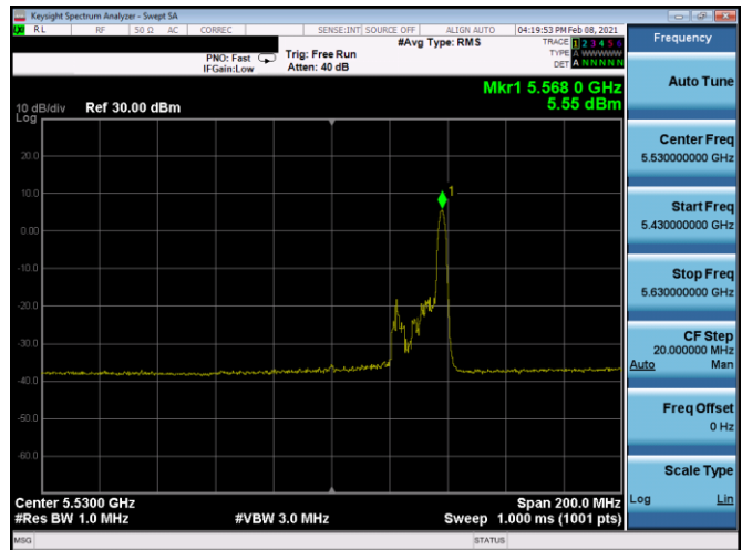
Plot 7-286. PSD CDD Antenna 4b (80MHz BW 11ax Index 36 – RU26 – Ch.106)
