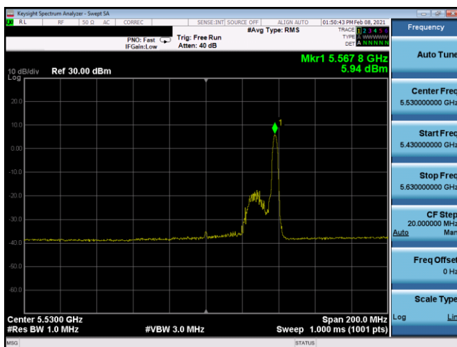
Plot 7-285. PSD CDD Antenna 5b (80MHz BW 11ax Index 36 – RU26 – Ch.106)
