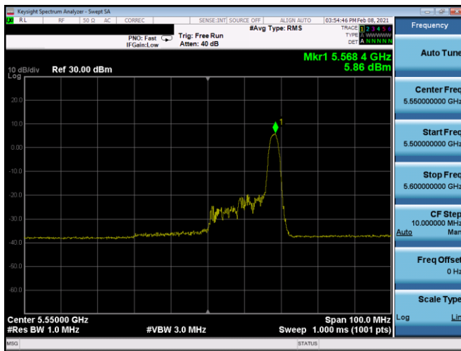
Plot 7-278. PSD CDD Antenna 4b (40MHz BW 11ax Index 17 – RU26 – Ch.110)
