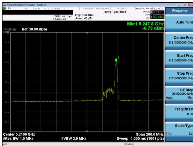
Plot 7-333. ISED PSD SDM Antenna 5b (80MHz BW 11ax Index 36 – RU26 – Ch.42)
