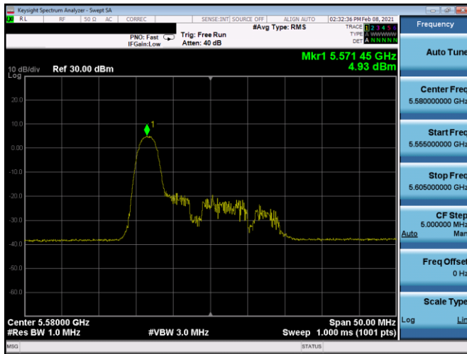
Plot 7-266. PSD CDD Antenna 4b (20MHz BW 11ax Index 0 – RU26 – Ch.116)
