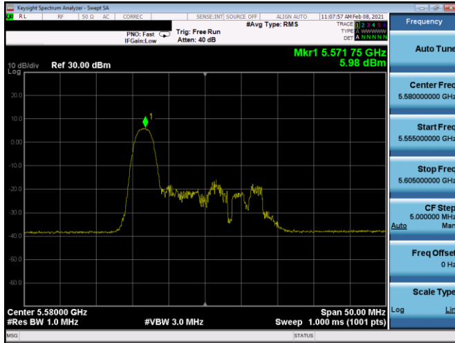
Plot 7-265. PSD CDD Antenna 5b (20MHz BW 11ax Index 0 – RU26 – Ch.116)
