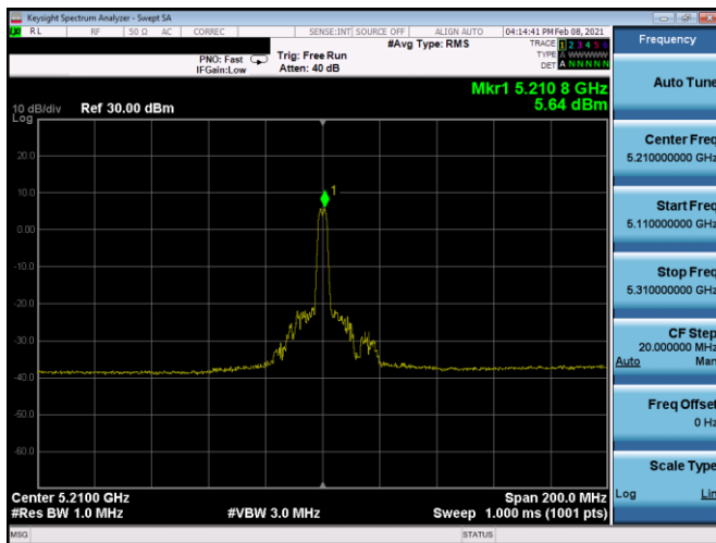
Plot 7-236. PSD CDD Antenna 4b (80MHz BW 11ax Index 18 – RU26 – Ch.42)
