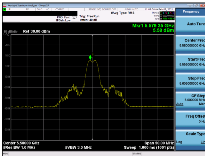
Plot 7-267. PSD CDD Antenna 5b (20MHz BW 11ax Index 4 – RU26 – Ch.116)
