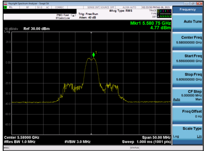
Plot 7-268. PSD CDD Antenna 4b (20MHz BW 11ax Index 4 – RU26 – Ch.116)
