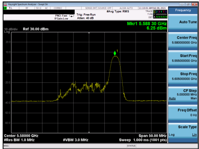
Plot 7-269. PSD CDD Antenna 5b (20MHz BW 11ax Index 8– RU26 – Ch.116)
