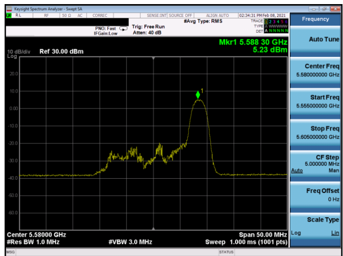
Plot 7-270. PSD CDD Antenna 4b (20MHz BW 11ax Index 8– RU26 – Ch.116)
