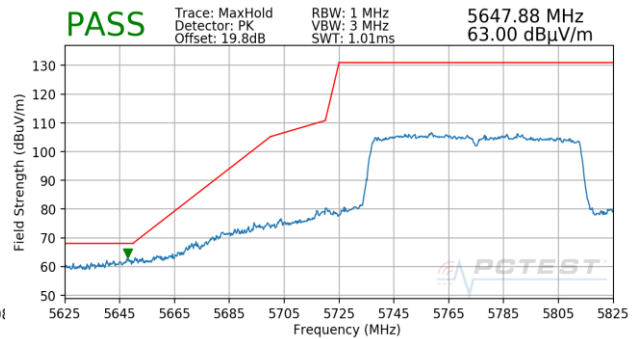
Plot 7-913. Antenna 4b (Pk, Ch.155, 802.11ac, MCS5)
